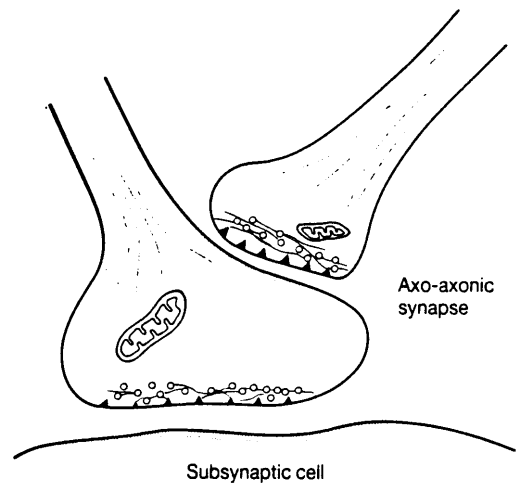
Figure 15.24 Axo-axonic synapse.
