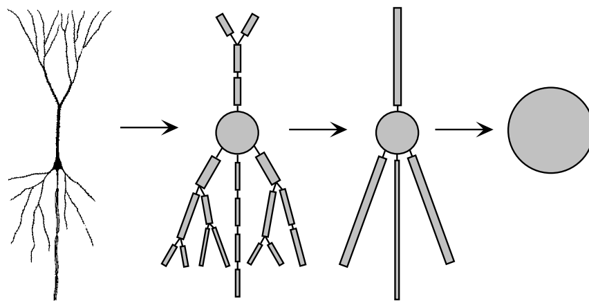
Figure 6.15: A sequence of approximations of the structure of a neuron. The neuron is represented by a variable number of discrete compartments each representing a region that is described by a single membrane potential. The connectors between compartments represent resistive couplings. The simplest description is the single-compartment model furthest to the right. (Neuron diagram from Haberly, 1990.)
