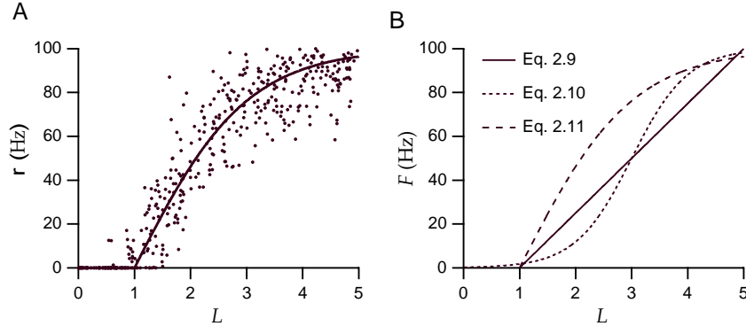
Figure 2.2: A) A graphical procedure for determining static nonlinearities. The linear estimate L and the actual firing rate r are plotted (solid points) and fit by the function F(L) (solid line). B) Different static nonlinearities used in estimating neural responses. L is dimensionless, and equations 2.9, 2.10, and 2.11 have been used with G = 25 Hz, L_0 = 1 , L_{1/2} = 3 , r_{\max} = 100 Hz, g_1 = 2 , and g_2 = 1/2 .
