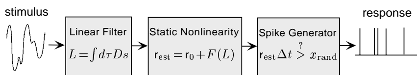
Figure 2.3: Simulating spiking responses to stimuli. The integral of the stimulus s times the optimal kernel D is first computed. The estimated firing rate is the background rate r_0 plus a nonlinear function of the output of the linear filter calculation. Finally, the estimated firing rate is used to drive a Poisson process that generates spikes.
