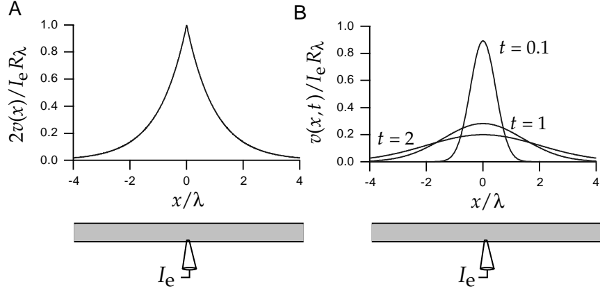
Figure 6.7: The potential for current injection at the point x = 0 along an infinite cable. A) Static solution for a constant electrode current. The potential decays exponentially away from the site of current injection. B) Time-dependent solution for a \delta function pulse of current. The potential is described by a Gaussian function centered at the site of current injection that broadens and shrinks in amplitude over time.
