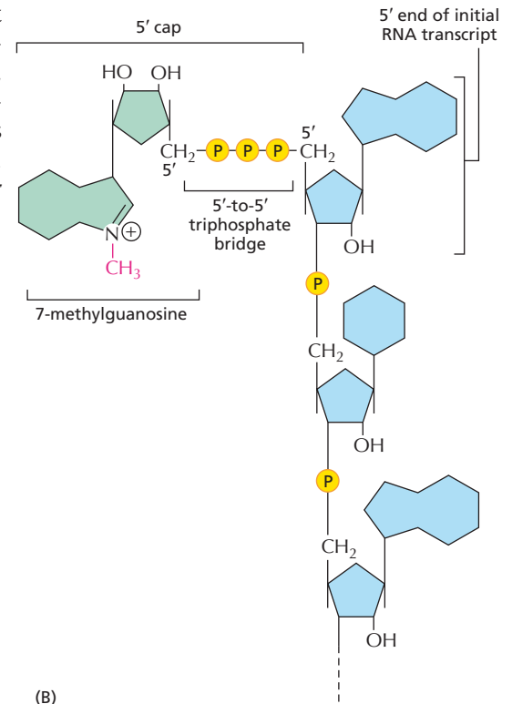
Figure 7-16 Eukaryotic pre-mRNA molecules are modified by capping and polyadenylation. (A) A eukaryotic mRNA has a cap at the 5' end and a poly-A tail at the 3' end. Note that not all of the RNA transcript shown codes for protein. (B) The structure of the 5' cap. Many eukaryotic mRNA caps carry an additional modification: the 2'-hydroxyl group on the second ribose sugar in the mRNA is methylated (not shown).
