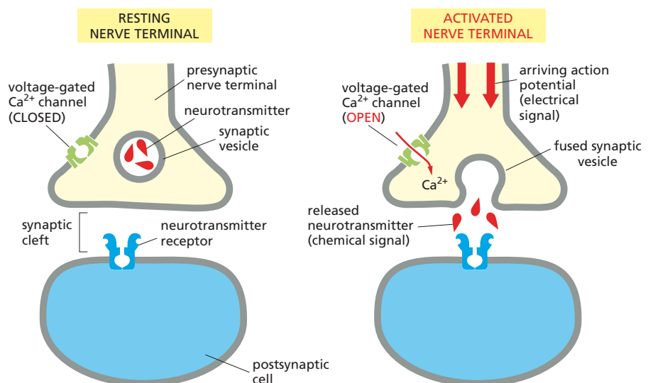
Figure 12-39 An electrical signal is converted into a secreted chemical signal at a nerve terminal. When an action potential reaches a nerve terminal, it opens voltage-gated \text{Ca}^{2+} channels in the plasma membrane, allowing \text{Ca}^{2+} to flow into the terminal. The increased \text{Ca}^{2+} in the nerve terminal stimulates the synaptic vesicles to fuse with the plasma membrane, releasing their neurotransmitter into the synaptic cleft—a process called exocytosis (discussed in Chapter 15).
