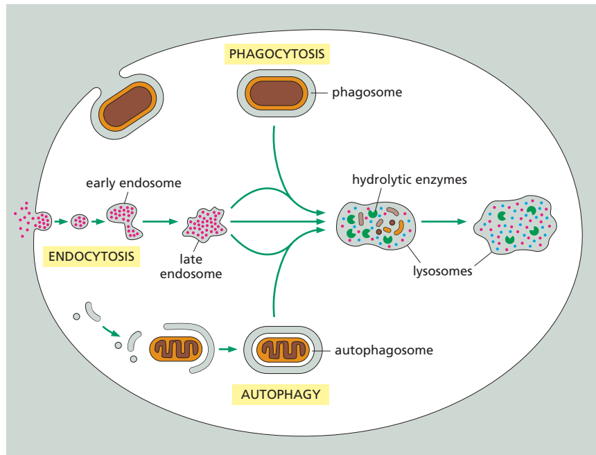
Figure 15–36 Materials destined for degradation in lysosomes follow different pathways to the lysosome. Each pathway leads to the intracellular digestion of materials derived from a different source. Early endosomes, phagosomes, and autophagosomes can fuse with either lysosomes or late endosomes, both of which contain acid-dependent hydrolytic enzymes.
