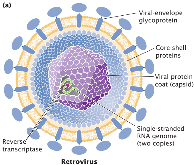
Retrovirus
