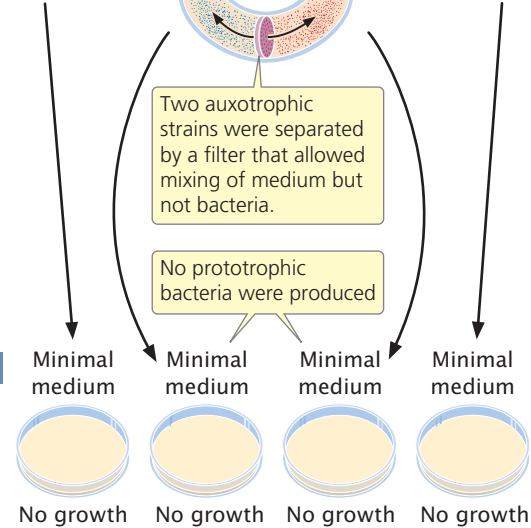
8.9 Davis's U-tube experiment.
