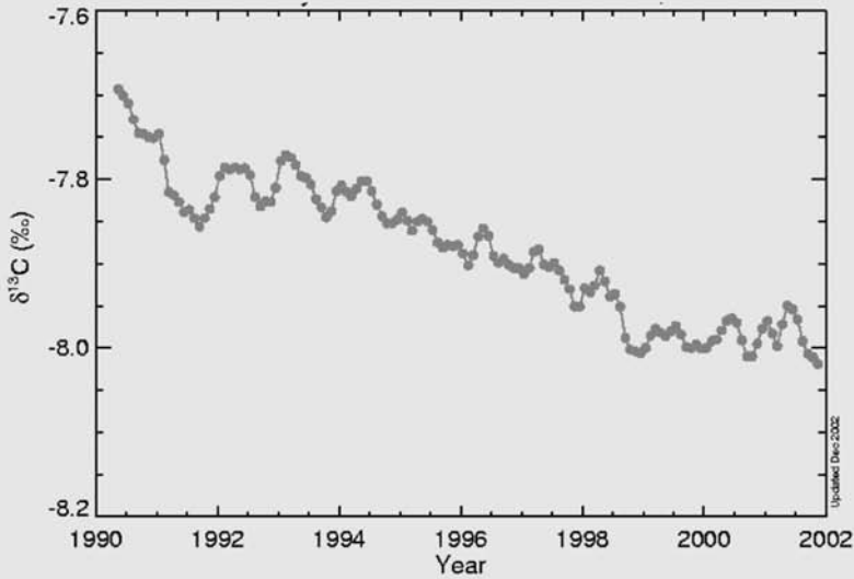
Figure 7.14. “Lightening” of the isotope composition of atmospheric \text{CO}_2 over time, measured from a monitoring station at the South Pole. CSIRO monthly mean flask data—South Pole, Antarctica. Source: CDIAC.
