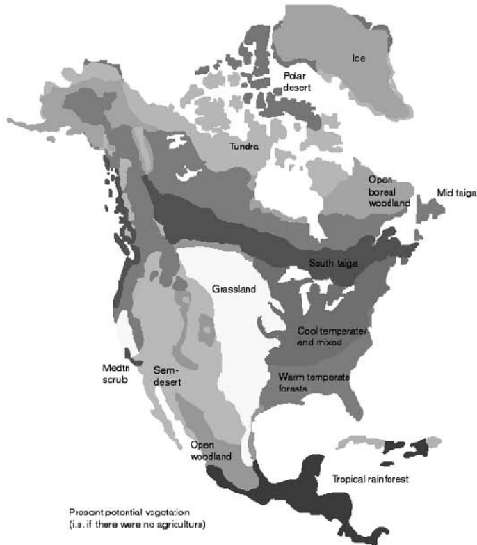
Figure 3.3. Biome distributions of Europe, North America at the present day (a, b) and last glacial maximum (22,000–14,000 ^{14}\text{C} years ago) (c, d). Part (d) is a map of the result of a collaboration between the author J. Adams, A. Beaudoin, O. Davis, P. and H. Delcourt, and P. Richard Source: Author.
