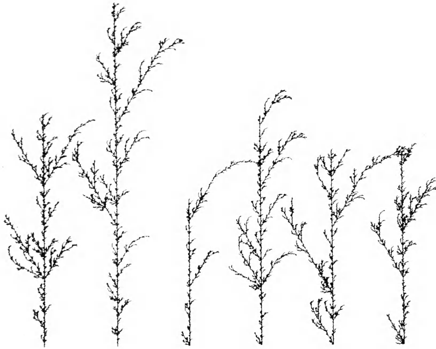
Figure 1.27: Stochastic branching structures
