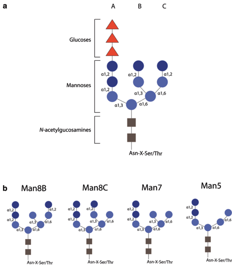
Fig. 11.1 Structure of an N-linked glycan. a Illustration of an asparagine-linked glycan composed of two N-acetylglucosamines (brown squares), nine mannoses (dark and light blue circles), and three glucoses (red triangles). The different branches are labeled A, B, and C. \alpha(1,2) -linked mannoses are shown in dark blue while the \alpha(1,6) -linked mannoses are in light blue. b Glycoforms generated as a result of glycan trimming in the endoplasmic reticulum (ER)
