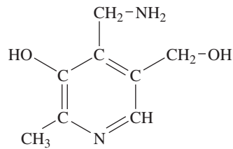
Pyridoxamine
