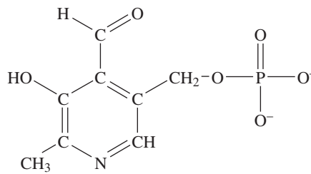
Pyridoxal phosphate
