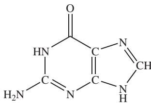
Guanine (G)
