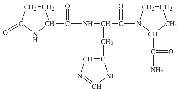
Thyrotropin-releasing factor
