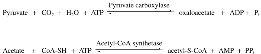
Figure 6-5: Reactions illustrating the action of the ligases pyruvate carboxylase and acetyl-CoA synthetase.
