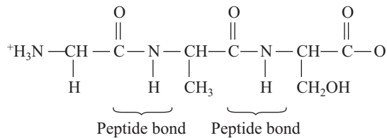
Figure 4-12: A tripeptide.
