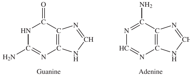
Figure 15-9: The purines.
