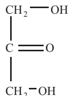
Dihydroxyacetone
