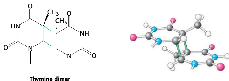
FIGURE 28.35 Cross-linked dimer of two thymine bases. Ultraviolet light induces cross-links between adjacent pyrimidines along one strand of DNA.
