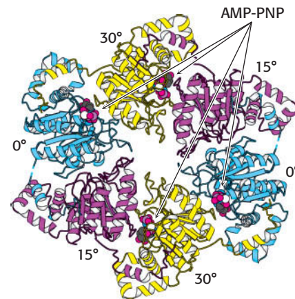
FIGURE 28.13 Helicase asymmetry. The structure of the T7 helicase complexes with the ATP analog AMP-PNP is shown. The three classes of helicase subunits are shown in blue, red, and yellow. The rotation relative to the plane of the hexamer is shown for each subunit. Notice that only four of the subunits, those shown in blue and yellow, bind AMP-PNP. [Drawn from 1E0K.pdb.]
