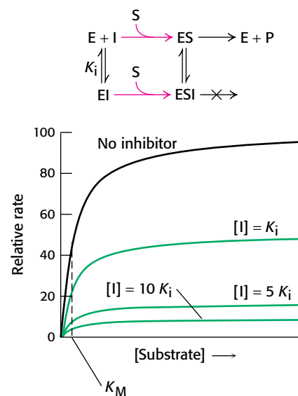
FIGURE 8.18 Kinetics of a noncompetitive inhibitor. The reaction pathway shows that the inhibitor binds both to free enzyme and to an enzyme–substrate complex. Consequently, as with uncompetitive competition, V_{\text{max}} cannot be attained. In pure noncompetitive inhibition, K_M remains unchanged, and so the reaction rate increases more slowly at low substrate concentrations than is the case for uncompetitive competition.
