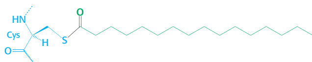
S-Palmitoylcysteine
