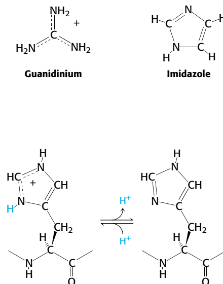
FIGURE 2.10 Histidine ionization. Histidine can bind or release protons near physiological pH.
