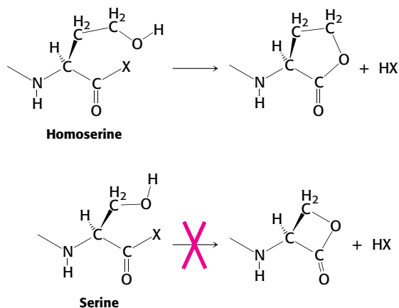
FIGURE 2.12 Undesirable reactivity in amino acids. Some amino acids are unsuitable for proteins because of undesirable cyclization. Homoserine can cyclize to form a stable, five-membered ring, potentially resulting in peptide-bond cleavage. The cyclization of serine would form a strained, four-membered ring and is thus disfavored. X can be an amino group from a neighboring amino acid or another potential leaving group.
