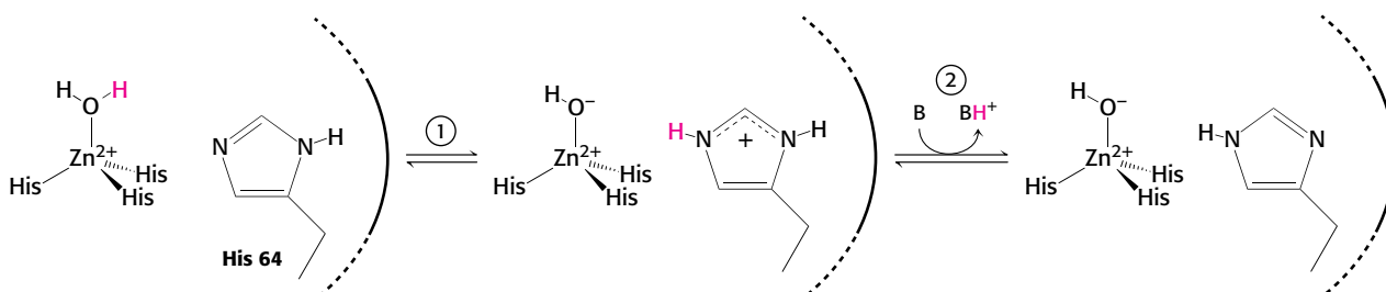
FIGURE 9.30 Histidine proton shuttle. (1) Histidine 64 abstracts a proton from the zinc-bound water molecule, generating a nucleophilic hydroxide ion and a protonated histidine. (2) The buffer (B) removes a proton from the histidine, regenerating the unprotonated form.
