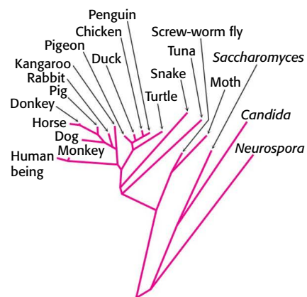
FIGURE 18.21 Evolutionary tree constructed from sequences of cytochrome c . Branch lengths are proportional to the number of amino acid changes that are believed to have occurred. [Information from Walter M. Fitch and Emanuel Margoliash.]
