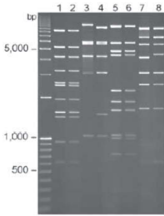
FIGURE 5.2 Gel-electrophoresis pattern of a restriction digest. This gel shows the fragments produced by cleaving DNA from two viral strains (odd- vs. even-numbered lanes) with each of four restriction enzymes. These fragments were made fluorescent by staining the gel with ethidium bromide. [Data from Carr et al., Emerging Infectious Diseases , www.cdc.gov/eid, 17(8), August 2011.]
