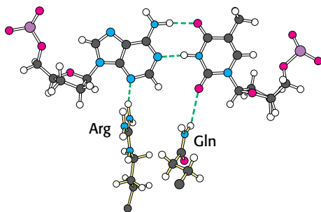
FIGURE 28.7 Minor-groove interactions. DNA polymerases donate two hydrogen bonds to base pairs in the minor groove. Hydrogen-bond acceptors are present in these two positions for all Watson–Crick base pairs, including the A—T base pair shown.
