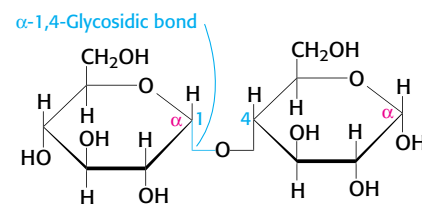
FIGURE 11.11 Maltose, a disaccharide.
