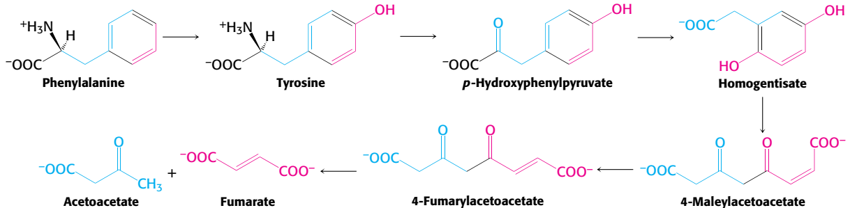
FIGURE 23.27 Phenylalanine and tyrosine degradation. The pathway for the conversion of phenylalanine into acetoacetate and fumarate.
