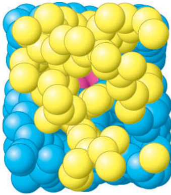
FIGURE 24.16 Substrate channeling. A 25-Å tunnel runs from the active site of the \alpha subunit of tryptophan synthase (yellow) to the PLP cofactor (red) in the active site of the \beta subunit (blue).
