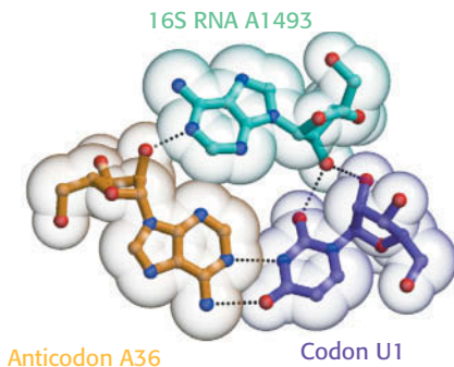
FIGURE 30.7 16S rRNA monitors base-pairing between the codon and the anticodon. Adenine 1493, one of three universally conserved bases in 16S rRNA, forms hydrogen bonds with the bases in both the codon and the anticodon only if the codon and anticodon are correctly paired. [Information from J. M. Ogle and V. Ramakrishnan, Annu. Rev. Biochem. 74: 129–177, 2005, Fig. 2a.]
