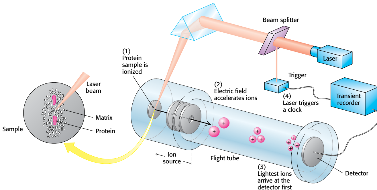
FIGURE 3.27 MALDI-TOF mass spectrometry. (1) The protein sample, embedded in an appropriate matrix, is ionized by the application of a laser beam. (2) An electric field accelerates the ions through the flight tube toward the detector. (3) The lightest ions arrive first. (4) The ionizing laser pulse also triggers a clock that measures the time of flight (TOF) for the ions. [Information from J. T. Watson, Introduction to Mass Spectrometry , 3d ed. (Lippincott-Raven, 1997), p. 279.]
