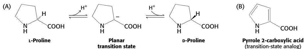
FIGURE 8.32 Inhibition by transition-state analogs. (A) The isomerization of L-proline to D-proline by proline racemase proceeds through a planar transition state in which the \alpha -carbon atom is trigonal rather than tetrahedral. (B) Pyrrole 2-carboxylic acid, a transition-state analog because of its trigonal geometry, is a potent inhibitor of proline racemase.
