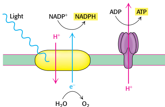
FIGURE 19.1 The light reactions of photosynthesis.
