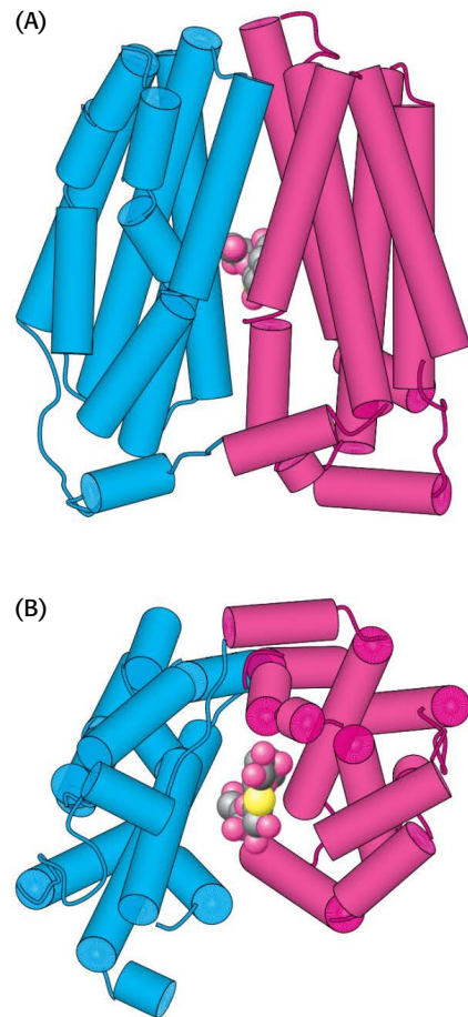
FIGURE 13.11 Structure of lactose permease with a bound lactose analog. The amino-terminal half of the protein is shown in blue and the carboxyl-terminal half in red. (A) Side view. (B) Bottom view (from inside the cell). Notice that the structure consists of two halves that surround the sugar and are linked to one another by only a single stretch of polypeptide. [Drawn from 1PV7.pdb.]
