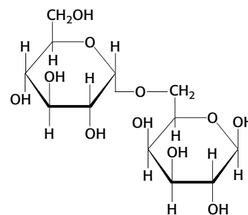
\alpha -Glucosyl-(1 \rightarrow 6)-galactose
