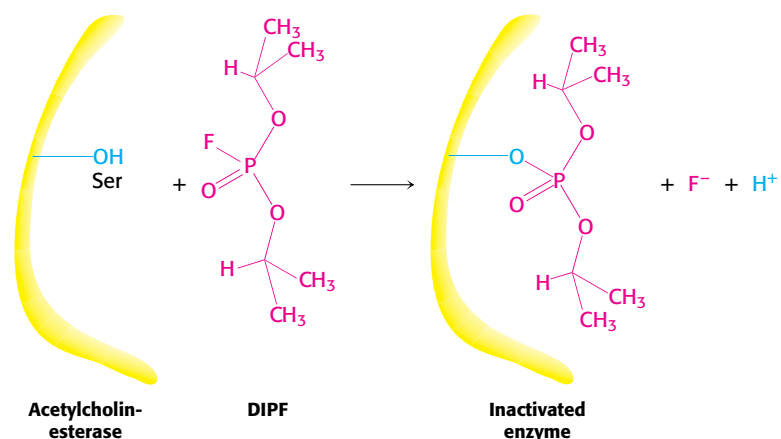
FIGURE 8.22 Enzyme inhibition by diisopropylphosphofluoridate (DIPF), a group-specific reagent. DIPF can inhibit an enzyme by covalently modifying a crucial serine residue.
