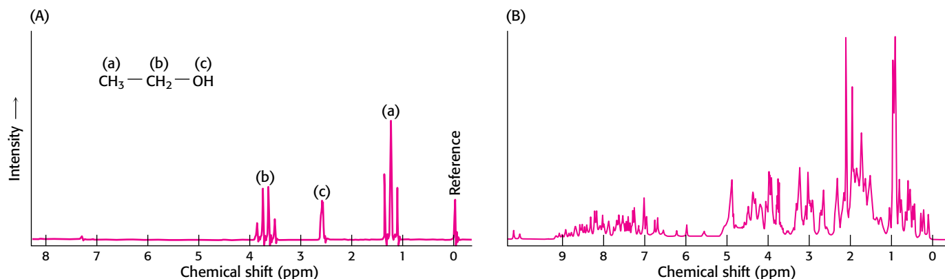
FIGURE 3.44 One-dimensional NMR spectra. (A) ^1\text{H} -NMR spectrum of ethanol ( \text{CH}_3\text{CH}_2\text{OH} ) shows that the chemical shifts for the hydrogen are clearly resolved. (B) ^1\text{H} -NMR spectrum of a 55 amino acid fragment of a protein having a role in RNA splicing shows a greater degree of complexity. A large number of peaks are present and many overlap. [(A) Data from C. Branden and J. Tooze, Introduction to Protein Structure (Garland, 1991), p. 280; (B) courtesy of Dr. Barbara Amann and Dr. Wesley McDermott.]
