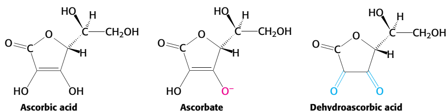
FIGURE 27.17 Forms of ascorbic acid (vitamin C). Ascorbate is the ionized form of vitamin C, and dehydroascorbic acid is the oxidized form of ascorbate.
