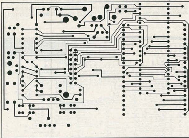
COMPONENT SIDE for the RadaAlert's display/beeper board.
