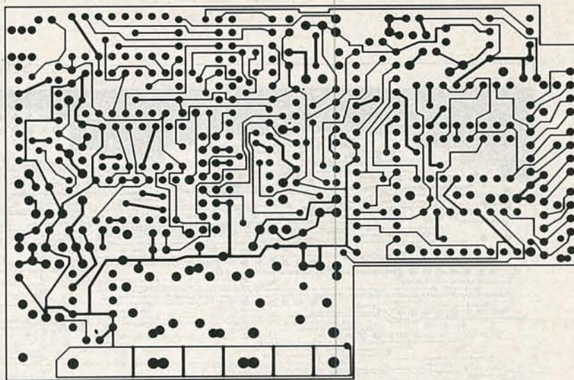
THE RADALERT main board component side.
