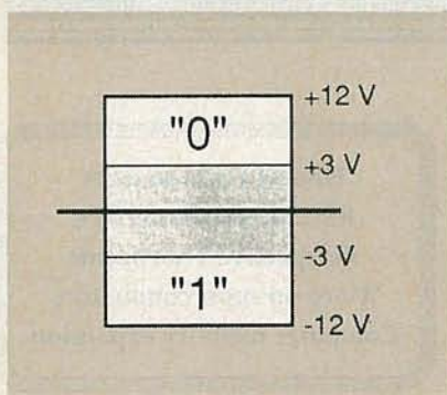
FIG. 2—HERE ARE the two logic levels that are needed for RS-232 communications. Note that a “negative-logic” convention is used.
