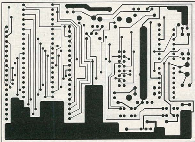
SOLDER SIDE for the display/beeper board.
