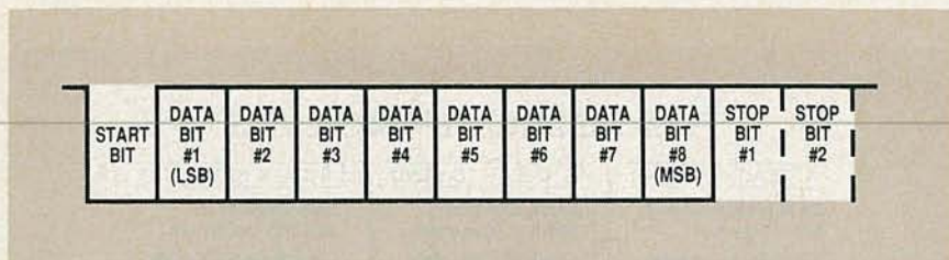
FIG. 3—MOST RS-232 SERIAL COMMUNICATIONS use this older “teletype” asynchronous code. Seven or eight data bits are normally used, with the least-significant bit always sent first. Any number of stop bits above the minimum can be sent between successive characters.
