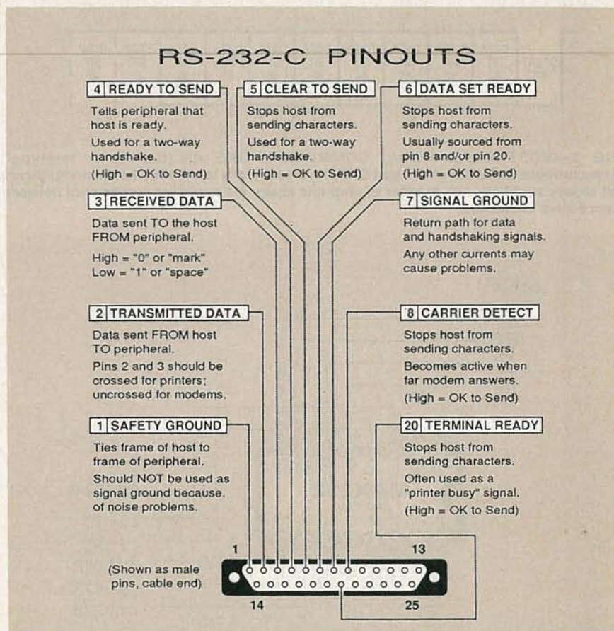
FIG. 1—HERE ARE SOME DETAILS on the RS-232 serial communications standard. Note that the data and handshake lines are often crossed for printers and uncrossed for modems.
