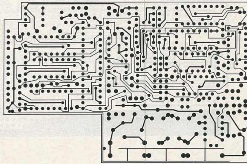
THE SOLDER SIDE of the main board.
