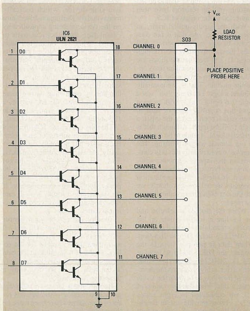
FIG. 4—THE DC OUTPUTS can be tested using the arrangement shown here.
