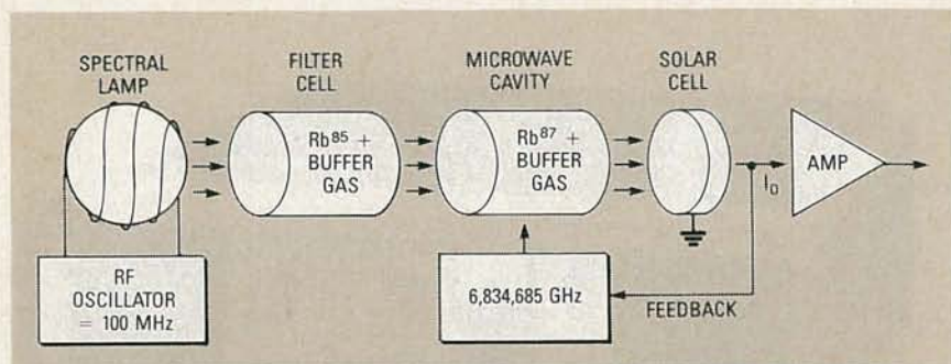
FIG. 6—FUNCTIONAL DIAGRAM of a Rubidium Frequency Standard.
