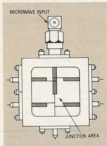
FIG. 9—THIS JOSEPHSON MICROSTRIPLINE JUNCTION is mounted in a metal enclosure. It is kept in a super-cooled environment enabling the Josephson junction to yield a very precise frequency-to-voltage transformation.
