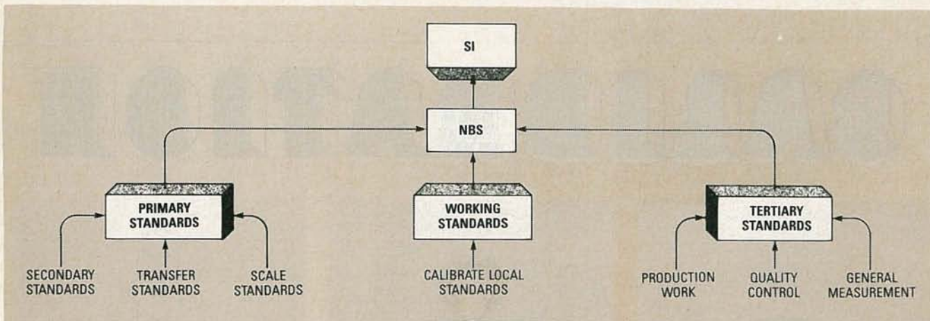
FIG. 1—AN INSTRUMENT IS CONSIDERED CALIBRATED only if its calibration is traceable to the National Bureau of Standards, and ultimately, to the physical units and constants of the International System of Units (SI).
