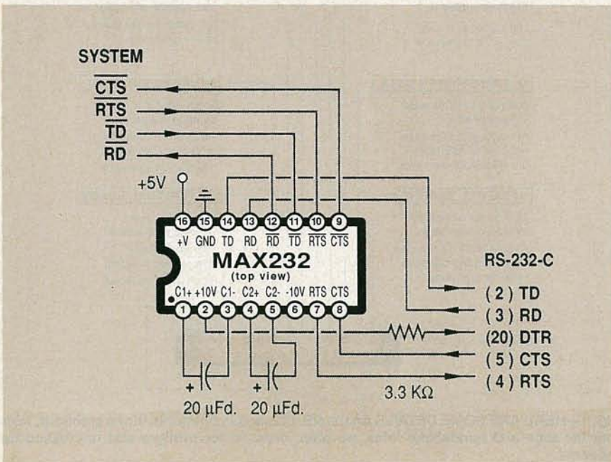
FIG. 4—THIS RS-232 DRIVER CIRCUIT needs only a single +5-volt supply. An internal charge-pump circuit generates the needed +10 and -10 volts for the actual interface levels.
