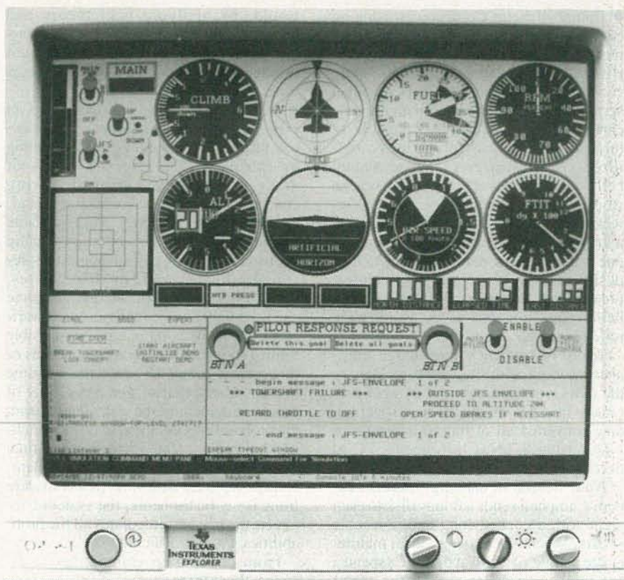
THE EMERGENCY PROCEDURES EXPERT SYSTEM , developed by TI, can either interact with the pilot and perform low-level flight operations or assume control of the aircraft and communicate directly with its automatic control systems until the pilot can regain control of the plane. Here, a simulated F-16 panel is shown on the screen of an Explorer computer. It is typical of the type of information that could be provided in an emergency situation.
