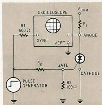
FIG. 8—AN OSCILLOSCOPE and a pulse generator are all that are needed for a t_{gt} test circuit.
