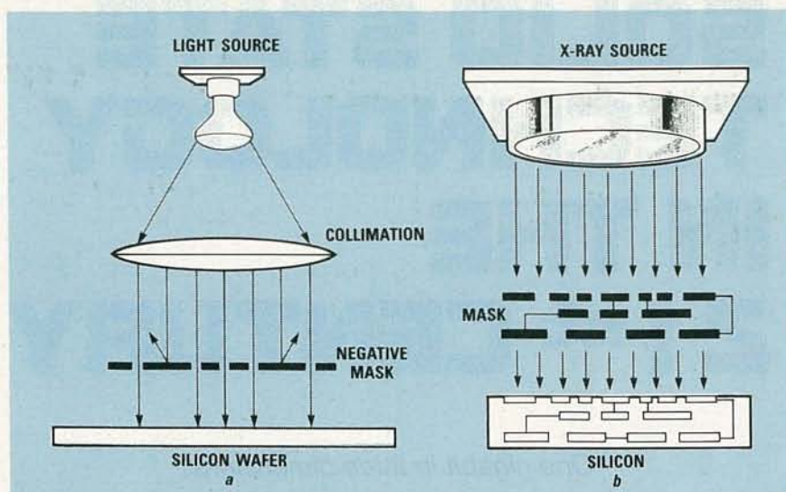
MULTILAYER, OR 3-D PROCESSING will sharply increase the active area per chip. As shown in a, in conventional optical processing a mask provides the surface pattern for a silicon chip. In 2001, 3-D processing, such as the X-ray system shown in b, will result in a multilayered chip having individual elements interconnected by metallic and/or optical paths.
