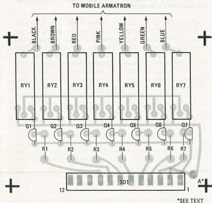
FIG. 2—ONCE ALL PARTS ARE MOUNTED, this double-sided PC board is inserted into a 12-position card-edge connector and the circuit is connected to the Armatron .
