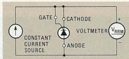
FIG. 4— V_{RRM} IS MEASURED using a constant-current source.
