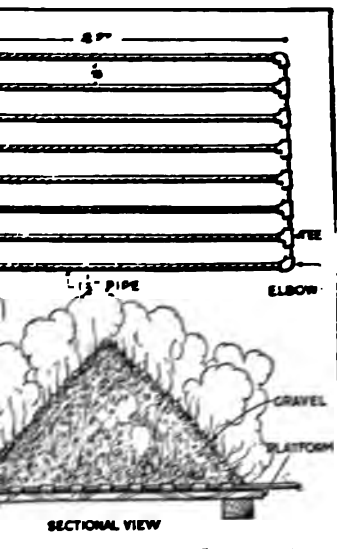
Method for Heating Gravel Used in Concrete: Made It Possible to Mix and Pour Material in Freezing Weather
