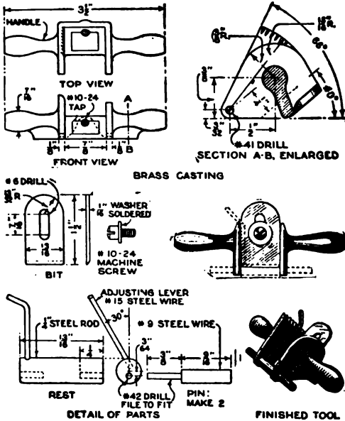
Full Working Drawings are Given for the Construction of a Small Spokeshave, Which a Skilled Patternmaker has Found to Be One of the Most Useful Tools in His Outfit
