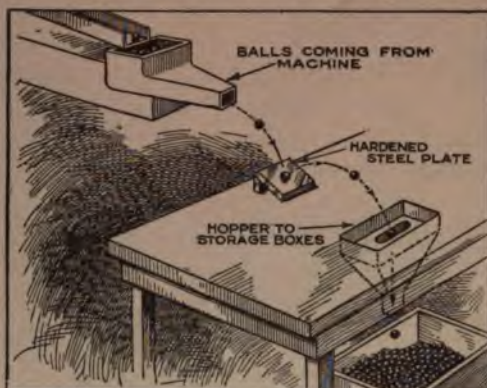
Correctly Hardened Balls Bounce into a Chute; Imperfect Balls Bounce Too Far or Fall Short of the Hopper
