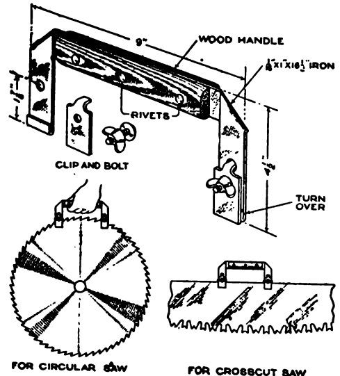
FOR CIRCULAR SAW FOR CROSSCUT SAW A Simply Made Handle Diminishes the Danger of Torn Clothing and Injured Hands, Incident to Carrying Crosscut or Circular Saws
