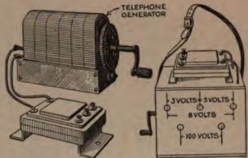
A Small Testing Set, Made Up of a Bell-Ringing Transformer and a Telephone Generator, Is Useful to the Mechanic
