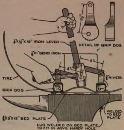
By Fitting the Tire Shrinker on the Anvil, a Tire can be Removed from the Forge Fire, Placed in the Machine, and Shrunken Before It Cools
