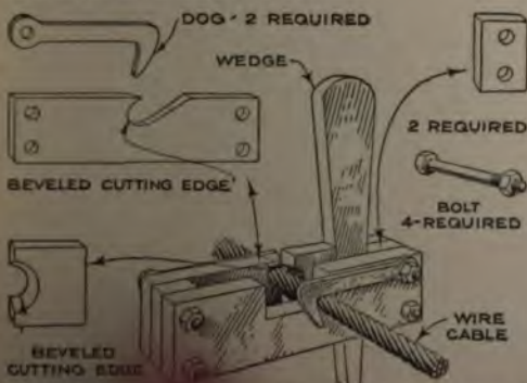
A Simple Tool for Cutting Wire Cable, the Value of Which is Appreciated by Seamen and Loggers
