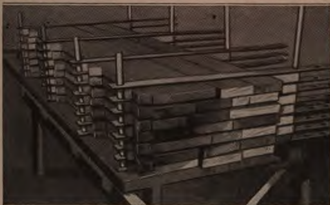
Where a Number of Large Panels are to be Glued Together, a Clamping Arrangement of This Type will be Found Handy
