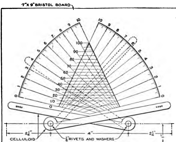
A Cardboard Device of Extreme Simplicity by Means of Which Problems of Multiplication and Division are Worked Out with Speed and Accuracy
