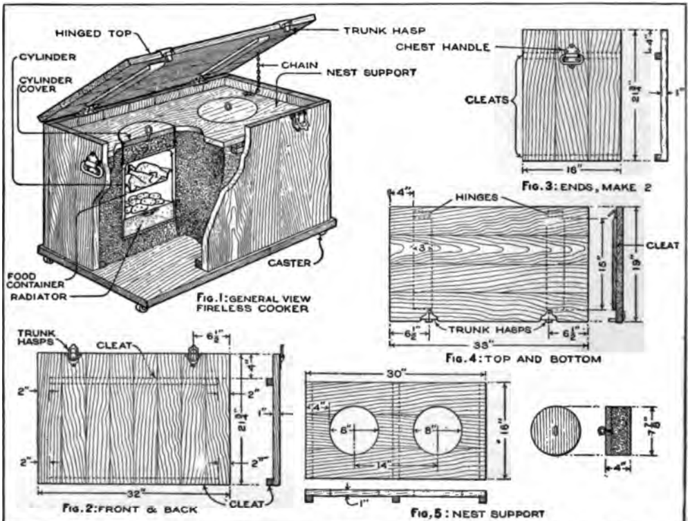
In Figs. 1 to 5 are Shown an Assembly View of the Fireless Cooker, and Details of the Various Parts of the Chest. This is Made Quite Solid, and Mounted on Casters for Easy Moving
