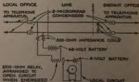
An Alarm Circuit Operates over Telephone Wires without Interfering with the High-Frequency, Sound-Producing Currents
