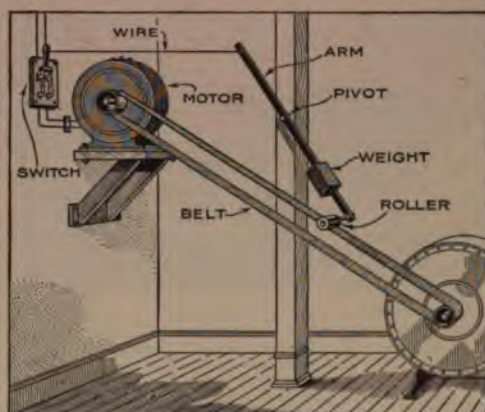
As Soon as the Belt Breaks or Slips off the Pulley the Weighted Arm Drops to a Vertical Position, Opening the Circuit and Stopping the Motor
