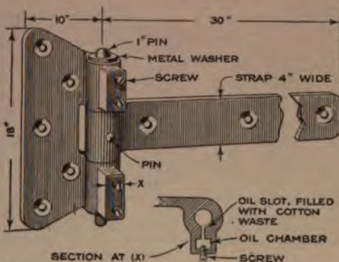
A Rusty Hinge on a Heavy and Expensive Gate Is Dangerous and Costly. This Specially Designed Hinge, for Heavy Gates, Is Proof against Sticking
