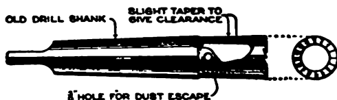
A Tool Made from the Shank of a Broken Twist Drill Provides a Ready Means of Cutting Out Small Wooden Plugs of a Given Diameter
