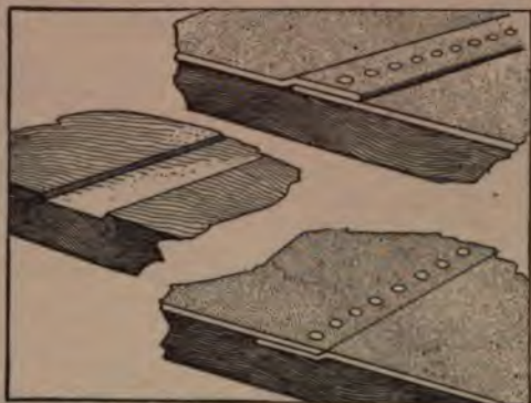
Porch Roofing, when Laid So as to Avoid Ridges Where the Strips Overlap, will Be Much More Durable
