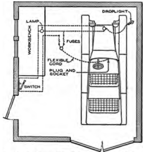
For the Car Owner Who Drives Chiefly in the Day-time, and Whose Storage Battery Therefore Has an Excess of Capacity, a Low-Voltage Garage-Lighting System Is Entirely Practicable
