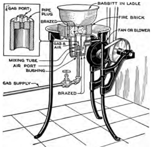
An Old Hand-Operated Forge Rebuilt to Burn Artificial Gas, for Melting Babbitt, Produces Exceptional Results and Holds the Heat within 10 Degrees
