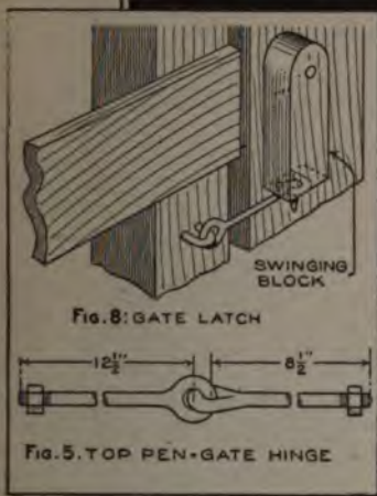
A Number of Construction Kinks, for the Farmer Who Contemplates Building Stock Pens and Corrals, are Illustrated in These Sketches of a Well-Designed Corral System
