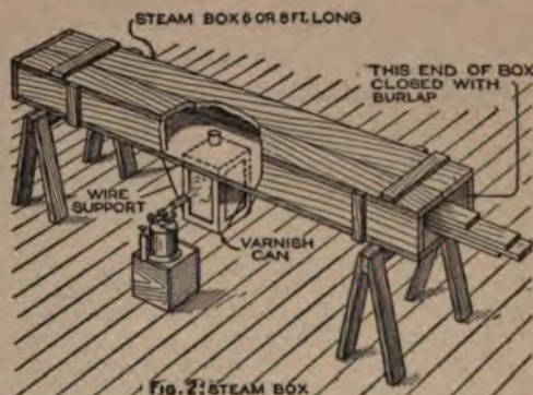
FIG. 2: STEAM BOX
