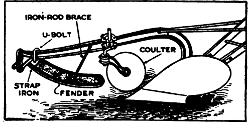
When Weeds Get a Good Start, Plowing Them Under Is Difficult. Part of an Old Auto Fender Turns the Weeds under the Coulters, Where They Are Cut and Turned under the Soil
