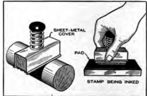
A Sheet-Metal Cover for a Rubber Stamp, Together with a Coil Spring on the Handle, Provides Means of Making Uniform Impressions on Cylindrical Surfaces
