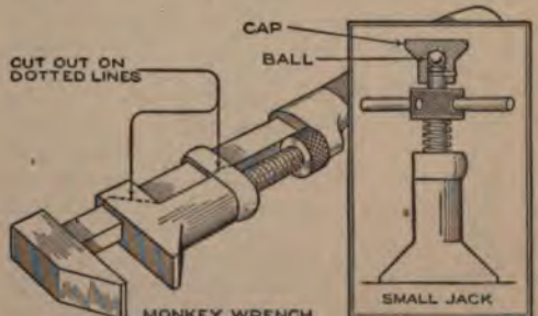
A Handy Small Jack, Which can be Used When an Ordinary Jack Is Too Large, is Made from an Old Monkey Wrench
