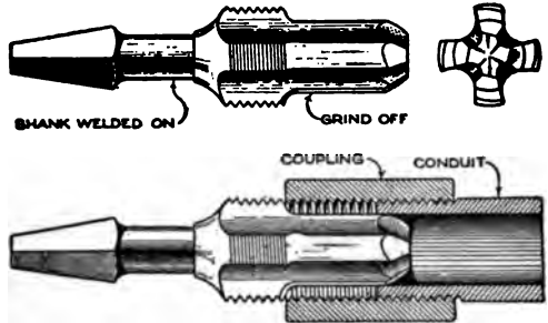
A Combination of Guided Reamer and Thread Chaser, All in One Tool, Adds to the Convenience of the Conduit Layer and Plumber
