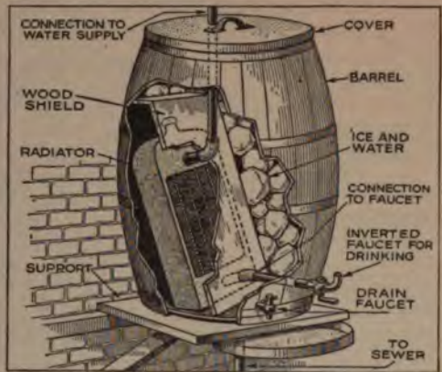
An Old Oil Barrel and a Discarded Radiator can be Combined to Furnish Cool Drinking Water
