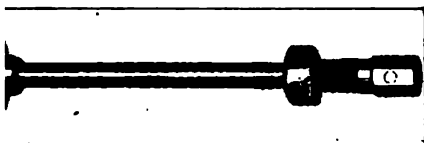
Lack of a Center Hole in the Valve Stem is Overcome by the Use of a False Center
