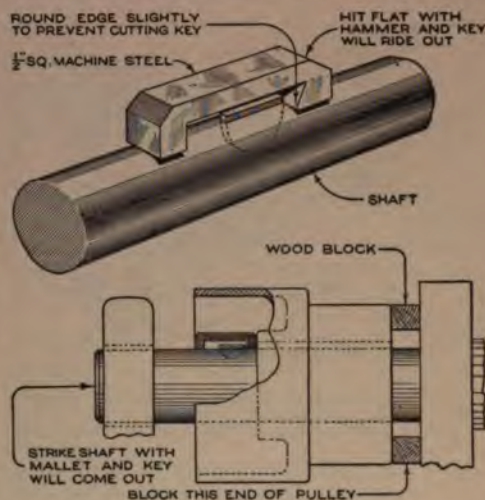
A Simple Tool That Makes the Task of Removing Woodruff Keys Easy
