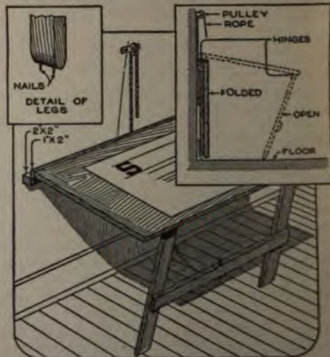
A Bench Made in This Way Takes Up Scarcely Any Room at All When Not Required, but Is Instantly Available When Lifted Up with the Hand
