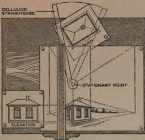
Draftsmen Who have Made Perspective Drawings by the Time-Honored but Tedious Method Commonly Used will Appreciate the Merit of a Swinging Perspective Rule
