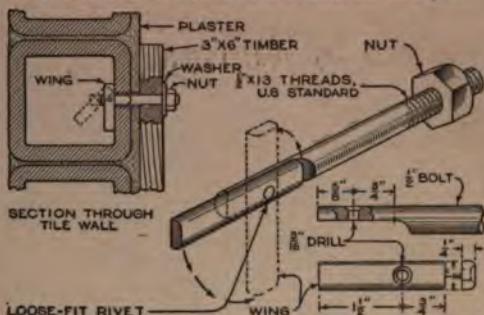
For Fastening Timbers to Hollow Tile the Wing Bolt Illustrated Is Better than Expansion or Anchor Bolts
