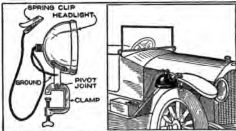
By Combining an Old Electric Headlight and a Clamp, as Shown Here, a Handy Trouble Lamp for Automobiles can be Made
