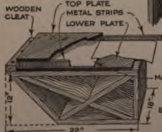
Fig. 3: ARRANGEMENT OF MATS
