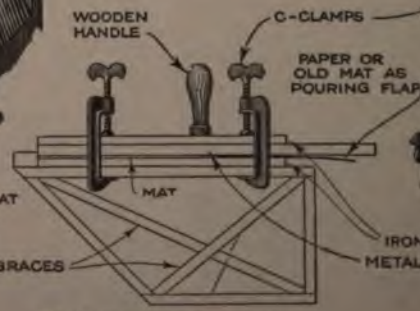
Fig. 4: CLAMPED FOR POURING
