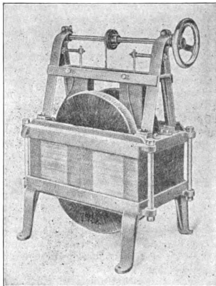
Transformer For Thawing Out Pipes
