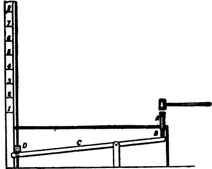
Fig. 3. Striking Box for Testing Force of Blow
