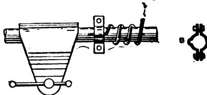
Fig. 2 and 3. Method of Bending Small Pipe.
