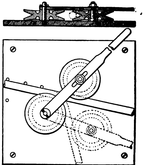
Bending Pipe Without Flattening It
