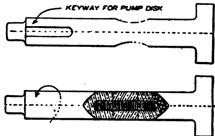
FIGS. 1 AND 2. REPAIR TO PUMP ROD.
