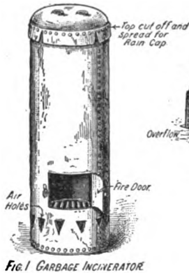
Fig. 1 GARBAGE INCINERATOR.
