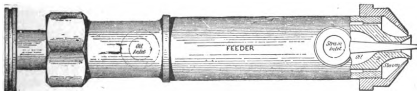
"HYDROLEUM" BURNER. NOW ATTRACTING MUCH ATTENTION IN ENGLAND.
