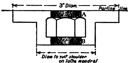
Faceplate for Self-Centering Chuck
