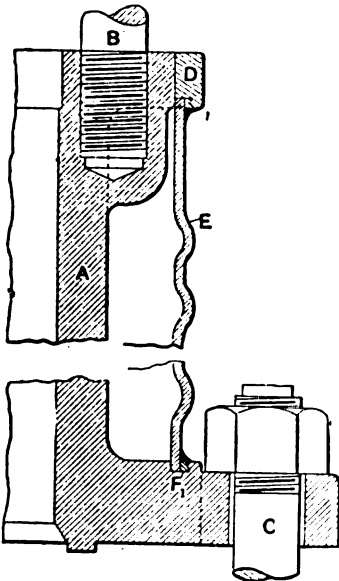
Fig. 1.—Showing How Water Jacket is Attached
