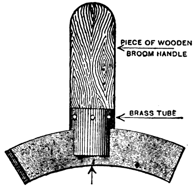
COMMUTATOR CLEANER.
