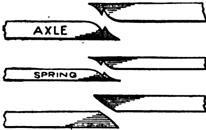
Welding Broken Buggy Springs
