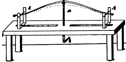
Device For Shaping Carriage Springs
