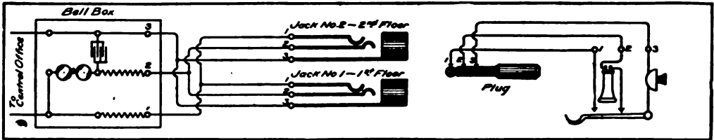
To Make One Telephone Serve Two Departments
