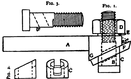
Details of a Tool-Holder.
