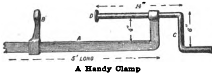
A Handy Clamp
