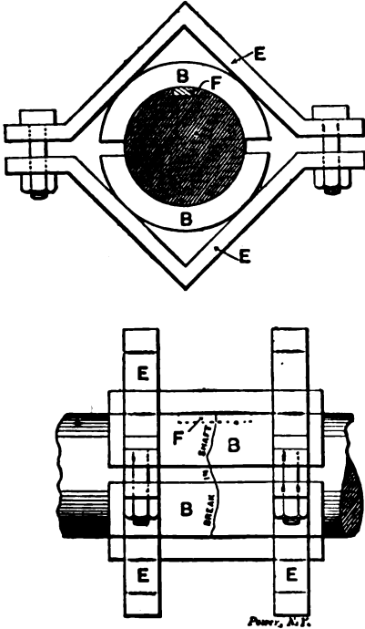
Showing Method of Repairing Broken Shaft
