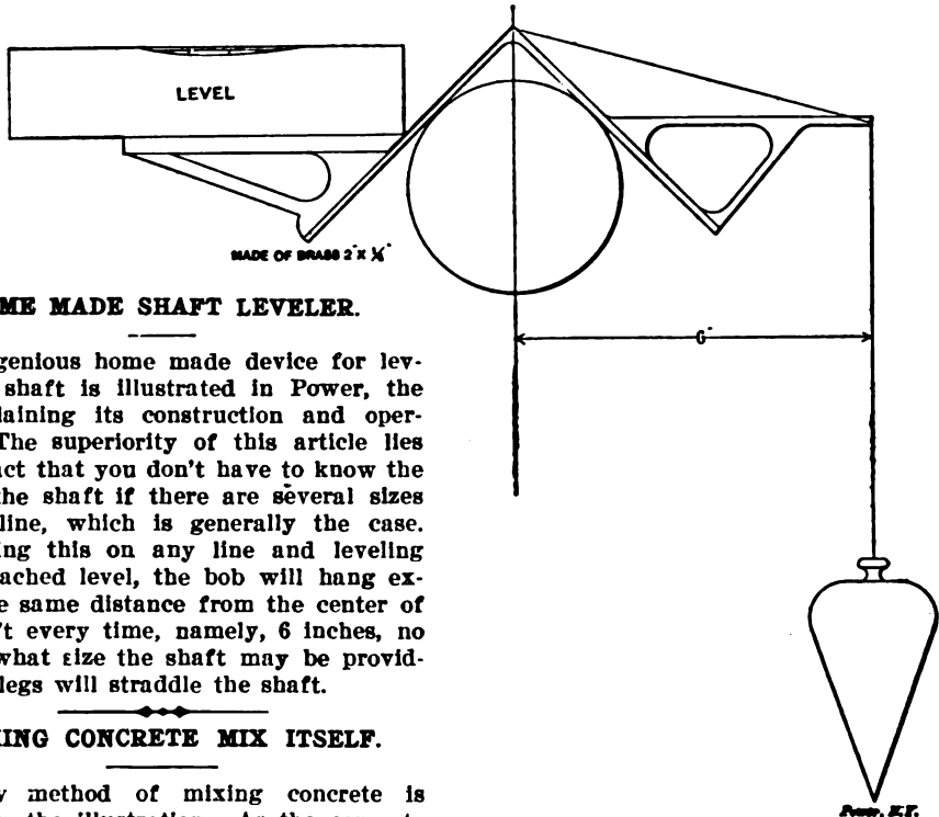
TOOL FOR LEVELING SHAFTING.
