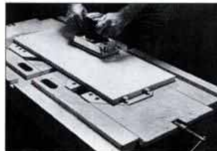
15 Use the clamping plates to secure flat stock. Open the sliding plates, place the pins in position. Then tighten clamps.
