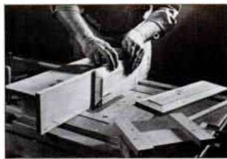
2 The extra-wide fence helps when passing the stock on edge. Tilt the saw blade for making these beveled panel edges.
