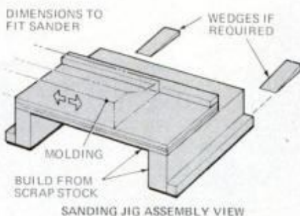
Support molding on jig and move laterally against the belt sander to smooth it.
