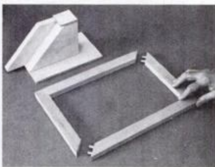
To assemble frame with mitered joints, you first join two diagonal corners.
