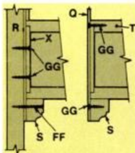
DETAIL 4, CABINET ATTACHMENT
