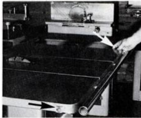
John Opfer eliminated original start/stop switch and installed a three-way switch on either side of table saw (arrows). Now he can turn saw on or off with either hand—no matter what size workpiece he is handling. At right, simple dust collector on grinder consists of a plastic fitting heated and forced on. Shop-vac hose is force-fitted.
