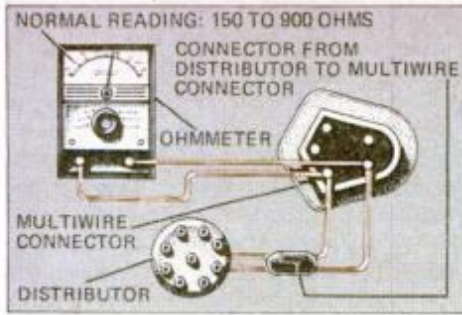
Test No. 4: Should read 150 to 900 ohms.
