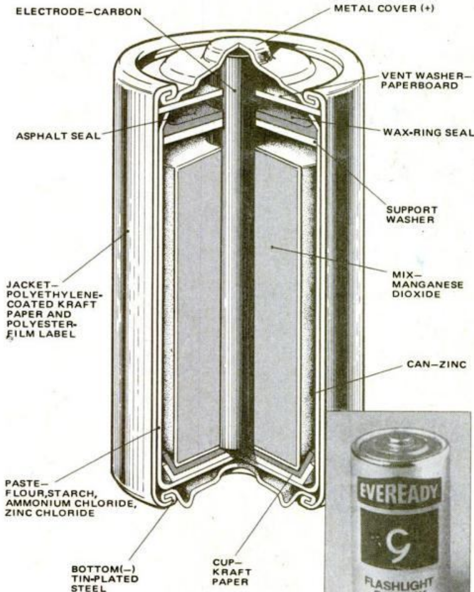
Carbon-zinc battery is the workhorse of the industry and is also the lowest priced.
