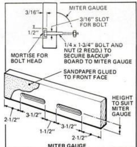
Author particularly liked miter gauge addition. It eliminates cutting through backup board. Drawing shows how it's made.
