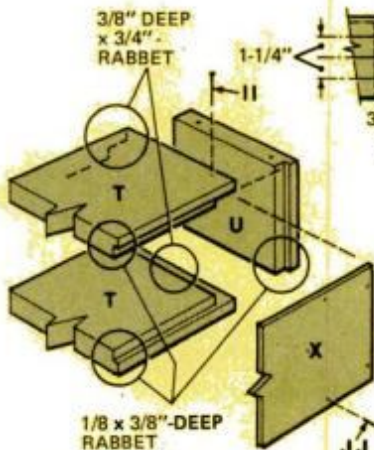
DETAIL 5, CABINET UNIT, REAR VIEW
