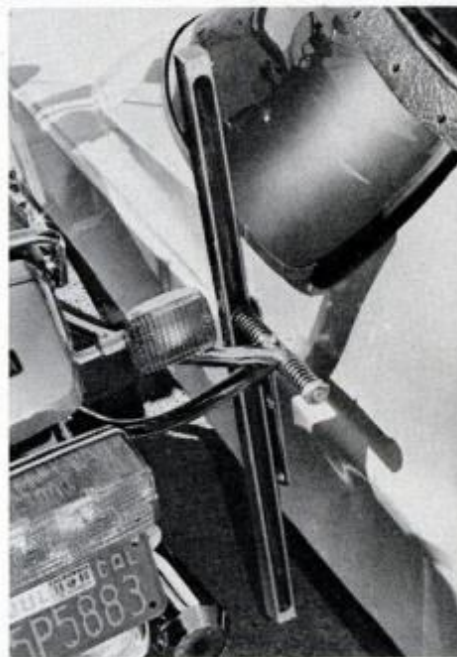
Off-road racing with a sidecar is not for the faint-hearted (above). It takes muscle and strong kidneys. Subframe for a Vespa sidecar is bolted, not welded, to the scooter (left). The sidecar is then bolted to the frame. Note the steel loop in front. It's there for crash protection. The heart of the flexi sidecar mechanism is the spring-loaded slider tube (right). It allows the sidecar to lean with the cycle.
