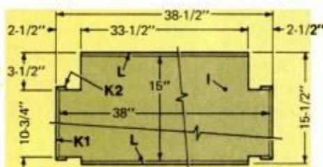
DETAIL 6, SHELF ASSEMBLY
