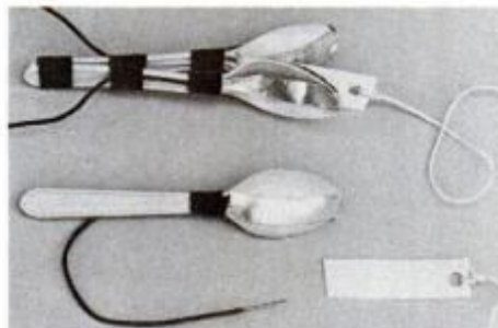
Trigger is made from string and plastic spoons. Pull spacer and foil strips touch.
