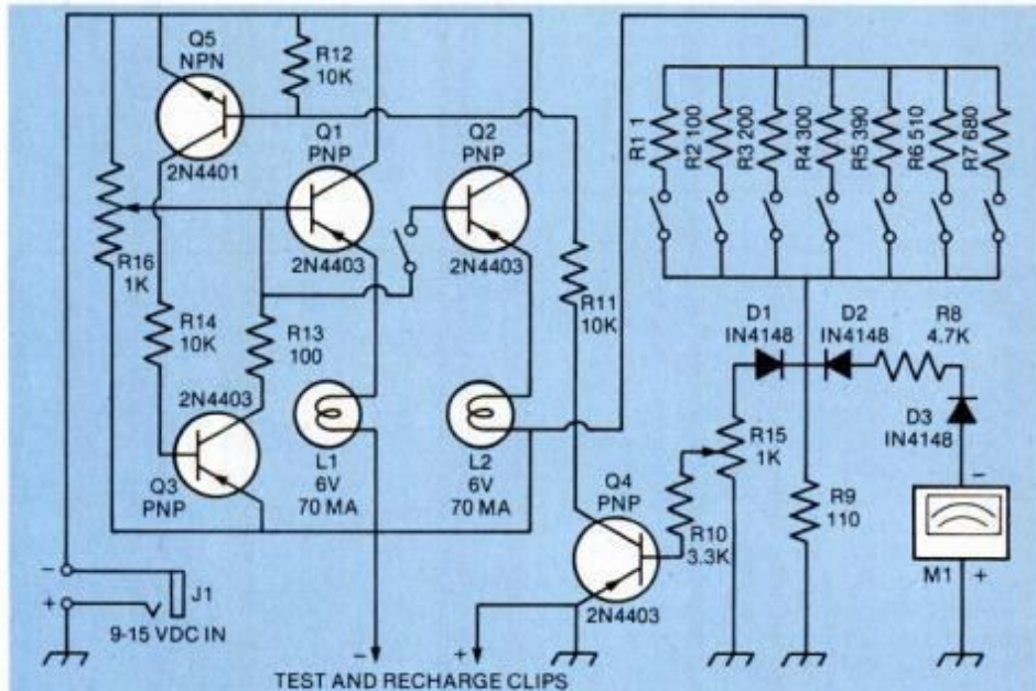
The schematic diagram (above) details how Battery Brain's components are interconnected. For complete list of parts required for the Battery Brain, see page 26.
