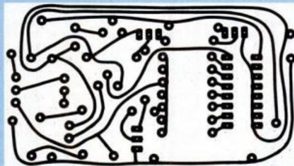
Component-side view (below) shows how all the parts of the Battery Brain are to be placed on the printed-circuit board. You can easily make the PC board by using the template which is shown above.
