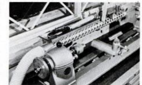
Collector for sander/grinder is a vacuum-hose fitting heated and pressed on tool.
