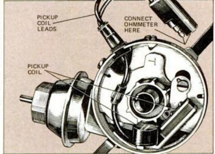
Test No. 5 (above): Should read 0 ohms. Test 6 (right): Should be 150 to 900 ohms.
