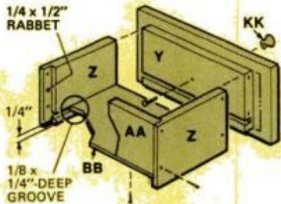
DETAIL 1, DRAWER ASSEMBLY
