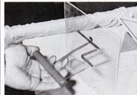
Z-shaped bar in dent-puller kit pulls out long creases on damaged body panels.
