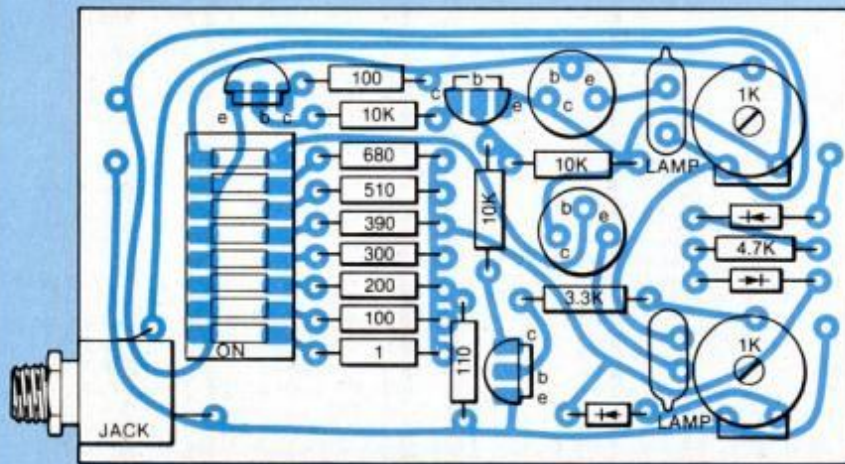
Component-side view (below) shows how all the parts of the Battery Brain are to be placed on the printed-circuit board. You can easily make the PC board by using the template which is shown above.
