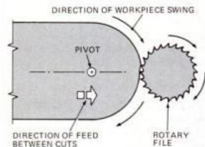
Swing strip so its end moves against the rotation of the file, as shown here.
