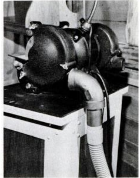
John Opfer eliminated original start/stop switch and installed a three-way switch on either side of table saw (arrows). Now he can turn saw on or off with either hand—no matter what size workpiece he is handling. At right, simple dust collector on grinder consists of a plastic fitting heated and forced on. Shop-vac hose is force-fitted.
