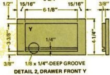
DETAIL 2, DRAWER FRONT Y
