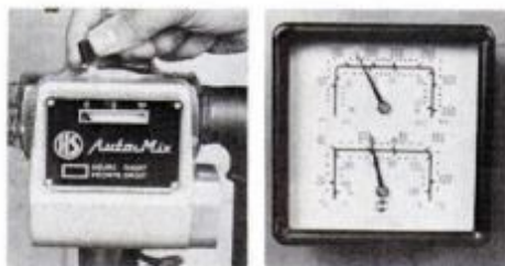
During off-season, mixing valve was closed (above, left) and boiler water temperature was kept at 140° F. to allow domestic-hot-water production (above, right).
