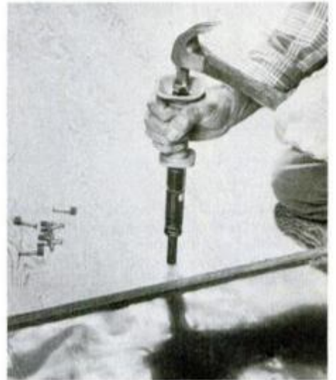
Plank and strip flooring usually require a nailing surface. Powder-actuated nailer makes the fastening of plywood easier.
