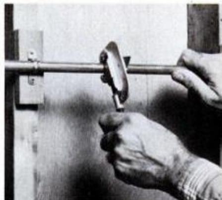
Cut a 6½-in.-long section out of the water supply line by using a tubing cutter.
