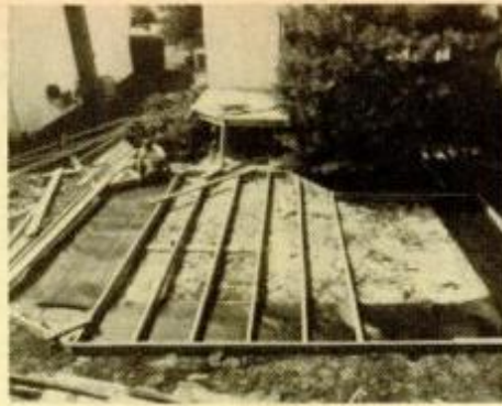
Soil beneath the deck is covered with 6-mil polyethylene (or 30-lb. felt) to keep grass from growing through deck. Joists on lower level are spaced 16 in. on center.
