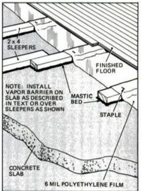
Alternate method, utilizing sleepers to raise flooring above slab, is preferred because it results in a more resilient floor.
