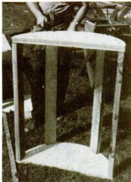
Half round counter is made with exterior plywood top and bottom and 2x4 studs. If desired, edges of 1x3 siding can be slightly beveled for neat-looking joints.
