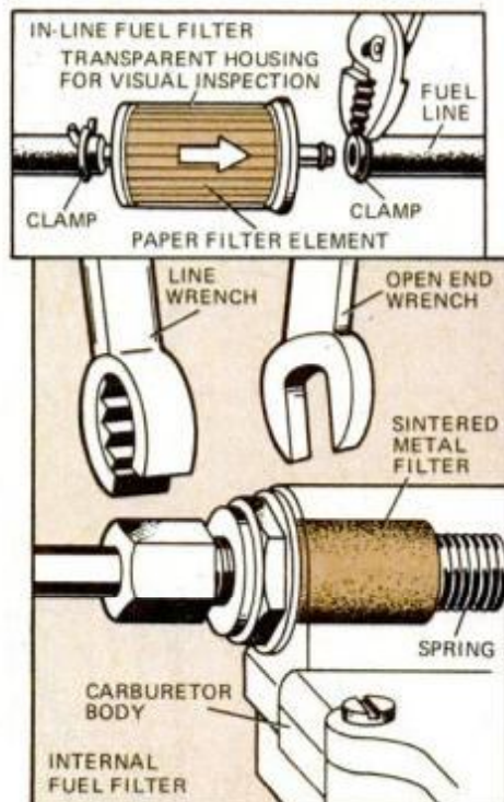
Dirty fuel filters will block the flow of fuel. You can inspect clear, in-line type visually; remove internal type to inspect.
