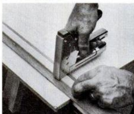
A strip of wood is used as a spacer to partially drive staples for temporary tacking of sawing guide (above, right).
