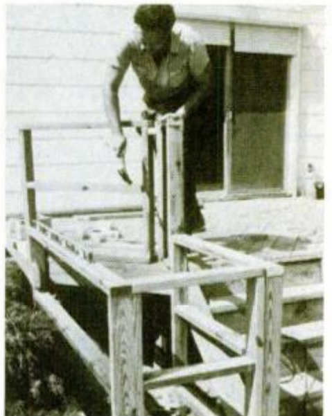
Planter and utility table is framed with minimal number of 2x4s. One-inch stock siding, which follows, adds great rigidity.
