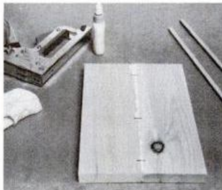
After gluing, gap is stapled closed to form a tight joint. Use a damp cloth to wipe glue squeezeout from stapler.
