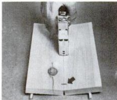
Staples serve as clamps for edge gluing. Boards are tilted so they are able to form a gap that will receive the glue.
