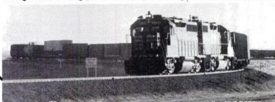
Hauling counterfeit cargo, train tests rails, ties during runs around 4.8-mile loop.
