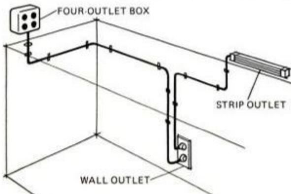
Wiring setup uses existing wall outlet behind bench to provide accessible power for tools through four-outlet, surface-mount box and continuous-outlet strip at other end of bench.
