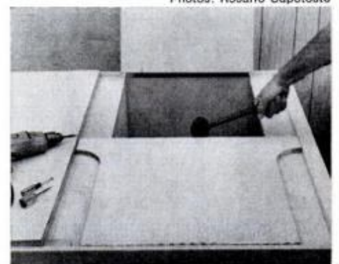
5. With hinge attached, lay door in place and tap with mallet. Screwheads will make indentations showing the correct location.
