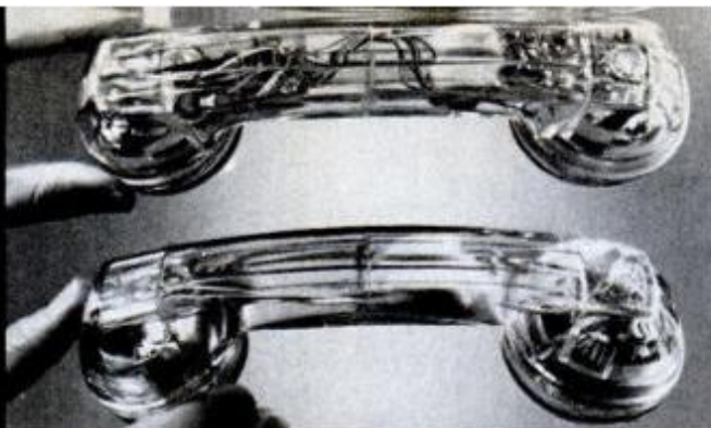
Amplified handset (top; note extra circuitry compared to standard model below it) will bring clearer reception to rural customers.
