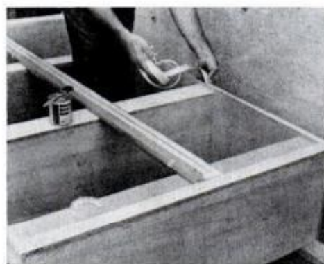
3. Surface long front edges carefully. If wood trim strip veers off, cut it short, butt-join a new piece and continue on.
