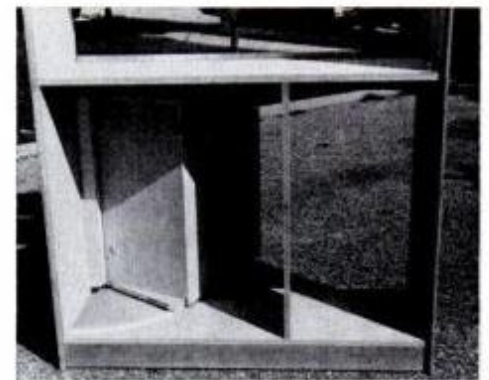
6. Rear view shows how bottom extension helps support weight of drawer box. Glide rides smoothly on track cut from laminate.
