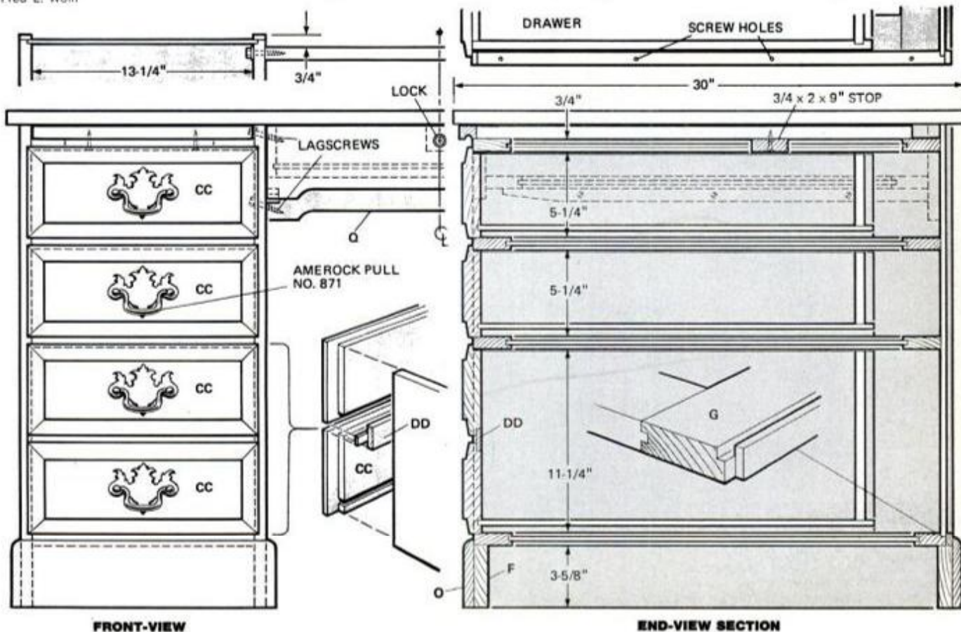
Grooved end members are added to sidepieces after latter are on dust panel.
