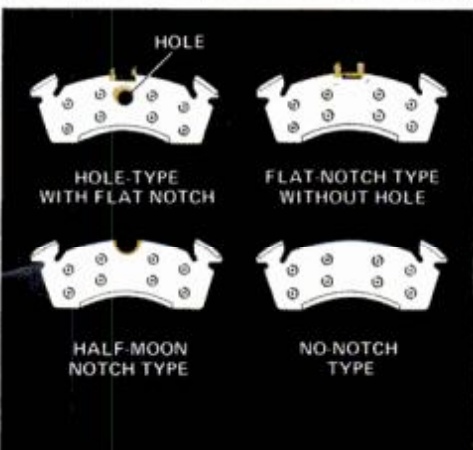
Four disc-brake-pad types that vary depending on configuration of the calipers.
