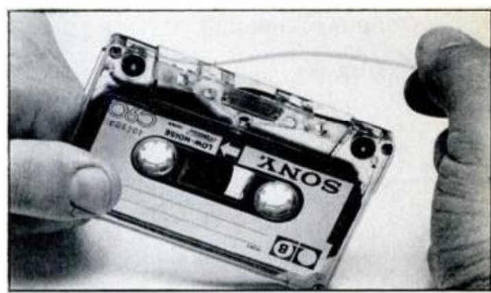
Too's for cassette repair include: Audio Accessories kit (far left) with spare shell, splicer, and splicing tabs; 3M kit (top left) shown in more detail below; Editall splicing block (left) with splicing tabs, special tape-marking crayon, and razor blade. 3M kit (photos below) includes strips that fish broken tape ends out of cassette shell, splicing block to repair broken ends, winder to take up slack in tape after completion of repairs.
