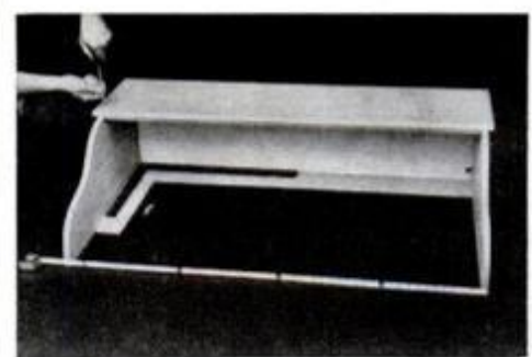
After parts are test-fitted, screws are driven in counterbored holes and capped.
