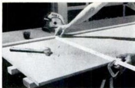
Block clamped to rule assures accurate straightedge placement to saw plywood.
