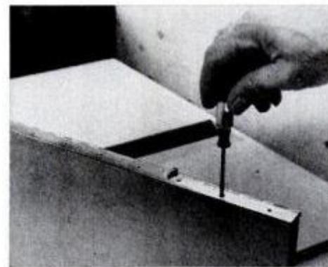
4. For perfect hinge alignment, attach a doubled-up hinge to the door and turn in roundhead screws near each end to hold it.
