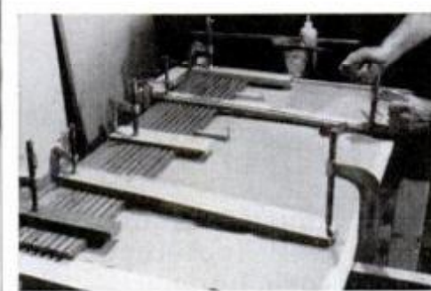
Slats are glued to cloth back 8 to 10 at a time, apply glue to cloth only.
