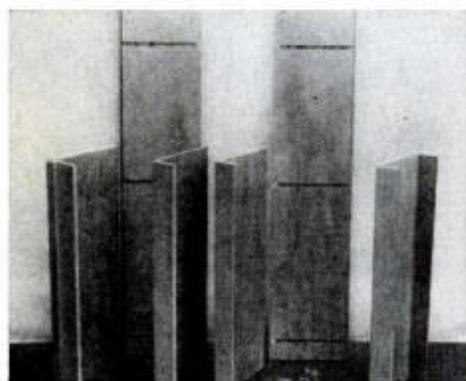
1. Major components ready for assembly—blind dados are made easily by gluing softwood inserts into the voids.
