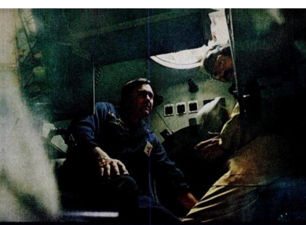
For maximum strength, Beaver's crew and passenger compartments are spheres. Interior of crew sphere is shown above. VOL L1 (below) permits crew to inspect pipelines through acrylic window. Divers can leave sub through lock-out hatch to make needed repairs. Divers (right, bottom) work on pipelines. The sub shown at the right, Pisces III , is launched and retrieved from "A" frame.
