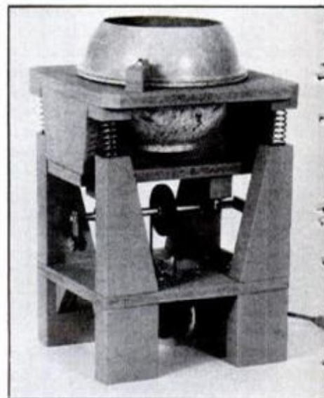
Complete polisher with bowl in place (the second hold-down clamp is hidden)
