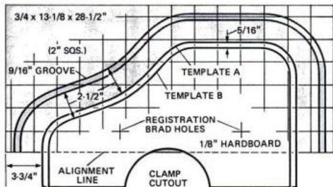
Two templates guide router to form 9/16-in. groove with 1/4-in. straight bit. Remaining 1/16 in. between 1/4-in. grooves is removed by guiding router freehand.
