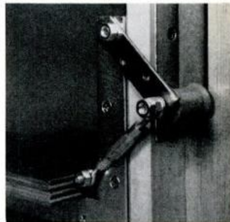
Thread spools serve as rollers for table movement; turnbuckles permit adjustment.
