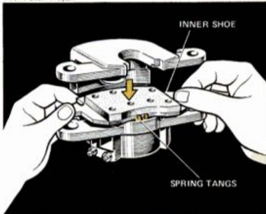
Inner pad is installed with the help of the spring-wire, antirattle spring.
