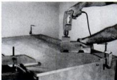
Counterbored holes for wood plugs are drilled at right depth with homemade jig.
