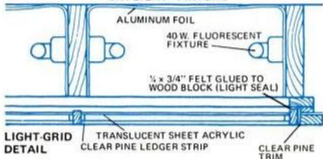
"SKYLIGHT" FIXTURE
