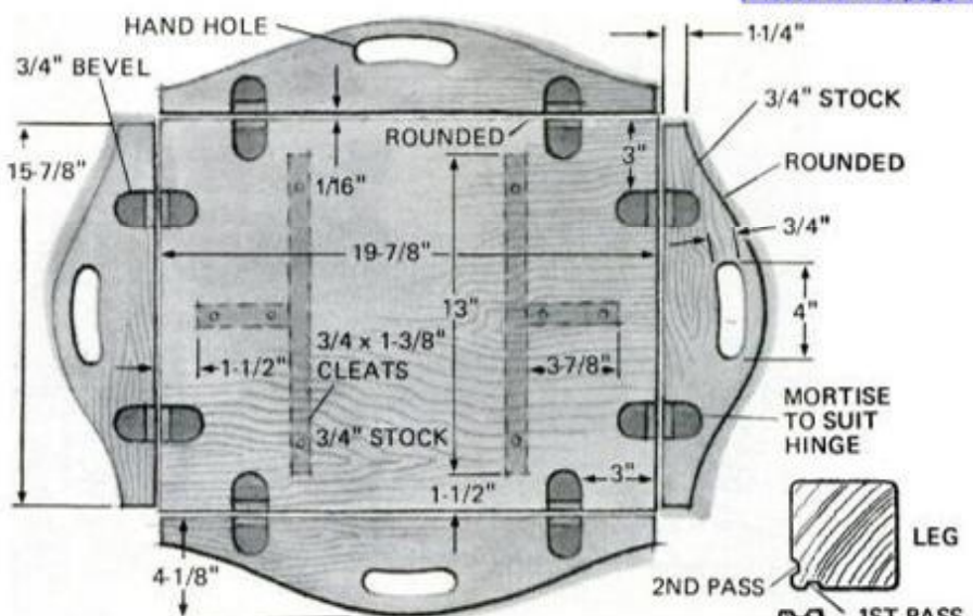
TRAY TOP
