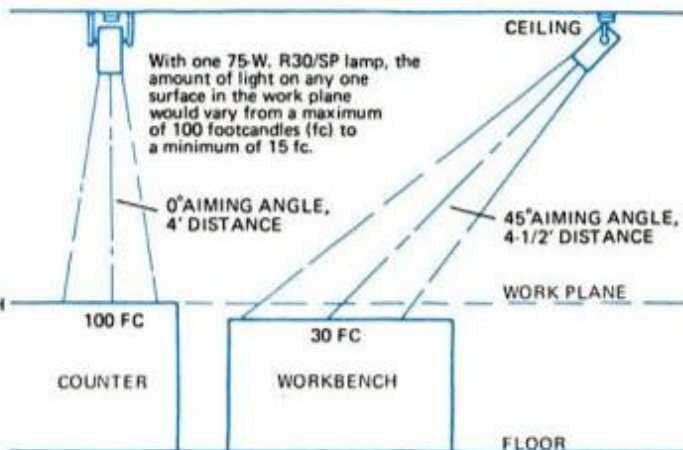
POWER-TRAC LIGHTING
