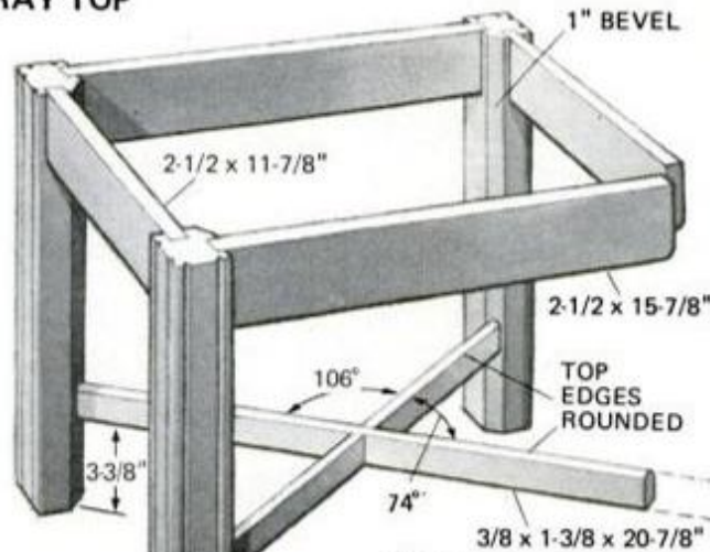
BASE
