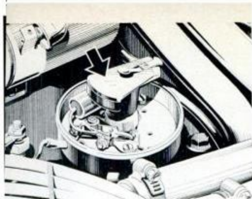
Distributor rotor conducts high current from the coil to sparkplug wires. Inspect it carefully, and always carry a spare.
