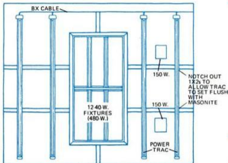
"SKYLIGHT" FIXTURE
