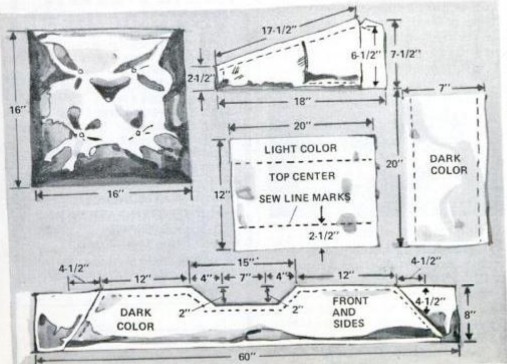
Backrest , with 2 1/2 x 7 1/2 x 17 1/2 x 18-inch cover, has pocket.
