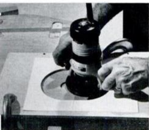
Use plywood template to guide router base for cutting semicircular hinge mortises.
