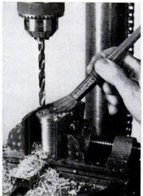
Pad vise jaws with leather when drilling holes. Start with small bit, switch to larger.
