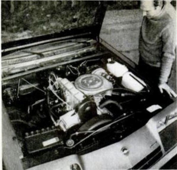
Four-cylinder engine has plenty of workroom around it. The V8, however, has a problem: One of the eight plugs is almost inaccessible without jacking engine.
