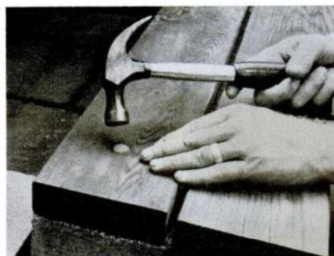
4 Flathead screw is turned home in counterbored hole; \frac{3}{4} -in.-dia. dowel plug hides screwhead. Use waterproof glue to assure dowel staying put in hole.
