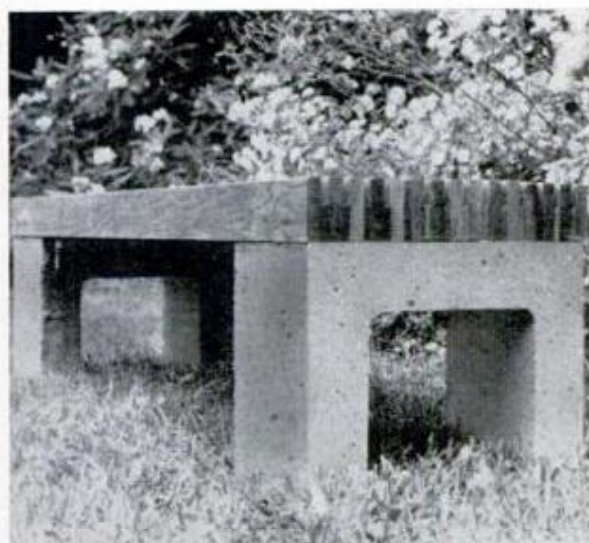
Slatted coffee table is a slight variation of the furniture shown on facing page. The \frac{3}{4} -in. redwood stock is separated by spacers, and the seat assembly is fastened to the blocks as detailed in the drawing at the right.
