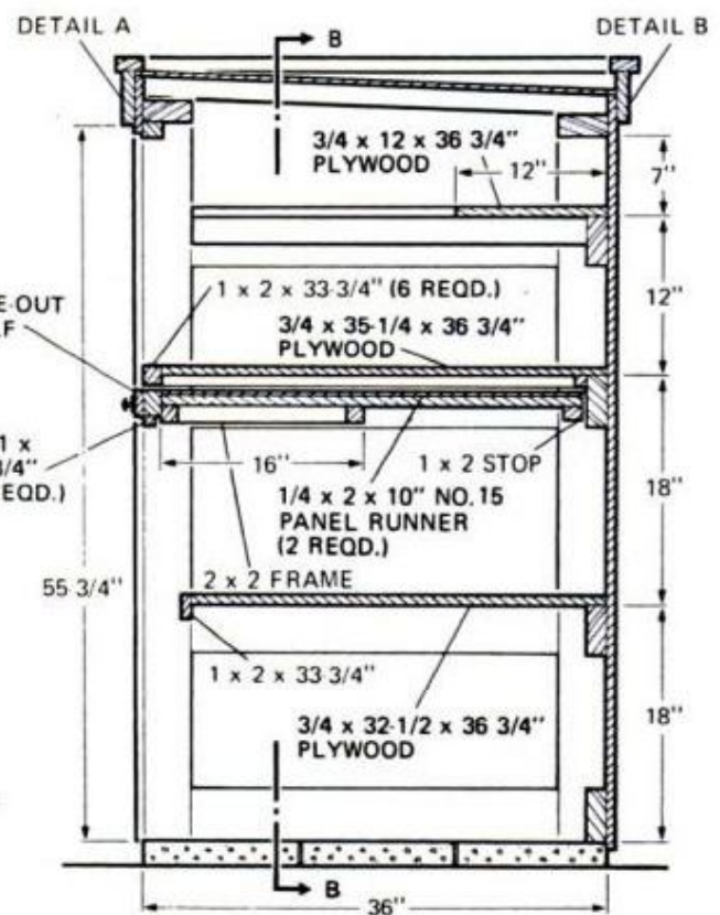
SIDE VIEW, SECTION A-A
