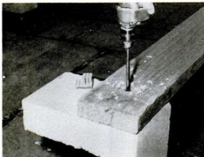
1 Bench seat boards are cut to length, positioned on blocks and \frac{3}{4} -in. holes are drilled through. Tip of bit marks spot where you will drill block.
