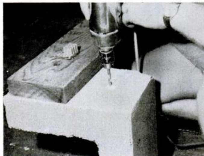
2 Holes in masonry should be bored in stages to make bits last longer. Start with a small bit and work your way up to the desired diameter.
