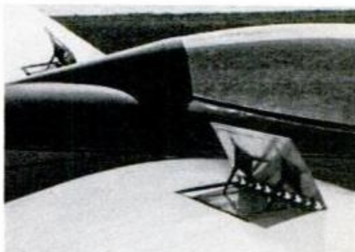
Extended, the dive brake allows plane to lose altitude without causing it to pick up speed. Dive brakes make landing easier, but plane can land without them.
