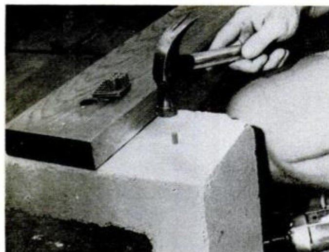
3 Masonry anchors are then tapped into the predrilled holes. Author used one at each end: Two per board at each end would be even better.
