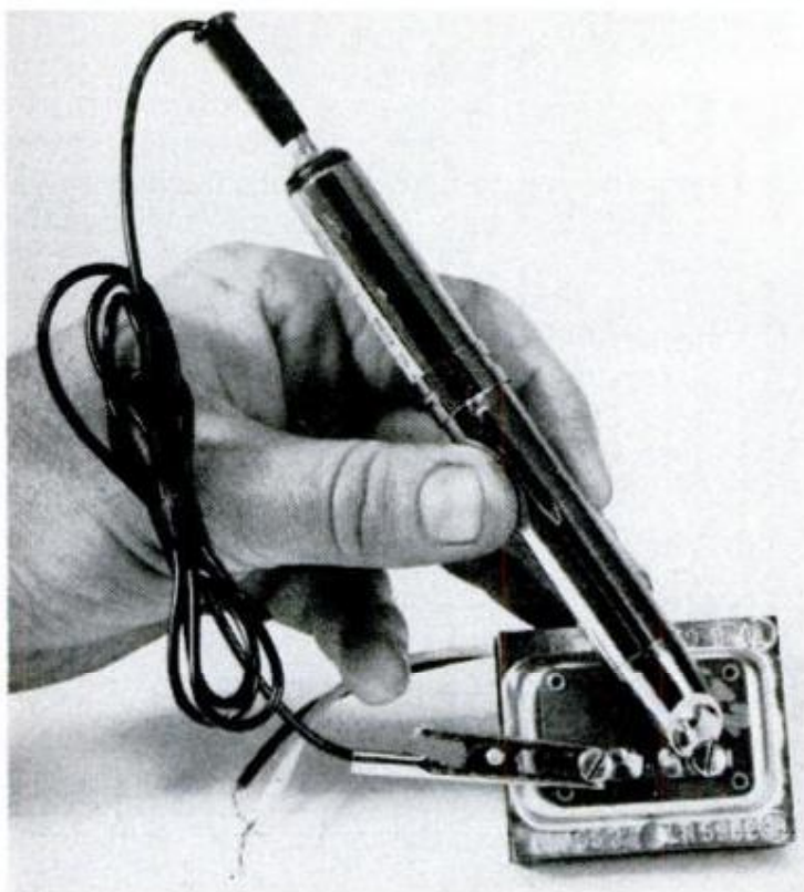
Transformer is checked for continuity by placing alligator clip on one screw, tester probe on the second.
