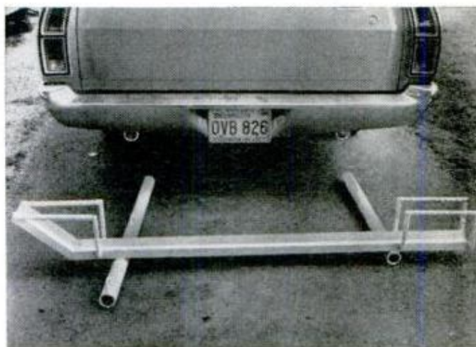
Carrier holds 315-lb. trail bike—too heavy for bumper-mounted types—slides into mounts welded or bolted to underframe of car, leaves bumper unmarred.
