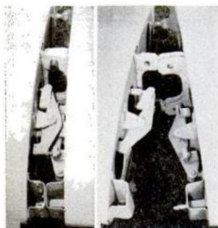
Wing-latch arrangement is shown at left. Wing swings on pivot fitting at rear. Snap-in strips cover slot.
