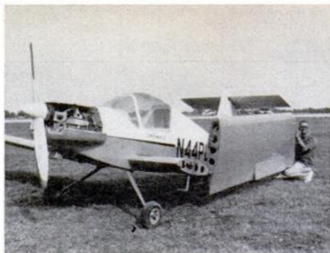
Rear-folding wings make ship compact for storing and towing. Note simplified landing gear—just two spring-steel struts. Wheel fairings can be added or omitted.
