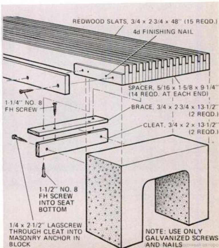
Slatted coffee table is a slight variation of the furniture shown on facing page. The \frac{3}{4} -in. redwood stock is separated by spacers, and the seat assembly is fastened to the blocks as detailed in the drawing at the right.
