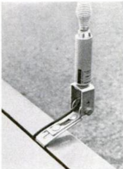
TRUNK-EDGE CLIP mounts mobile antenna without drilling the body
