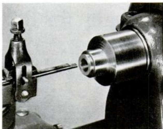
BORING BAR is used to finish-bore the axial hole. The hole in the side is for a chuck-removing wrench
