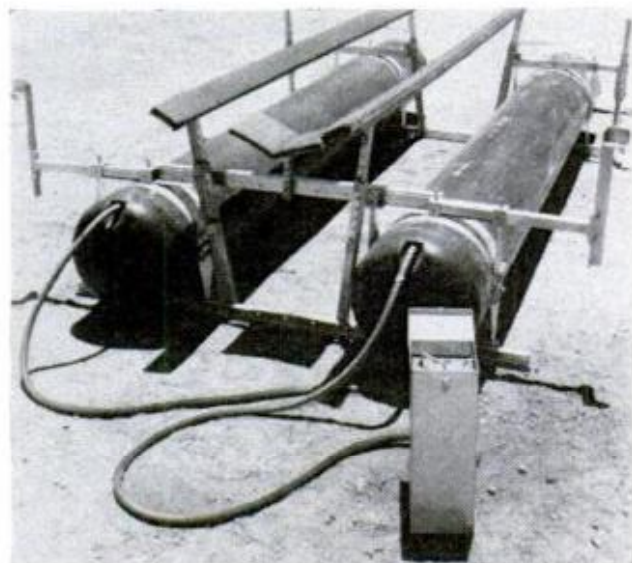
HOIST GUIDES on each side slide up, down in dock brackets. Installation takes less than three hours
