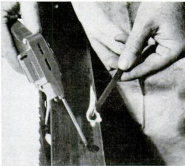
FOR BEST BOND , a clean soldering iron is used to heat base around gouge edges. Molten repair-stick "spaghetti" is dripped in. Extinguish burning drops
