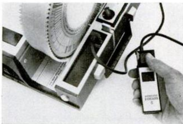
REMOTE SLIDE ADVANCE and reverse control on this Sawyer doubles as projector's own control panel. Autofocus projectors usually lack remote focus
