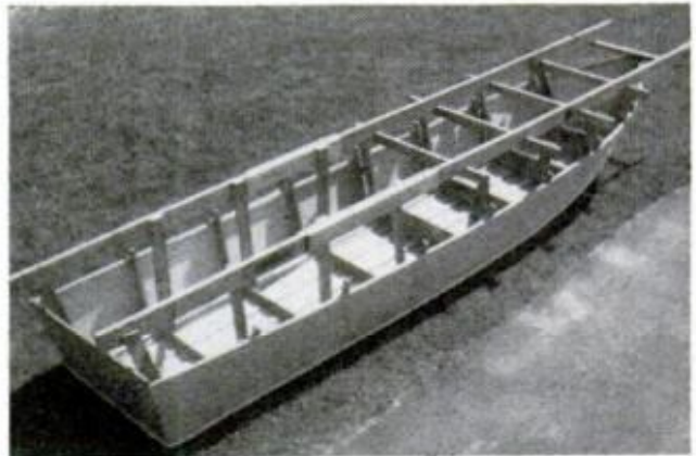
PREPARATIONS for framing out may require space of a rented warehouse. Figure you'll start job upside down, then right the planked hull for final decking
