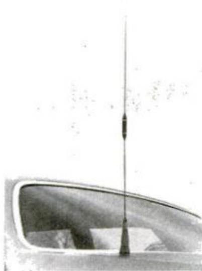
LOADING COIL in middle of whip electrically "extends" its length
