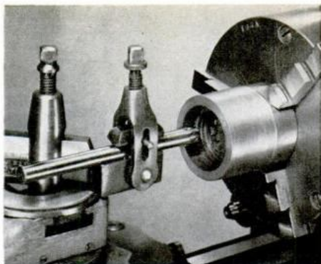
AFTER RECESS IS BORED 1½-in. x 8 threads are cut into the chuck body to fit the 9-in. lathe spindle
