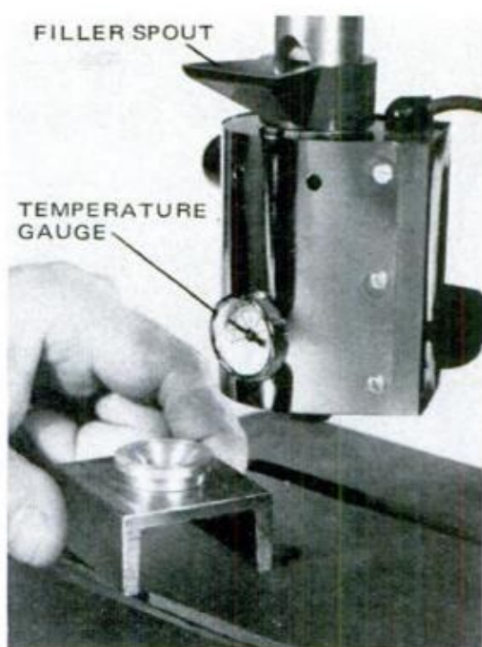
INJECTOR IS CLEANED of leftovers by placing purging block and ring under the nozzle
