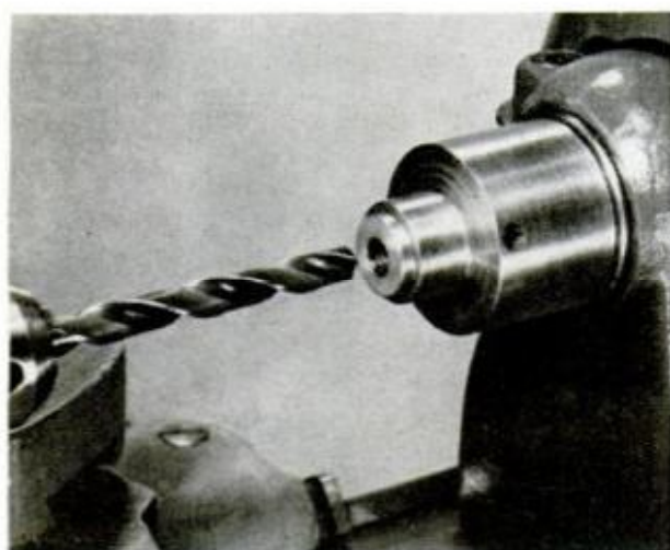
REGULAR TWIST DRILL is used to bore a slightly undersized axial hole in body of the screw-on chuck
