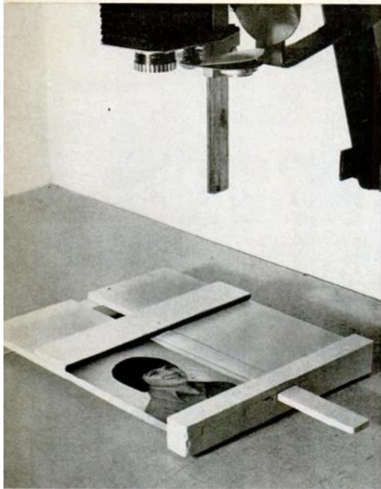
OVERHANGING BEVELS on the two stops that contact the enlarging paper hold the paper flat without casting a border shadow onto it. The "T-square" stop slides to adjust for any size of enlarging paper
