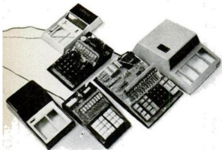
KITS: Heath IC-2008 (rear) is $110, has fixed and floating decimals, takes six hours to build. Aries (lower left) costs $99, takes six hours. MITS 1440 ($200 kit, $250 wired) takes 15 hours because of memory and other functions (see page 88)
