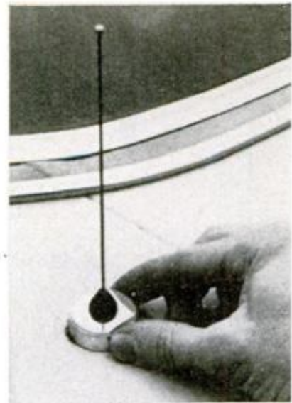
MINIATURE WHIP is quarter-wave aerial for 450-470 MHz 2-way FM
