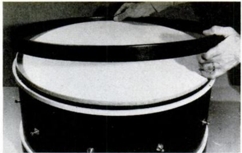
8 TOP BAND is positioned on the drum so that it will support the top hoop \frac{1}{2} in. above the laminate-covered tabletop
