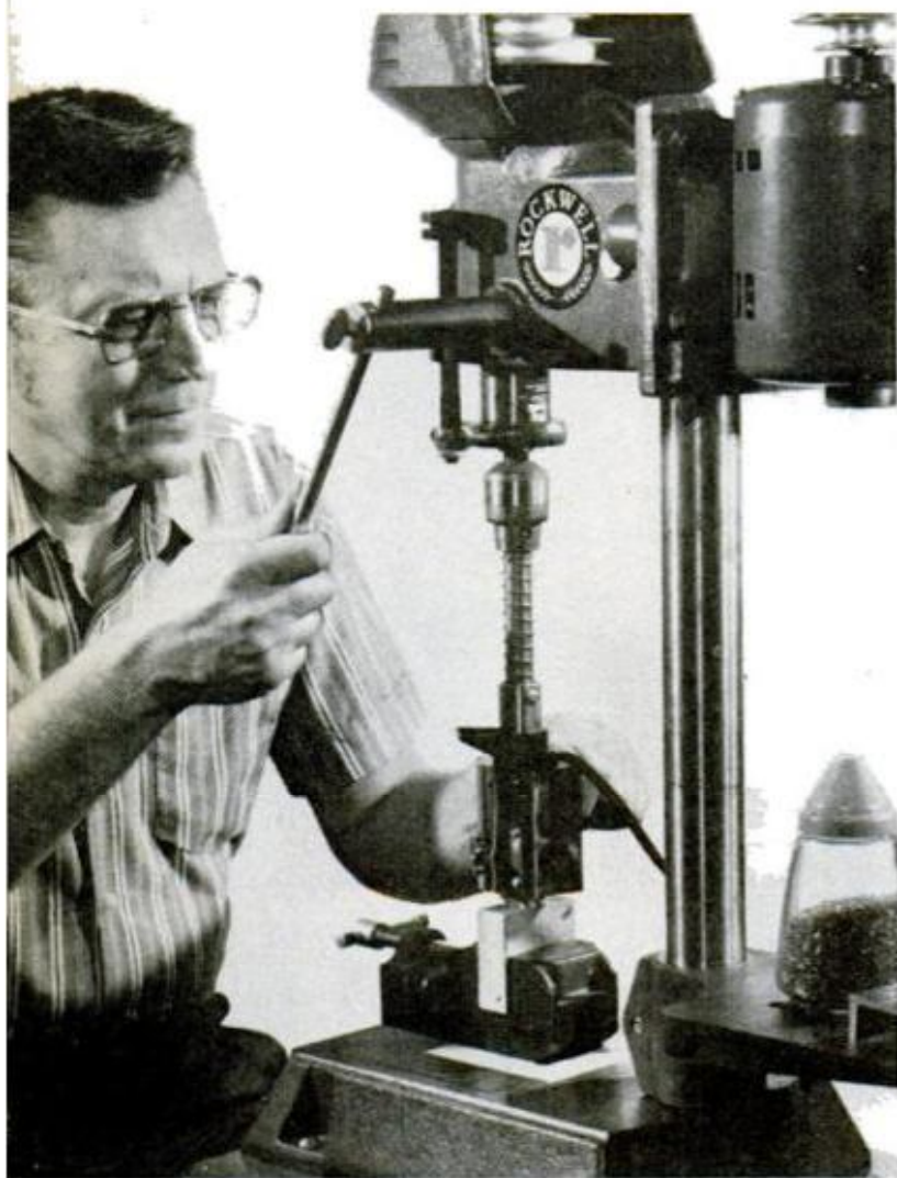
STRIPS OF TAPE on drill-press base provide quick way of positioning mold each time when making production run. Drill press must be sturdy to exert needed pressure
