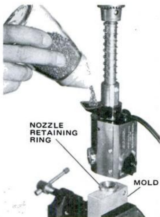
INJECTOR IS FILLED with plastic pellets through top filler spout, holds \frac{1}{2} ounce
