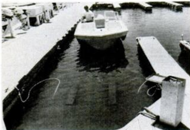
INSTALLED in slip, hoist unit is completely submerged and only hoses to blower pump can be seen
