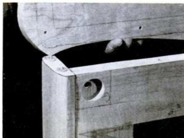
SIDEPieces are attached to the frame with glue and dowels. Use dowel-centers to locate hole positions
