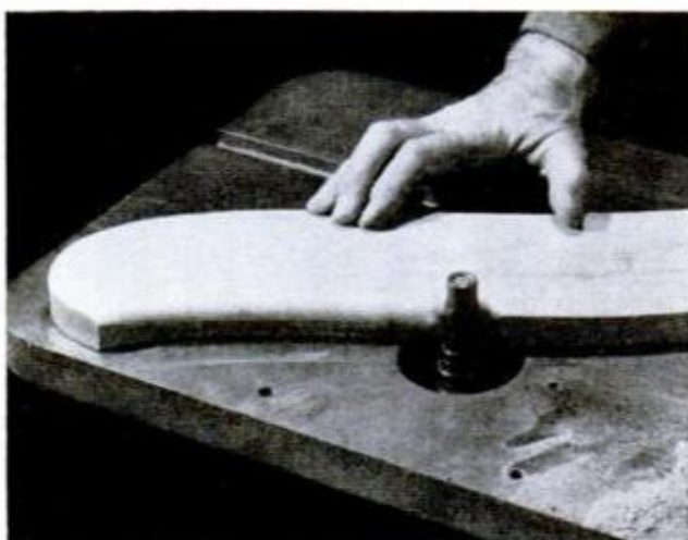
HALF-ROUND CUTTER AND SHAPER are used to shape radius on sides. Bottom inside part is not rounded
