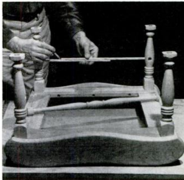
DETERMINE SPINDLE LENGTH by inserting legs and using two sticks (in spindle holes) as depth gauge
