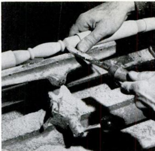
EASY WAY TO BEAT WHIPPING: Grasp work lightly with one hand while your thumb guides turning tool
