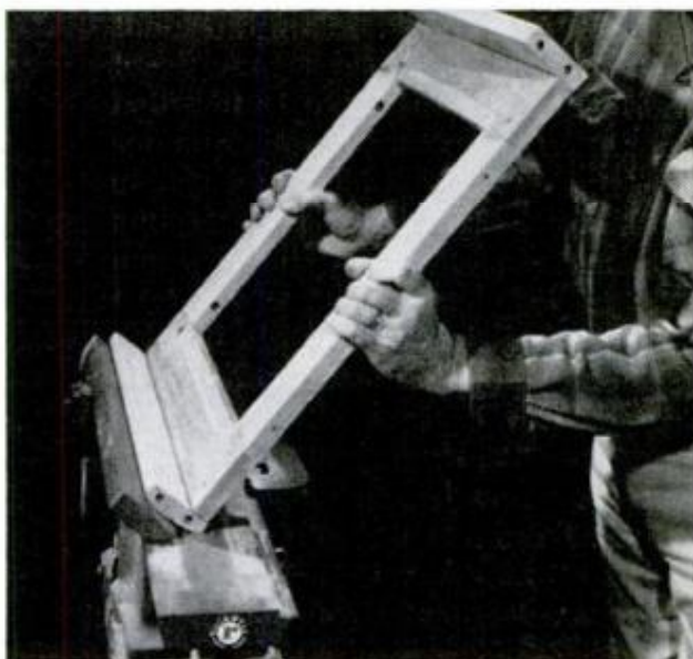
AFTER FASTENING ENDPieces to the frame, you can shape the curved profile freehand on the jointer
