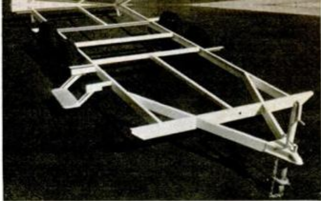
COMPLETED TRAILER FRAME for 20-ft. Laguna-20 with tandem axles. Note the coupler with jack stand
