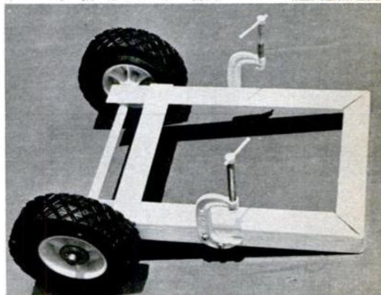
WITH LIGHTWEIGHT TOTOER you can single-handedly haul your small boat from storage to the big boat
