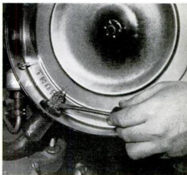
MESH FILTER used in some PCV systems is found where the hose attaches to the air-cleaner housing
