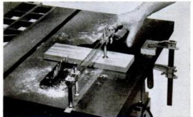
BLOCK OF WOOD clamped to saw table will serve as a stop for mass-cutting short lengths of stock
