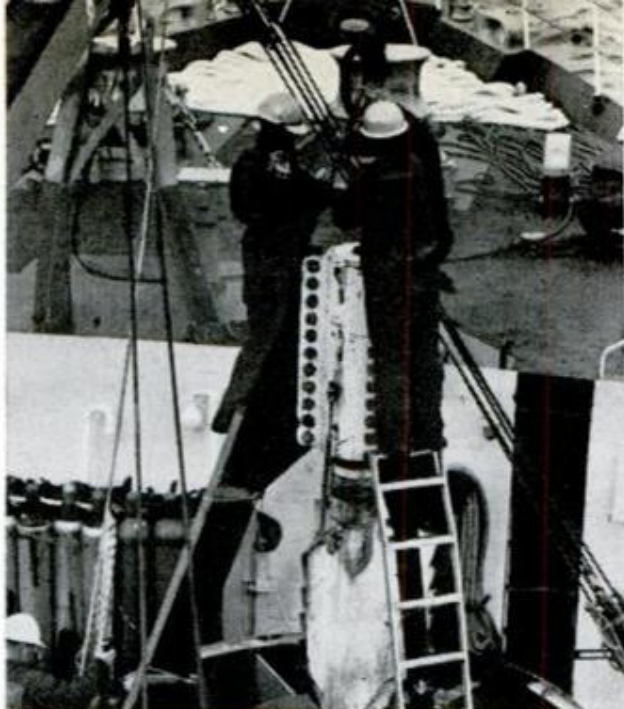
EXPLOSIVE ANCHOR is readied aboard Coast Guard cutter. It broke when fired into seamount surface
