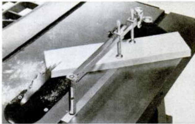
HOLD-DOWN ATTACHMENT fitted to miter gauge will keep workpiece from creeping during miter cuts
