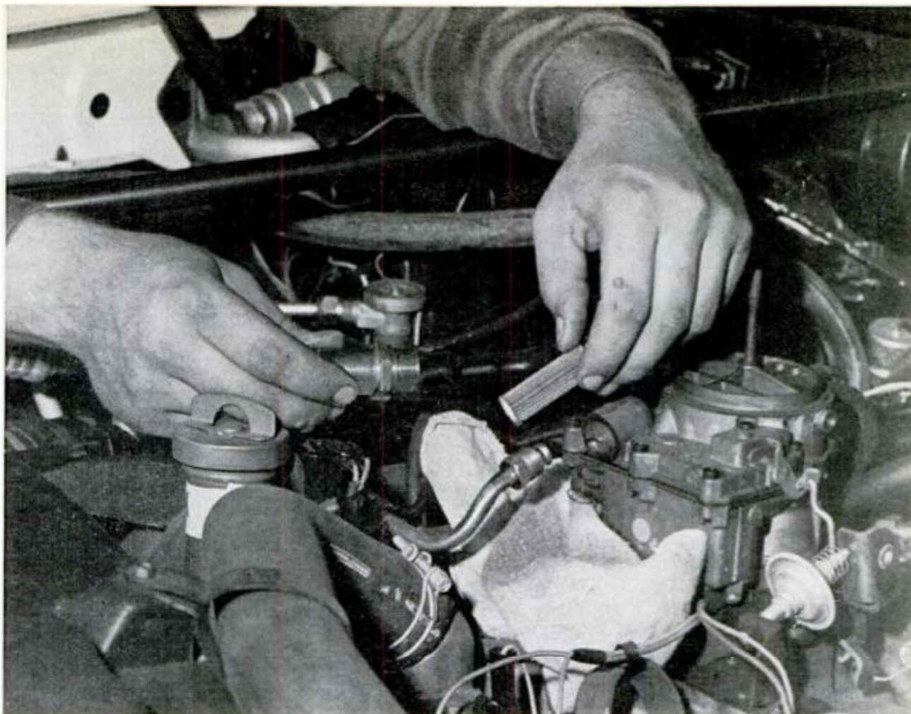
FUEL FILTER OF INTERNAL TYPE is found in carburetor. Disconnect the fuel line and filter retaining nut
