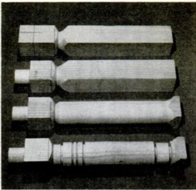
LEG-TURNING PROGRESSION , top to bottom: Chamfer cut, tenon, rough cylinder, then parting cuts
