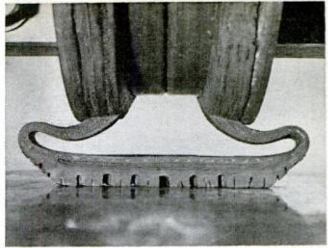
CUTAWAY OF TIRE at left shows tire after a blowout. Note the wide bead that remains in place. A special fluid inside the tire vaporizes immediately after the blowout to lubricate against friction, to seal small punctures and to partially reinflate the tire as you continue to drive on it as shown in the photo at right
