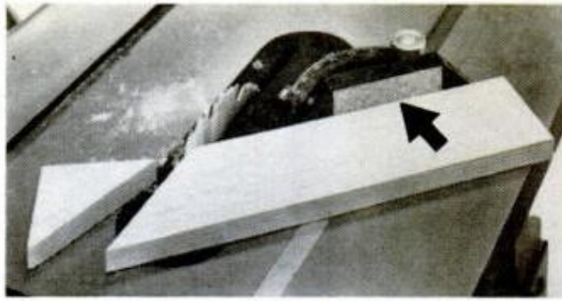
SANDPAPER GLUED to face of miter gauge will provide noncreep work surface when making miter cuts
