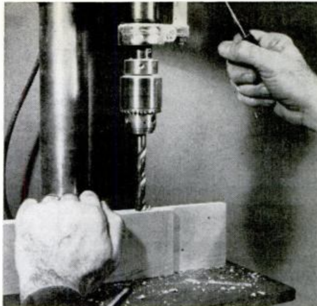
COUNTERBORE screw holes in seat-frame members, then use glue and the screws to assemble the frame
