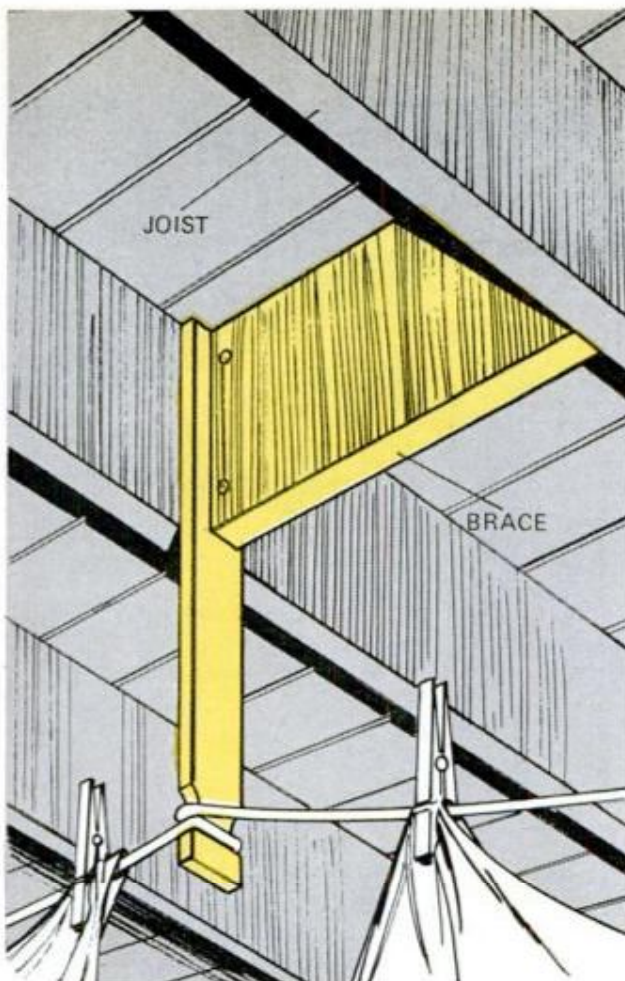
INDOOR CLOTHESLINE SUPPORTS will stay where you want them if they are braced as shown above. The bridging can be toenailed or held by nails driven through the joists.—R. E. Murray, Circleville, Ohio
