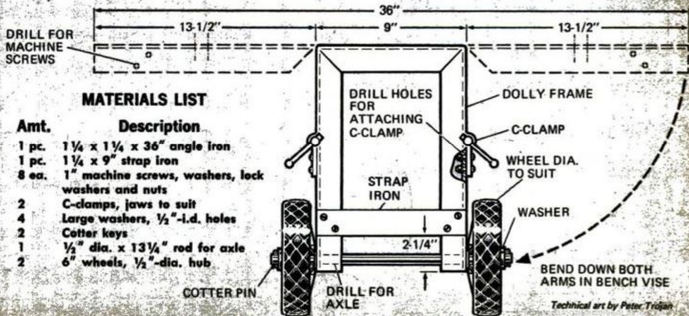
WITH LIGHTWEIGHT TOTOER you can single-handedly haul your small boat from storage to the big boat
