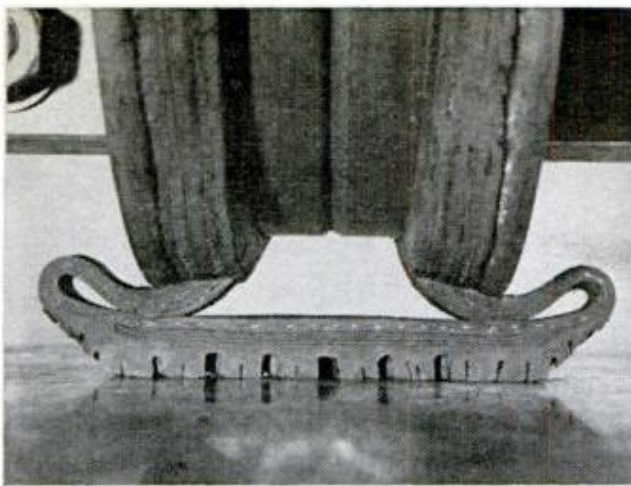
CUTAWAY OF TIRE at left shows tire after a blowout. Note the wide bead that remains in place. A special fluid inside the tire vaporizes immediately after the blowout to lubricate against friction, to seal small punctures and to partially reinflate the tire as you continue to drive on it as shown in the photo at right
