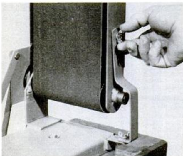
SLOTTED STANDBY BRACE helps support machine when swung to vertical position. Wingnut holds it
