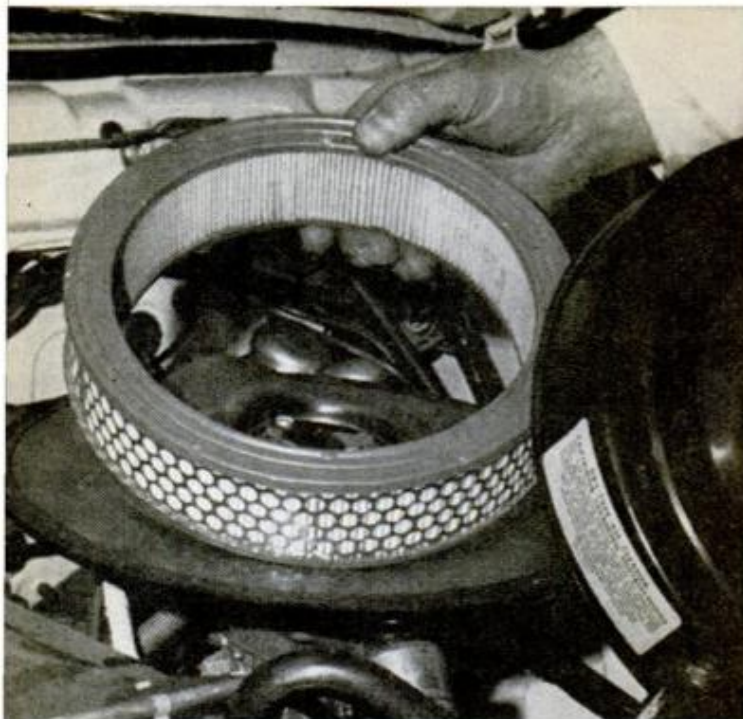
AIR-CLEANER PAPER ELEMENT is easily replaced. Often service intervals are on sticker on the cover
