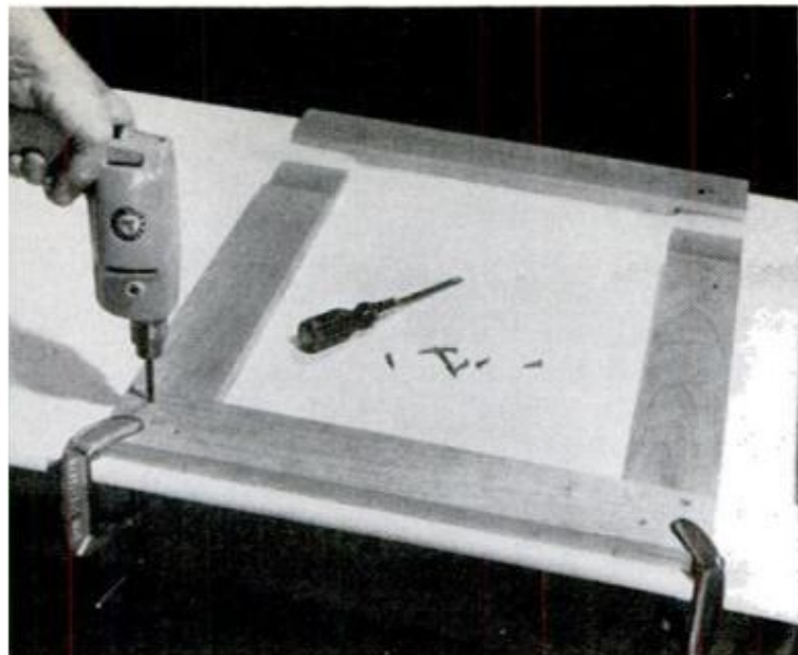
SEAT-FRAME MEMBERS are readied for assembly by boring two holes for \frac{3}{4} -in. screws at each corner
