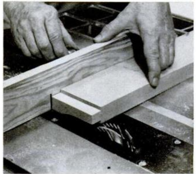
SHORT TENONS are made with one pass, each side, by switching from regular saw blade to a dado head
