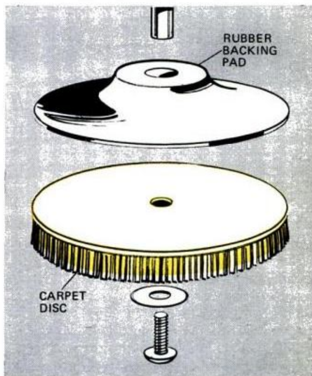
DISPOSABLE BUFFING PADS for power polishers can be fashioned from scraps of wool carpet. Just use the backing pad as a template; cut and assemble it like a sanding disc.—Lawton P. Evans, Seattle, Wash.
