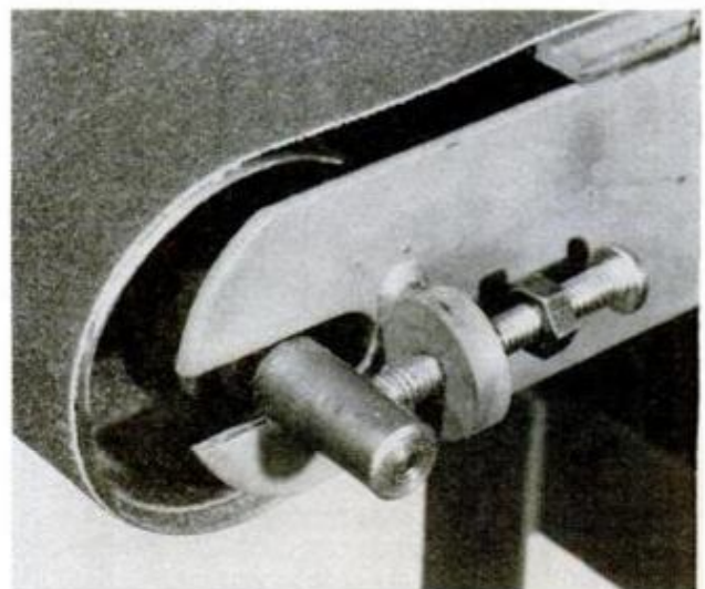
BELT TENSION AND TRACKING adjustment is made simply by turning a stovebolt against idler front roller
