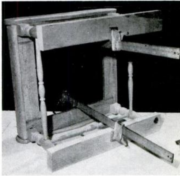
MINIMAL CLAMPING is required. Legs are bridged with two lengths of lumber to seat the leg tenons
