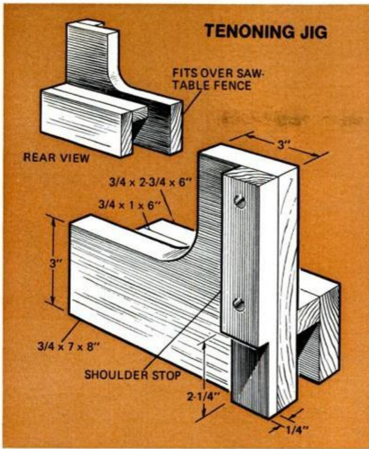
DESIGNED TO STRADDLE SAW FENCE , this homemade tenoning jig lets you cut accurate-fitting tenons safely on narrow stock. Diagrams show how jig is made from scrap wood. In use, work is clamped to jig
