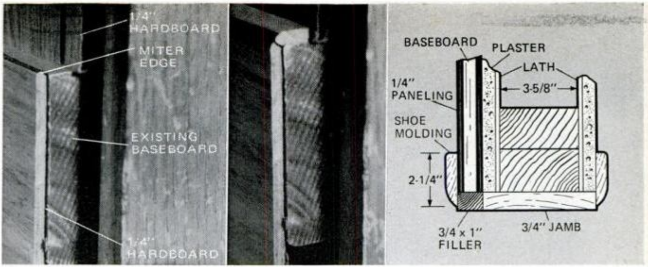
EXISTING BASEBOARD was left for 4x8-ft. panels to rest on. Base was then concealed with strips of the paneling ripped to width on table saw. Drawing shows pine filler-strip added to the existing jamb
