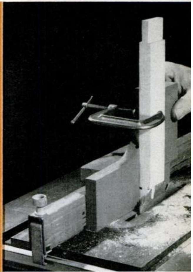
DESIGNED TO STRADDLE SAW FENCE , this homemade tenoning jig lets you cut accurate-fitting tenons safely on narrow stock. Diagrams show how jig is made from scrap wood. In use, work is clamped to jig
