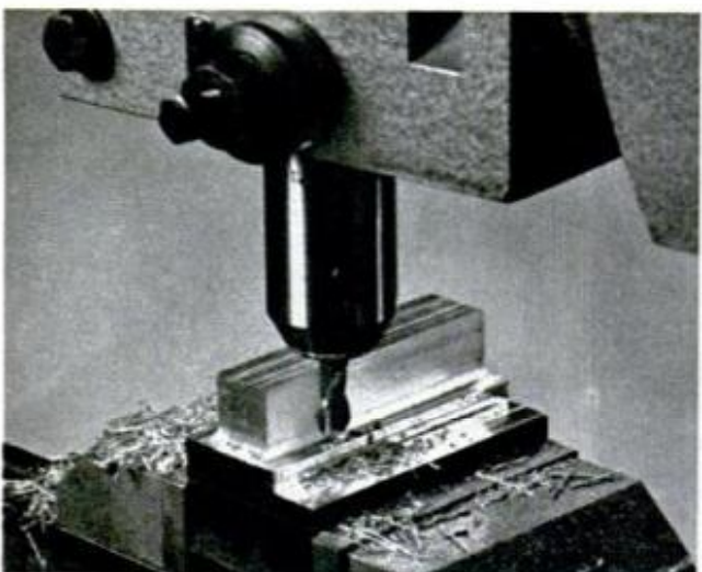
END MILLS are available in a variety of shapes, can be used to mill complex parts from solid stock
