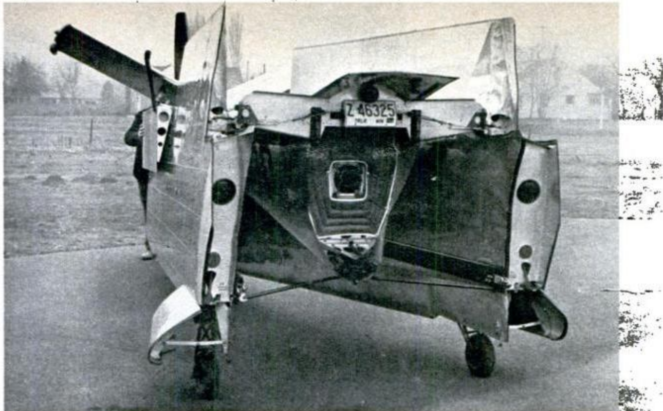
THE FLIGHT TRAILER , towed backwards on the road, is turned around on its small wheels to mate with car
