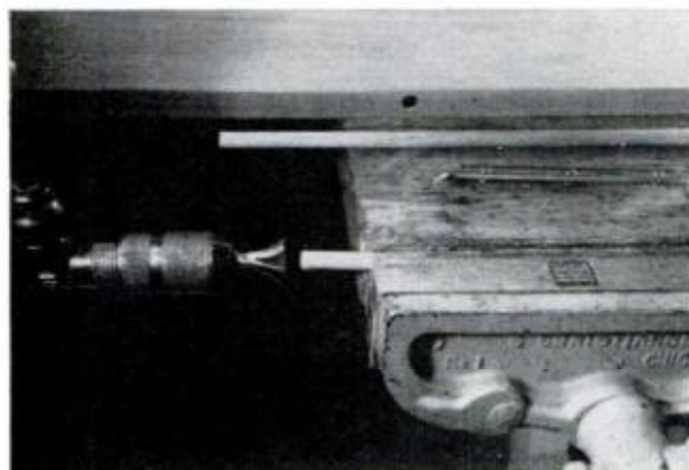
DOWEL SHARPENER is used to taper both ends of dowels, simplifying the job of inserting them into holes. Model chucked in brace above is from Stanley AUGUST 1971
