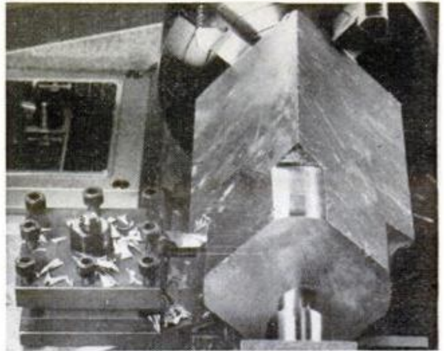
LATHE'S GEARED SPINDLE gives good power for smooth, interrupted cuts as in rounding square stock
