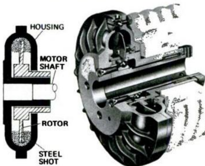
FLUID PROP DRIVE uses steel shot which pack between rotor and housing, providing no-slip coupling
