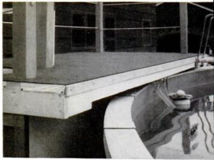
PLATFORM OVERHANGS pool slightly; measurements might vary from drawing to suit different size pool
