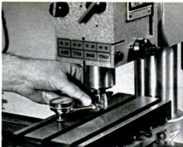
DIAL INDICATOR on an arbor makes it a simple task to set vertical spindle perpendicular to the worktable
