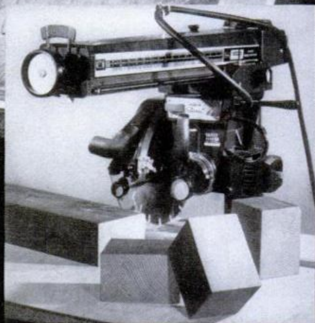
PLYWOOD PANEL (top) was easy to rip on this new saw. Tool also sliced 4x6 timber (above) effortlessly.
