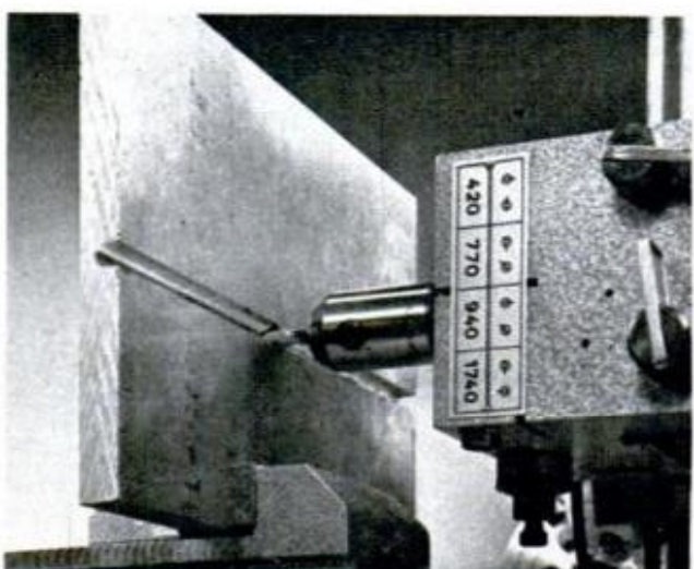
THICK METAL is easily cut if slotted with a two-flute mill until stock is thin enough for hacksawing
