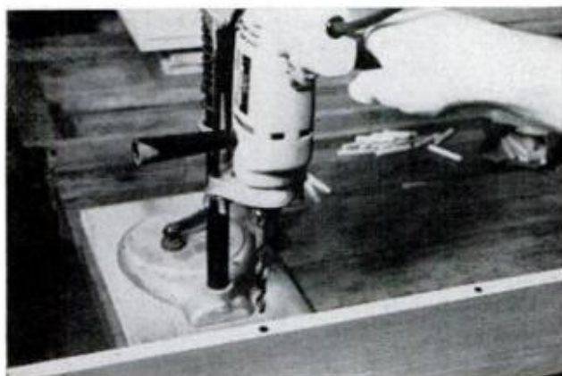
STUBBY SPUR BIT won't drift from center point as metal bits often do, and it will also drill deeper than a spade bit without piercing the other side
