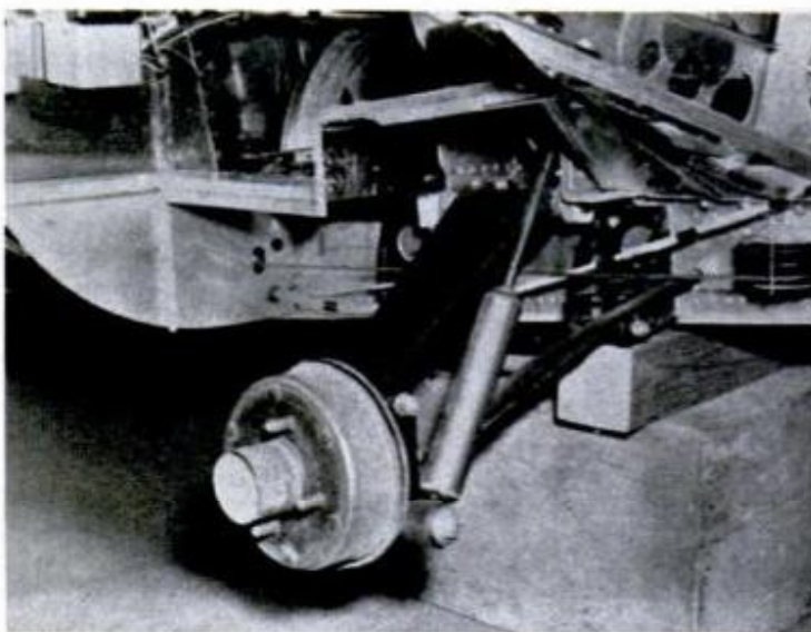
RETRACTABLE WHEELS are extended for takeoff, retracted for flight. A midposition is for road use
