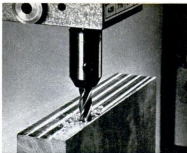
WITH DEPTH SET , end mill machines surfaces perfectly flat with successive cuts, moderate power feed
