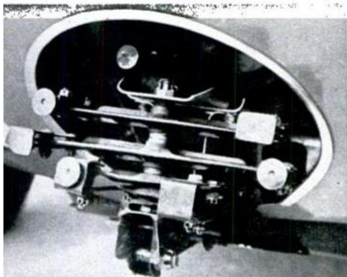
AIRCRAFT CONTROL connectors on car automatically lock to matching connectors on flight component
