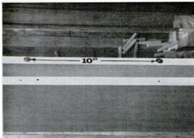
DOWEL CENTERS are slipped in holes bored in first board; then, to transfer centers to second board, both boards are lined up and tapped with a mallet
