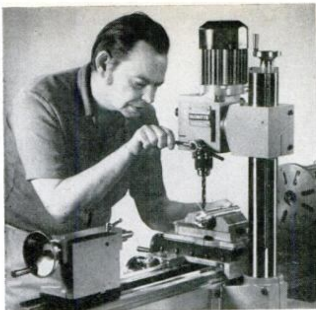
FOR DRILL-PRESS WORK , compound slide is unbolted from carriage worktable, replaced by machine vise
