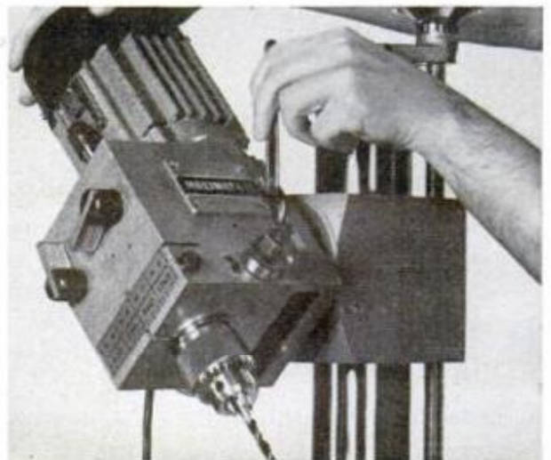
DRILLING-MILLING HEAD rotates 360^\circ in its mount. The rotating column permits compound-angle settings
