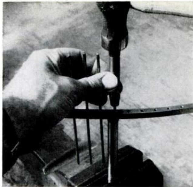
RIBS are driven with special setting tool. After all ribs are in place, cut them to the shape of a fish
