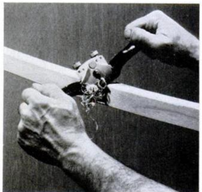
USE A SPOKESHAVE to round off the 1/8-in. plywood facing that must be added to one side of frame
