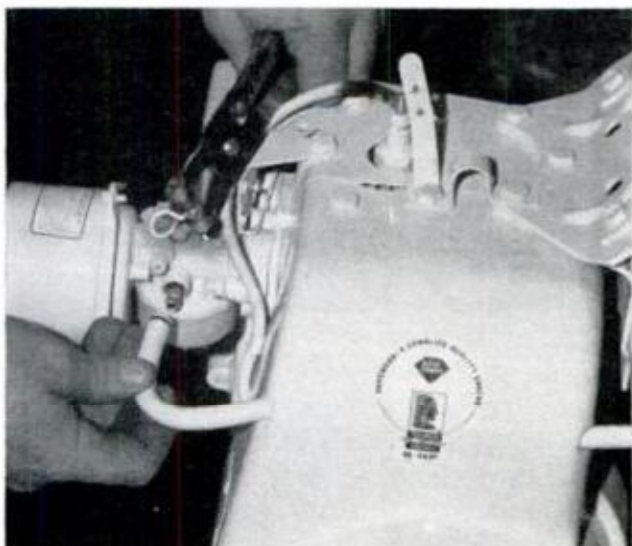
FUEL STOPPAGE AT CARBURETOR? Unhook fuel line at carb. Fuel flows? It's getting to, not through, carb MARCH 1971
