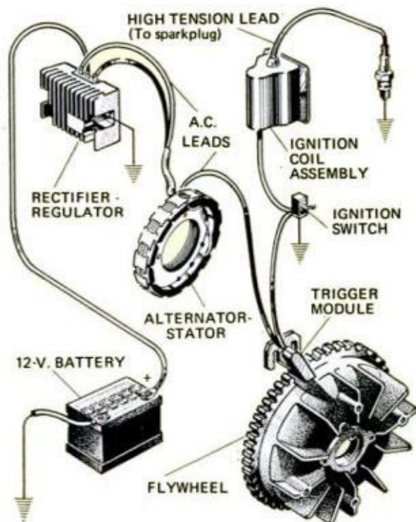
SOLID-STATE IGNITION on some Wisconsin, Kohler and Lauson-Tecumseh tractor engines uses electronic devices that eliminate breaker points. The timing is permanently set and will need no adjustment
