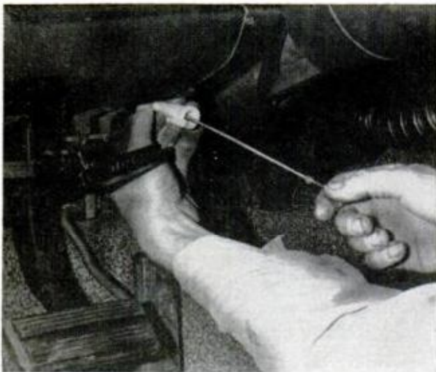
IN TRANSMISSION PINION SYSTEM, detach cable from speedometer head, then pull it from housing
