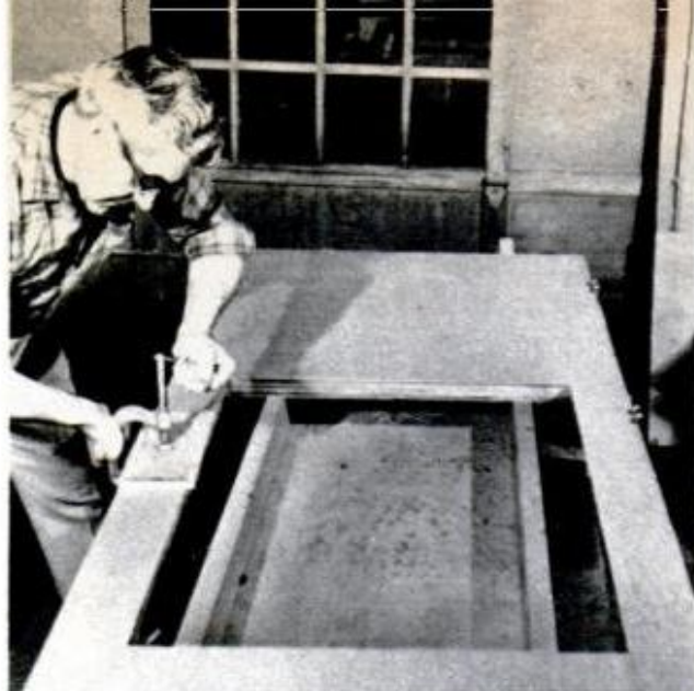
POSITION PANEL and drive a few brads to prevent it from shifting. Use weights until the glue is dry
