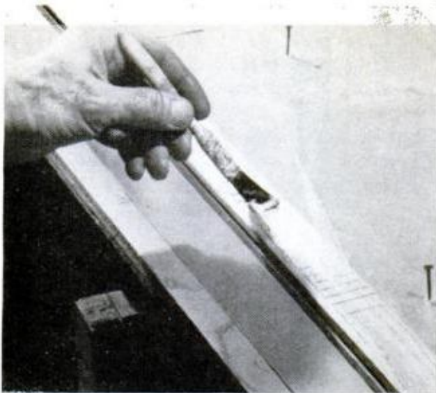
WATER-SOLUBLE GLUE , mixed with fine sawdust, is brushed into the kerfs, serves as an effective filler
