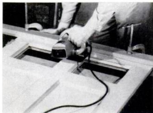
INTERNAL CUT required plunge cut with sabre or circular saw. Use straightedge for the neatest cut
