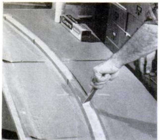
BEFORE GLUE DRIES , flex the strip to desired arch by bridging preset nails. Scrape off glue ooze-out
