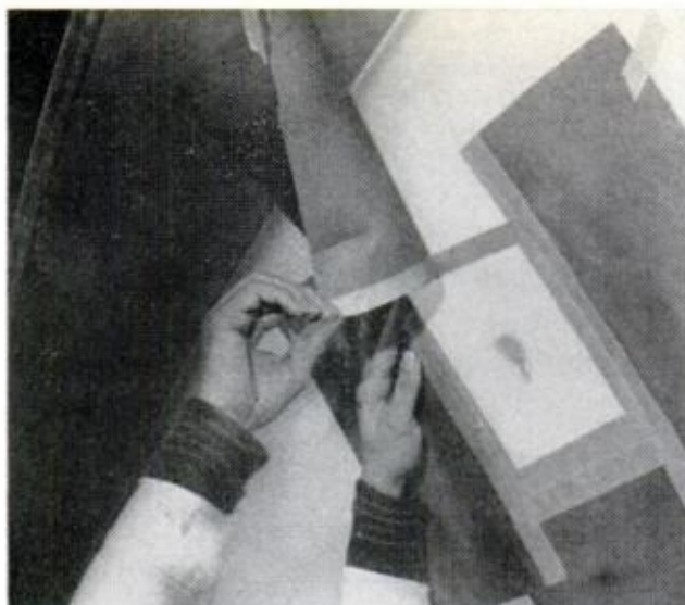
MASKING can be done before or after sanding the repair patch. It's necessary to avoid affecting adjacent areas, especially if gel coat is applied by spray
