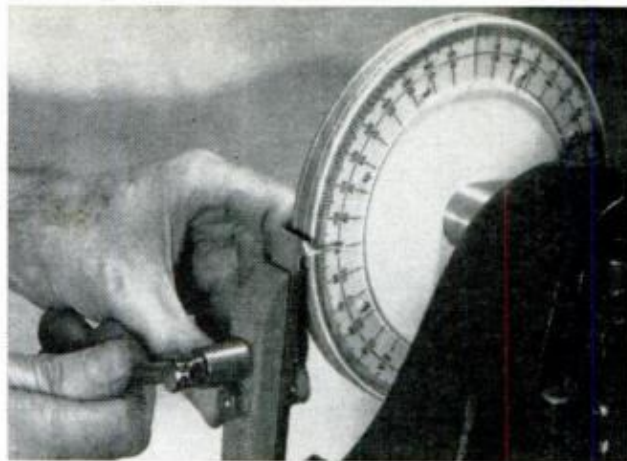
PROTRACTOR EDGES are concentric with a center hole. Simple pointer is cut from a sheet of aluminum
