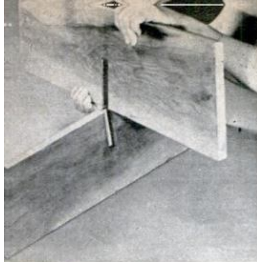
CROSS BRACES are joined, using a snug half-lap joint. Apply glue generously to the mating surfaces
