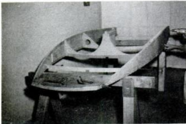
BOAT CAN BE BUILT on two sawhorses with top members parallel; use cord to hold the side planking
