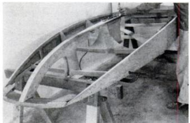
GLUE IS APPLIED and keel is sprung into position. Use clamps to hold forward deck-beam blocking
