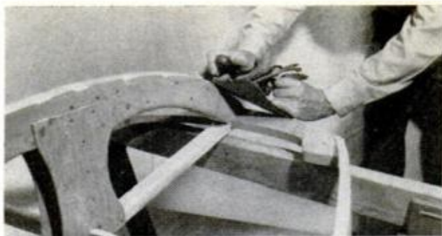
AREAS BETWEEN GROOVES are removed in a smooth, sweeping curve to eliminate any humps or dips
