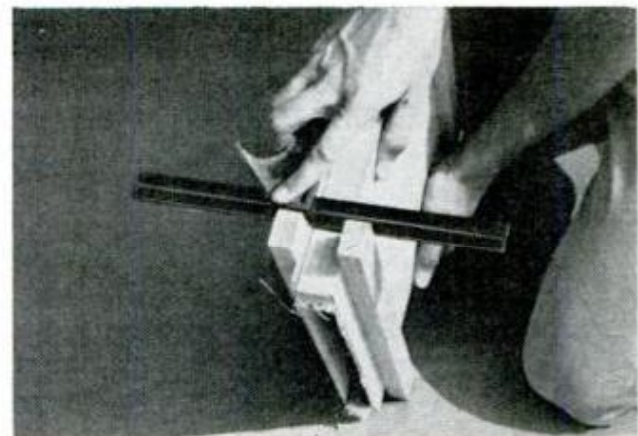
DAGGERBOARD TRUNK is fiberglassed inside before assembly. Below: Bed logs must be carefully aligned
