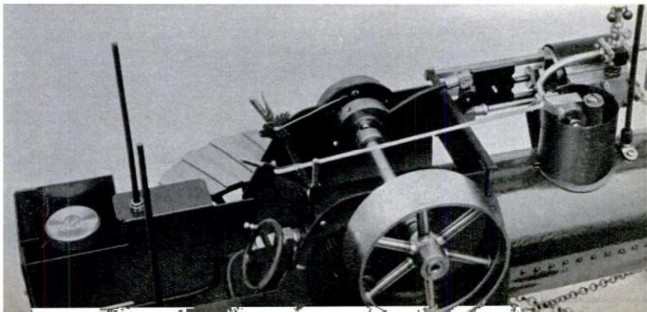
DISPLACEMENT LUBRICATOR supplies oil to inner "works" of cylinder. Small valves are for let-off
