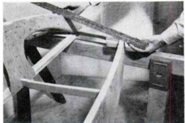
YARDSTICK is used to simulate planking which must rest on both keel and chine and not just one edge
