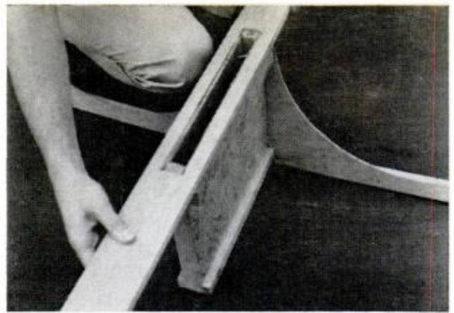
KEEL IS PRECUT to fit over the daggerboard trunk. Both ends are left oversize for custom fitting
