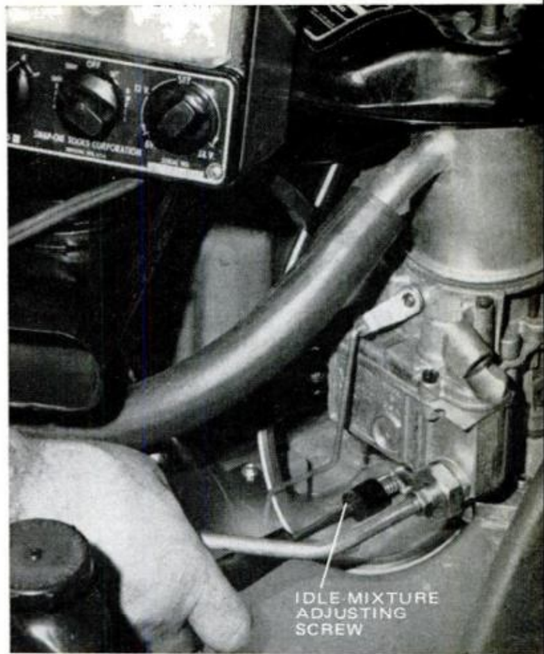
CARBURETOR ADJUSTMENT is made using tachometer to get right idle mixture for optimum performance
