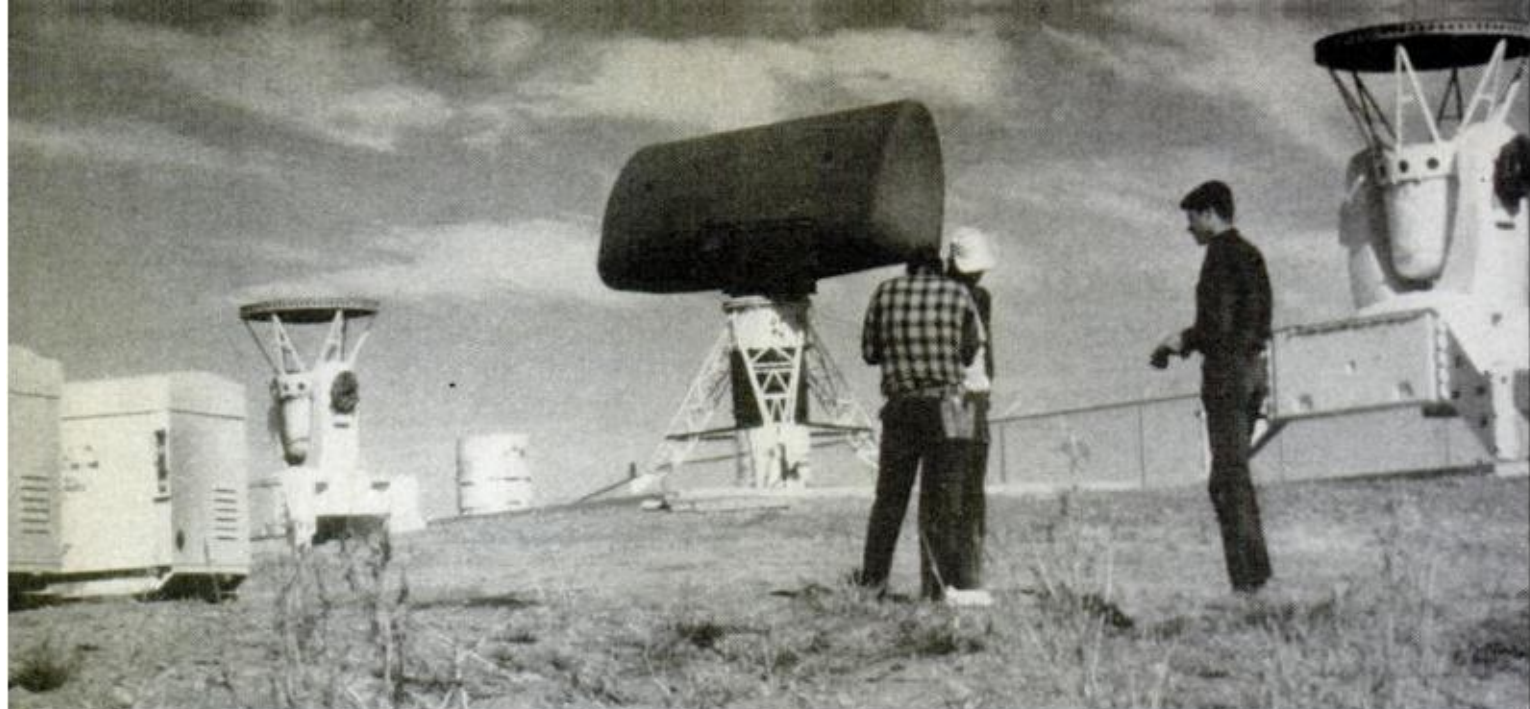
RADAR INSTALLATION IN COLORADO is used to track high-flying balloons for wind computations and to scan for precipitation echoes. Work is part of research involving the seeding of wintertime snow clouds
