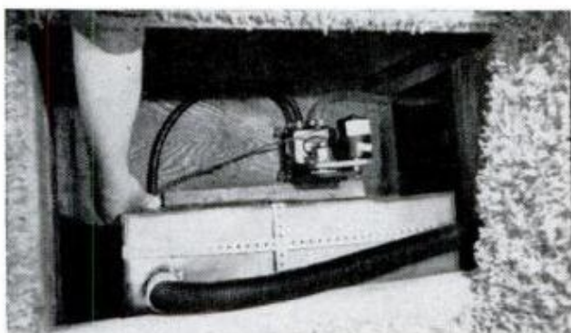
WATER PUMP , easily accessible, is neatly hidden from view under cutaway section of carpeted deck
