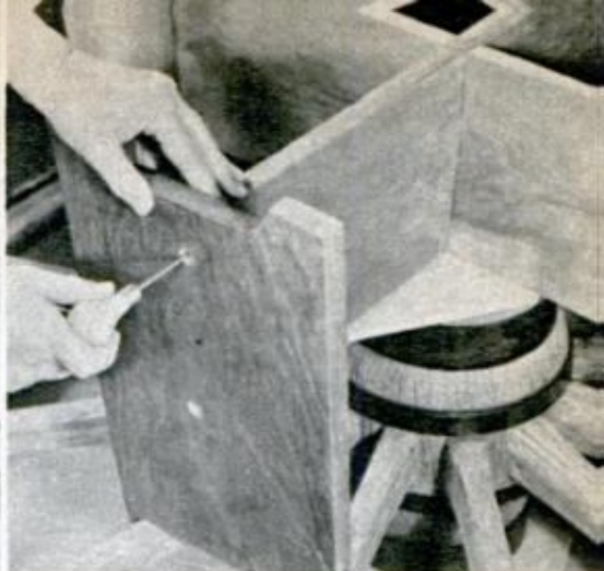
COUNTERBORE the legs about \frac{1}{8} -in. deep to conceal the screw-head, finishing actual assembly
