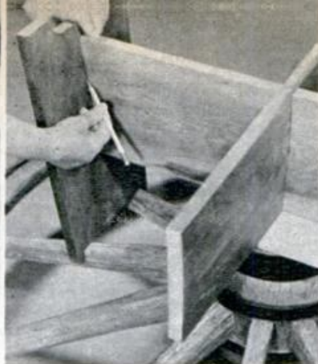
EACH LEG is marked, drilled and attached to cross brace individually to assure its proper location
