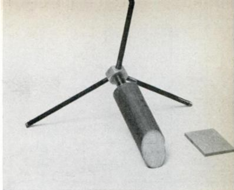
SPIDER for diagonal consists of broom handle cut at 45° miter, a \frac{3}{8} -in. bolt with head cut off and three lengths of threaded rod into \frac{3}{8} -in. tapped nut
