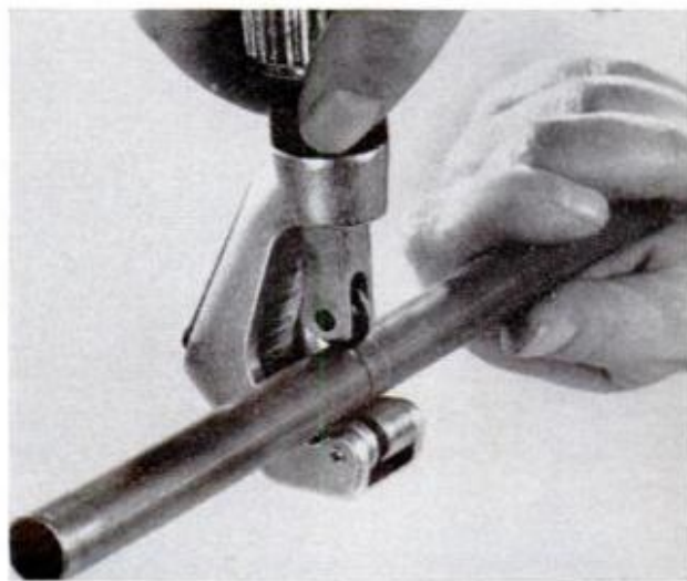
TUBE CUTTER cuts any type copper tube. Burr (below) is reamed out with the cutter's triangular reamer
