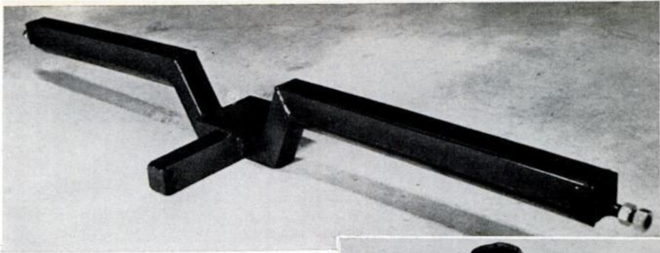
2. OVERDRIVE SUPPORT cross member, made from 1½ in. steel tubing, has dip for most ground clearance
