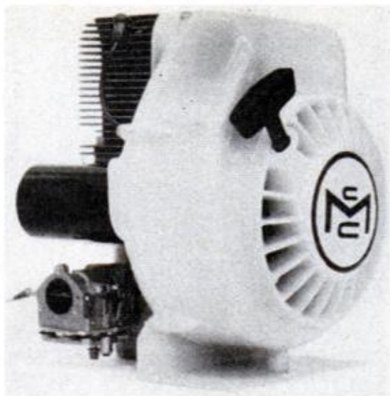
TWO OF McCULLOCH'S LINE of 12 new snowmobile engines are the 399-cc two-cylinder (left) and the 199-cc one-cylinder (right). Both engines boast a speed ranging between 2000 and 7000 rpm and a 2.75-in. bore
