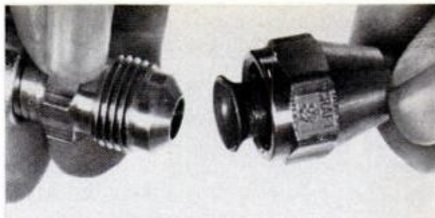
SLIP FLARE NUT on tubing with the threaded end out before forming the flare. Seat must be mar-free
