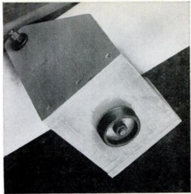
PIPE REDUCER (2½ to 2 in.) is bolted to yoke bottom. For smooth action, lap threads of reducer and flange with grinding compound, apply oil or grease
