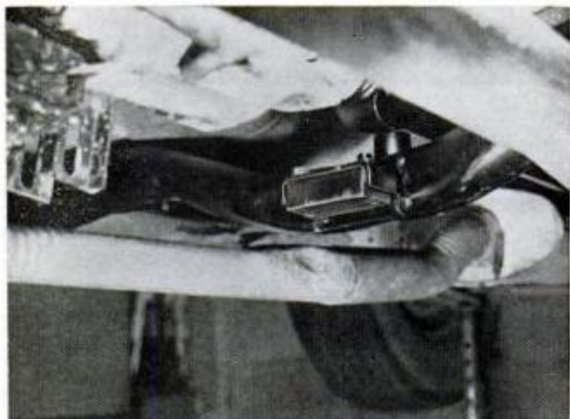
9. NEW CROSS MEMBER provides attachment point for the rear tongue of the overdrive cross member
