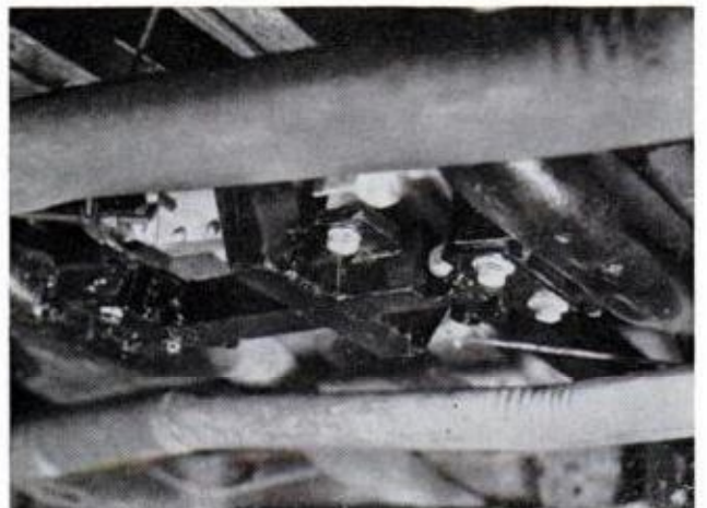
10. REAR TONGUE of overdrive cross member attaches same as front tongue, using a rubber isolator
