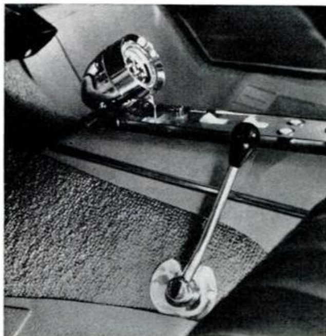
12. OVERDRIVE SHIFT LEVER mounts on side of transmission tunnel (also available for flat floors)
