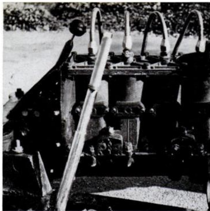
CONVERTED ENGINE , with pistons driven by steam, puts out between 30 and 50 hp. Car has gone 50 mph
