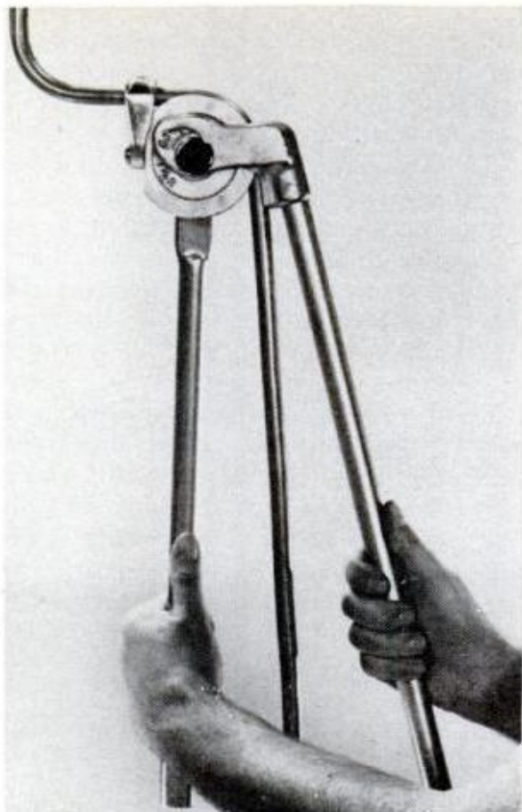
LEVER-TYPE BENDER makes wrinkle-free, short-radius bends. Rigid tube can be bent if torch-annealed
