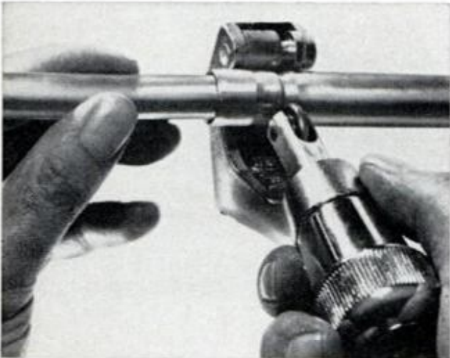
A CONSTRICTOR , a pipe cutter with roller, rolls a groove for sweating small-size tube into a large one
