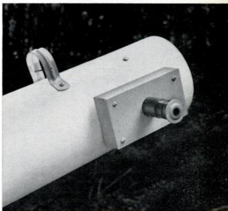
EYEPIECE ADAPTER consists of two pieces of plywood glued together with a 1\frac{3}{8} -in. hole at center to accept the telescoping brass tubing and the eyepiece
