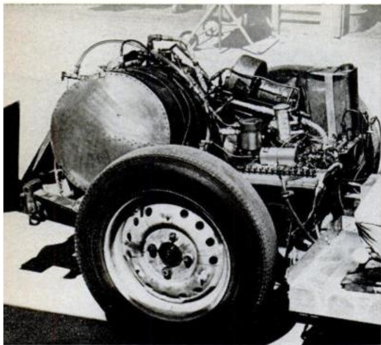
HIGH-PRESSURE STEAM is 700 psi and 650°F. as it leaves rear-mounted boiler on its way to the engine
