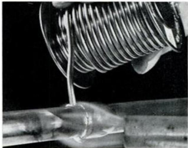
SWAGED OR CONSTRICTED JOINTS are soldered like solder-type fittings. Fill the joints with solder
