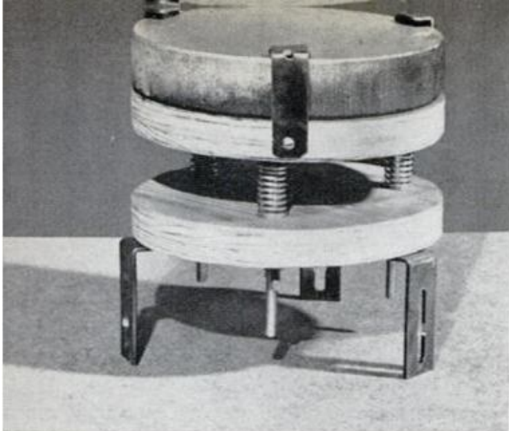
CELL FOR THE MIRROR is made of two plywood discs that are separated by three springs. The mirror is fastened to the top disc by means of three clips
