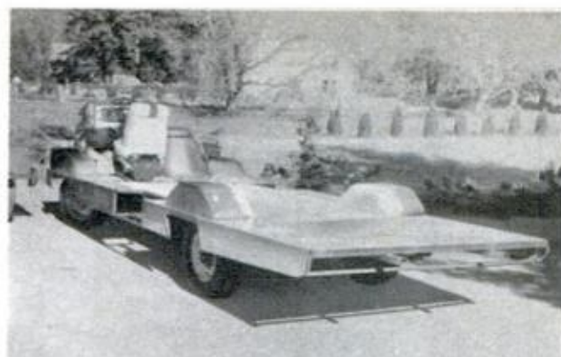
CHASSIS IS READY for sidewalls after old van body has been cut off. Frame is widened and lengthened
