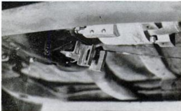
8. OVERDRIVE cross member's front tongue attaches at flange. Adjustment slots for static U-joint loading
