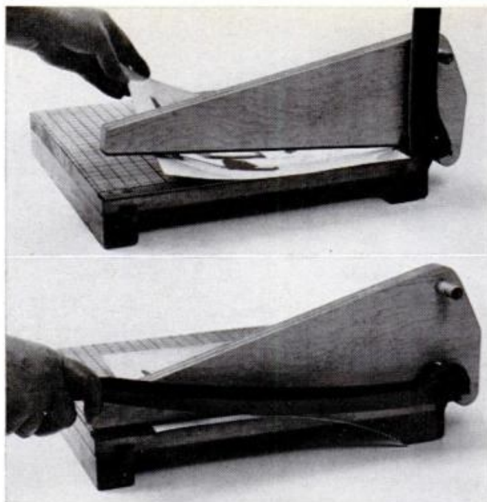
ARM LIFTS AUTOMATICALLY as cutter blade is raised to insert a print (top photo). Then it presses down as blade is lowered to grip print snugly during trimming (bottom)
