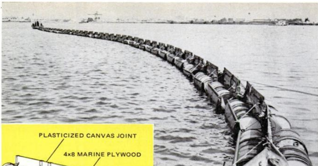
HEFTY BOOM developed by Murphy Pacific is deployed in the Gulf of Mexico to contain oil in Chevron spill. As drawing at left shows, there's nothing fancy about this oil drum and plywood barrier
