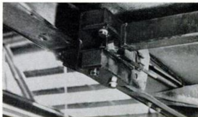
5. FOR MAXIMUM STRENGTH , horizontal mount is recommended for vehicles with adequate clearance
