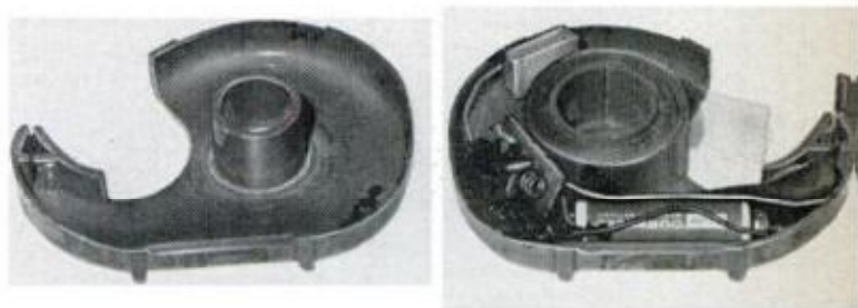
PLASTIC TAPE DISPENSER on executive's desk was hiding place for this battery-powered transmitter
