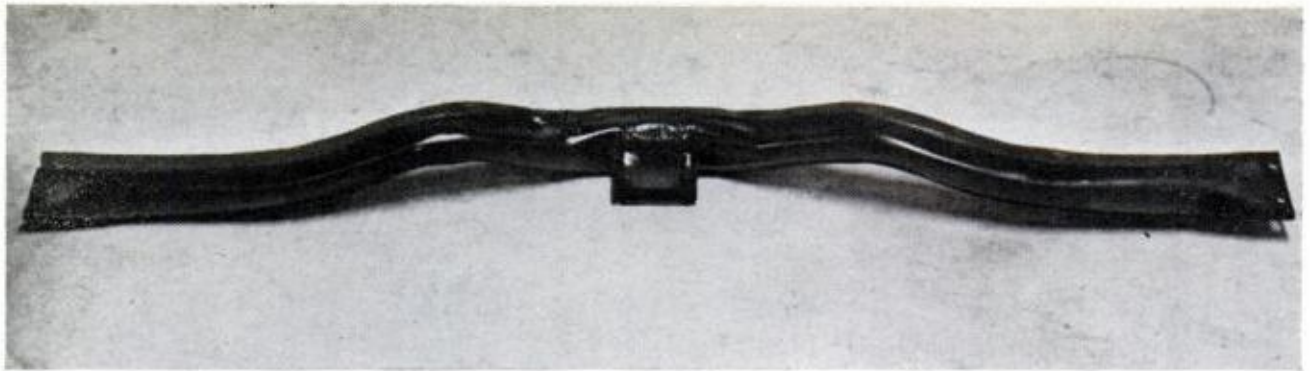
6. SECOND transmission support cross member with flange is installed behind the stock transmission support
