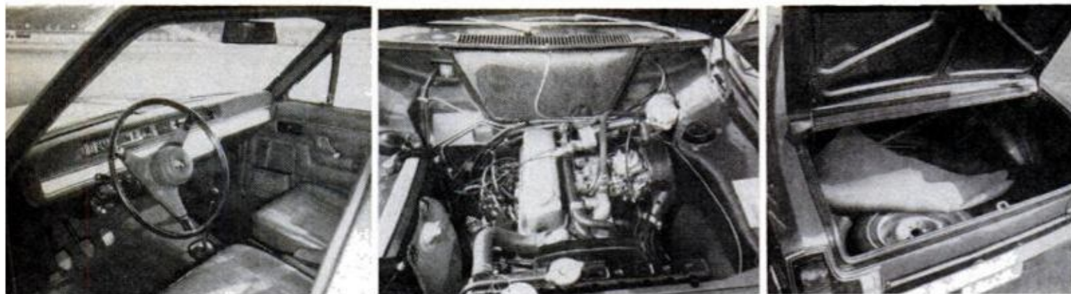
PLYMOUTH CRICKET , made in England, was styled here. Water-cooled ohv Four can be had with optional two-barrel carb, twin exhausts for 13 extra bhp. Trunk has 14-cu.-ft. space compared to 9 in Colt four-door
