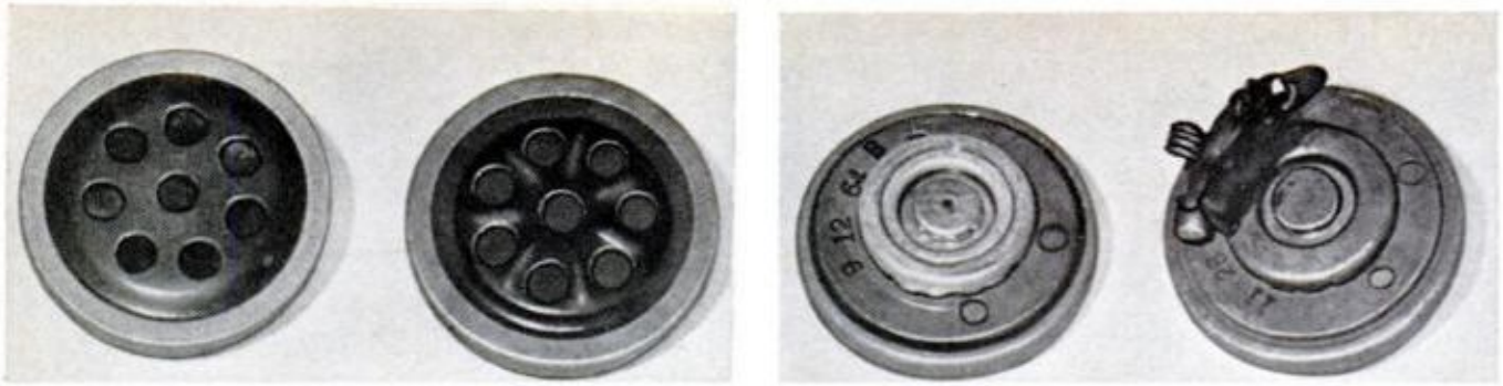
TWO TELEPHONE MOUTHPIECES at left seem identical when unscrewed from instrument. Debugging specialists check these first to look for the kind of tiny transmitter discovered on back of one (far right)
