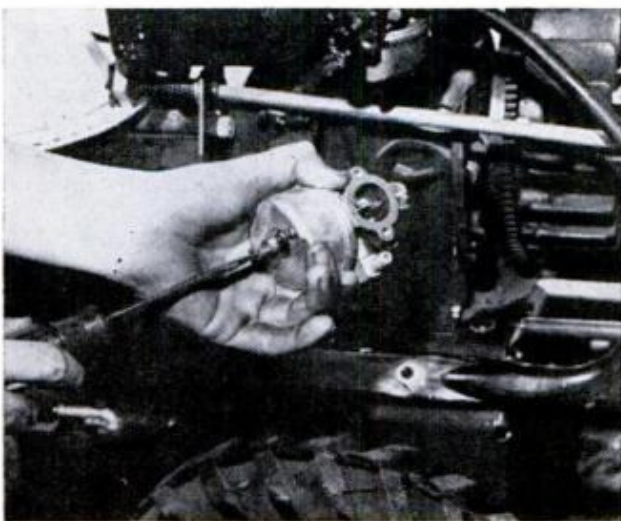
HIGH-SPEED ADJUSTING SCREW is sometimes under the carburetor in the bowl. If you remove the bowl to replace needle and seat, remove this screw, too
