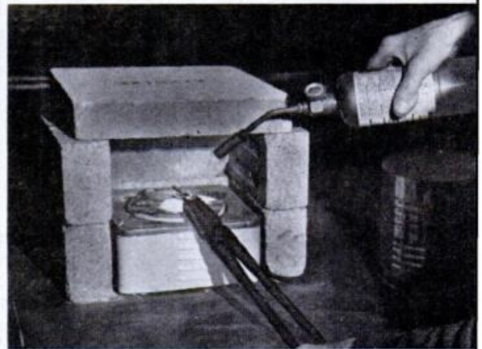
FLAME IS PLAYED back and forth until parts are cherry red, then parts are immersed immediately. Here, flame regains the heat loss caused by tongs
