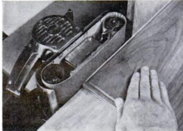
CLAMPED ON ITS SIDE , the belt sander can be used for "planing" jobs. Vertical board serves as a fence
