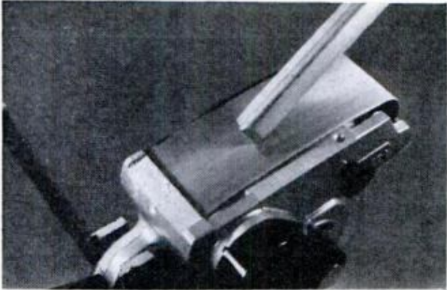
TO WORK SMALL PIECES , sander can be clamped upside down on the workbench to free both hands
