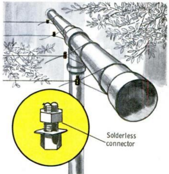
GOOD WAY TO ANCHOR wire clothesline to a post is with solderless connectors. Electricians use them to join wires. They can't rust because they're made of Bakelite. Use the large size.— Clarence Breitenfeldt
