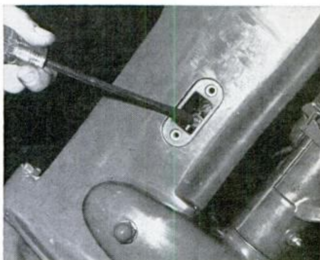
4. IF YOUR UNIT IS THIS TYPE, remove inspection cover and unscrew lower pin to disengage shift rod
