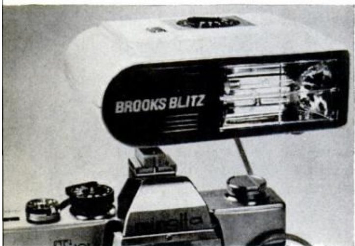
REVOLVING SHOE on some models, like this Brooks Blitz, lets you turn strobe vertically or horizontally. In horizontal position, light coverage is slightly broader, which is useful when shooting wide scenes
