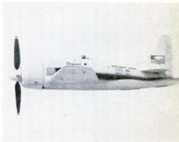
GREENAMYER'S BEARCAT , once a carrier-based Navy fighter, underwent many modifications, including addition of larger propeller and spinner, cutting back of wingtips, closing of air inlets and gunports
