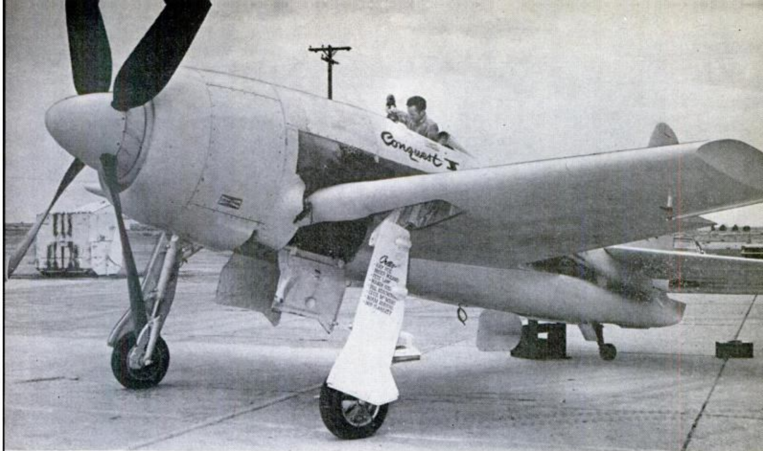
GREENAMYER'S BEARCAT , once a carrier-based Navy fighter, underwent many modifications, including addition of larger propeller and spinner, cutting back of wingtips, closing of air inlets and gunports
