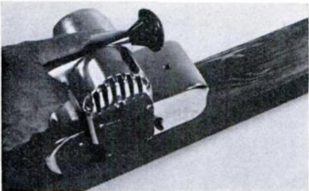
TO STRIP PAINT , use a coarse, open paper to start, then complete the job with finer, closed-coat belt
