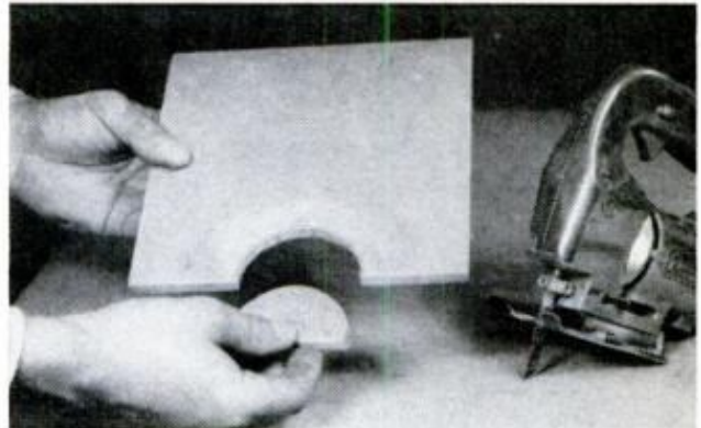
SAWING QUARRY TILE when fitting it around floor pipes and other obstructions is no problem. Here abrasive-coated blade works best at a slow speed
