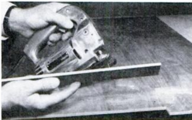
SINCE BLADE CUTS on both forward and reverse strokes, kerf in plywood is sand-smooth, splinter-free
