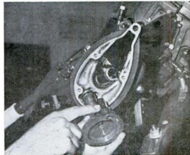
14. CHECK WATER TUBE fit in water-pump housing
