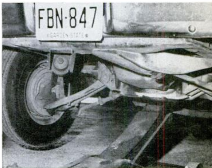
JACK IS PLACED beneath the front cross member to check upper compression-loaded ball joint on this 1967 Falcon. Coil spring is on the upper control arm
