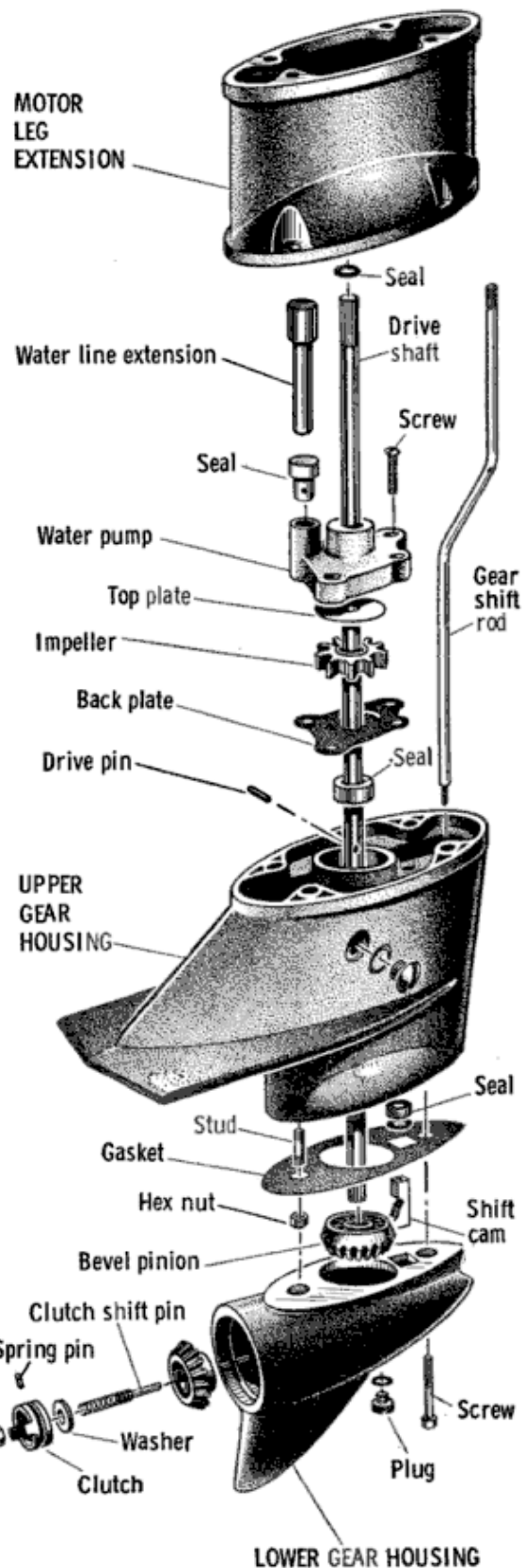
TYPICAL LOWER UNIT
