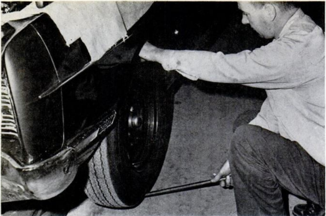
UP-AND-DOWN MOVEMENT of ball joint is checked using a pry bar beneath tire to force wheel up and down
