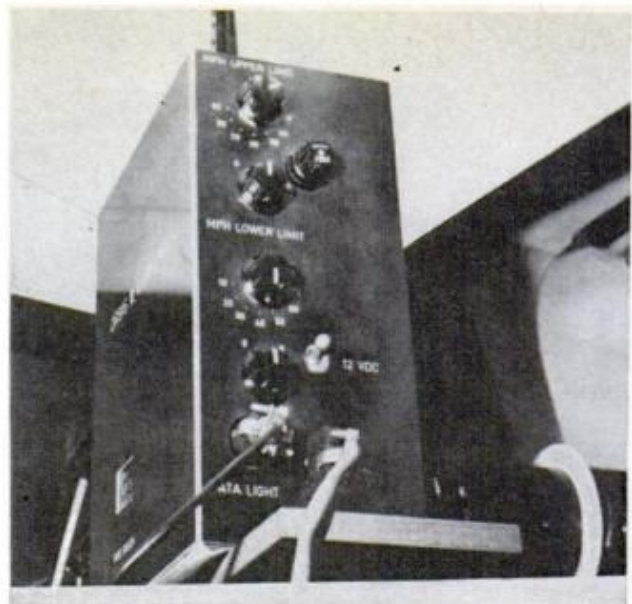
BRAIN OF SYSTEM is computer, with dials to set upper and lower limits. It trips camera, illuminators
