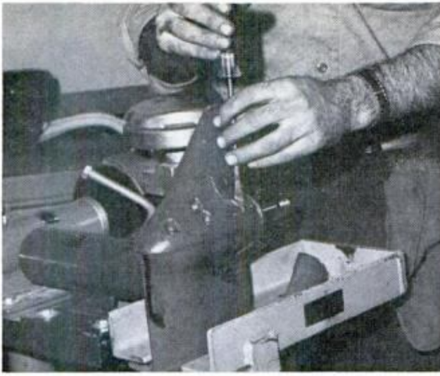
11. LIFT GEAR TRAIN carefully from the gearcase
