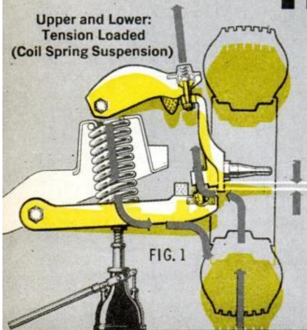
Upper: Tension Loaded Lower: Compression Loaded (Coil Spring Suspension)
