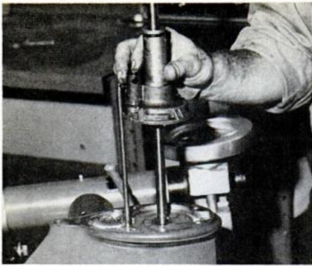
7. DETACH WATER-PUMP HOUSING , slide off shaft
