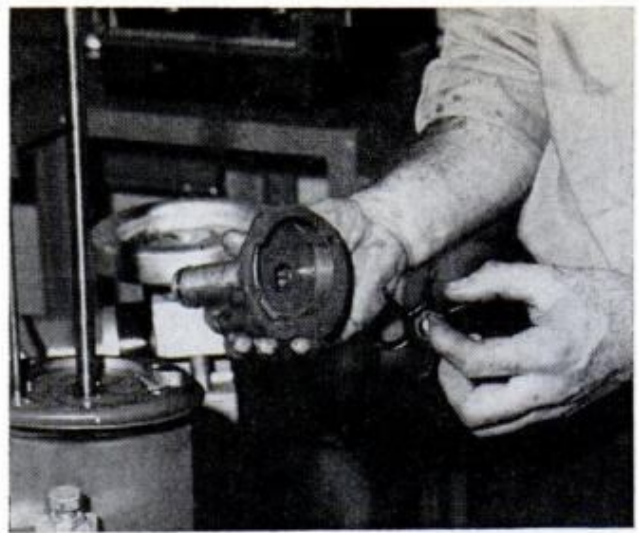
8. REMOVE IMPELLER from the water-pump housing
