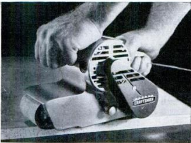
USING AN 80-GRIT BELT , plastic laminate self-edge is quickly and easily smoothed flush with plywood
