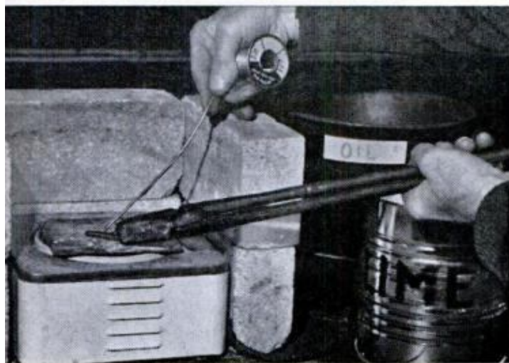
TEMPERING TECHNIQUE. Punch is tested with piece of solder for correct drawing of heat. Solder begins melting and starts flowing at approximately 400° F.
