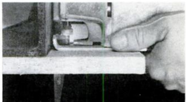
SHAPE OF FLUSH-CUT BLADE lets you cut right up to a vertical surface without saw interference
