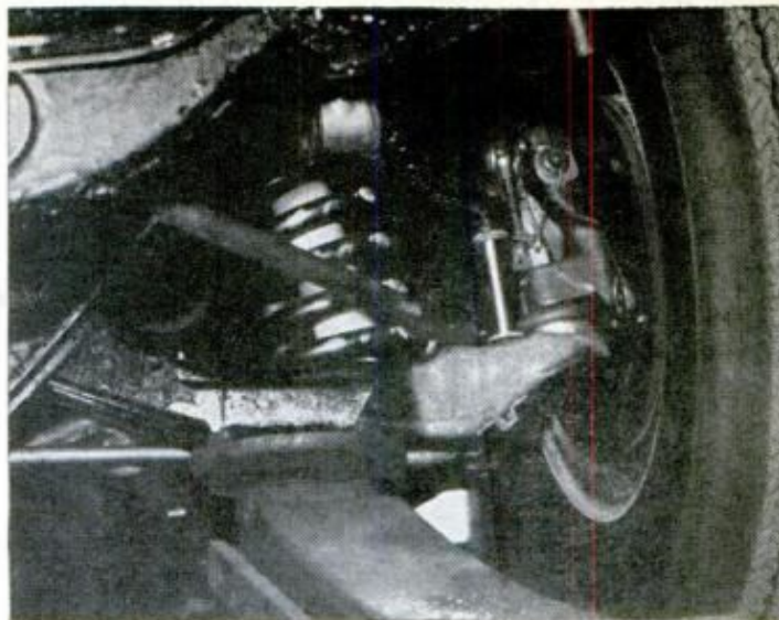
JACK IS PLACED as close as possible to center line of spring to check lower tension-loaded ball joint. Coil spring is on lower control arm. Car is '69 Ford
