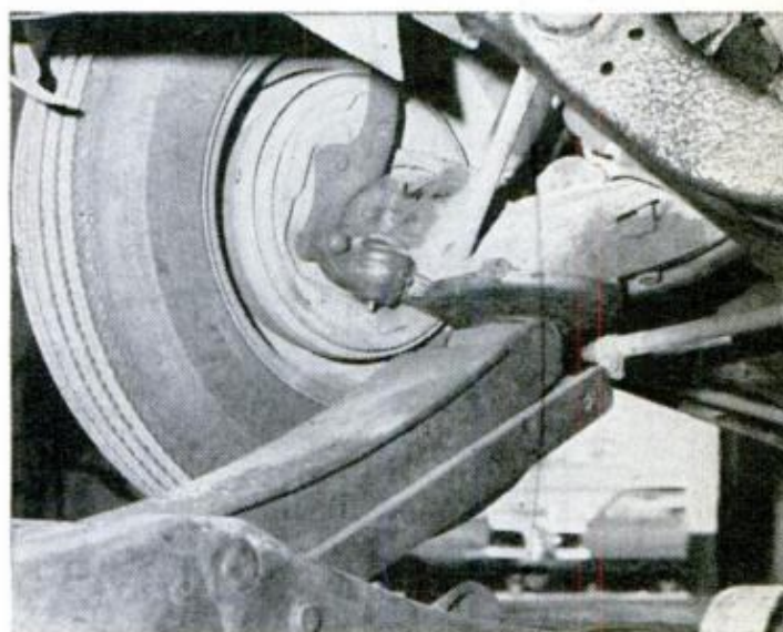
TO CHECK lower compression-loaded ball joint of this 1965 Dodge (which has torsion-bar suspension), jack is placed as close as possible to the wheel
