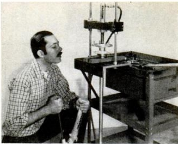
PRESSING AXLE BEARING is easy and fast. Hydraulic-control characteristics insure smooth pressing job
