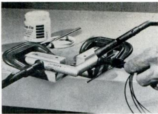
SIMPLE WOOD JIG holds the work securely, is built with space between the blocks to prevent scorching
