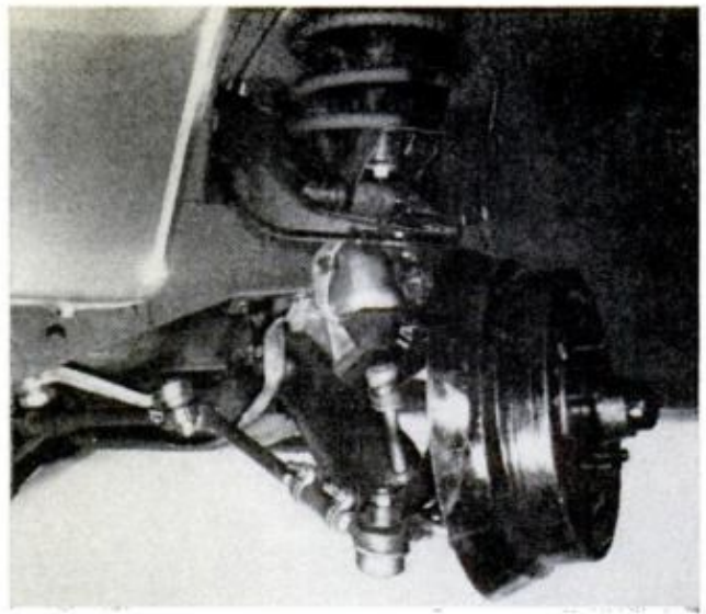
AMC cars for 1970 offer new twin-ball-joint front suspension. System features antinosedive braking
