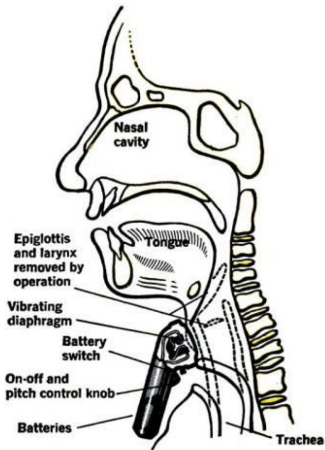
ELECTRONIC LARYNX is simple vibrating device that makes speech possible for those whose larynx has been removed (usually because of cancer.) Pressed against neck, the electrolarynx's vibrating diaphragm substitutes for the vibrations of vocal cords. Components (left) are vibrating transducer, mercury batteries and two transistors—an amplifier and an oscillator
