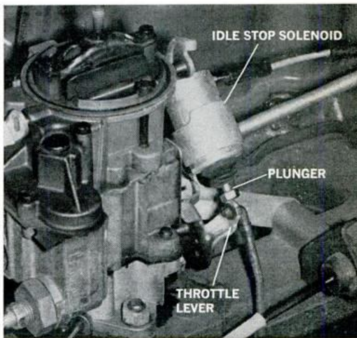
IDLE-STOP SOLENOID on some newer cars operates a plunger that retracts to allow the complete closing of the throttle when the ignition is turned off
