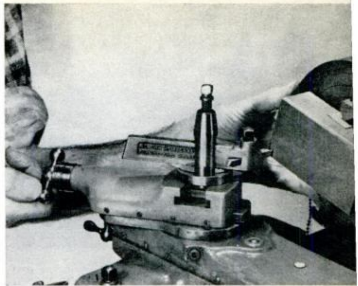
MICROMETER SCALE used on compound slide is angled at about 30^\circ to check alignment of block being machined to reduce thickness, true up the surface
