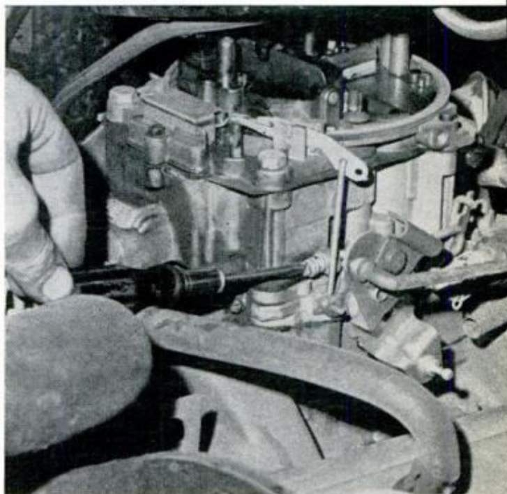
CARBURETOR ADJUSTMENTS include fast-idle setting that's right on specification. Turn the fast-idle screw until tachometer reads the correct engine rpm
