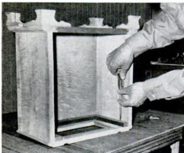
BASE IS COMPLETED when upper frame is attached with screws turned up through the fastening strips
