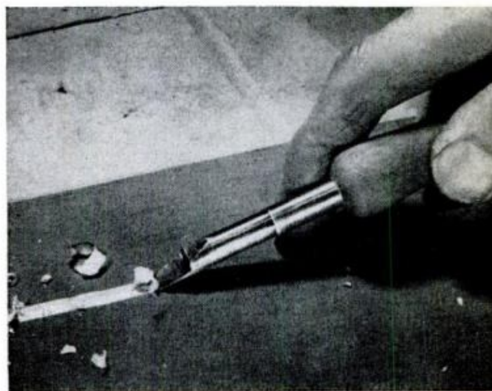
CUTTING EDGE OF GOUGE was formed with compound slide set at about 15° angle to lathe axis. Radius of swing was approximately 3/8-in. minimum
