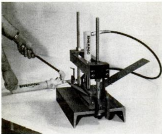
SMOOTH 90° BEND is made with reduced opening. Clamped steel acts as female die, bar serves as mate
