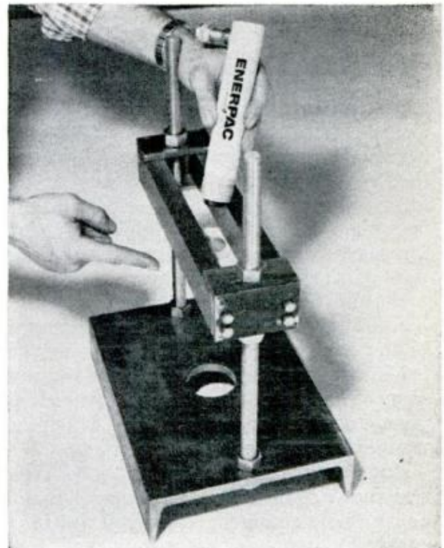
MOUNTING FLANGE bolted to header, receives the threaded end of cylinder, securely holds it in place
