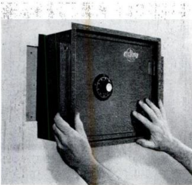
3 SAFE IS SHOVED in opening until flanges are seated. Pilot holes for bolts are made in studs
