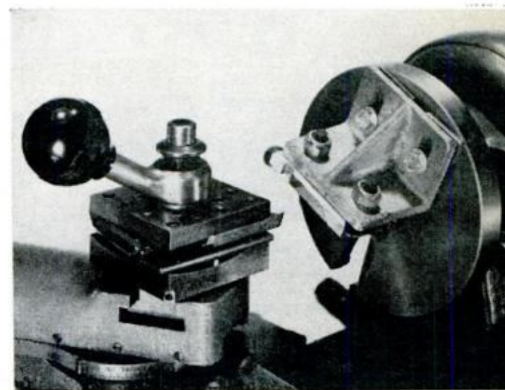
MACHINING A FLAT END of \frac{1}{2} -in. steel rod, slightly curved margin is usually not objectionable. Below, workholder is used when planing small work
