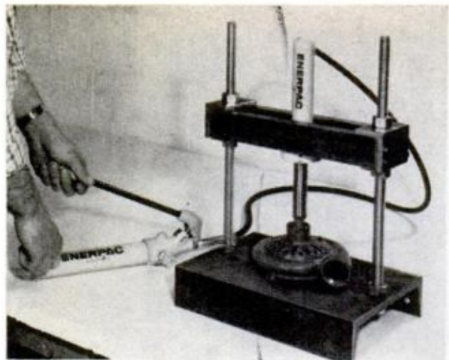
NEW BEARING being pressed in, pushes out old bearing through hole in base plate in the same operation
