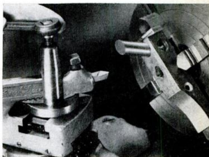
MOUNTED AT AN ANGLE to chuck or faceplate, end of rod is machined flat and diagonal. Here, end slope depends on angle of hole drilled in holding block
