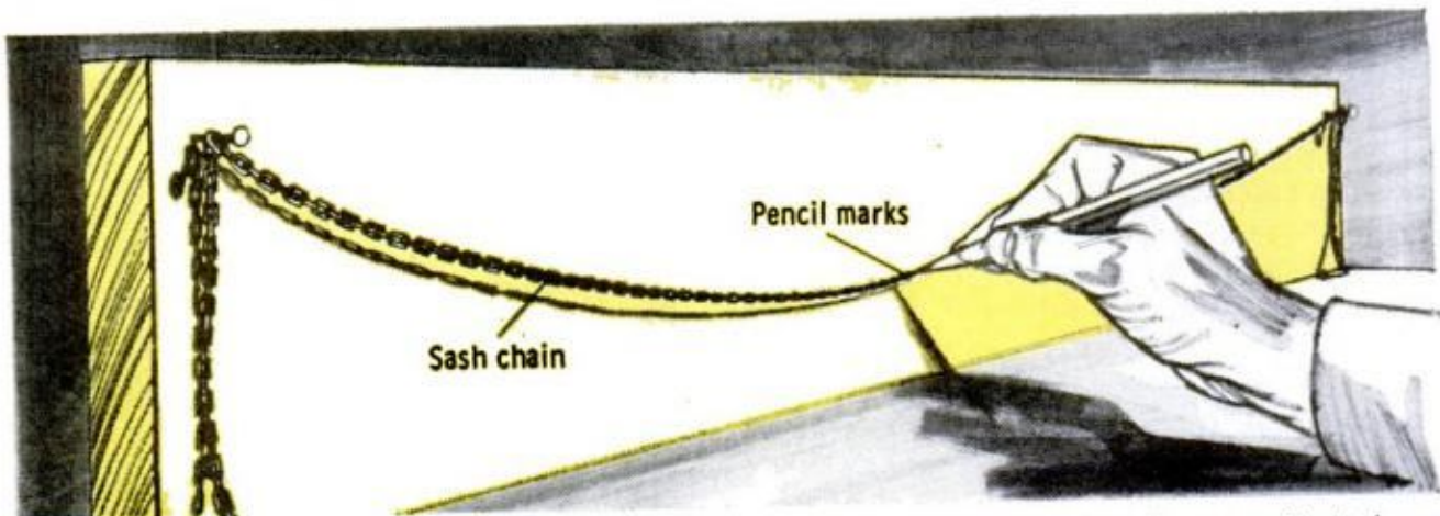
LENGTH OF SASH CHAIN makes simple compass for drawing large arc. Suspend chain by two nails, let hang free and make a dot every four or five links. Then connect dots to form unbroken line.— Victor H. Lamoy
