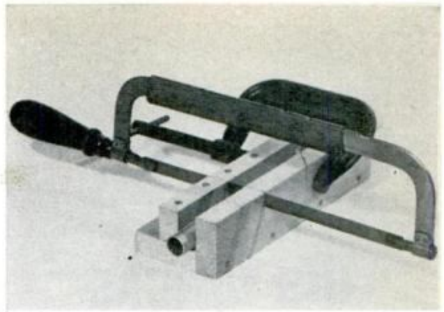
DO ALL CUTTING with a 32-tooth hacksaw. Miterbox will assure craftsmanlike square and miter cuts
