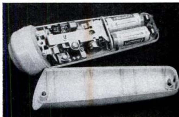
ELECTRONIC LARYNX is simple vibrating device that makes speech possible for those whose larynx has been removed (usually because of cancer.) Pressed against neck, the electrolarynx's vibrating diaphragm substitutes for the vibrations of vocal cords. Components (left) are vibrating transducer, mercury batteries and two transistors—an amplifier and an oscillator
