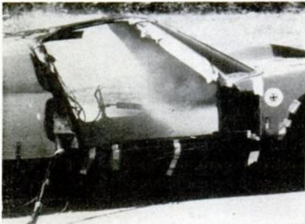
IN LESS THAN AN EYE BLINK , Freon floods cockpit to snuff out fire before you even see a flame
