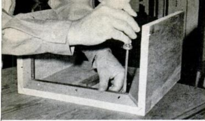
SCREW-FASTENING STRIPS are glued and screwed inside the three-sided base, flush with the top edge
