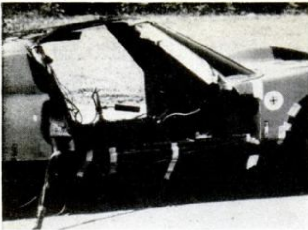
FIRE IS STARTING to break out in this wrecked sports car used in test of new Freon extinguisher
