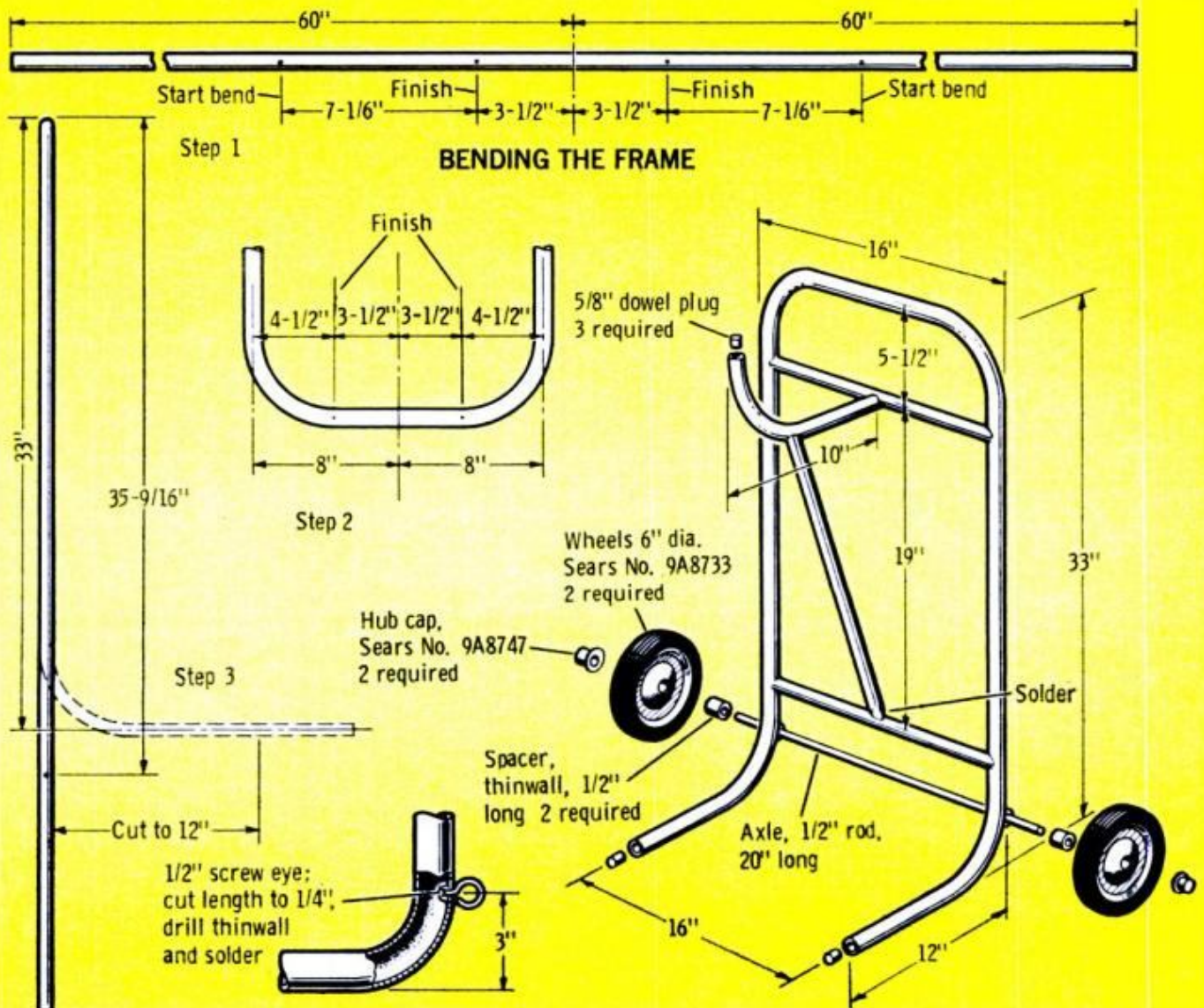
HOSE CART
