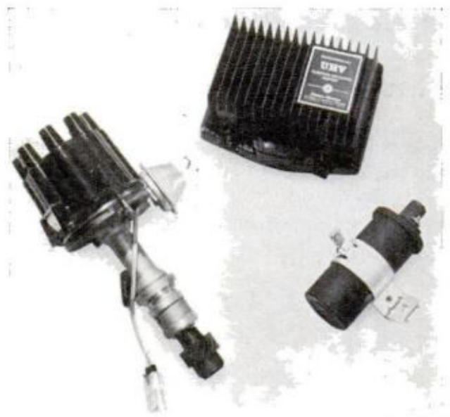
CAPACITOR DISCHARGE ignition system builds up high voltage for firing sparkplugs, prevents fouling
