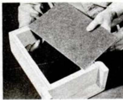
BACK OF CASE fits flush in rabbets previously cut in top and sides. Back laps bottom of case
