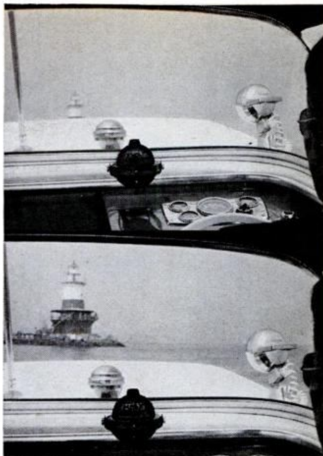
HELMSMAN'S VIEW while climbing to plane demonstrates tab's safety advantages. Top photo was taken as boat was squatting; bottom, on reaching plane
