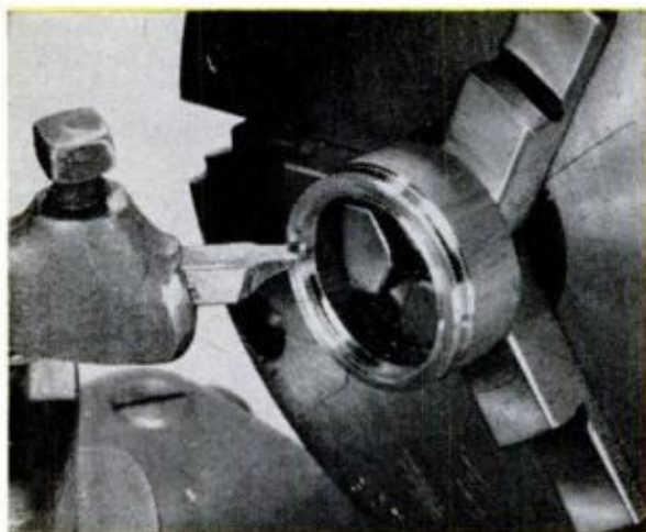
INNER LIP of stock is machined by feeding tool with compound-slide screw. Final cut (cut No. 4) has been started here, will be deepened later to part ring from stock as the last step
