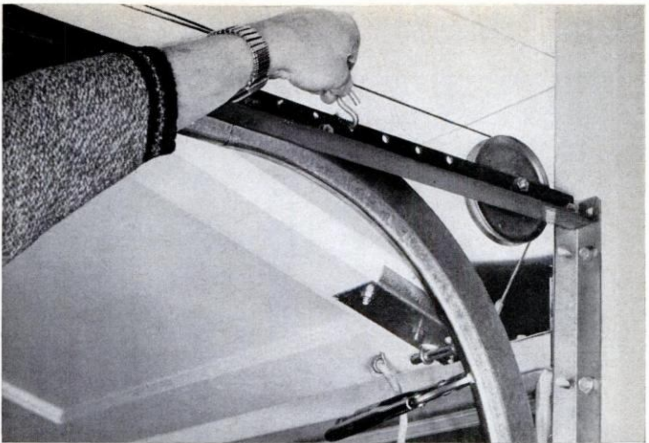
COMMON WAY to adjust spring tension is to change S-hook placement. Vise clamp keeps door from falling
