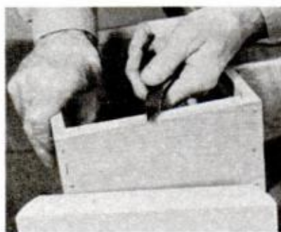
BRAD POINTS keep base pieces from shifting when gluing. Drive them part way, then cut off heads
