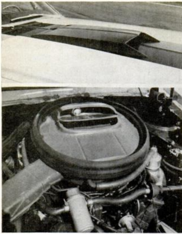
COLD-AIR SCOOPS are on some cars now. Cold air rammed into carb means more engine power output
