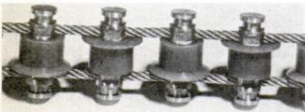
FLANGED PLASTIC ROLLERS clinched between flexible stranded cables form a single-pitch concept
