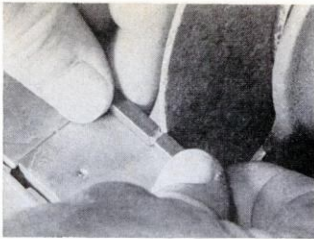
EASY WAY TO CUT BLANK TOOL BIT to the desired length is with a \frac{1}{8} -in.-thick abrasive cutoff wheel
