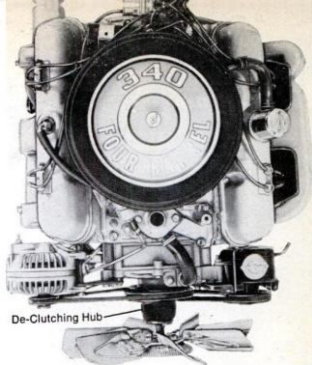
DECLUTCHING HUB disconnects fan from engine at high speeds, saving horsepower needed to drive it
