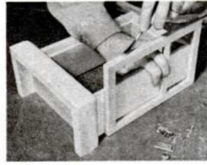
HINGE MORTISES are cut in frame only. Make approximately \frac{1}{16} -in. deep to assure proper clearance
