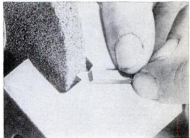
CAREFULLY FINISH GRINDING the fly-cutter bit by adjusting the grinder's toolrest to the required angle
