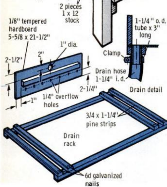
REMOVABLE DRAIN RACK supports processing trays, is lifted out for easy cleaning of sink. Drawing shows how sink bottom is rounded to drain off water
