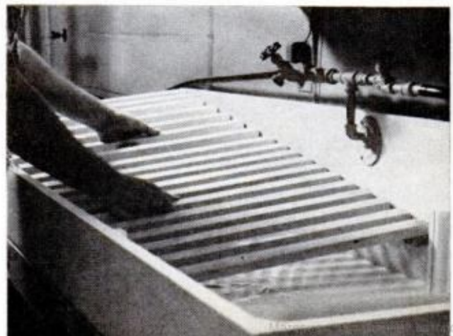
REMOVABLE DRAIN RACK supports processing trays, is lifted out for easy cleaning of sink. Drawing shows how sink bottom is rounded to drain off water
