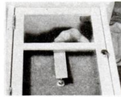
STRIP OF PAPER is used to check minimum clearance between minute-hand shaft and glass of door
