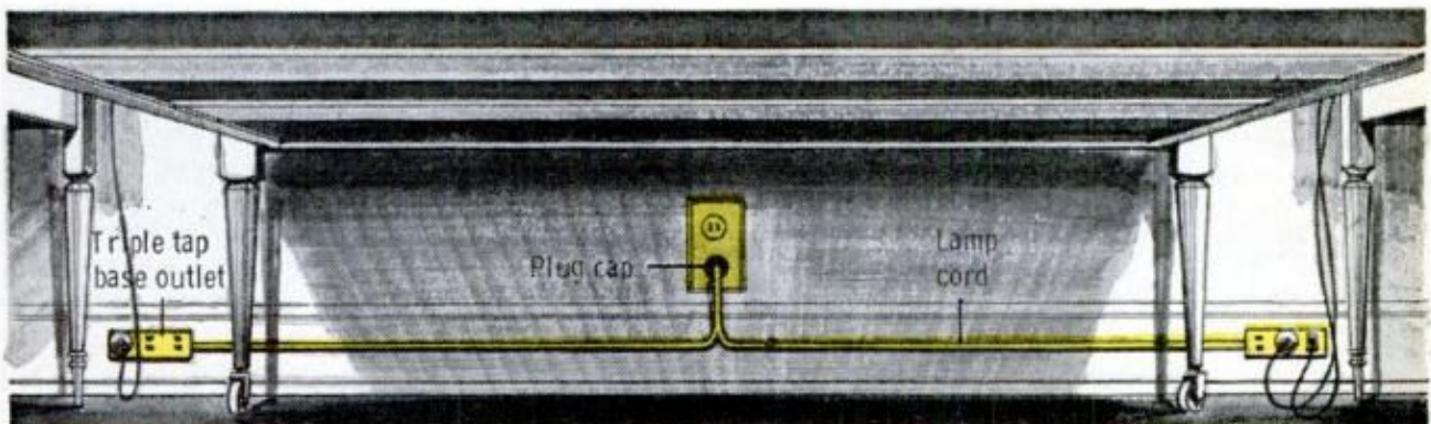
DOUBLE EXTENSION CORD provides outlets on both sides of a bed or sofa. Just cut the plugs from the ends of two triple-socket extension cords designed for baseboard mounting and connect them to single plug
