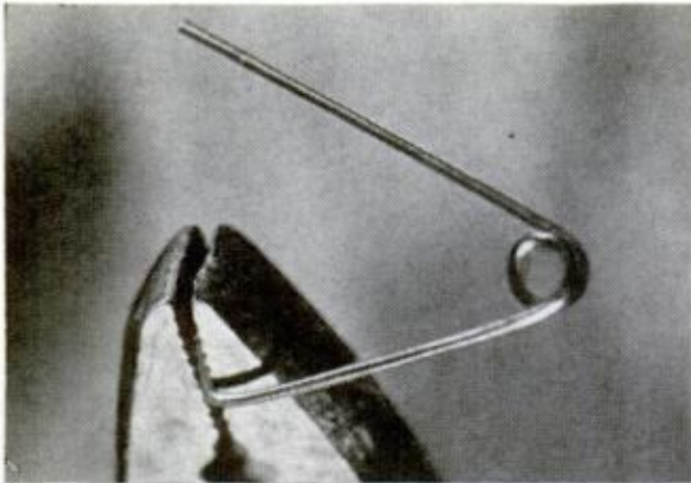
STEP 1. Trim ends off a safety pin; bend remaining tips
