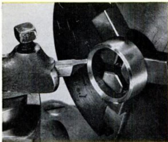
OUTER CORNER of stock can be removed in two ways. You can feed toward headstock, as here, using square end of bit to do forming, or swing compound 90^\circ and feed from opposite direction
