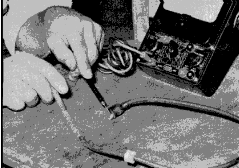
SPARKPLUG CABLE RESISTANCE , checked with ohmmeter, should meet specs, usually about 20,000 ohms
