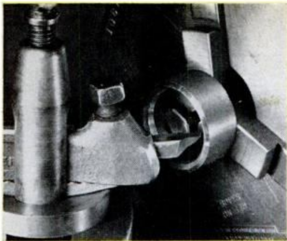
INSIDE CUT on diamond-shaped ring (cut No. 1) is made at far side of stock with lathe reversed. All other cuts are made at stock's near side with lathe running forward, as shown in diagram
