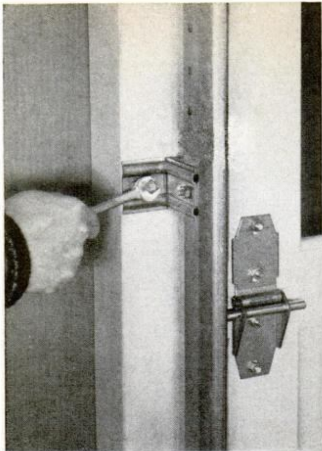
REDUCING FRICTION between the door and track (left) or door and stop (right) requires bolt adjustment
