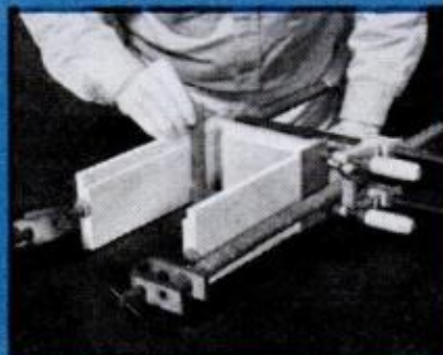
SIDES AND TOP are glued together after miter cuts have been made. Bottom piece is installed later.
