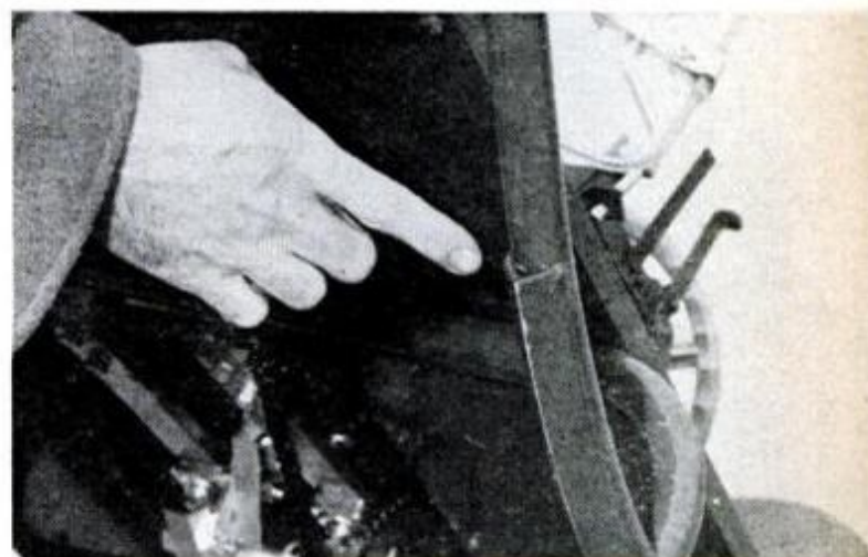
SLED RUNNERS are angle iron welded to the tubular steel frame. The sharp edge, acting like the edge of an ice skate, adds to the sled's stability
