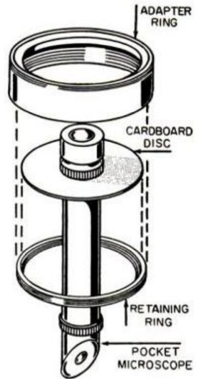
HERE IS HOW cardboard disc, sandwiched between adapter and retaining rings, is used to attach microscope to camera
