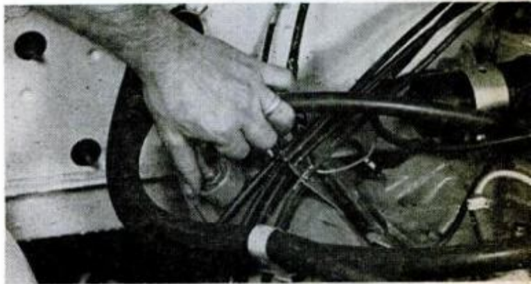
A CLEAN CRANKCASE VENT VALVE helps conserve gas. To clean or replace it, remove the cover and pull away vent line. Check manual before doing this job
