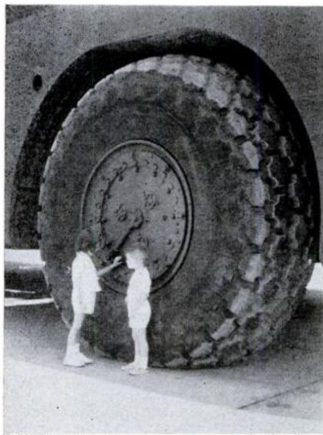
Nine-and-a-half-foot tire towers over small fry. It's one of four used on Army's new amphibious "Bard," a 100-ton vehicle that will haul 120,000 pounds of cargo or 100 soldiers over land or water. Each tire weighs nearly 1½ tons and includes enough rubber for 600 passenger car tires.
