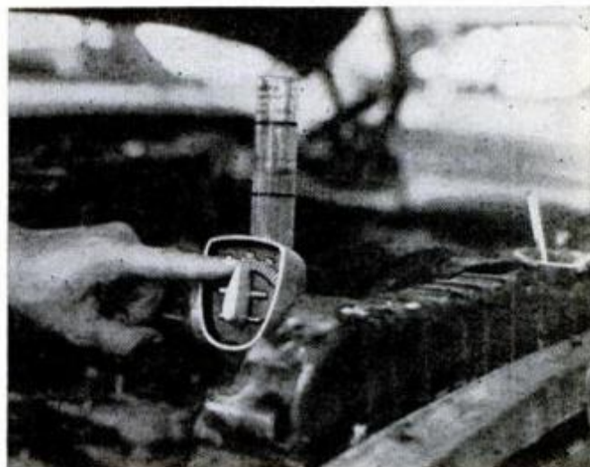
Cooling-system tester. When your engine is overheating you can quickly trace the trouble to a sticking thermostat, balky water pump or clogged water passage by connecting the flow pipe of the new Morgan Tester between the radiator and its inlet hose. Action and level of the water after it passes through a butterfly valve and tiny hole into a clear plastic standpipe tell the story with readings on a simple flow meter. The tester also reveals if the system needs flushing or has a combustion leak into the water jacket. It is sold, complete with adapters for 1¼ to 2-inch hoses, for $24.95 by the Morgan Manufacturing Co., 29 S. Brown Ave., Scottsdale, Ariz.
