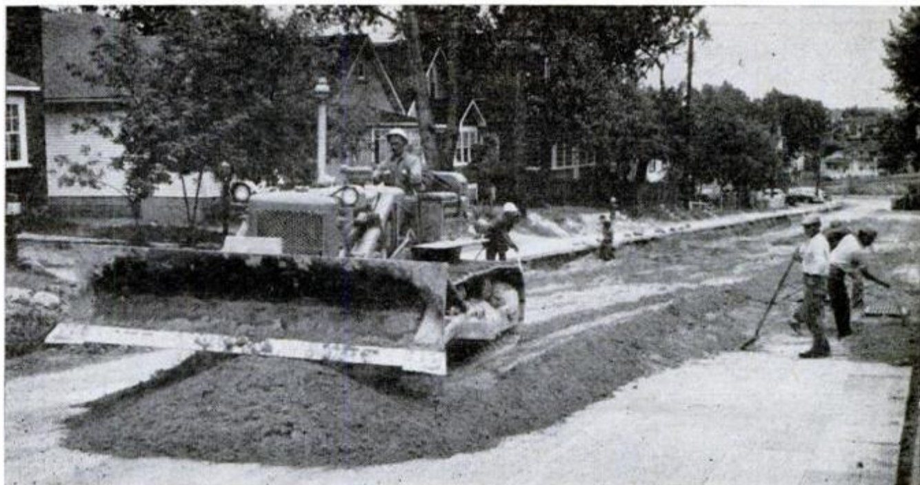
To beat Jack Frost. Canadian engineers are experimenting to determine if a layer of two-inch-thick polystyrene boards between the asphalt surface and the base course of a road will prevent heaving in extremely cold weather. Test site is a 100-foot section of road in Ontario. Thermocouples were buried in the roadbed to provide constant temperature readings.
