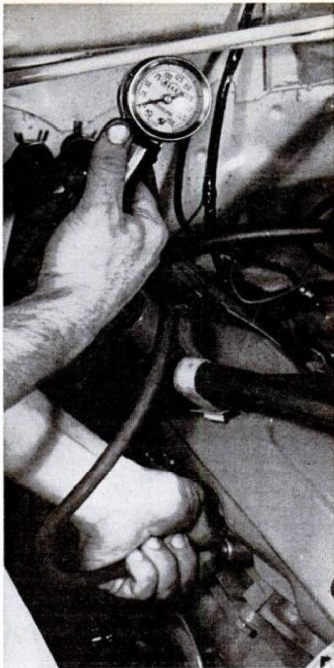
POWER ROBBERS inside the engine can be detected by conducting a compression test (shown above) and a vacuum-gauge test. Do both tests every 12,000 miles
