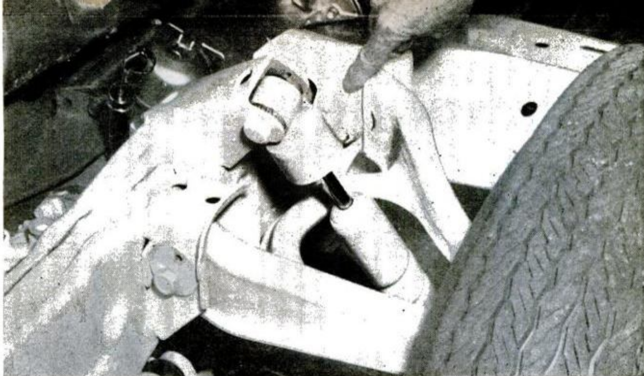
CAM-TYPE CASTER and camber adjustment points are indicated here. Steering gear is horizontally located
