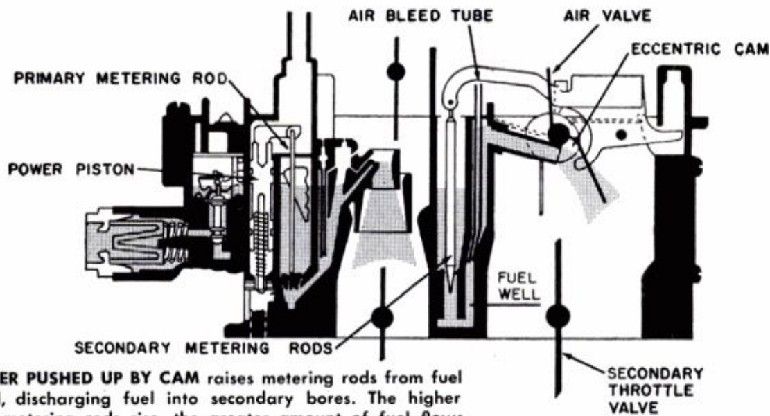
AIR VALVE in GM Quadra-Jet carburetor is attached to plastic cam. Air pressure opens valve against spring pressure (circled inset), which in turn rotates cam
