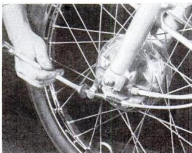
BRAKE ADJUSTMENTS are made by activating brake lever on handlebar and brake pedal while turning brake adjusting nuts on the front and rear wheels
