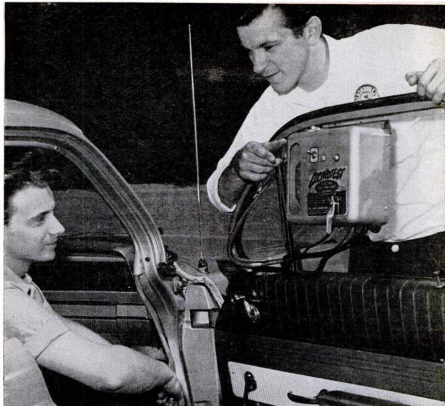
THE ONLY WAY to determine accurately how much gas a car is using is with a gas-per-mile gauge (shown fastened to door of car above). With gauge tapped into fuel system, a test run is made over a planned course
