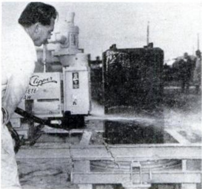
Concrete-cutting saw. Capable of slicing through reinforced concrete, the saw is used in Australia, where it was developed, to lop the tops from harbor piles. It has a diamond-edged blade that's horizontally mounted, driven by compressed air and water-cooled. The saw's frame, which is adjustable, is dropped over the top of the pile. The tool can cut piles up to 18 inches square.
