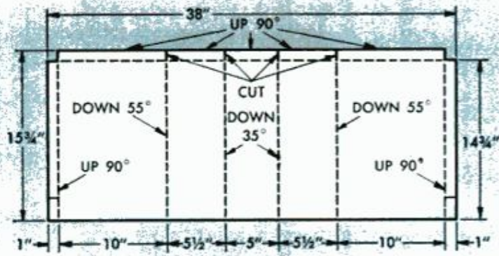
HOOD
