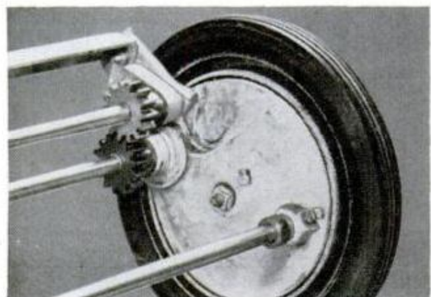
ORIGINAL MOWER wheel, wheel plate with spur gears, brush shaft, jackshaft and drive shaft in place
