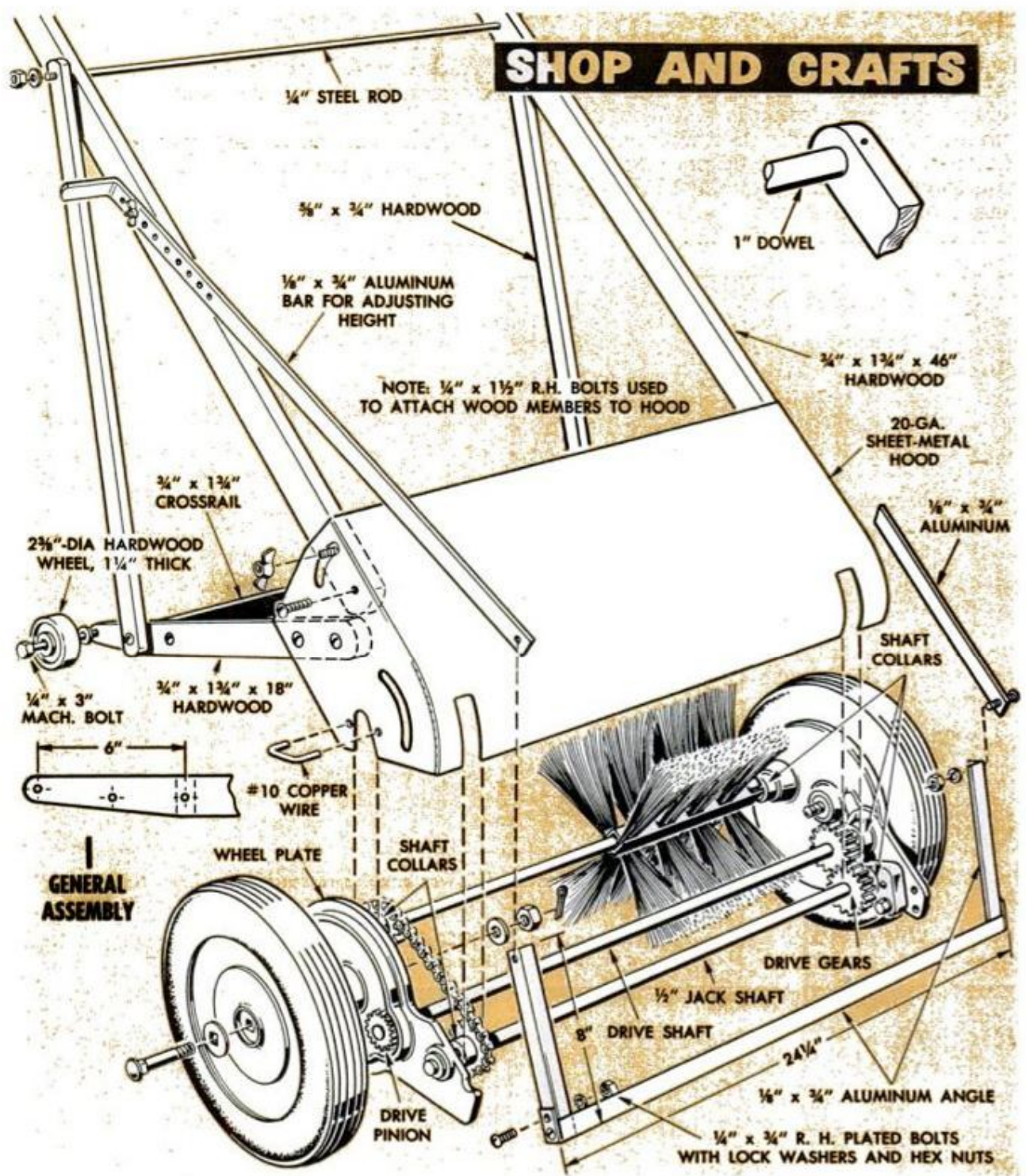
ORIGINAL MOWER wheel, wheel plate with spur gears, brush shaft, jackshaft and drive shaft in place
