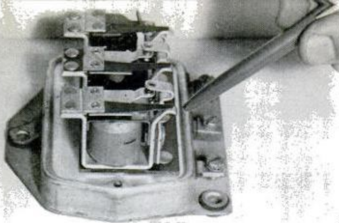
7. REGULATOR of riveted construction is adjusted by bending brackets (pointer). There are no screws
