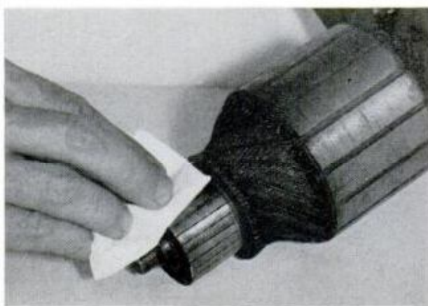
12. A COMMUTATOR in good condition can be cleaned with a soft cloth. Very fine sandpaper also is used
