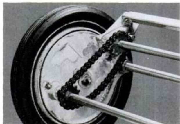
OPPOSITE MOWER WHEEL showing roller-chain drive to the brush shaft. This drive reverses brush rotation
