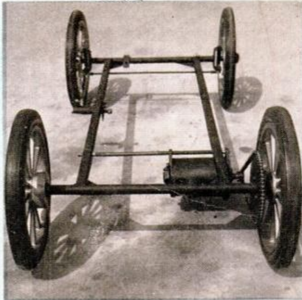
1. FRAME AND AXLES are constructed of steel tubing, both square and round. Motor is mounted in the rear
