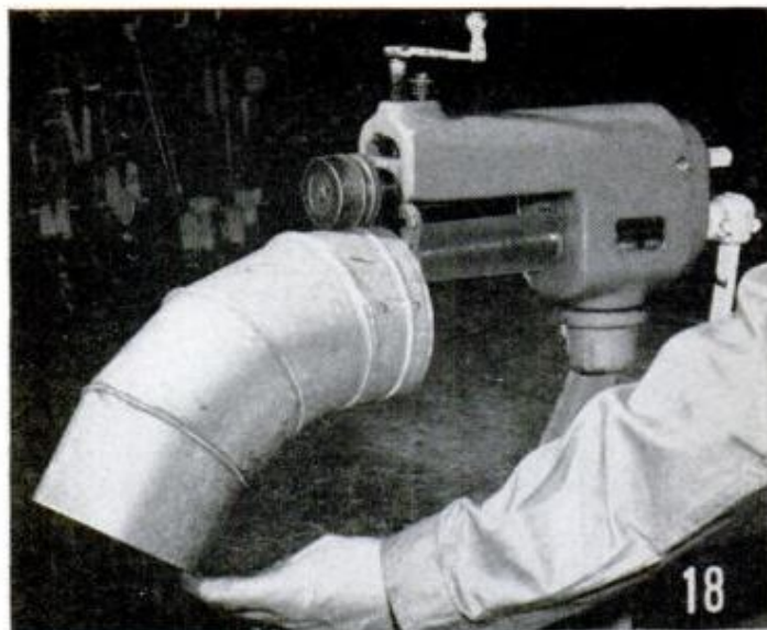
ROTARY MACHINE with deep throat. See also Fig. 20. Here a bead is being rolled on a smoke-pipe elbow
