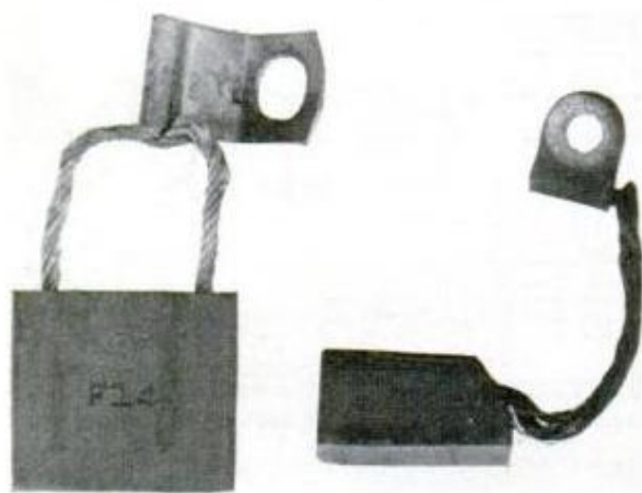
11. COMPARE OLD and new generator brushes, above. Below, be sure brushes are correctly seated
