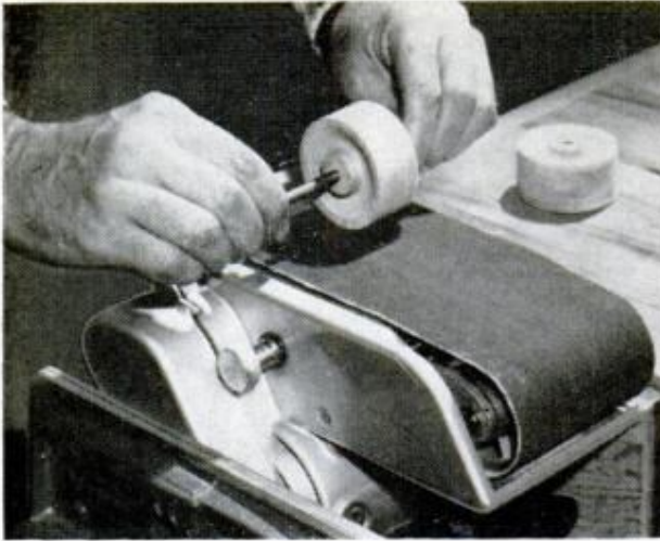
TRUE UP dolly, or trailer, wheel treads on belt sander. Hex-head machine bolts serve as wheel spindles
