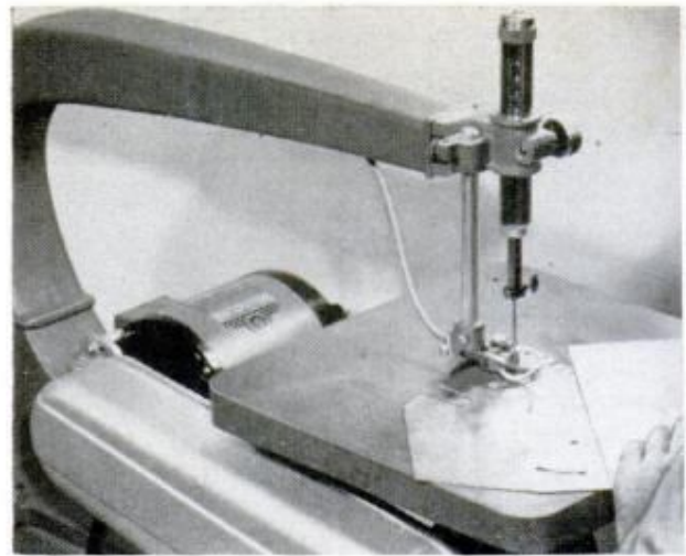
MUCH OF THE WORK of cutting out sheet-metal hood can be done on jigsaw with metal-cutting blade
