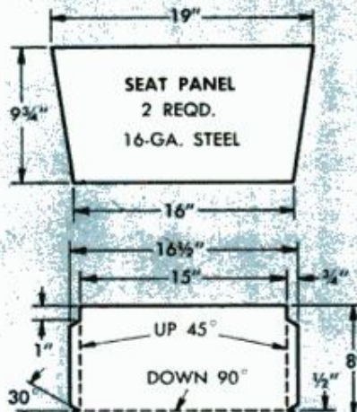
SEAT PANEL 2 REQD. 16-GA. STEEL
