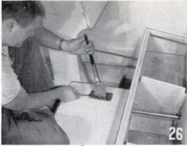
SHIFT LEVER mounts on a small, rigid floorboard panel outside and slightly aft of the control stand
