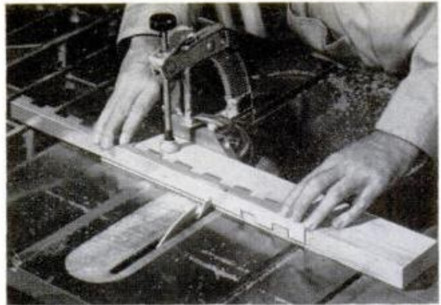
ALUMINUM ANGLES which hold brush sections in place are notched on table saw. Note backing strip
