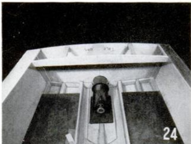
TRANSOM CUTOUT for the jet exhaust should be cut and tested for fit before installing the gas tank
