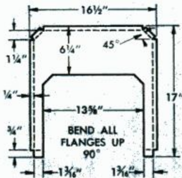
DASH PANEL
