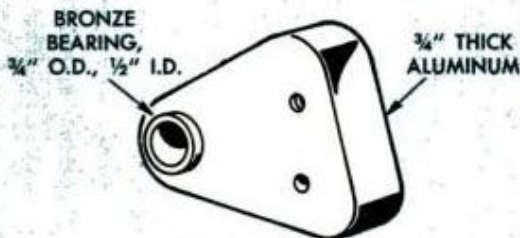
JACK-SHAFT BEARING BLOCK
