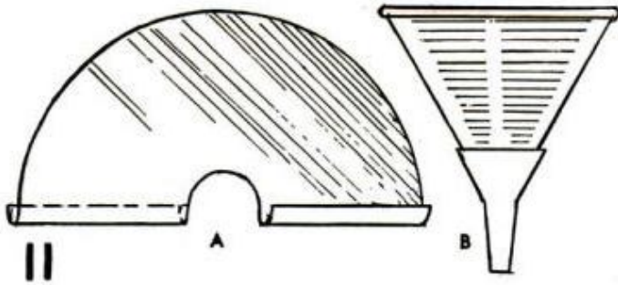
FUNNEL TOP , or bell, is laid out by the rollation method, Figs. 3 and 14 through 16. Note that in detail A the locks are formed for the joining seam which is being hammered down on a stake as in Fig. 12
