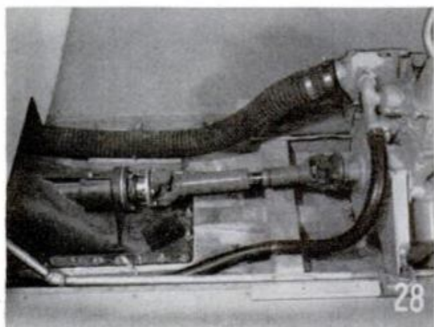
DRIVE SHAFT, motor exhaust tubing, water hose and jet unit all fit under the low-profile walkover cover
