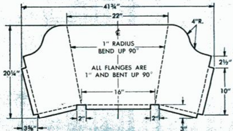
SEAT AND BACK
