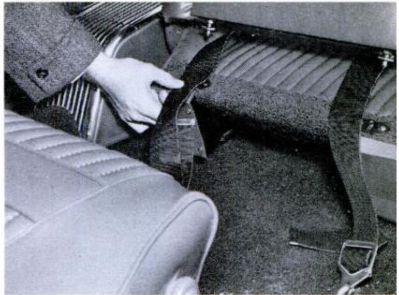
A GOOD IDEA gone wrong. Spikes on pivoting seat back stick in sockets to prevent tilting but could stab seat belts
