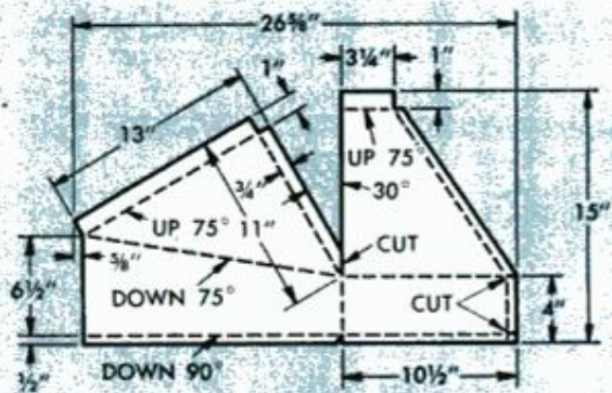
FENDER 4 REQD. RIGHT AND LEFT-HAND
