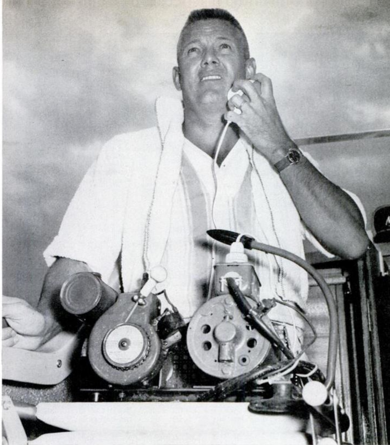
MORNING SHAVING aboard boat is no problem: Pull the two-cycle midget motor's starter cord, open the choke and it revs up to 6300 r.p.m., belt-driving a.c./d.c. alternator, supplying 110-volts a.c. for razor
