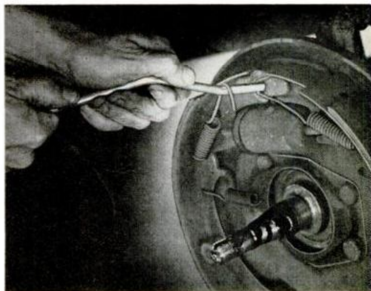
9. TRICKY JOB on Bendix brake is removing and replacing retracting springs. This tool does it easily
