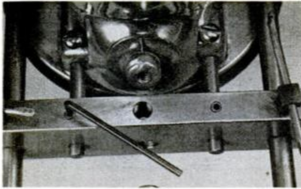
4. BASES OF SOME portable routers permit mounting by means of a coupling bar and short coupling pins
