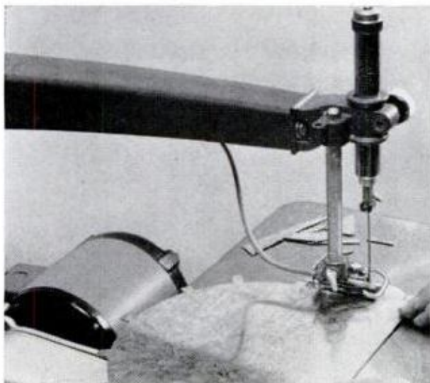
END COVERS of hood are neatly cut out with jigsaw fitted with metal-cutting blade. Note soldering tabs
