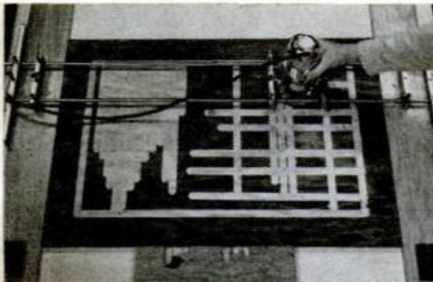
7. HERE router is supported clear of recessed surface by second coupling bar attached to handle boss
