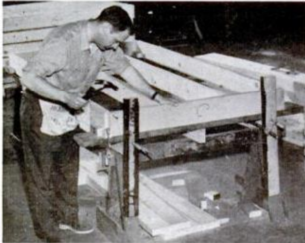
UPRIGHT STOPS ON JIG quickly position closure members for nailing to ends of longitudinal members
