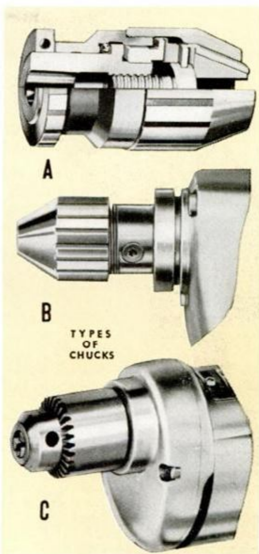
THREE TYPES of chucks supplied on portable drills. Geared chuck, C, is most widely used
