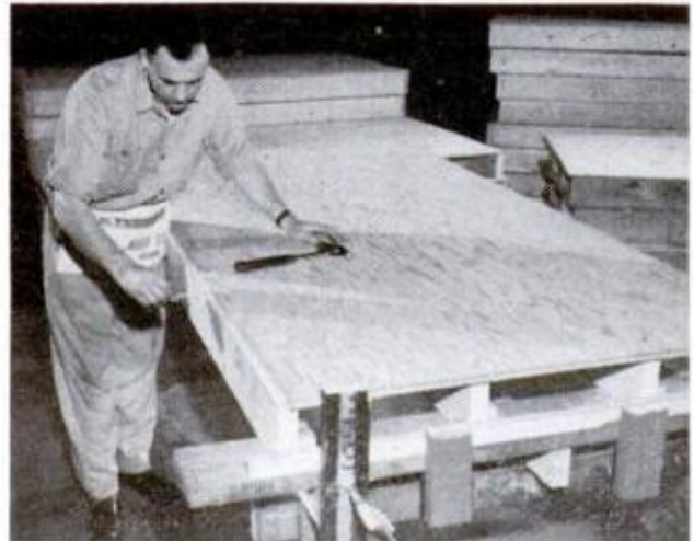
SHEETING ON SOME floor units center on edges of 2 x 6s to provide nailing ledges for adjacent units
