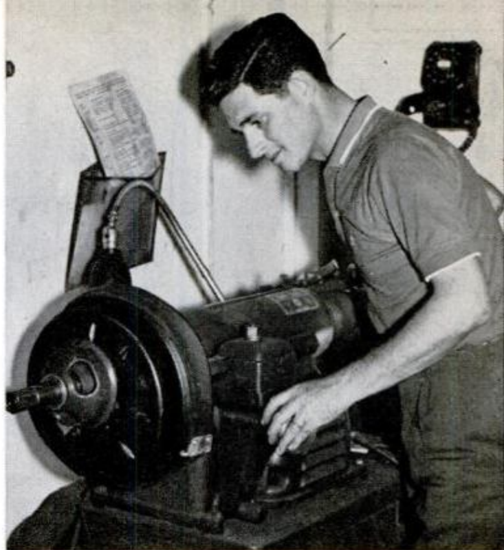
2. TRUING BRAKE DRUMS on a brake-drum lathe is advisable if you suspect that drums are out of round
