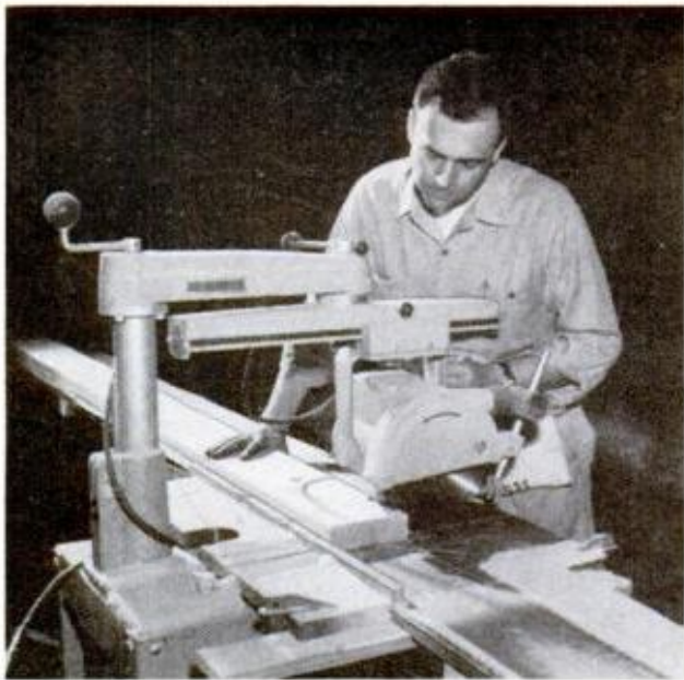
RADIAL-ARM SAW makes play of cutting duplicate floor members squarely and to exact same length
