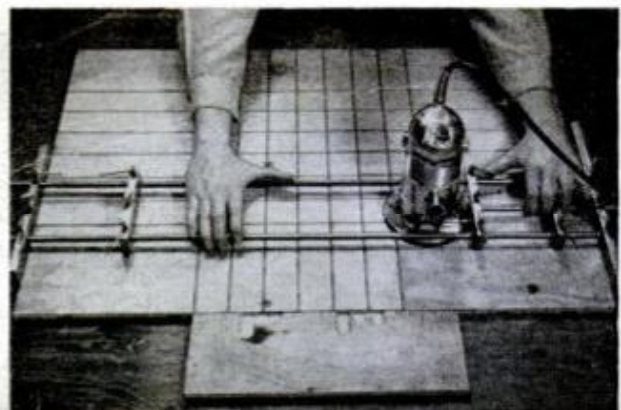
9. SPACED DADOES , run in two directions, complete a pattern on face of stock. Note that stopblock is used
