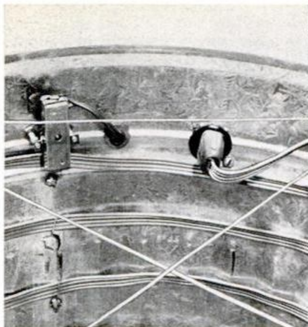
11. HEATING TAPE , above, is plugged into wafer-type outlet. Right, solder spots being sweated onto can
