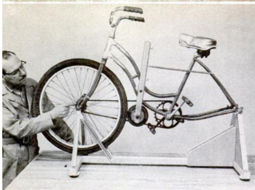
ASSEMBLED bike exerciser (left) ready for painting. Note rubber caster-cup feet and hooks for varying tension on friction wheel
