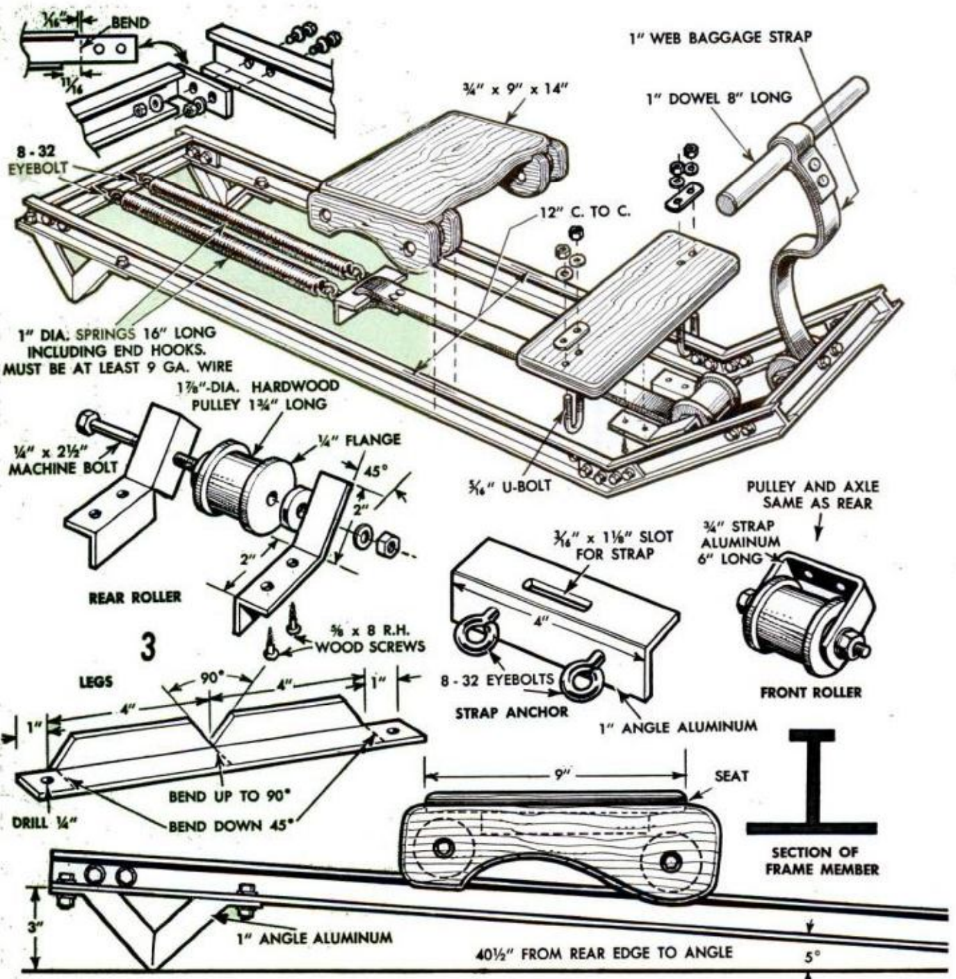
VIEW OF FRAME at rear of rowing machine shows how twin coil springs are attached to the pull strap
