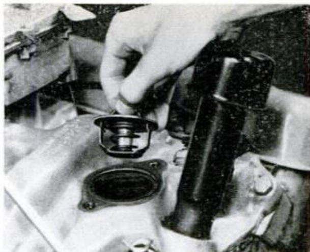
1. THERMOSTAT should be changed each time antifreeze is drained in spring or added in fall. Be sure to use 'stat rated for your climate and kind of driving
