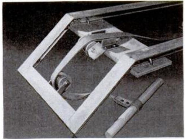
UNDERSIDE VIEW of rowing machine at front shows web baggage strap doubled to minimize stretching
