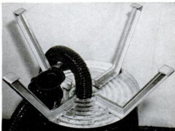
2. LEGS can be made by notching and bending aluminum T-shapes. Note how suction hose slips over outlet
