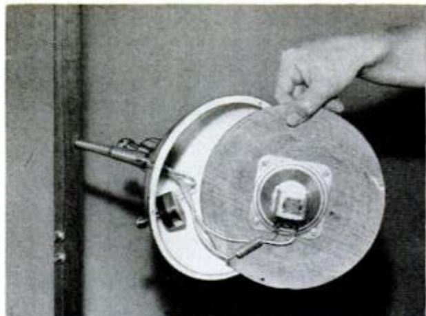
INSIDE OF BULLET shows speaker mounted to baffle with volume control and crossover capacitor wiring
