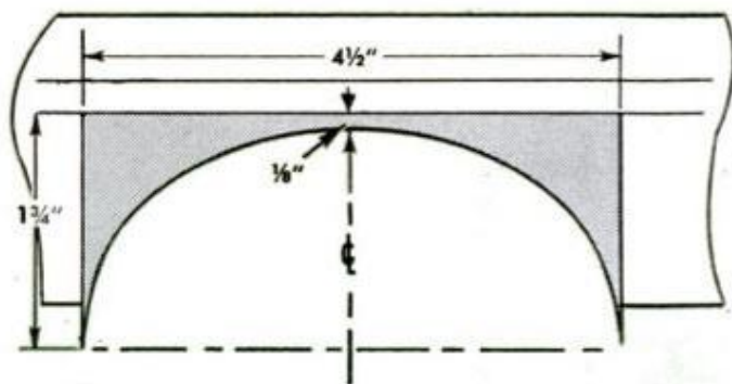
13 FILLER BLOCK FOR SIDE POCKET CUT FROM 3/4" PLYWOOD SCRAP
