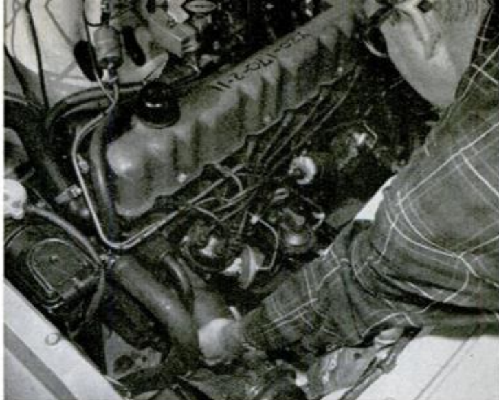
FAIRLANE AND METEOR SIXES are very accessible. Oil filter can be reached from topside, spark plugs are at hand. There's plenty of wrench and wrist room around distributor and fuel pump
