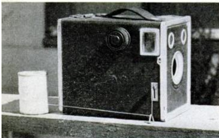
BOX CAMERA (below) can be used in bird photography. String arrangement trips shutter from remote position when bird alights at predetermined spot
