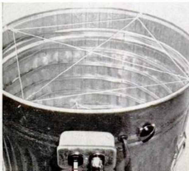
9. FILM RACKS are made by stringing picture wire arranged in a square with diagonals as pictured here
