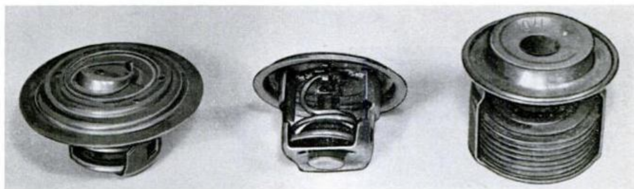
5. THERMOSTATS you'll find in most of today's cars. Two at left are pellet type; one at the right is a bellows type. Always test a stat before installing in your car, even a new one, as it may have been damaged
