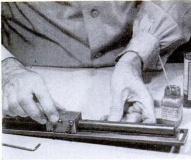
4. SLIDE BLOCKS should be lapped after reaming to assure smooth operation. Drill-rod track is coated with lapping compound. Block is stroked by hand
