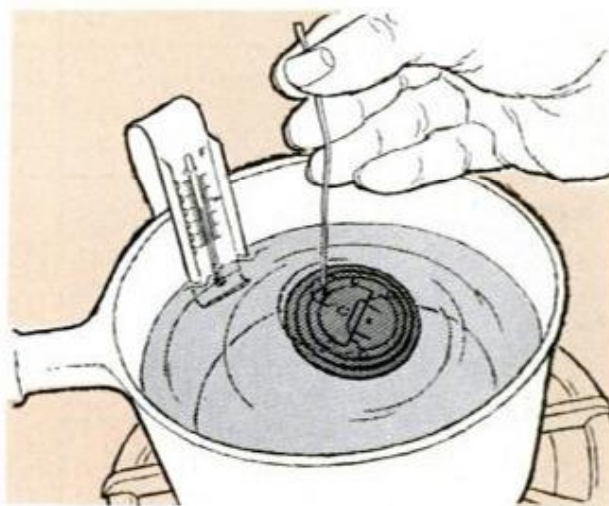
2. SATURDAY MECHANICS can check a stat in a few minutes with this setup. Use a reliable thermometer and clean water. Hook thermometer over side of pan with bulb submerged. Stat should open at rated reading
