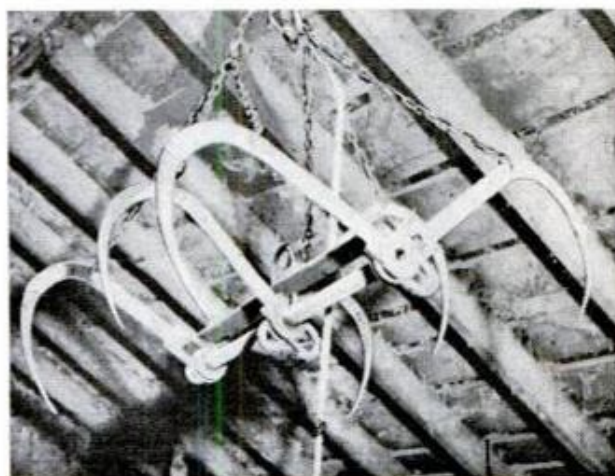
A grapple fork on carrier is sometimes used to get baled hay into mow. Fork tines are altered to grip bales
