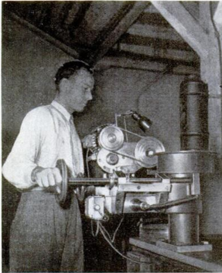
Six hundred atmospheres of pressure leakproof the slots in piston rings in the machine above, built for the plant. Below, the new "Rodel" portable shipboard grinding and milling tool
