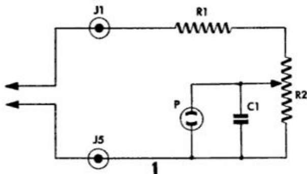
1 VOLTAGE TESTER—AC OR DC (FOR 100 VOLTS OR GREATER)
