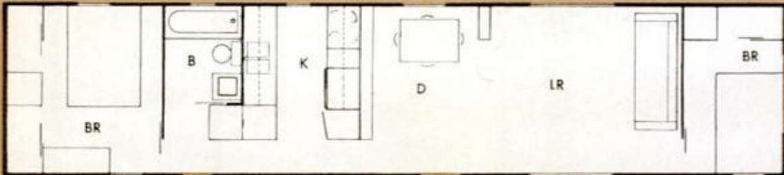
50 x 10 CAPRI—SPLIT THREE BEDROOMS
