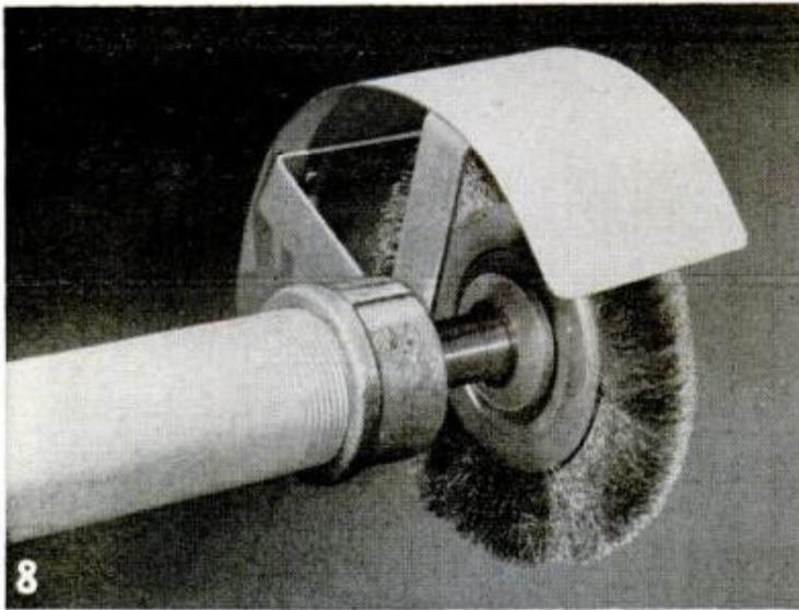
8 Above, if you don't have a face shield, then the wheel always should be guarded. Make a guard by riveting sheet metal to L-shaped brackets and attaching to pipe cap with small screws turned into holes drilled and tapped in the cap. Below, bearings are carried on flanged collars setscrewed to spindle
