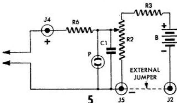
5 VARIABLE POWER SUPPLY
