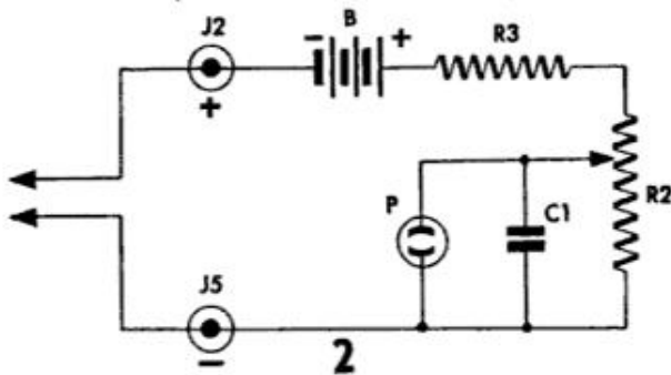
2 LOW DC VOLTAGE TESTER (LESS THAN 100 VOLTS) CONTINUITY TESTER CAPACITOR CHECKER
