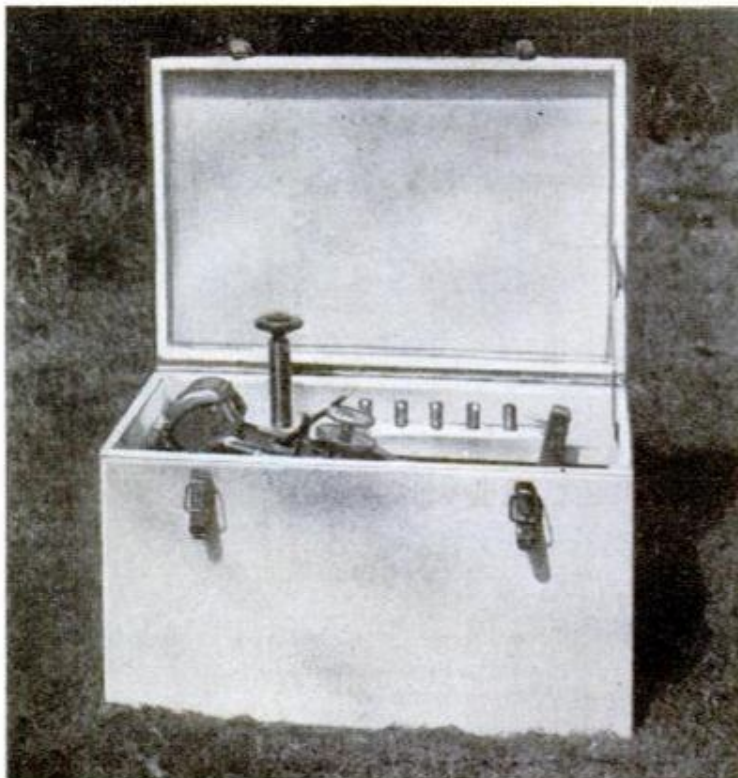
Six hundred atmospheres of pressure leakproof the slots in piston rings in the machine above, built for the plant. Below, the new "Rodel" portable shipboard grinding and milling tool
