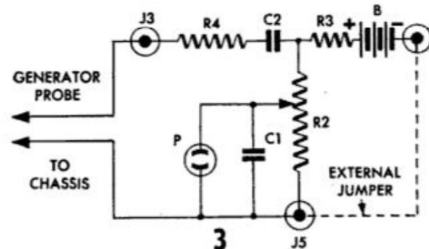
3 AUDIO GENERATOR
