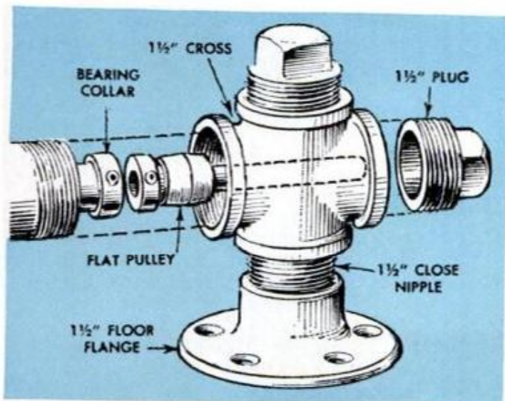
6 SPINDLE ASSEMBLY AT PULLEY END
