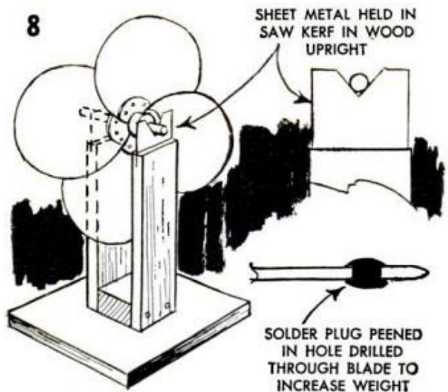
METHOD OF TESTING FAN FOR BALANCE
