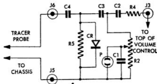
4 RF-IF TRACER
