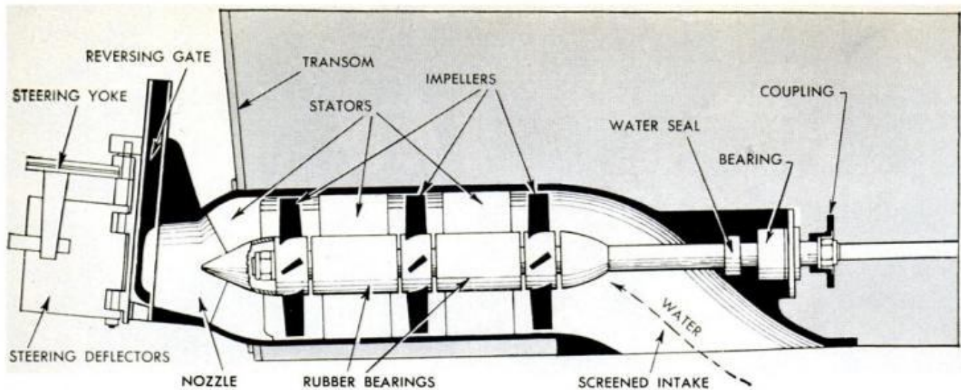
Above, the basic works of a Hamilton water-jet unit. Water comes in at right through a half-inch grid, passes through turbine and shoots out between the steering deflectors at left. Reversing gate here is in neutral position; drawings below show forward and reverse positions. Bottom photo shows exterior view
