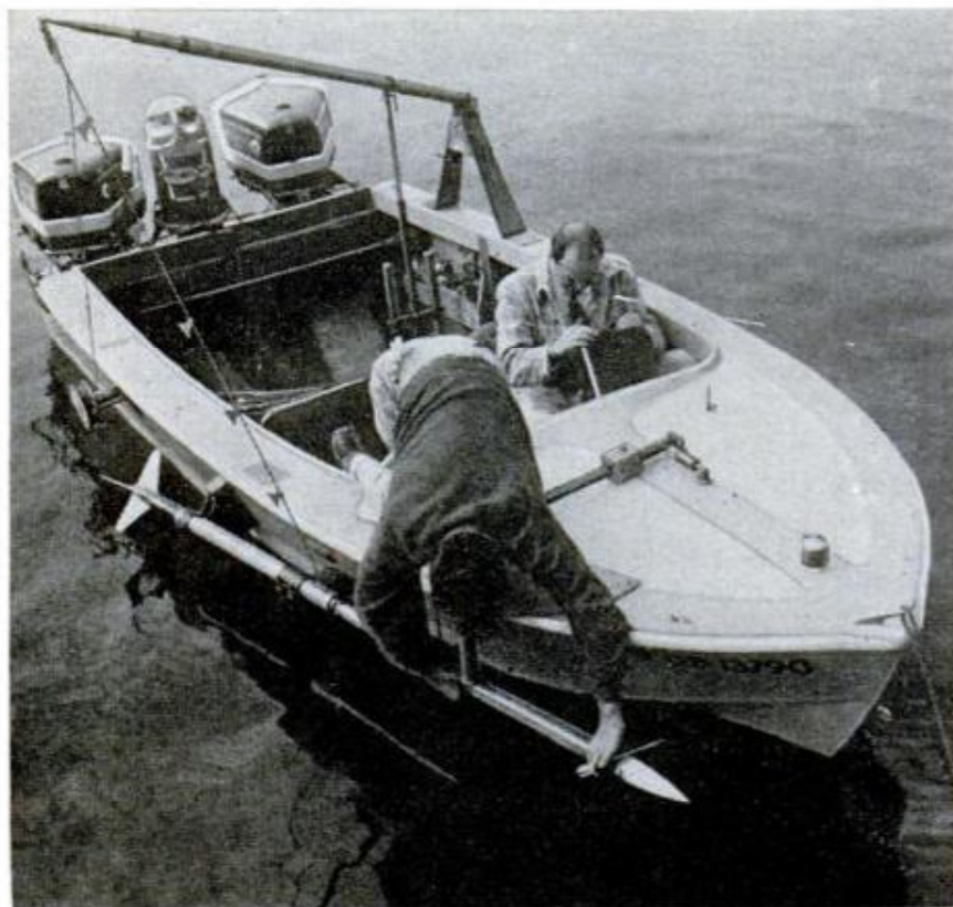
Testing the membrane. A model underwater vehicle is towed by the test boat while sensitive instruments record the comparative frictional drag
