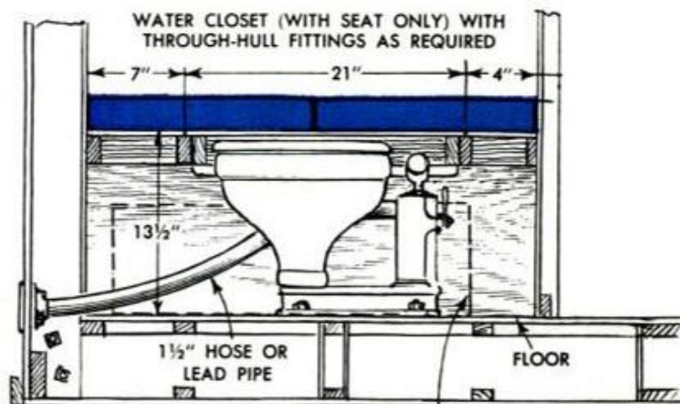
DOTTED LINE REPRESENTS CHLORINATOR (OPTIONAL) FOR USE ON RESTRICTED WATERS
