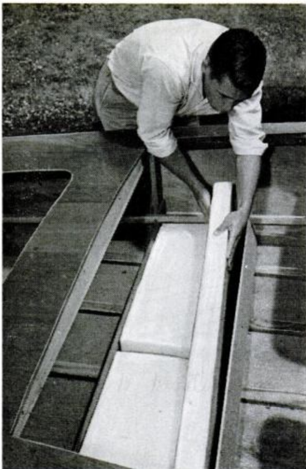
4. To ease job of filling space under seat with foamed plastic, three pieces are used instead of one
