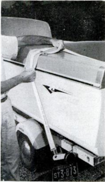
2. For long trips padding is placed under tie-down strap at sheer to prevent strap from marring finish
