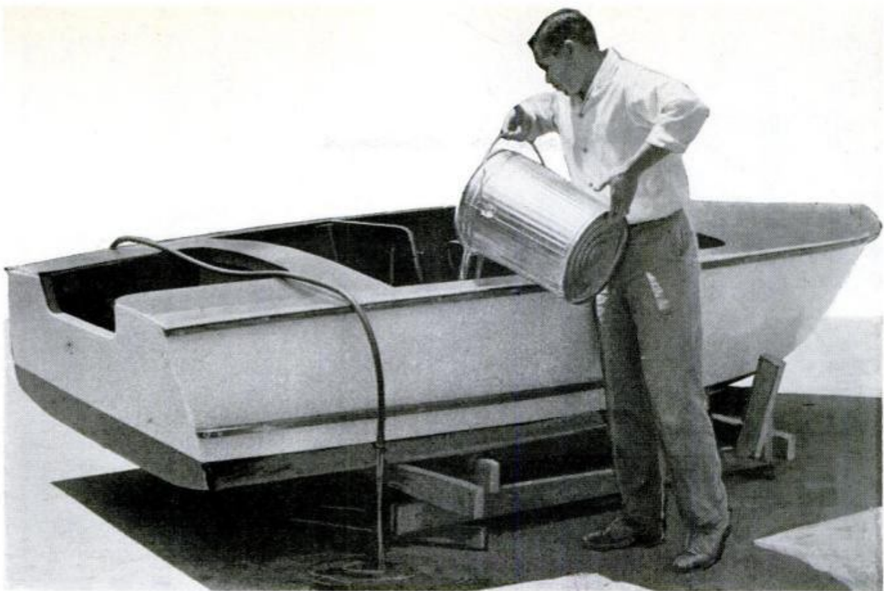
6. Boat is filled to transom cutout with measured water, as means of determining load capacity of hull
