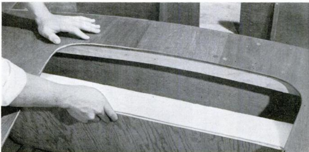
7. Foamed-plastic piece located next to motor-well bulkhead is boxed in with protective panel of plywood
