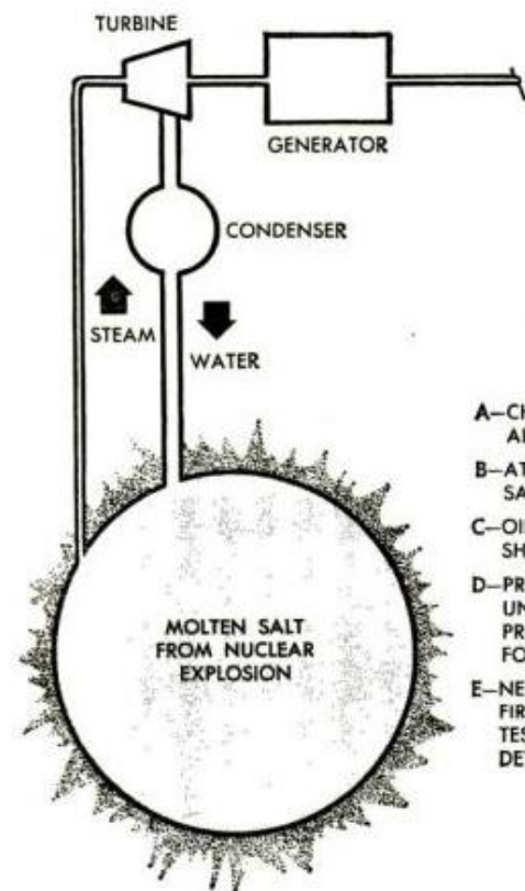
Five experiments of the Atomic Energy Commission's Plowshare program are located on the map. Project Gnome will test the possibility of "mining" heat from an underground nuclear blast to generate electricity. Simplified drawing shows how water would be pumped into the deposit of heat and then extracted as steam to run a turbine
