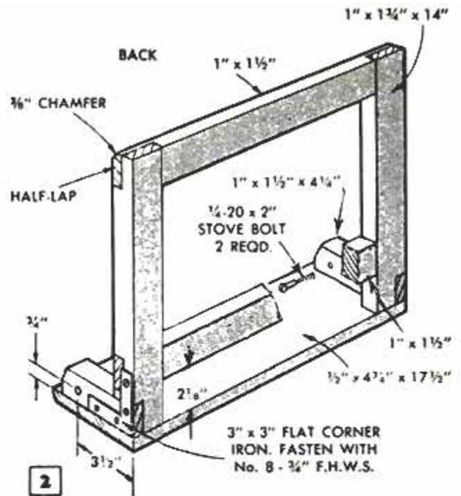
Half-lapped frame members for the folding back are rabbeted crosswise and then ripped to right width
