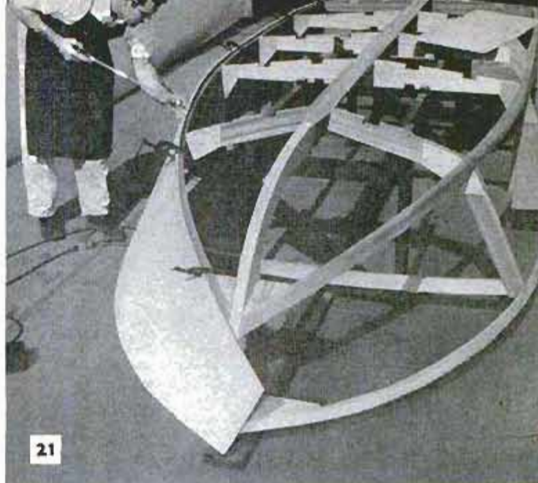
Above, side planking is clamped and screwed into position after it is recut to allow excess of ½ in. on all sides and glue applied to all facing members
