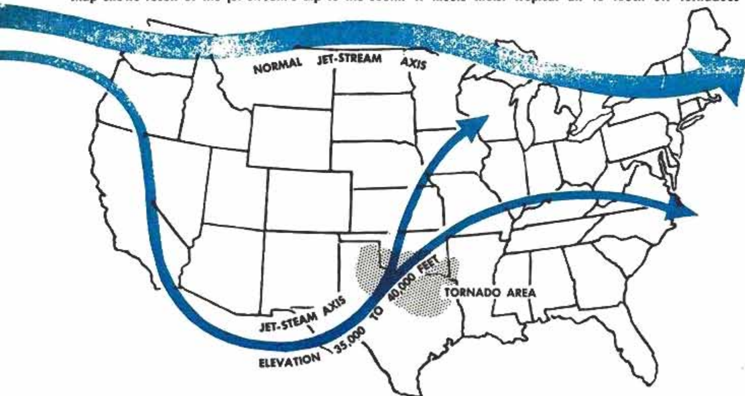
Map shows result of the jet stream's dip to the south. It meets moist tropical air to touch off tornadoes
