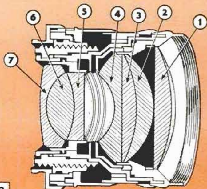
MULTIPLE-ELEMENT LENS
