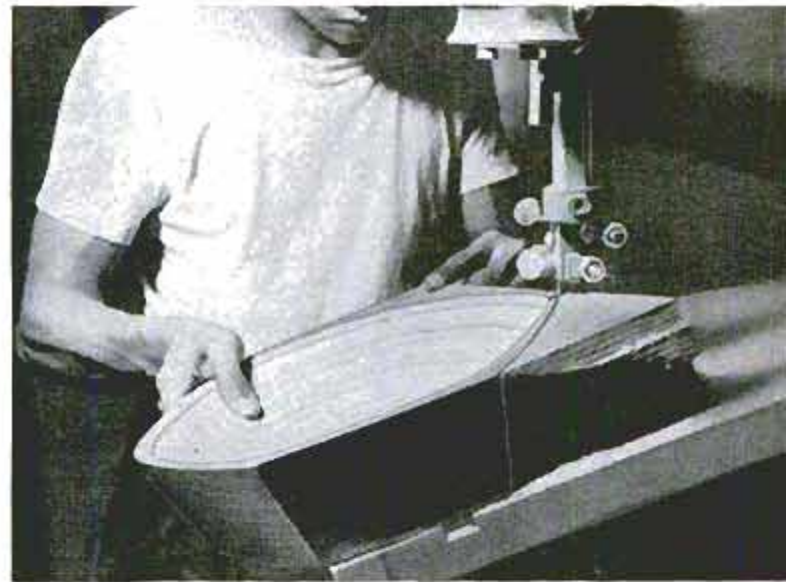
Bowl begins to take shape as he saws unwanted exterior. Goo also plans to use this process in sculpturing
