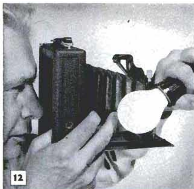
12 Electric light is held close to camera to locate light leaks that are most likely to develop at sharp bends and points of attachment of bellows
