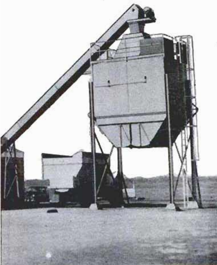
Two sets of dials on panel below control the exact weight of each type of feed to be blended in mixer
