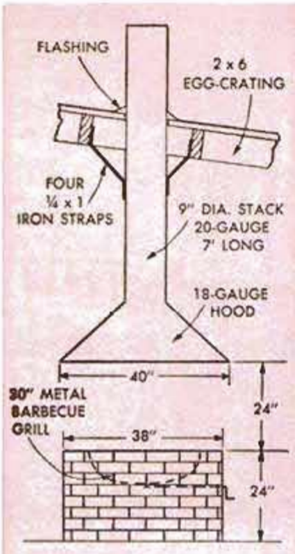
Detail at left shows how barbecue stack was suspended from roof and fireplace built; right, grill is guide
