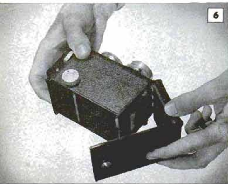
Fig. 6, chipped edges on sides of plastic reflex-camera body, or warped or bent back may result in improper closing of camera to cause light leaks
