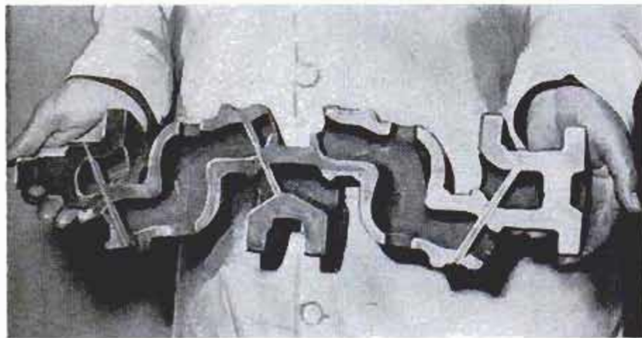
Hollow crankshaft is lighter in weight and is said to be better balanced than a solid one. Below, steel tubes in the casting carry lubrication
