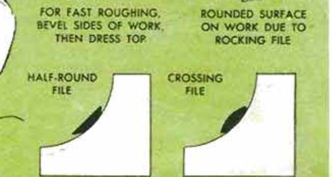
23 FILING CONCAVE SURFACES
