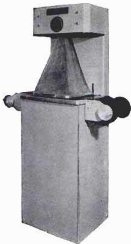
Photoprinter, built into a metal cabinet, has a feedback system which varies light according to the negative
