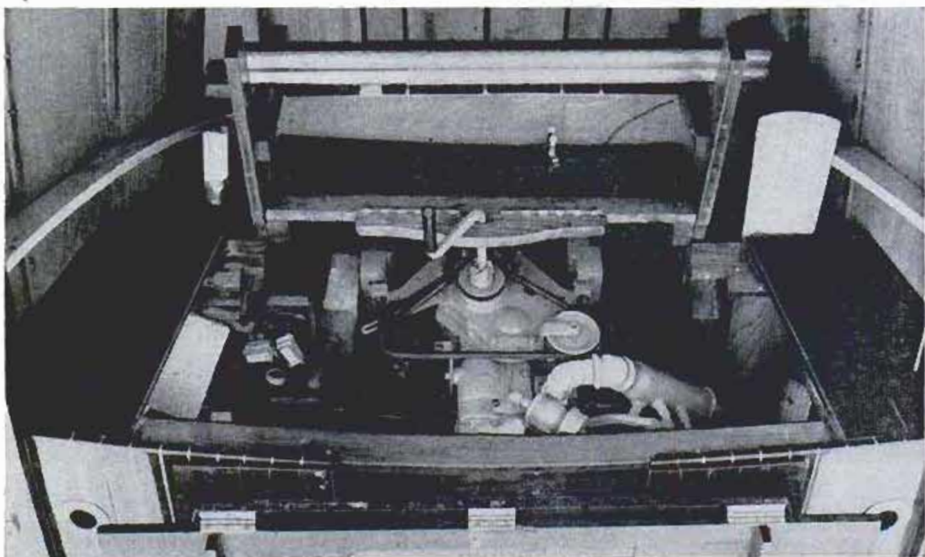
Reynolds has added special parts to the 18-horsepower motor including thermostat, oil filter, vacuum oil changer and vernier throttle. The motor hatch is lined with soundproofing material. Also on hand is a jointed sweep for sculling the boat if the motor should fail
