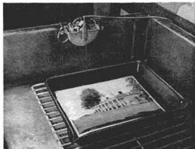
Agitator is made from windshield-wiper motor and vacuum-operated by running water through aspirator
