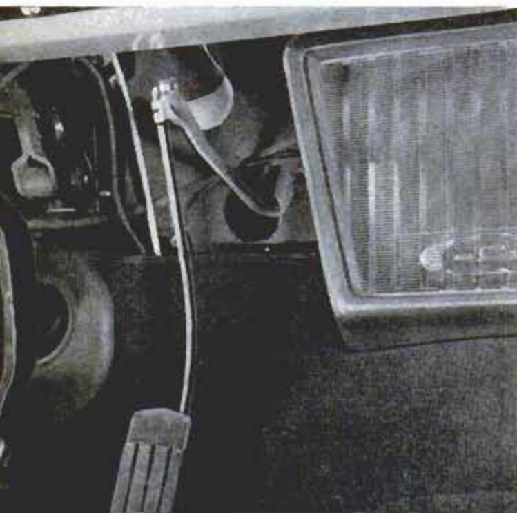
Carburetor air is drawn through grille via duct in foreground. Despite crowded compartment, long dipstick is easy to use. Below, accelerator linkage is "suspended" to eliminate need for hole in floor mat
