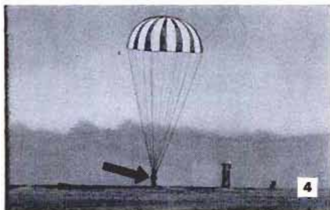
4. Pilot coming down safely under parachute. Below, sled is built for 16 rockets, but so far no more than eight have been used. Two of 10 rockets shown are used to sustain top speed. Water brake stops sled
