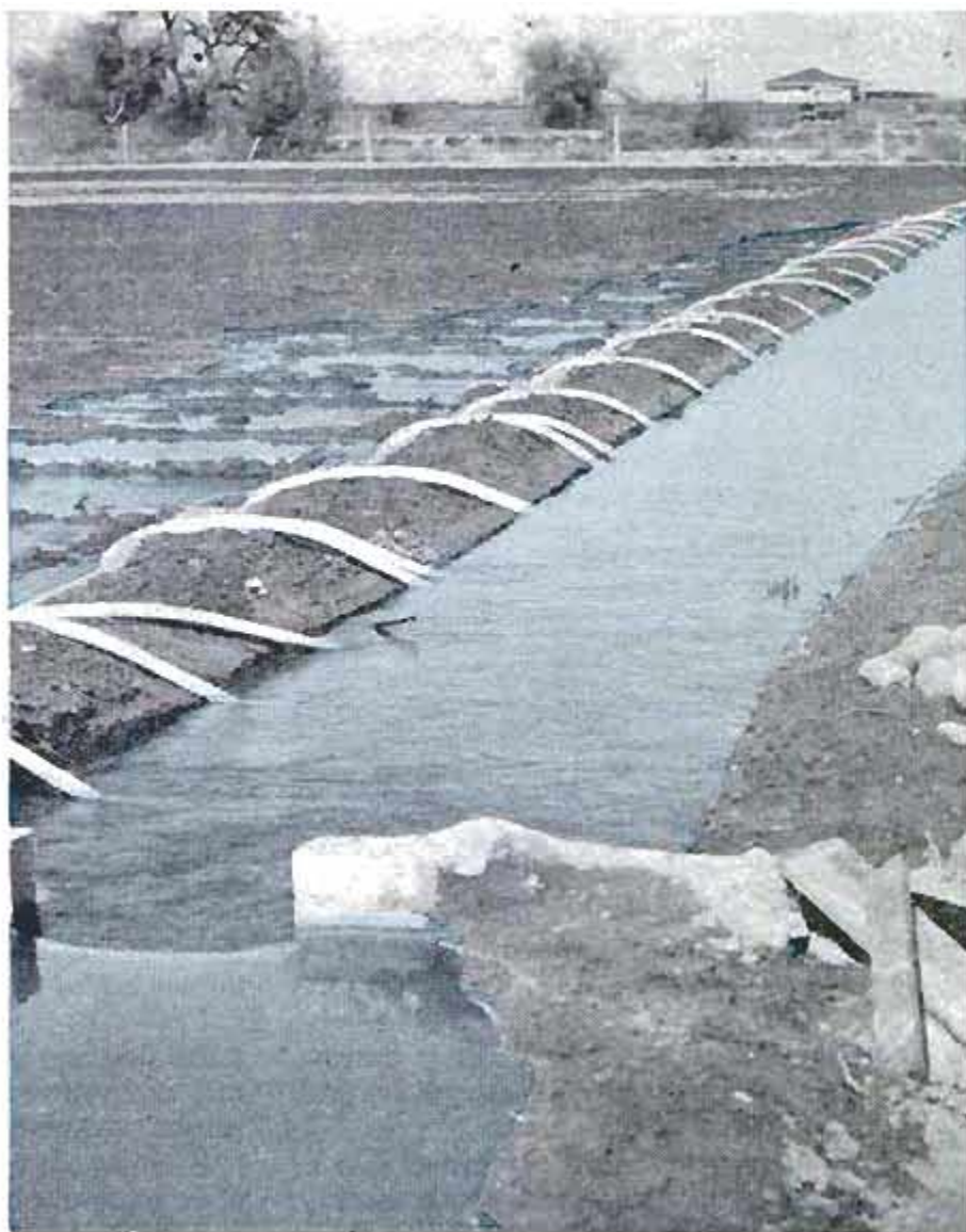
Field containing border crop is flooded by siphoning water from irrigation ditch over the bank by means of regularly spaced six-inch aluminum pipes
