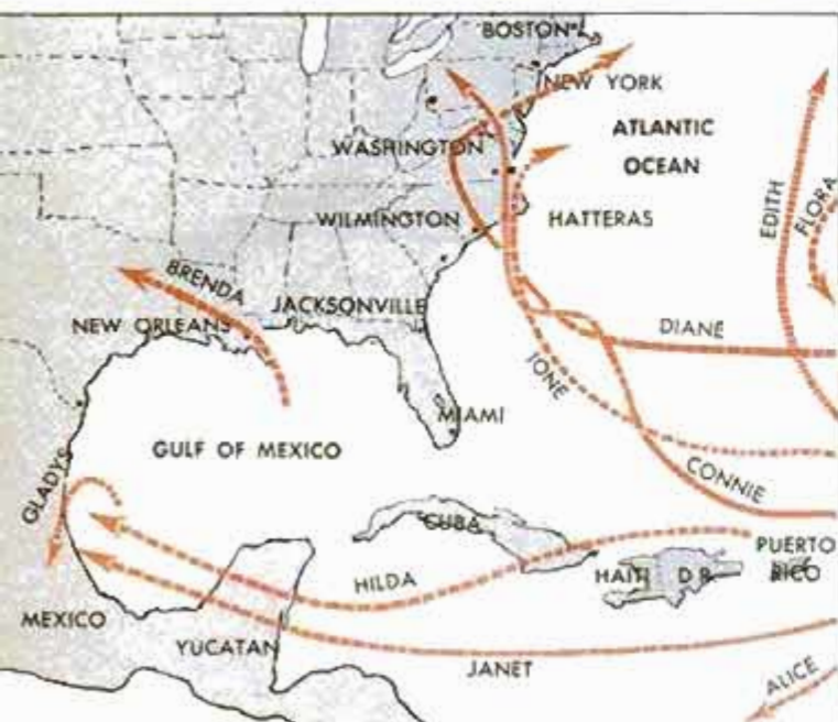
U.S. Weather Bureau chart above shows some of the 1955 hurricanes. Below, position of high-pressure troughs in 1955 helped swing the hurricanes inland
