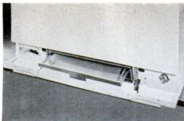
Above, lint screen of warm-air drier should be cleaned after each use. Left, lint is removed from condenser of air-condenser drier by flushing with water
