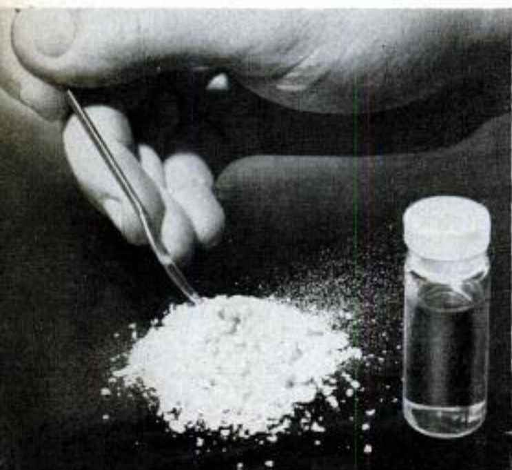
Slight irradiation causes a rubber band to crack and lose its elasticity (above), while two hours' exposure to gamma rays changes acrylonitrile from a liquid to a dry popcornlike polymer (below)
