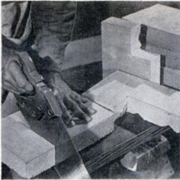
Lightweight slabs or blocks of perlite concrete can be sawed, nailed, drilled or channeled with ease
