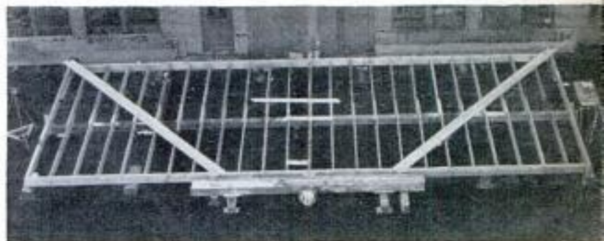
In structures of average size, two diagonal braces have been found to be ample floor bracing for conventional floor framing. Larger buildings and those with long floors require more
