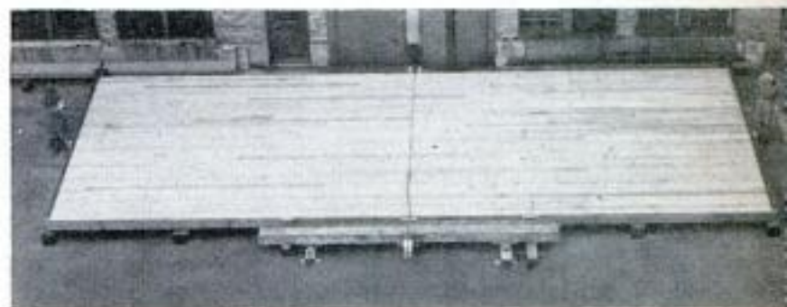
Above, a partially completed model floor frame with spaced diagonal braces laid one way under lengthwise flooring. This construction proved by far the stiffest on exceptionally long floor frames. Below, the finish flooring is laid the long way
