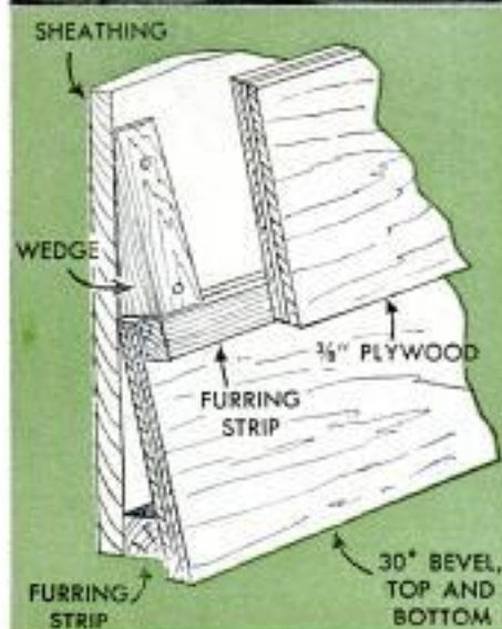
Exterior-grade fir plywood can be sealed with clear primer-sealer. A more common procedure is to use a regular grade of exterior primer thinned with 1 pt. of raw linseed oil per gallon of house paint
