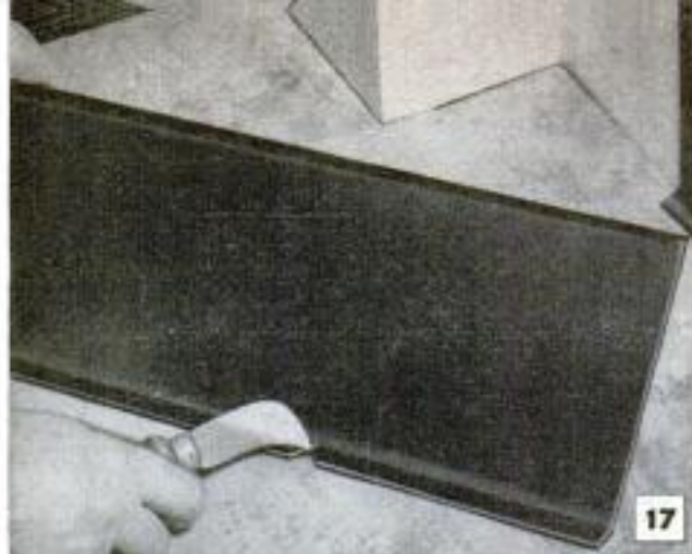
Above, asphalt tile used for top-set cove is notched, heated and bent to form inside corner as shown below
