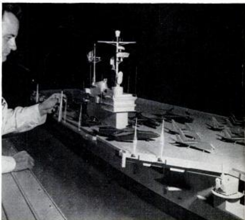
Side view of model shows 60-foot overhang of the flight deck. Planes land on the port side of angled deck and island side is for parking
