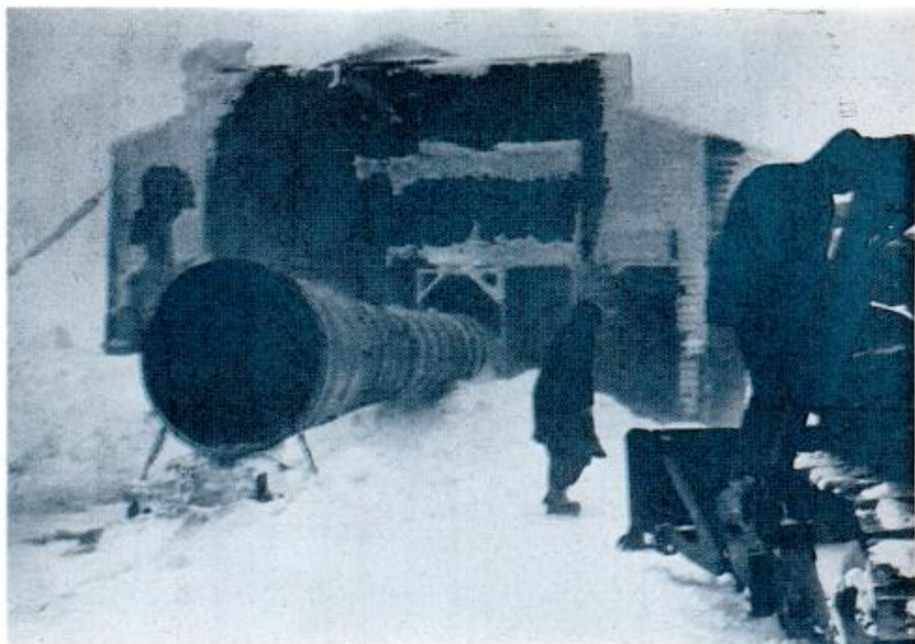
Exit end of wind tunnel juts from icing-research hangar at summit. Savage weather is ideal for test purposes
