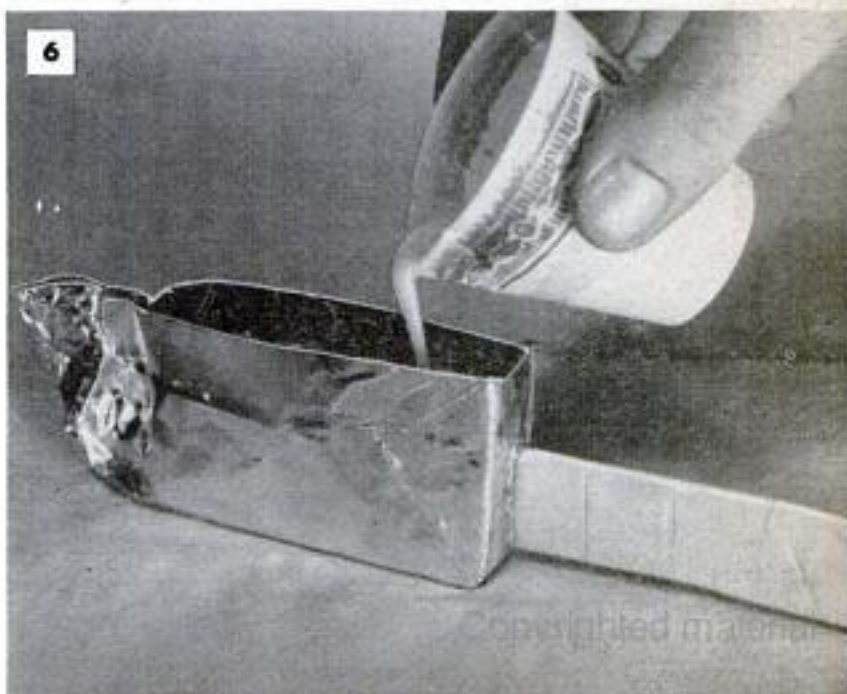
A second aluminum-foil trough is made, this time to enclose the entire knife handle. Holes and joints of trough must be sealed carefully and plastic poured in slowly, as shown below
