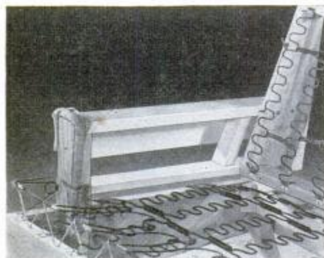
Above, edge roll is tacked around the front of each arm to soften hard edge and prevent excessive cover wear. Notice torsion spring and how edge wire is tied
