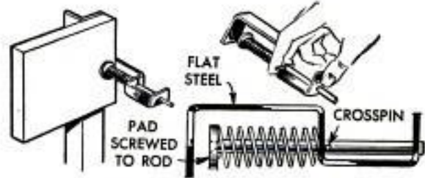
A handy tension clamp for holding light work is made by bending flat steel to a squared-S shape, drilling it to receive a length of rod fitted with pad. A crosspin in the rod provides a fingerhold for opening clamp
