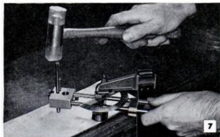
Above, a protractor is fitted into a slot cut in the head of the pivot bolt as in detail on opposite page. Protractor is held in place with setscrew. Below, circle tool can be attached to work or bench top. Works on full circle or any size segment
