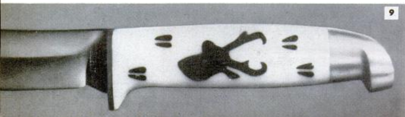
Roughly shaped handle is given a secondary sanding with 180-grit paper and then a final sanding with 320-grit paper, as above, both sandpapers being used wet. After sanding has resulted in desired shape, handle is given final polishing with cloth
