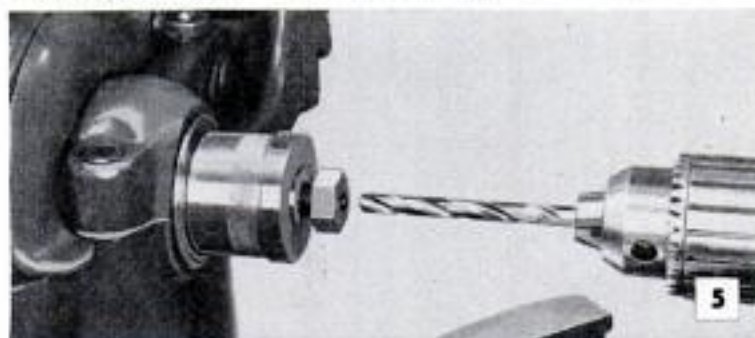
Drilling the pivot bolt axially also can be done in the lathe or drill press. Hole is for insertion of \frac{1}{4} -in. attachment bolt
