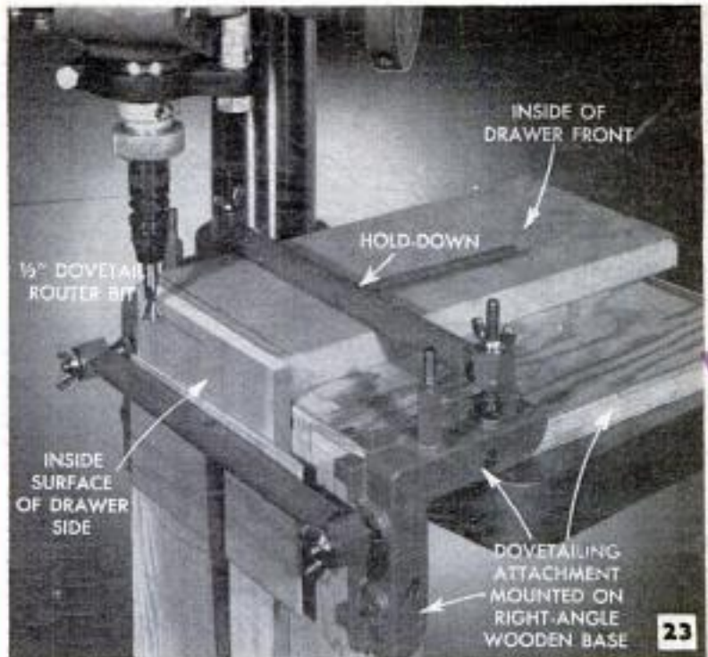
Multiple dovetails, such as used in drawer construction are the easiest of all to cut with the aid of the dovetailing jig shown
