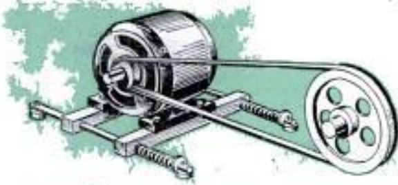
Compression springs provide constant tension on belt between motor and pulley. Simple mount consists of lengths of wood to which motor is bolted. Mount slides on two rods
