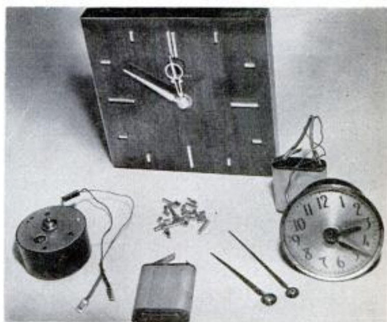
Completed battery-powered clock is in the background, with the kit units in the left foreground. Clock movement and battery are shown at the right assembled as an auto-clock replacement.
