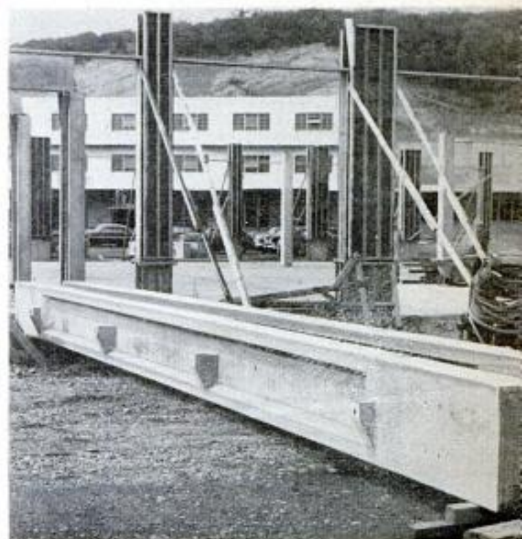
Concrete from traveling bucket is dropped into the form. Wires in form have already been placed under extreme tension. Below, girders ready for erection
