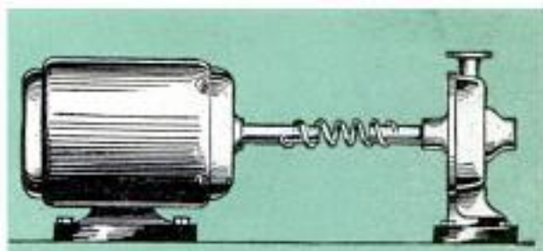
A temporary shock-absorbing coupling between electric motor and pump or other machine can be made from heavy spring of same or slightly smaller diameter than the shafts
