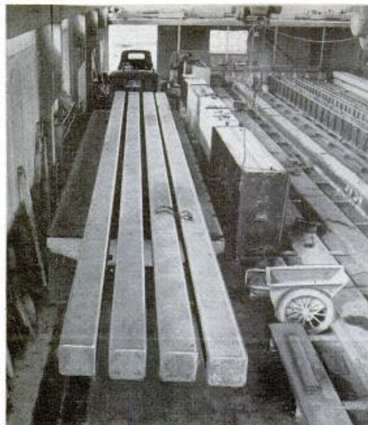
Four 50-foot lengths of piling made of prestressed concrete are shipped by truck, like other materials, to building site
