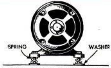
Springs under electric motor assure quiet, vibration-free running. Adjusting length of each bolt against spring tension provides means of aligning shafts
