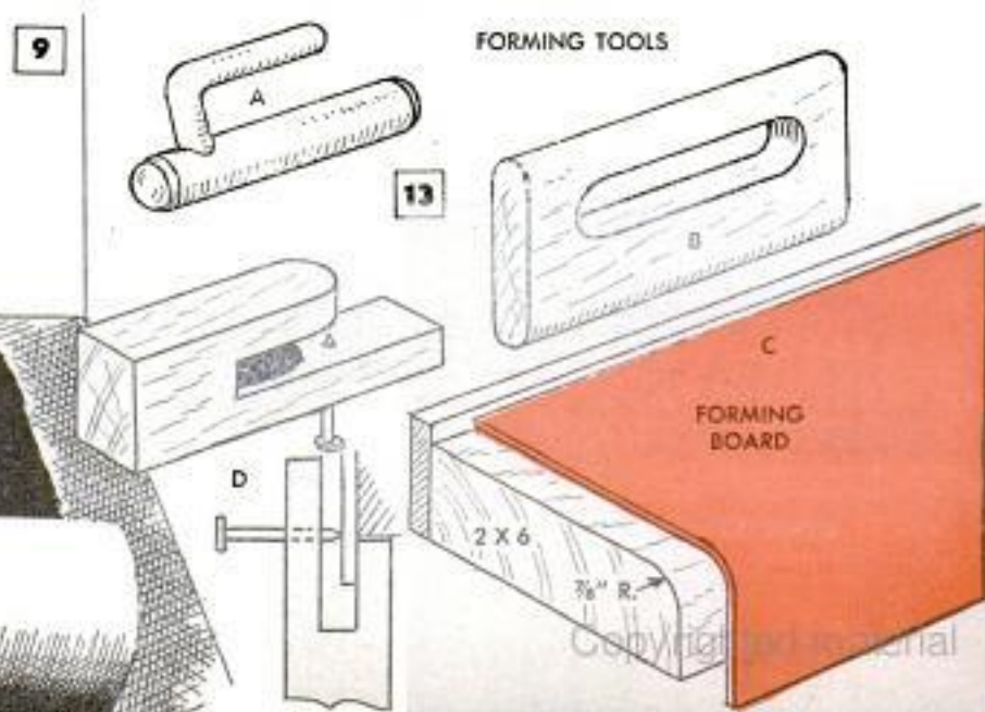
Below are shown tools that can be purchased or made which aid fitting and shaping cove base in corners
