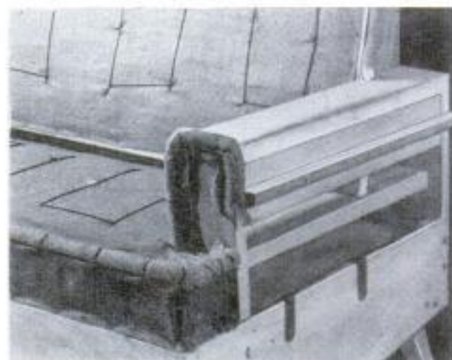
Above, close-up view of arm and corner of seat show how edge roll should look. Roll is tacked to arm and sewed to seat. Long stitches fasten burlap to springs
