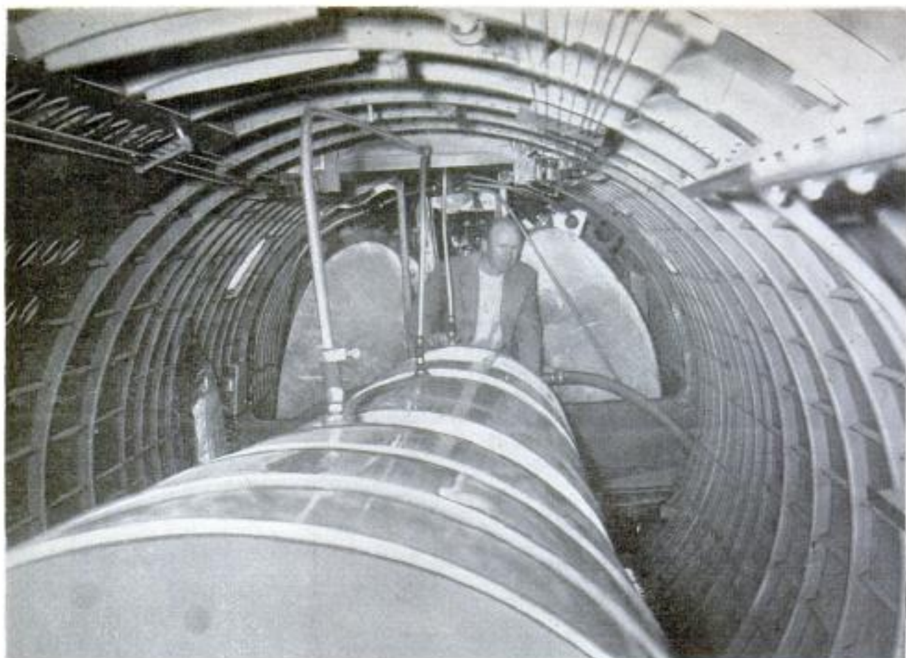
Built to carry bombs, the B-17's fuselage is almost filled by the eight interconnected insecticide tanks
