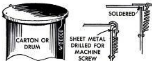
The lids on cartons, drums and garbage cans will be held on tightly if springs are used in one of the three ways shown in detail above. Place the springs under just enough tension to hold the lids firmly
