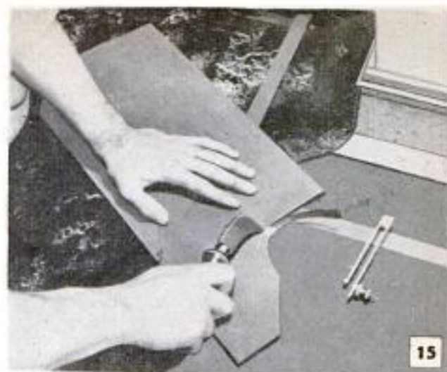
Above, linoleum on self corner is cut at 45-deg. angle down to middle of fillet on outside corners
