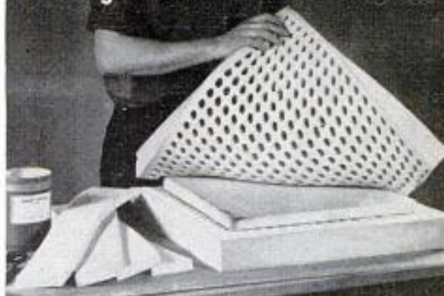
Above, solid slab stock is sandwiched between two cored slabs and then all three are cemented together
