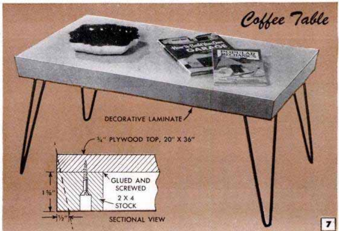
HAIRPIN LEG
