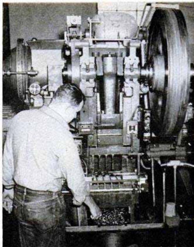
Copper cups are fed into die press which makes four or five precise "draws" to form the bullet jackets
