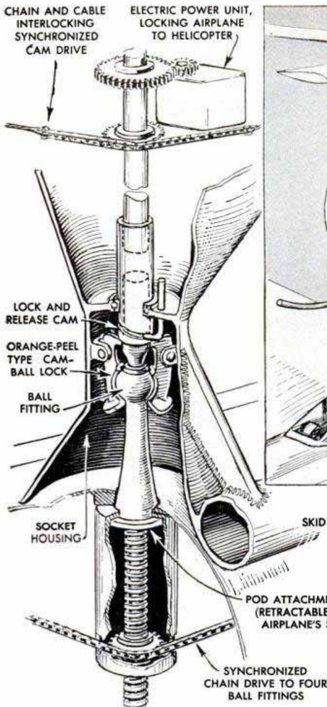
Sketch of Doctor Bennett's quick-release mechanism, left, for locking airplane to helicopter. Carrying craft would straddle the cockpit canopy of fighter below
