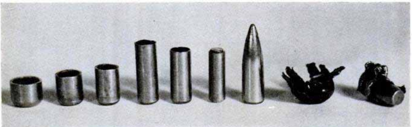
How a bullet is made: Left to right, copper jacket is stamped out as a cup; three stages of jacket being drawn to shape; trimmed jacket; lead core; completed bullet; two mushroomed bullets which killed big game
