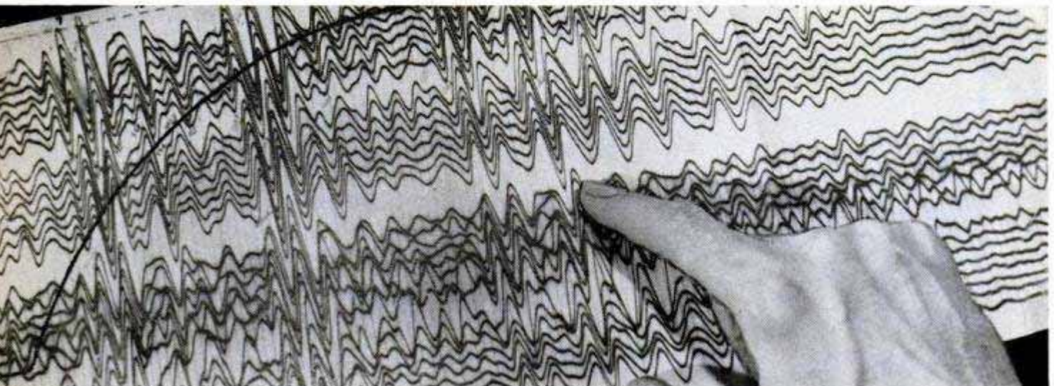
Finger points to broad wiggles that denote reflections of shock wave from rock structures beneath the surface
