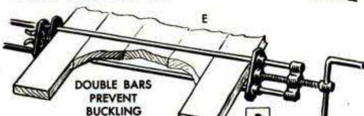
EXCESSIVE PRESSURE CAUSES WORK TO BUCKLE
