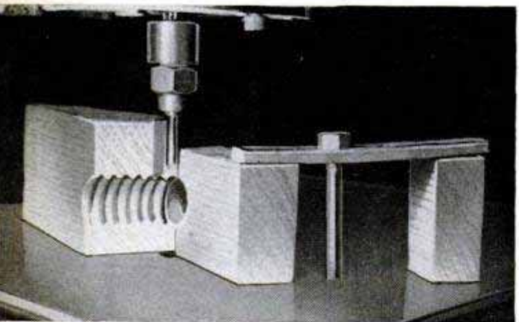
Photos above and below show jig set up on over-arm router for cutting a round-bottom thread. Here a table clamp rather than a C-clamp is used to hold jig in position. Note coarser pitch of thread
