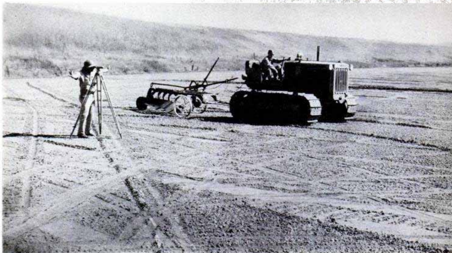
Surveyor followed by tractor and plow lays out paddies of different elevations in big California rice field
