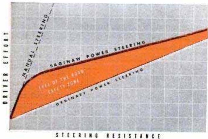
This simplified graph shows the basic difference between Saginaw Power Steering and ordinary types. The latter apply power at the slightest touch of the wheel, tending to cause overcontrol. Saginaw Power Steering goes into action only when more than "fingertip" pull is needed. This SAFETY ZONE is purposely provided to assure normal "feel of the road" and prevent oversteering.
