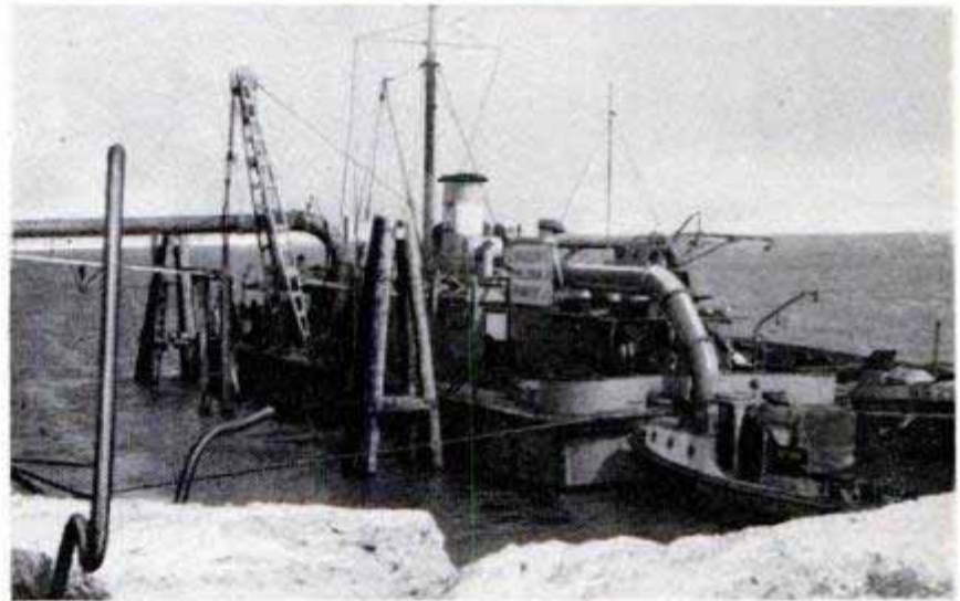
Above, sand-pumping ship. Pipe at left carries sand to shore. Barge is behind ship. Below, sand pouring from pipe line onto rebuilt beach
