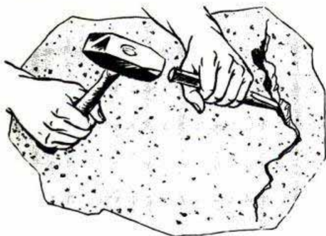
To seal cracks in walls, undercut with cold chisel, above, and fill with cement-paint mortar, as below
