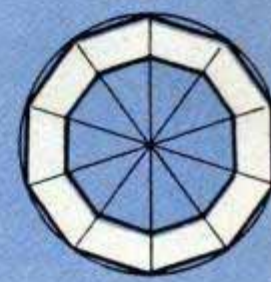
10 SIDES — DECAGON CENTER ANGLE—36° MITER—72° BEVEL—18° OUTSIDE CIRCLE—.618 INSIDE CIRCLE—.650
