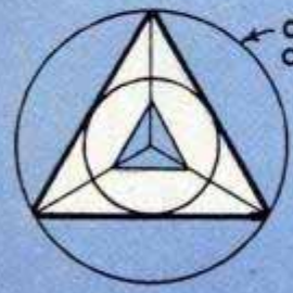
3 SIDES — TRIANGLE CENTER ANGLE—120° MITER—30° BEVEL—30° OUTSIDE CIRCLE—1.732 INSIDE CIRCLE—3.464
