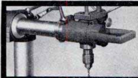
DRILL PRESS. 3" stroke, 18" throat. Drill, rout or mortise at any angle, in 36" circle.
