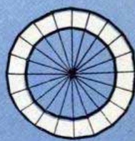
20 SIDES CENTER ANGLE—18° MITER—81° BEVEL—9° OUTSIDE CIRCLE—.313 INSIDE CIRCLE—.317
