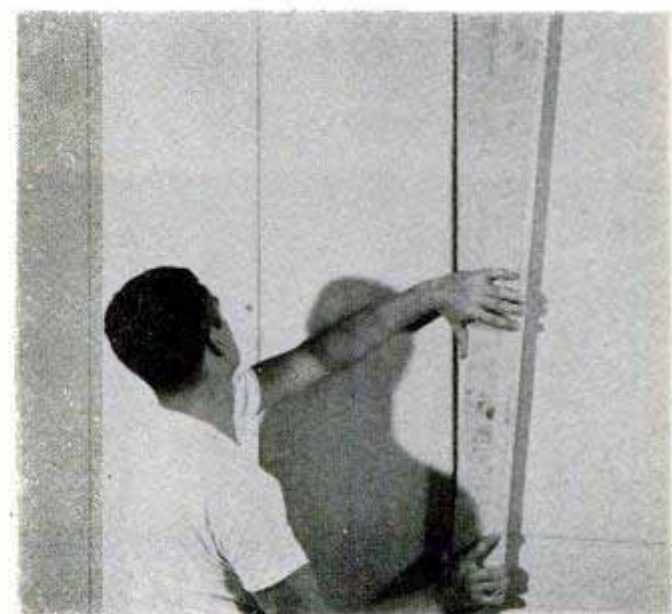
Above, place the first panel at a corner and plumb it with a carpenter's level. Press board lightly against surface to assure even adhesion. Below, succeeding panels are kept snug by tapping with 2 x 4
