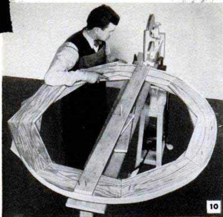
SAWING TO SHAPE AFTER ASSEMBLY IS ONE METHOD OF MAKING A SEGMENT RING. THIS METHOD AND TWO OTHERS ARE SHOWN IN THE DETAILS BELOW
