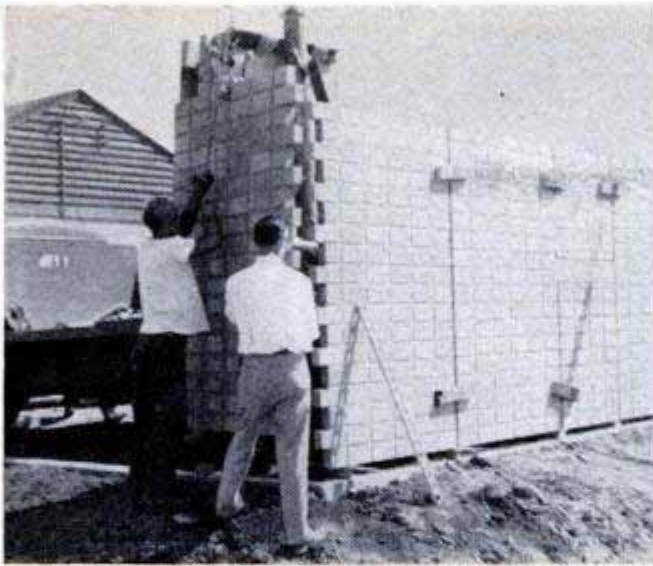
Workman, left, lowers a large brick-wall panel into place. Panel fireplace at right is assembled in an hour
