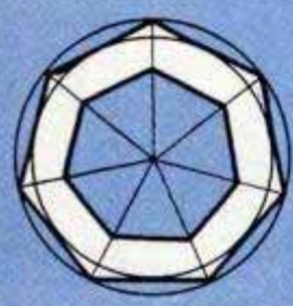
7 SIDES — HEPTAGON CENTER ANGLE—51.43° MITER—64.28° BEVEL—25.71° OUTSIDE CIRCLE—.868 INSIDE CIRCLE—.963
