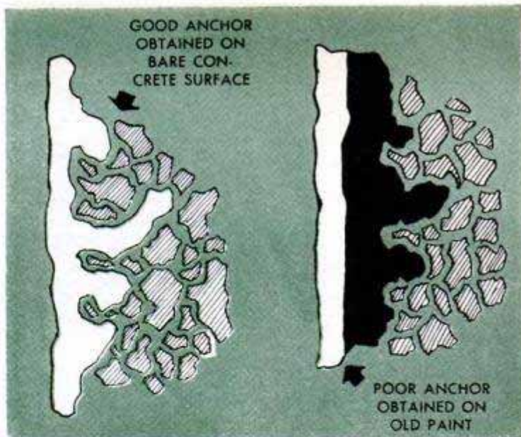
Drawings above illustrate how removal of old paint from masonry surface permits new coating of cement paint to obtain good anchor on the porous surface
