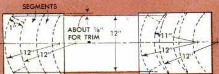
ALL EXAMPLES 6-SIDED FIGURE TO FINISH 24" DIA. (ALLOW FOR TRIMMING IF REQUIRED)
