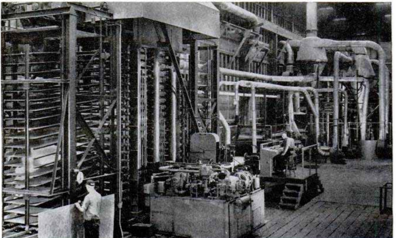
Chips are softened in cooker section, right, before entering hot press, left. Few workers are needed in process
