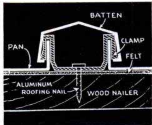
Cross-section drawing shows how panels are joined by overlapping clamp that is topped by batten. Below, finished roof laid with the portable machine
