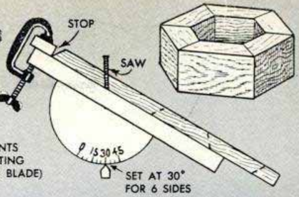
MITERED SEGMENTS ARE CUT BY SETTING MITER GAUGE AT REQUIRED ANGLE
