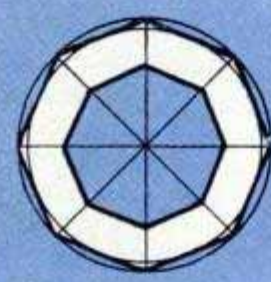
8 SIDES — OCTAGON CENTER ANGLE—45° MITER—67.5° BEVEL—22.5° OUTSIDE CIRCLE—.765 INSIDE CIRCLE—.828
