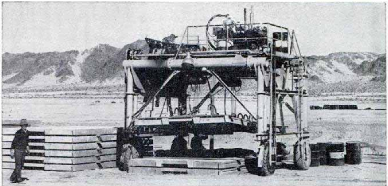
Converted lumber carrier gently lowers a partially cured concrete section into position on stock pile
