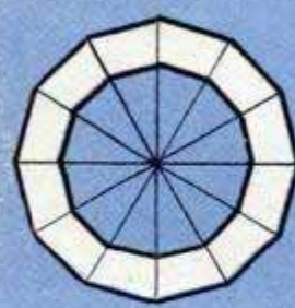
12 SIDES CENTER ANGLE—30° MITER—75° BEVEL—15° OUTSIDE CIRCLE—.518 INSIDE CIRCLE—.536
