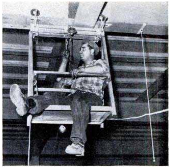
Ceiling work was done from an ingenious "trolley scaffold" in sections that had a roof but no floor
