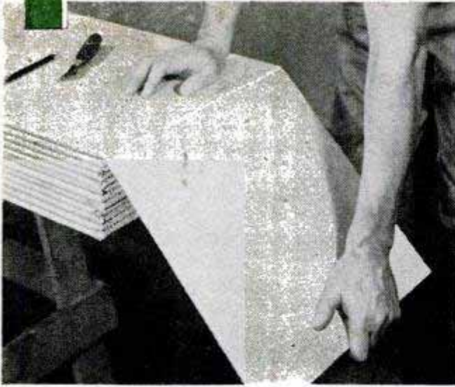
Panels are cut by cutting through paper covering on both faces, then snapping off to break gypsum core
