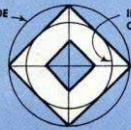
4 SIDES — SQUARE CENTER ANGLE—90° MITER—45° BEVEL—45° OUTSIDE CIRCLE—1.414 INSIDE CIRCLE—2.000
