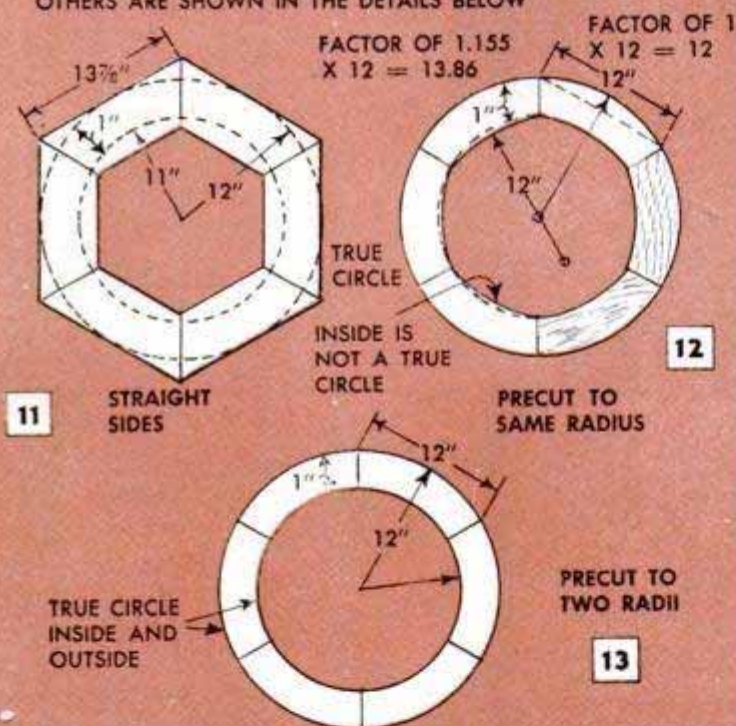
SAWING TO SHAPE AFTER ASSEMBLY IS ONE METHOD OF MAKING A SEGMENT RING. THIS METHOD AND TWO OTHERS ARE SHOWN IN THE DETAILS BELOW
