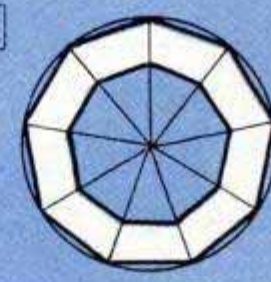
9 SIDES — NONAGON CENTER ANGLE—40° MITER—70° BEVEL—20° OUTSIDE CIRCLE—.684 INSIDE CIRCLE—.728
