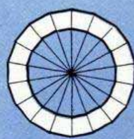
18 SIDES CENTER ANGLE—20° MITER—80° BEVEL—10° OUTSIDE CIRCLE—.347 INSIDE CIRCLE—.353
