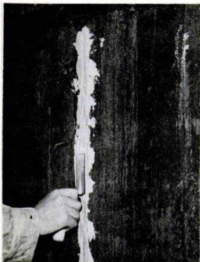
To seal cracks in walls, undercut with cold chisel, above, and fill with cement-paint mortar, as below
