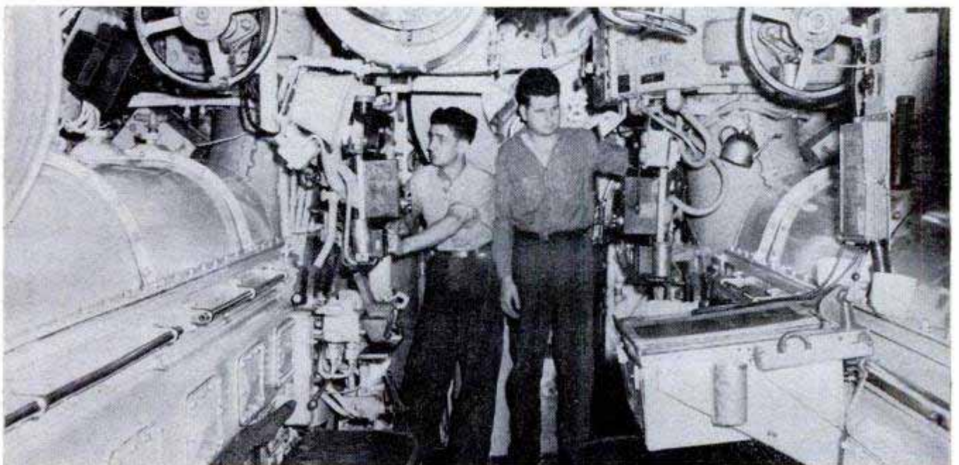
Throttleman and oiler check two of the four engines which propel the submarine and charge the batteries
