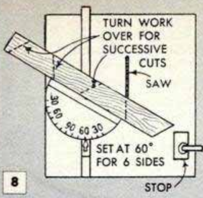
MITERED SEGMENTS ARE CUT BY SETTING MITER GAUGE AT REQUIRED ANGLE
