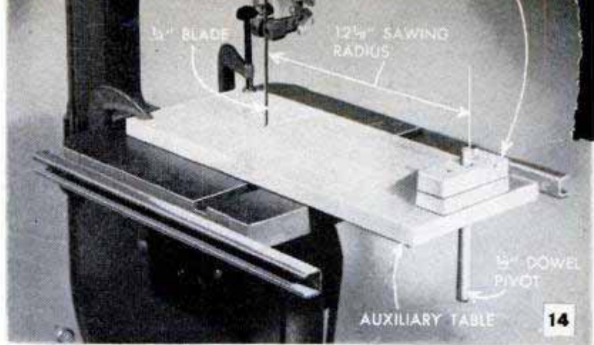
In order to work circular segments on a small bandsaw, an auxiliary table carrying the pivot pin is clamped to the bandsaw table. Two raising blocks are required for two thicknesses
