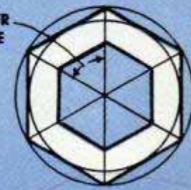
6 SIDES — HEXAGON CENTER ANGLE—60° MITER—60° BEVEL—30° OUTSIDE CIRCLE—1.000 INSIDE CIRCLE—1.155
