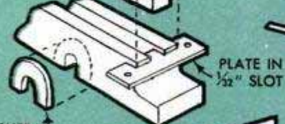
3/16" WASHER SOLDERED
