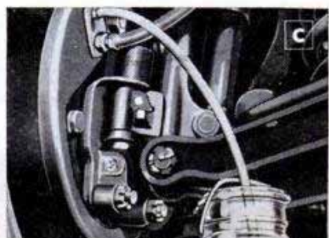
Leave reconditioning and servicing of hydraulic brakes to your serviceman as he will have special equipment required. Dismantled master and wheel cylinders are shown above. Below, bleeding air out of brake lines
