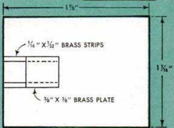
CAB ROOF
