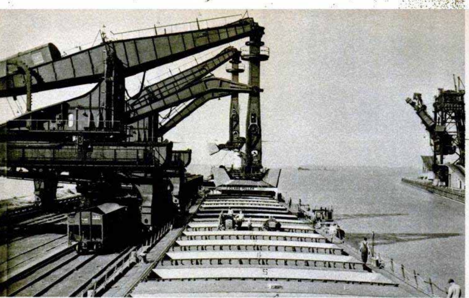
Here's a view aft of leg men unloading the cargo. Some lake ships are quite long; one measures 714 feet
