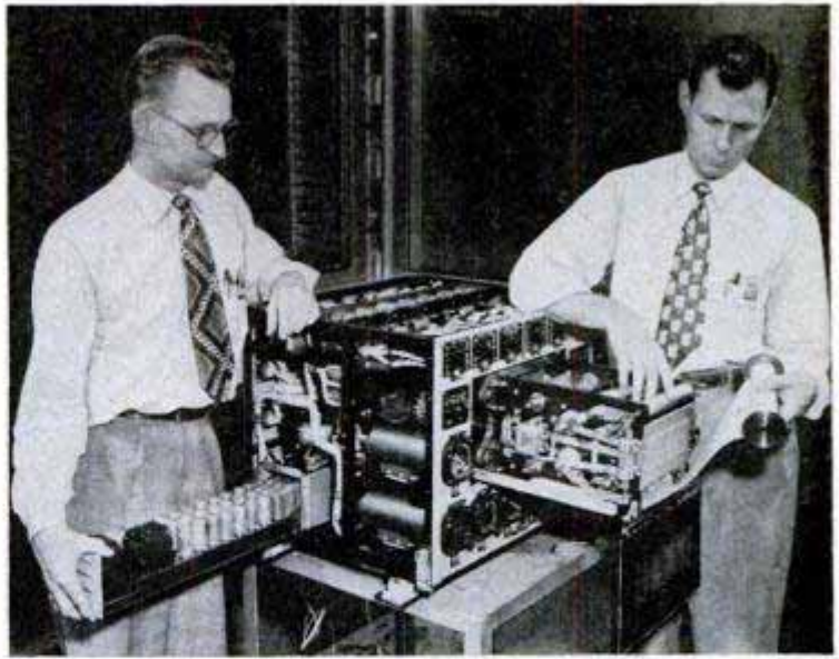
Punching flight plan into a tape. Man at right points to 430 sensing pins which detect data holes on tape
