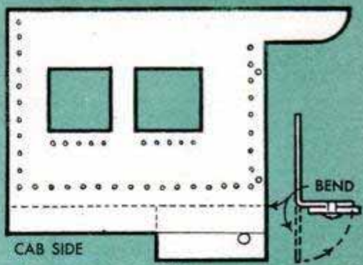
CATWALK ASSEMBLY
