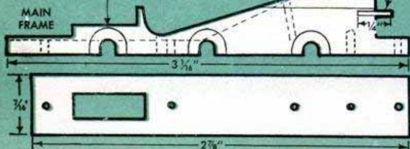
3/16" WASHER SOLDERED
