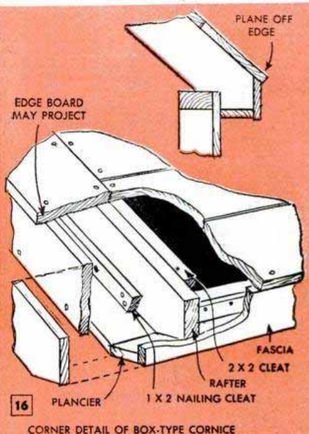
CORNER DETAIL OF BOX-TYPE CORNICE
