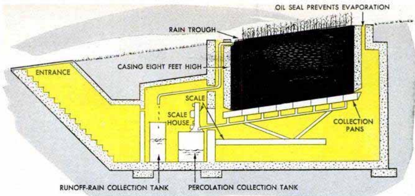
Scale built beneath 65-ton "block" of earth preserves natural drainage, yet weighs all moisture on the plot
