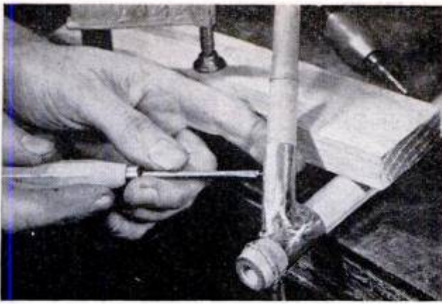
Diagonal brace is inserted in sheet-metal bracket fitted to chair leg. Wood screw prevents slipping
