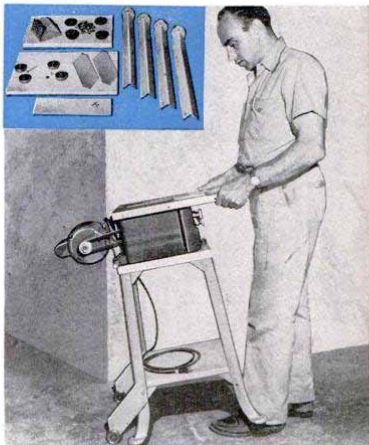
→ PORTABLE POWER-TOOL STAND comes knocked down and consists of four steel legs with bolt holes drilled, brackets, four rubber feet for legs and ball-bearing rollers. The top and shelf can be made by the purchaser
