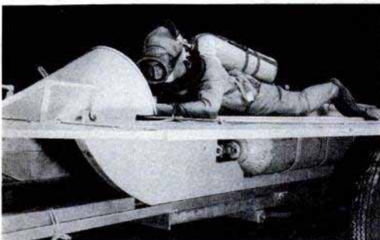
Twin compressed-air tanks are built into the runners. Frame of the submarine sled is made of wood covered with a skin of aluminum. Below, forward and aft diving planes are controlled by hands and feet. Holes near elbows give access to air valves
