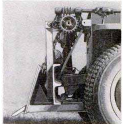
Raising gear is operated by a crank attached to extended shaft supported by a bracket welded to the Jeep body
