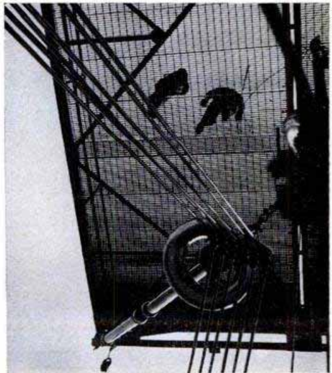
"Doughnuts" around antenna lead-in trunk prevent corona discharge. Right, ant's-eye view of transmitter tower
