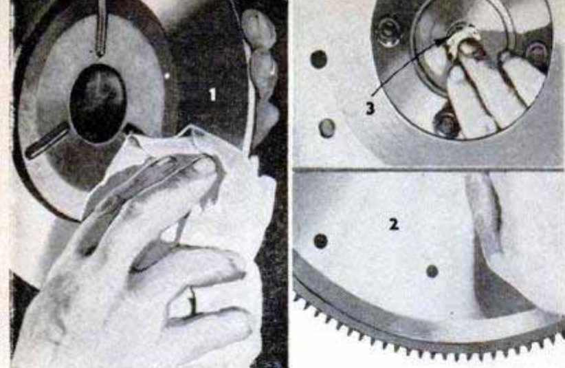
Do a careful job on the clutch, especially on the pressure plate, flywheel and pilot bearing, parts 1, 2 and 3
