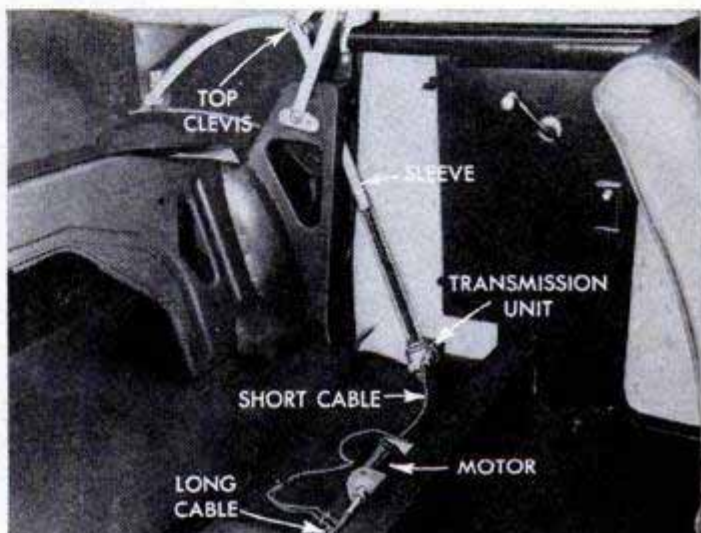
Dismantle the electrical lift for convertible top and clean and dry all the parts. Then relubricate the transmission unit
