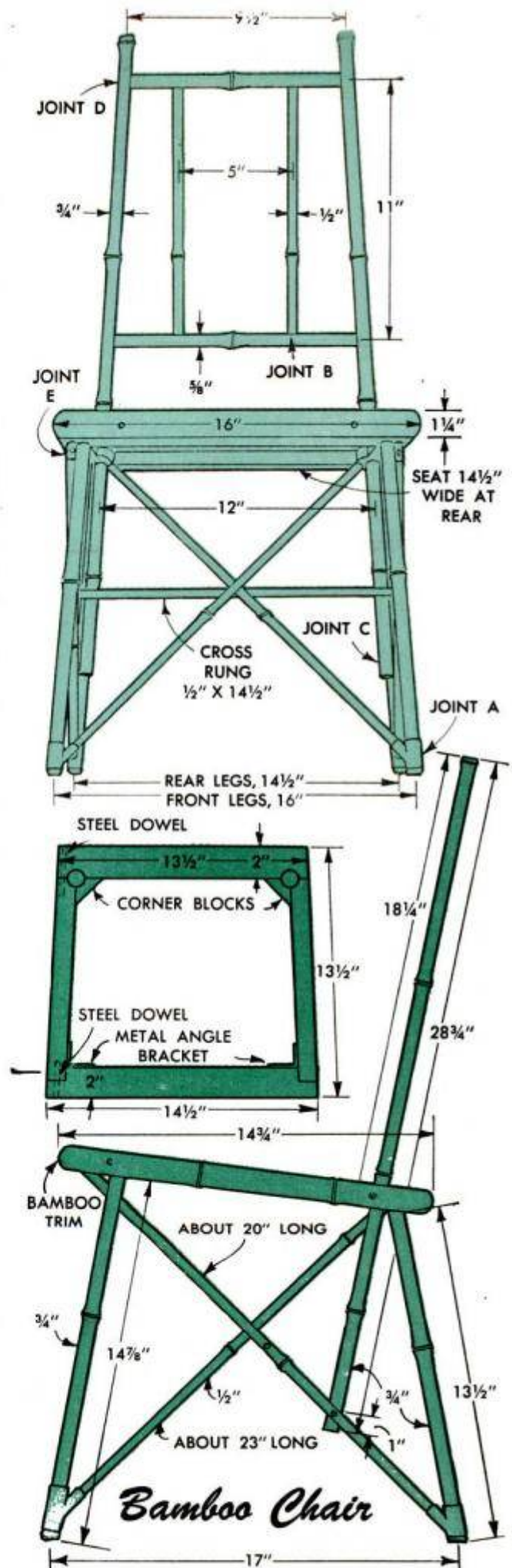
Diagonal brace is inserted in sheet-metal bracket fitted to chair leg. Wood screw prevents slipping
