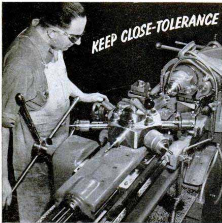
South Bend 2-H Precision Turret Lathe —1" collet capacity, 16 1/4" swing, 96 power turret feeds, 48 cross slide feeds, 48 carriage feeds, 48 thread cutting feeds.
