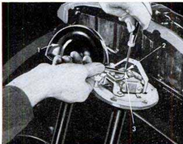
Above, door panels should be removed so that glass-lifting mechanism can be cleaned and serviced. Below, it may be necessary to readjust the horn by removing cover and adjusting the screws, parts 1, 2 and 3
