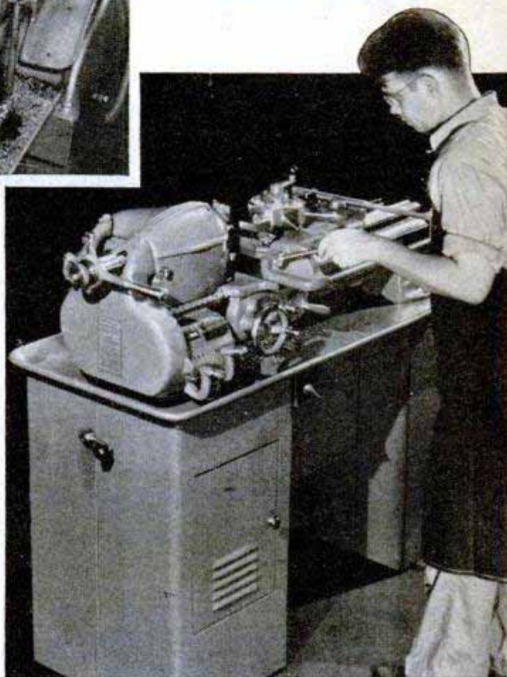
South Bend CL930-Z Precision Turret Lathe —1/2" collet capacity, 9 1/4" swing, 48 carriage feeds, 48 thread cutting feeds, handlever cross slide, handlever turret.
