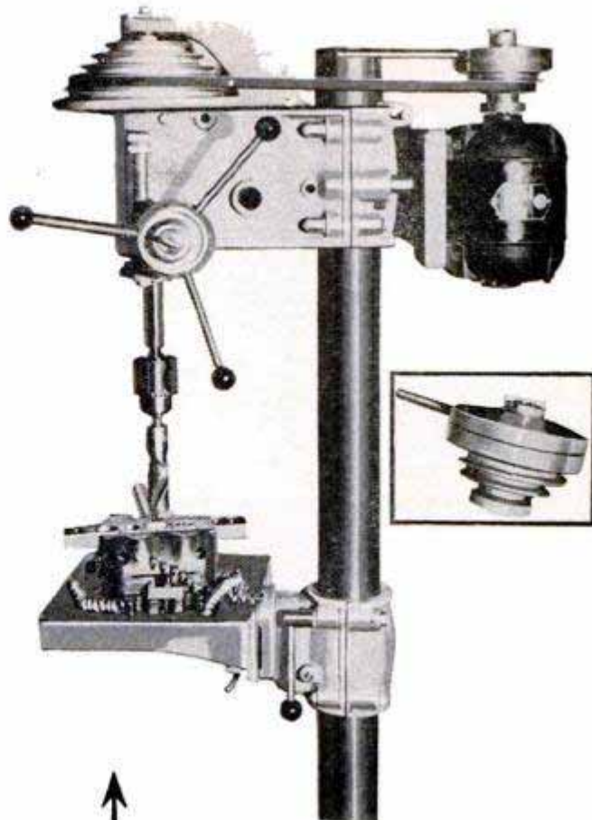
↑ SPEED-REDUCING PULLEY has been designed to increase the use range of a small drill press. Reducer is gear driven and models are available with 4½:1 and 7:1 reductions, the speeds ranging from 75 to 2000 r.p.m. through six variations on a three-step pulley
