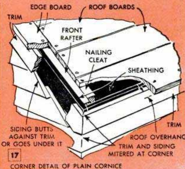
CORNER DETAIL OF PLAIN CORNICE
