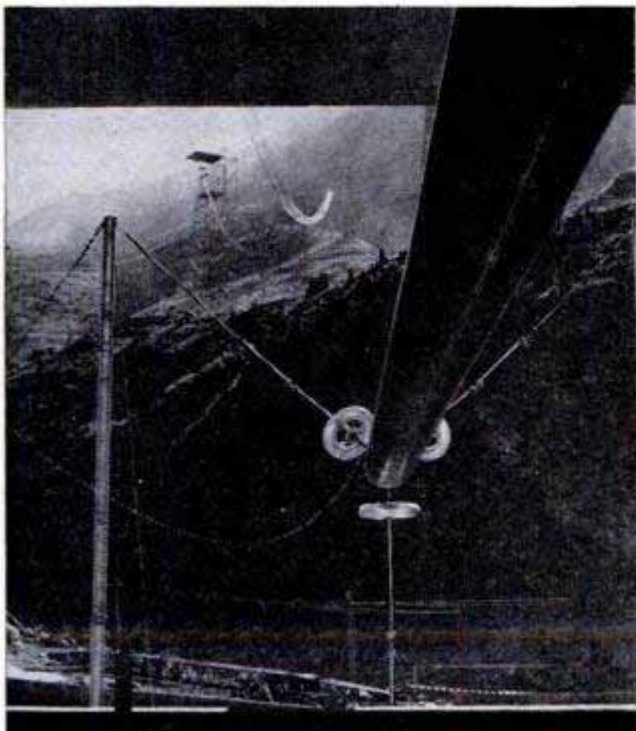
"Doughnuts" around antenna lead-in trunk prevent corona discharge. Right, ant's-eye view of transmitter tower
