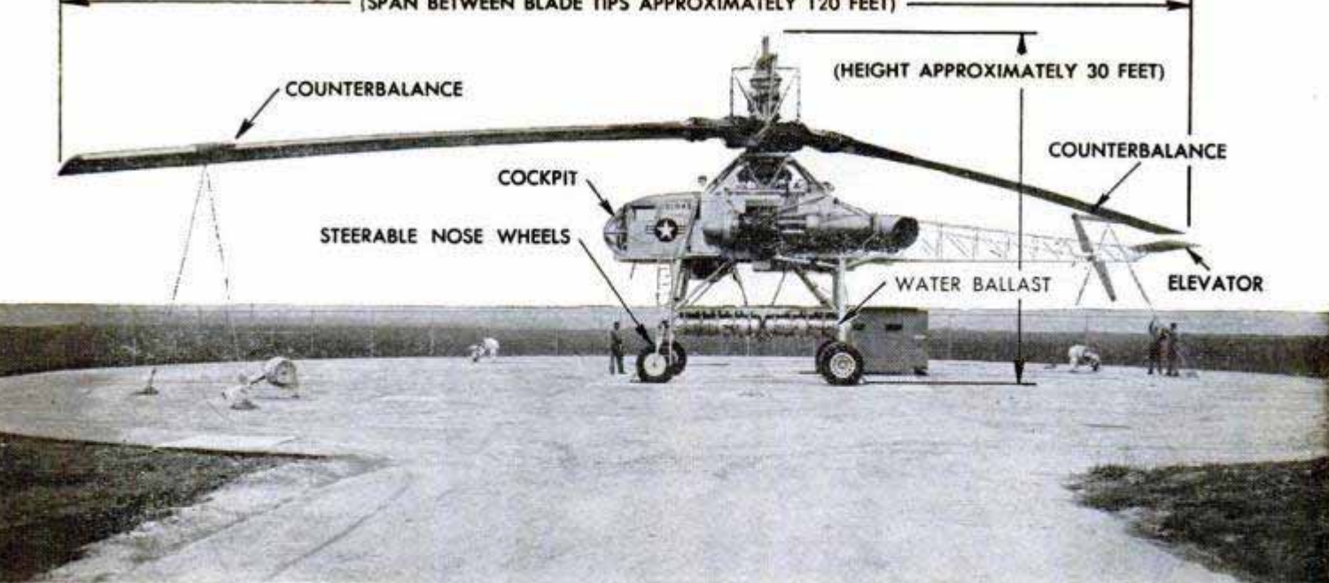
Tied down during ground tests, the huge XH-17 dwarfs near-by workers. During earlier experiments it broke loose from its moorings and was slightly damaged
