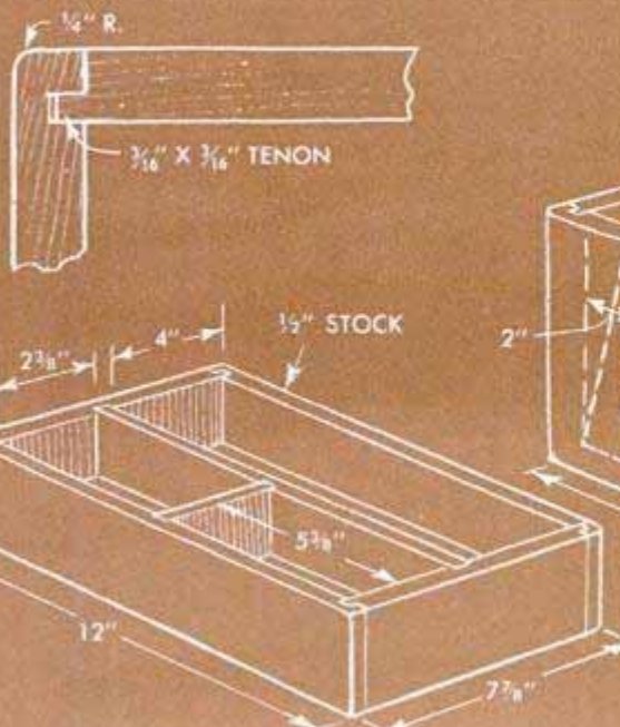
REMOVABLE SMALL-TOOL TRAY
