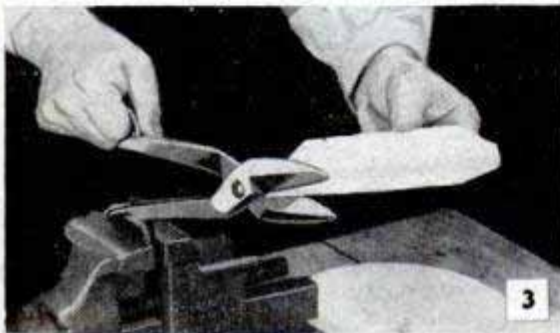
Snips should be held square with work, except aviation type which cut best with right tilt. Below, vise mounting aids in cutting thick stock
