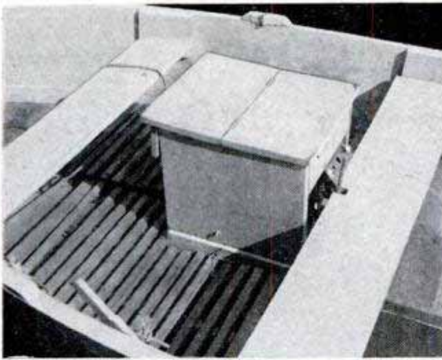
Top of the engine cover or hood should be hinged for easy access to starting cord. Note the open ends
