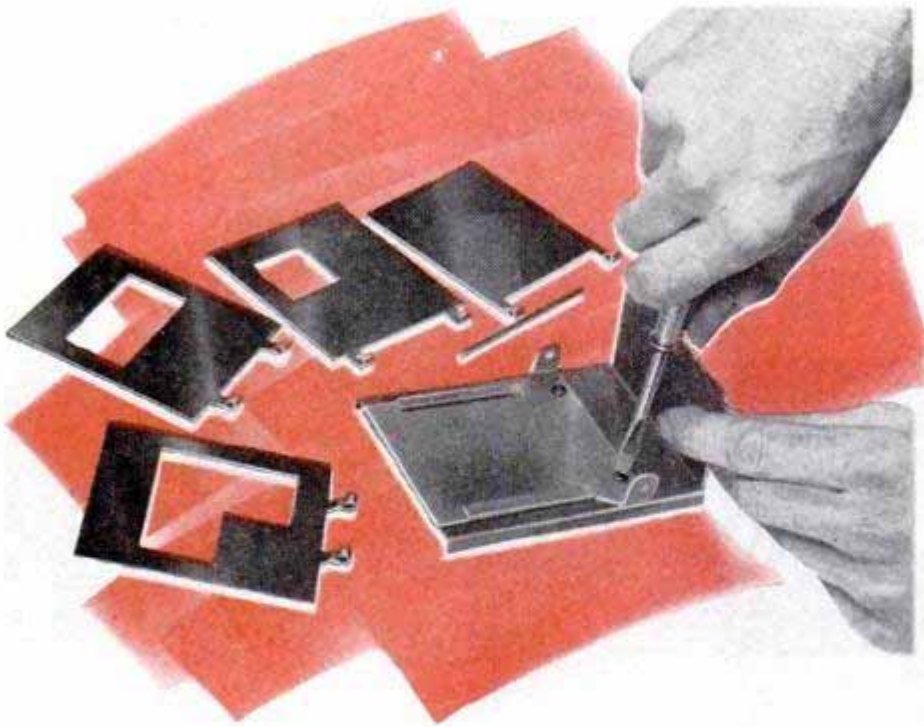
Here are all the parts cut and ready for final assembly. Two sheet-metal screws are used to fasten the paper holder to the base member
