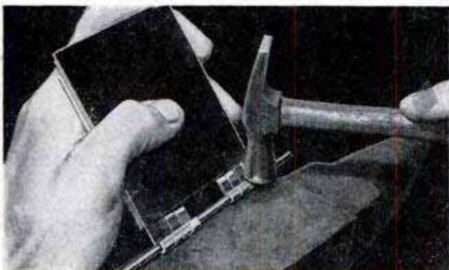
Brazing rod, which serves as hinge pin, is used in forming eyes in ends of tabs by tapping metal around it
