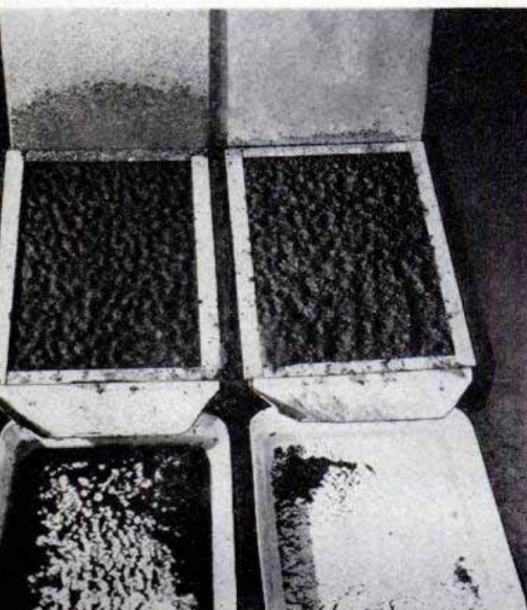
Treated soils were tested under this rain-making machine that duplicates nature's rainfall. Below, soil at left was untreated. Notice the runoff and splatter. Soil in right flat was mixed with Krilium
