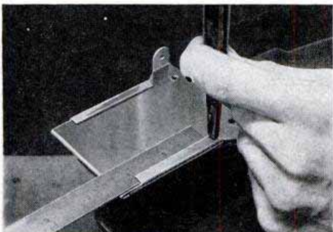
Channels which guide the paper are formed by bending the metal over a suitable shim such as a steel rule
