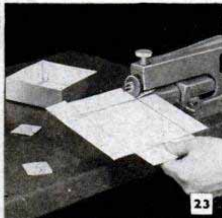
Straight cuts can be made freehand by following a pencil line, but a better way is to improvise a guide as in left-hand photo. Center photo shows how notches are cut to form box corners. Right-hand photo shows how a curved guide can be used to form a true radius. In this case, an ordinary washer served the purpose
