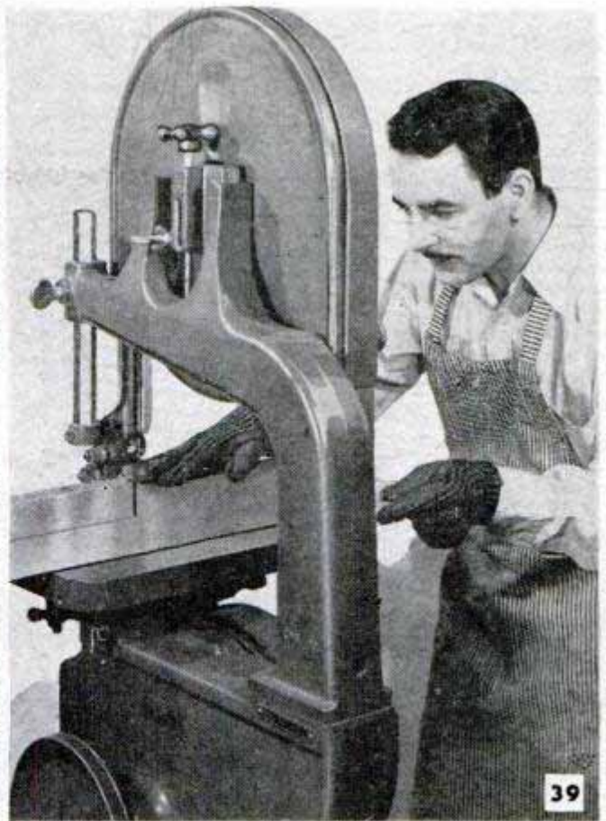
Bandsaw used as friction saw cuts fast and accurately on sheet metals of all kinds up to 1/8 in. thickness
