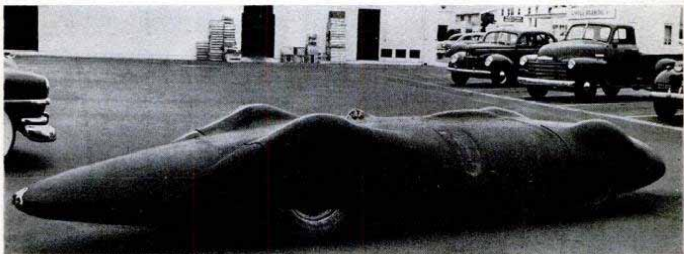
Side view of the Post-Hartelt hot rod displays its extreme streamlining. "Patch" on side is fuel tank
