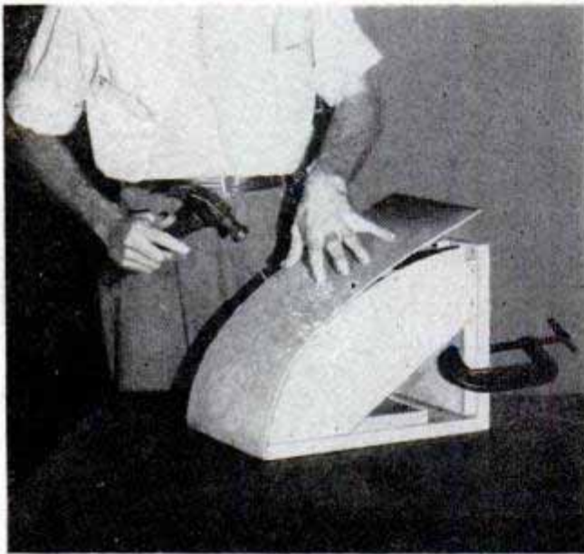
Above, compartment frontpiece is glued and nailed in place with brads. Heads are set below surface and holes filled. Below, after bandsawing to contour and applying facing, bottom frame is nailed to shelf
