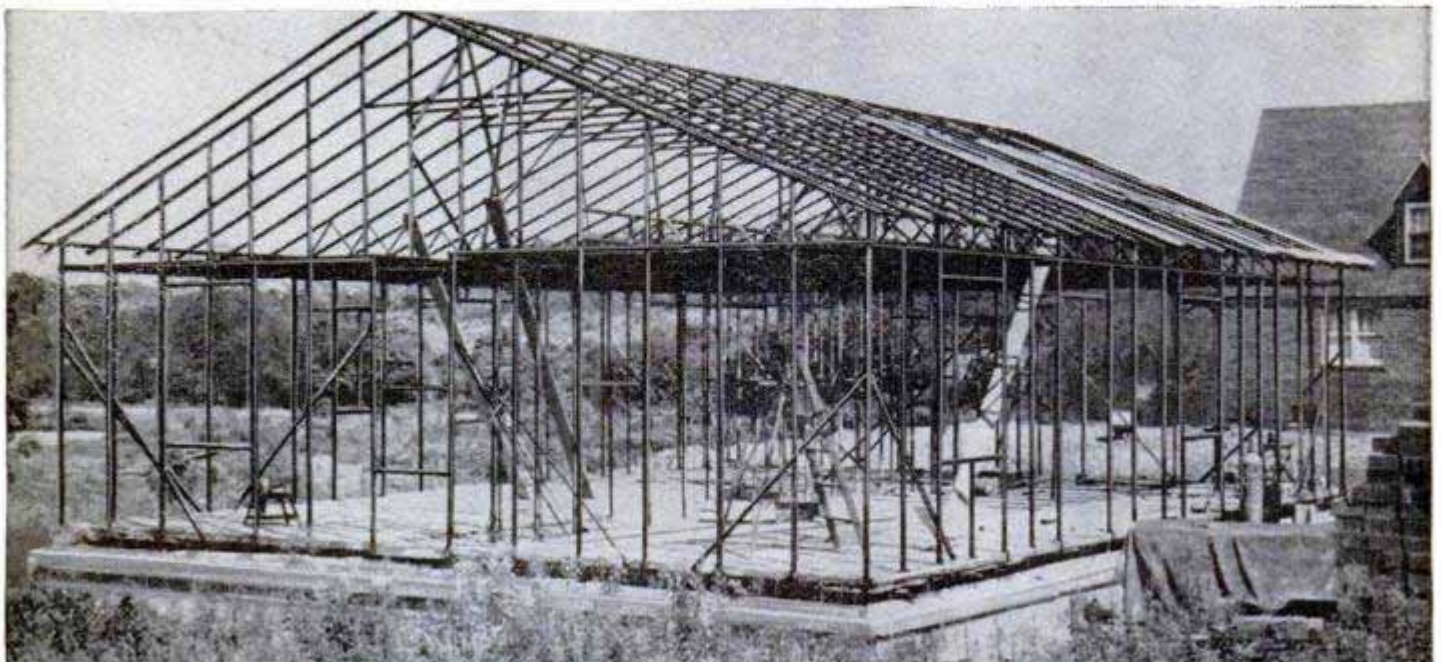
Wagner is covering the outside of his house with brick. The Celotex beneath the brick is fastened to the pipe framework. He estimates the cost at $5000
