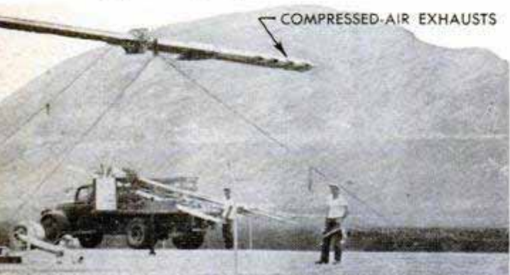
Air from compressors run by two turbojet engines is lifted up through the rotor shaft, above, and out to the rotor-blade tips. Fuel is burned at the exhaust outlets, providing a jet effect that turns the blades
