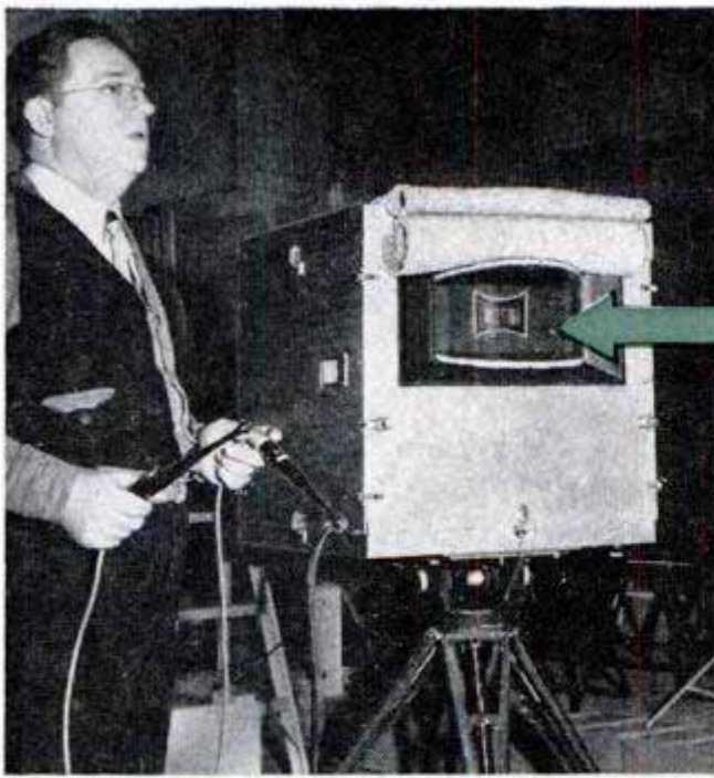
Three lenses look out through the hourglass-shaped slot in the camera front. Each lens covers about a third of the 146-degree angle of "vision." A single shutter is used. It rotates in front of the lenses at the point where their lines of view cross. Thick layers of absorbent material muffle noise from motor chamber
