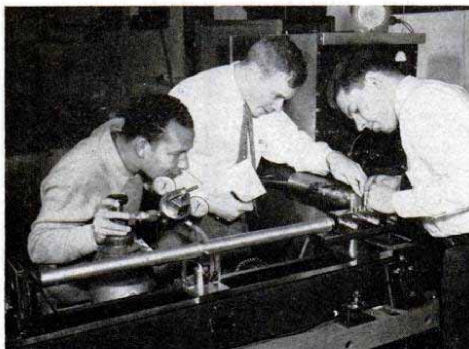
Specimen is placed in microscope. X rays pass through tube to film, left
