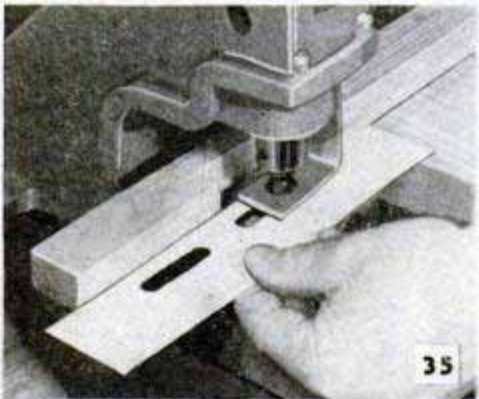
A hand punch does accurate slotting
