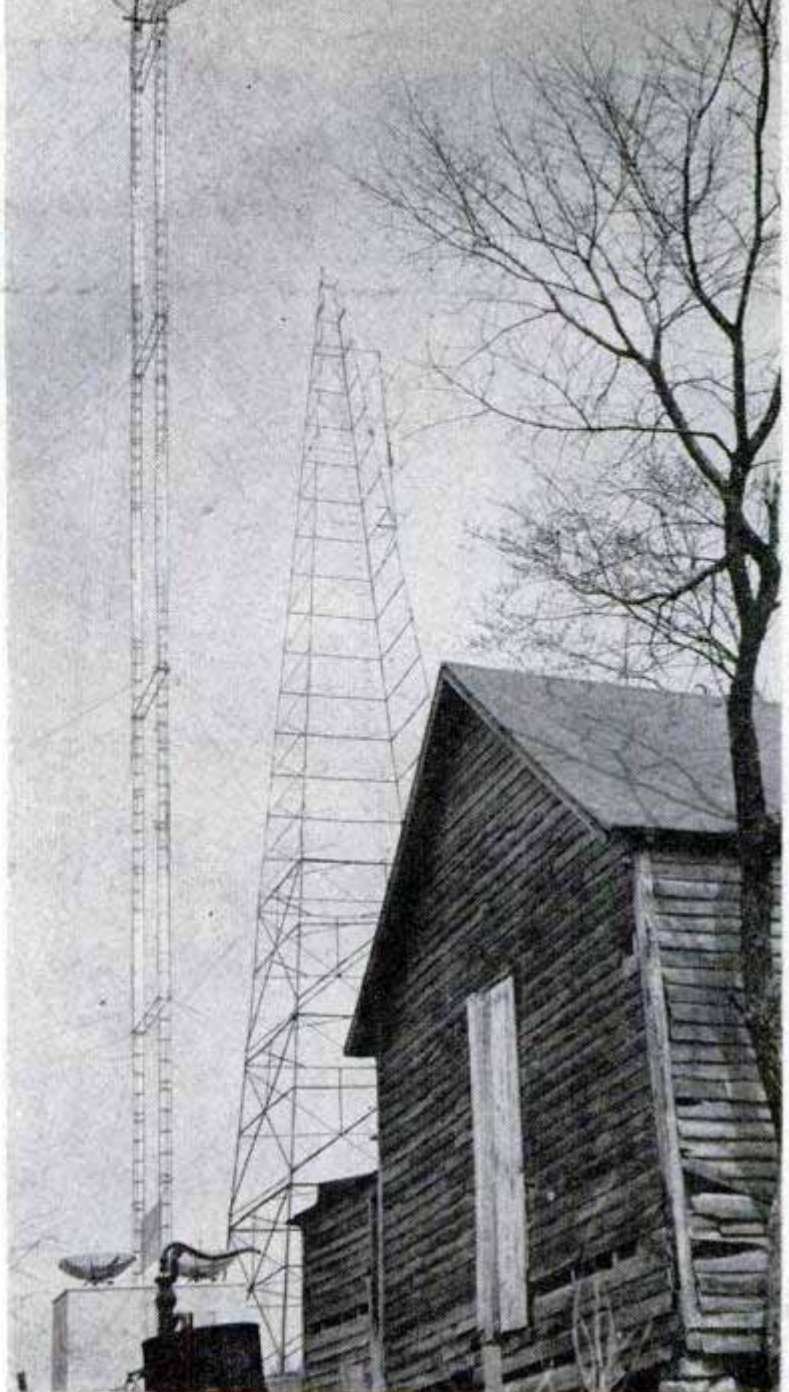
Above, microwave station near Pikes Peak, Ind., relays network shows to Bloomington from Cincinnati (see map below). Tower at left is used. Windmill tower at right was original installation. Transmitter is inside block house under "dishpans" at tower base
