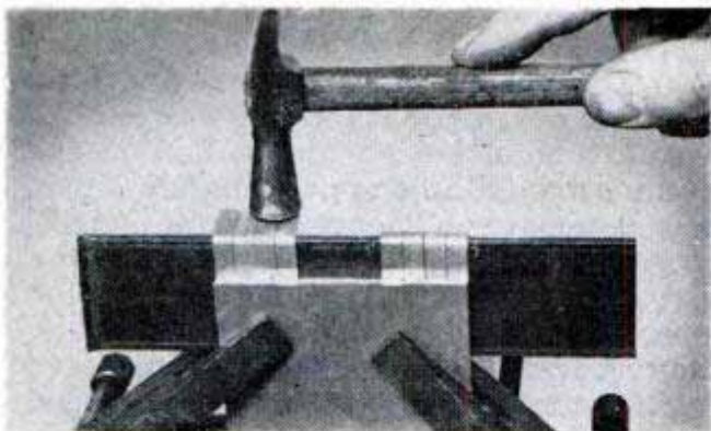
Offset hinge tabs on masks are formed by clamping stack to backing plate and hammering tabs over edge
