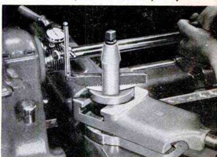
Bearing clearance
