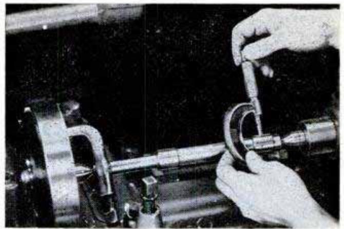
9 Testing alignment
