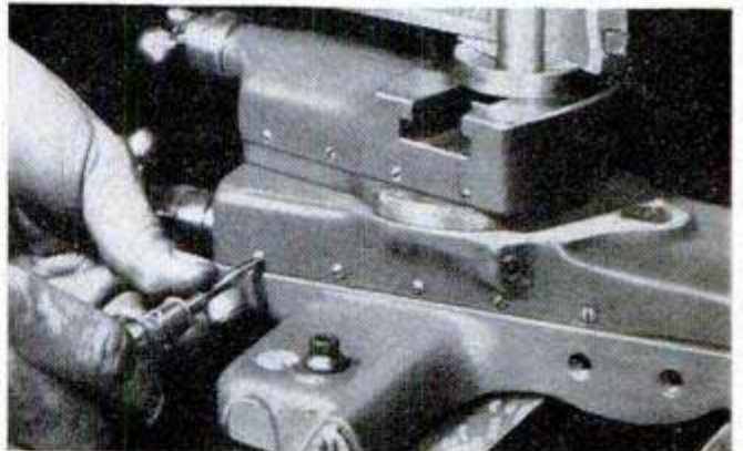
11 Gib clearance
