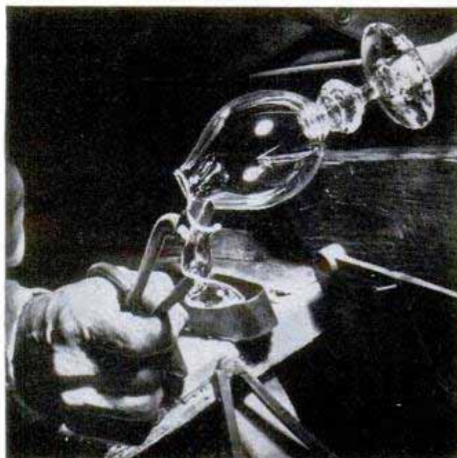
Shears snip excess glass from the end of a bubble just before it is opened to form the bowl of a goblet
