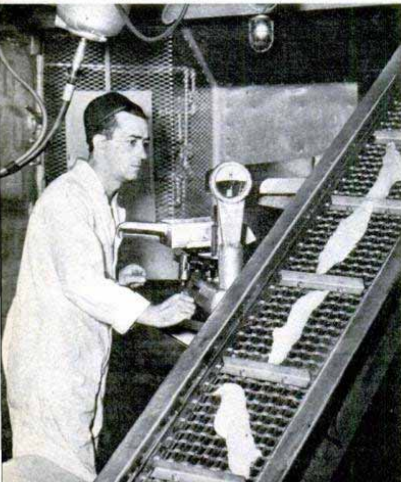
Close-up of a stainless-steel conveyor shows fillets being carried from cutters to weighers and packers
