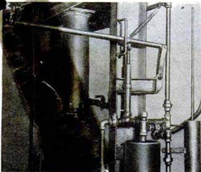
A hand-operated hydraulic pump gives the operator delicate control of pressure applied to the work
