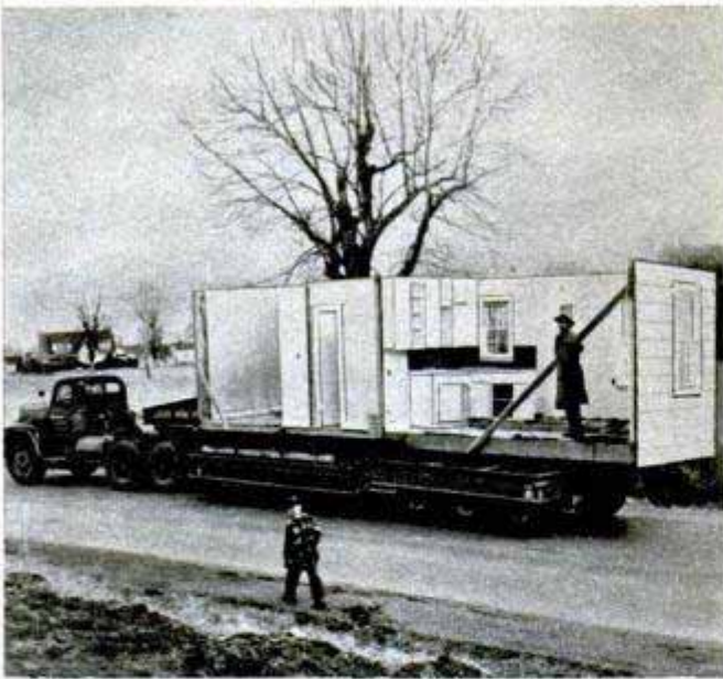
After being cut into five trailer-size sections, the factory-built house is trucked to the building site
