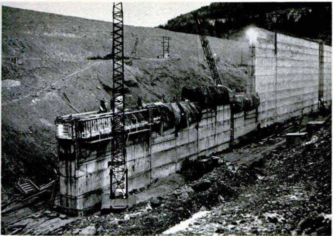
Banks of lamps glow around the just-poured upper sections of the wall. They warm the concrete for 72 hours
