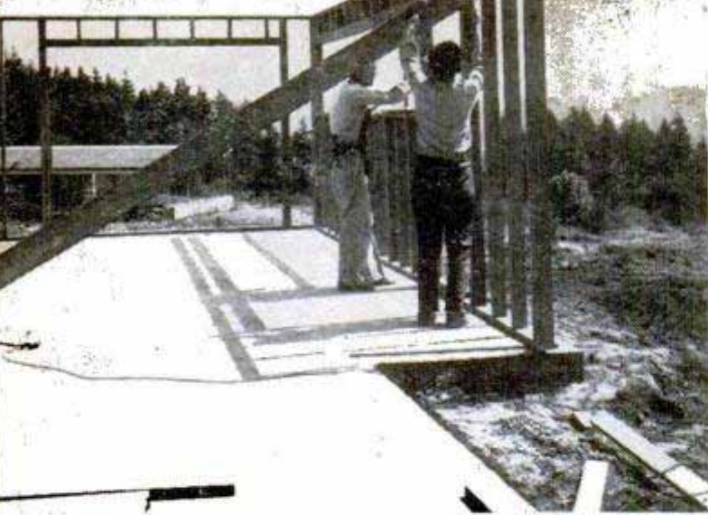
After the walls are "prefabbed" flat on the subfloor, they are raised, plumbed and braced. Later a second top plate will be added to tie wall sections together
