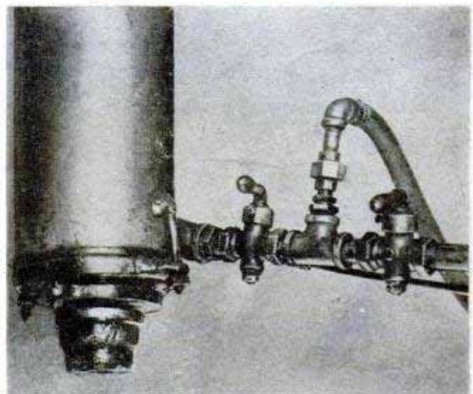
Valves control air pressure to hydraulic cylinder and reservoir. Press can be operated with one hand
