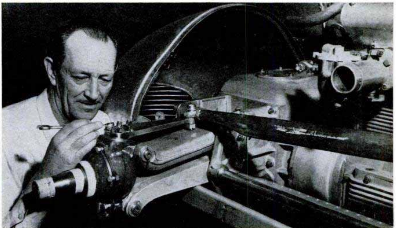
Front-wheel bearings of aluminum-built car are mounted on novel kingpins to keep wheels in perfect alignment
