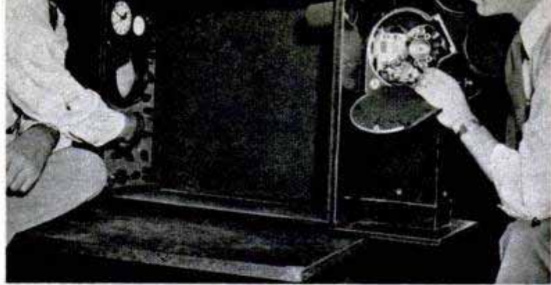
Camera automatically photographs flashes of lightning as recorded in waves on oscilloscope screen
