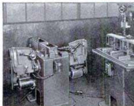
Another example of CRAFTSMAN utility . . . two CRAFTSMAN drill press heads used horizontally in special set-up for production-line side drilling
