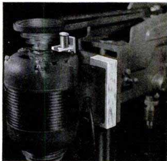
Here's the motor in place and belted to the drill-press spindle. Note spacer block
