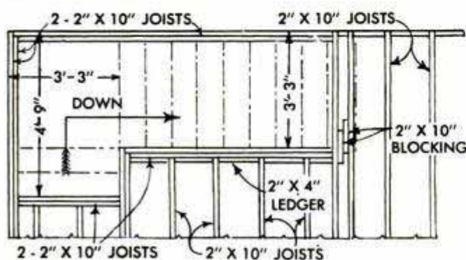
JOIST PLAN FOR BASEMENT STAIRWAY
