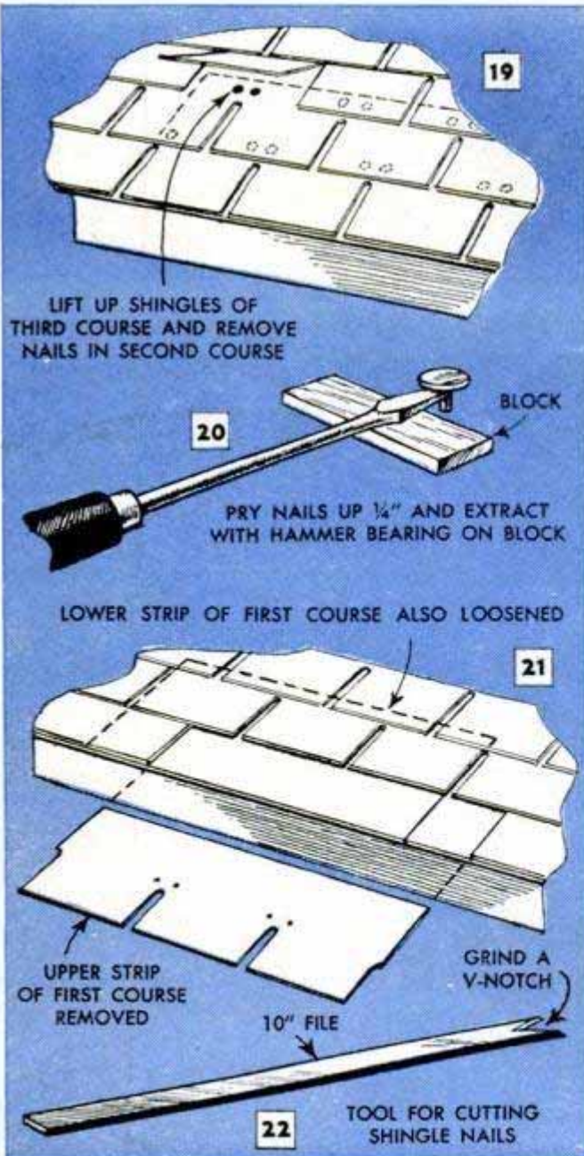
When applying new gutter hangers on old roofs, shingles should be lifted so that hanger can be nailed directly to the roof boards. On asphalt-shingle roofs, the individual shingles are easily removed for this job
