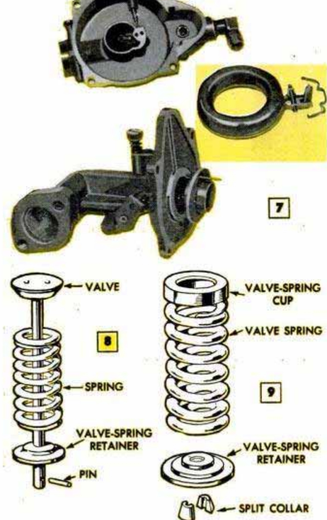
Above and below, cleaning the carburetor and grinding, or lapping, valves are important servicing operations on older engines with long records of extra-hard usage
