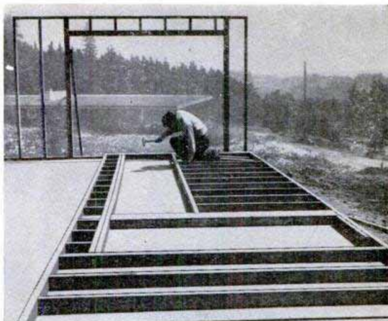
Typical 2 x 4 stud walls are "prefabbed" flat on the subfloor, all windows and door openings being framed in place before walls are erected. Two men can raise 20 to 30-ft. section easily
