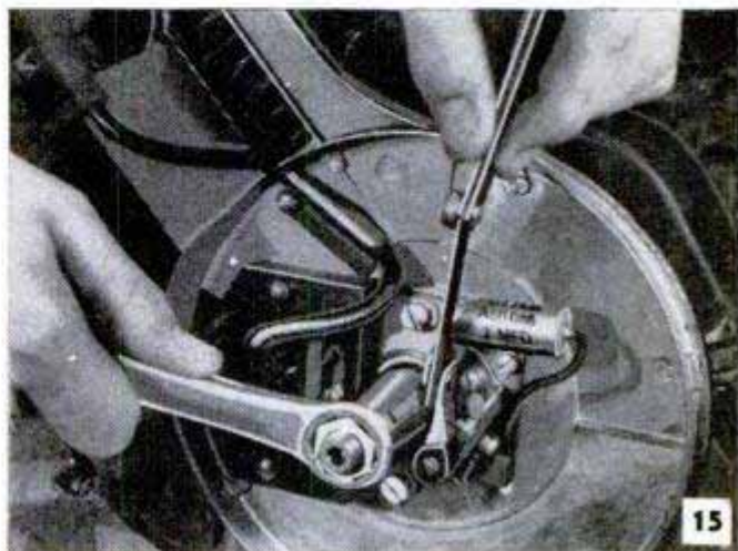
Then check distance points open with feeler gauge. Ordinarily, gap opening should be .20 in. but may vary
