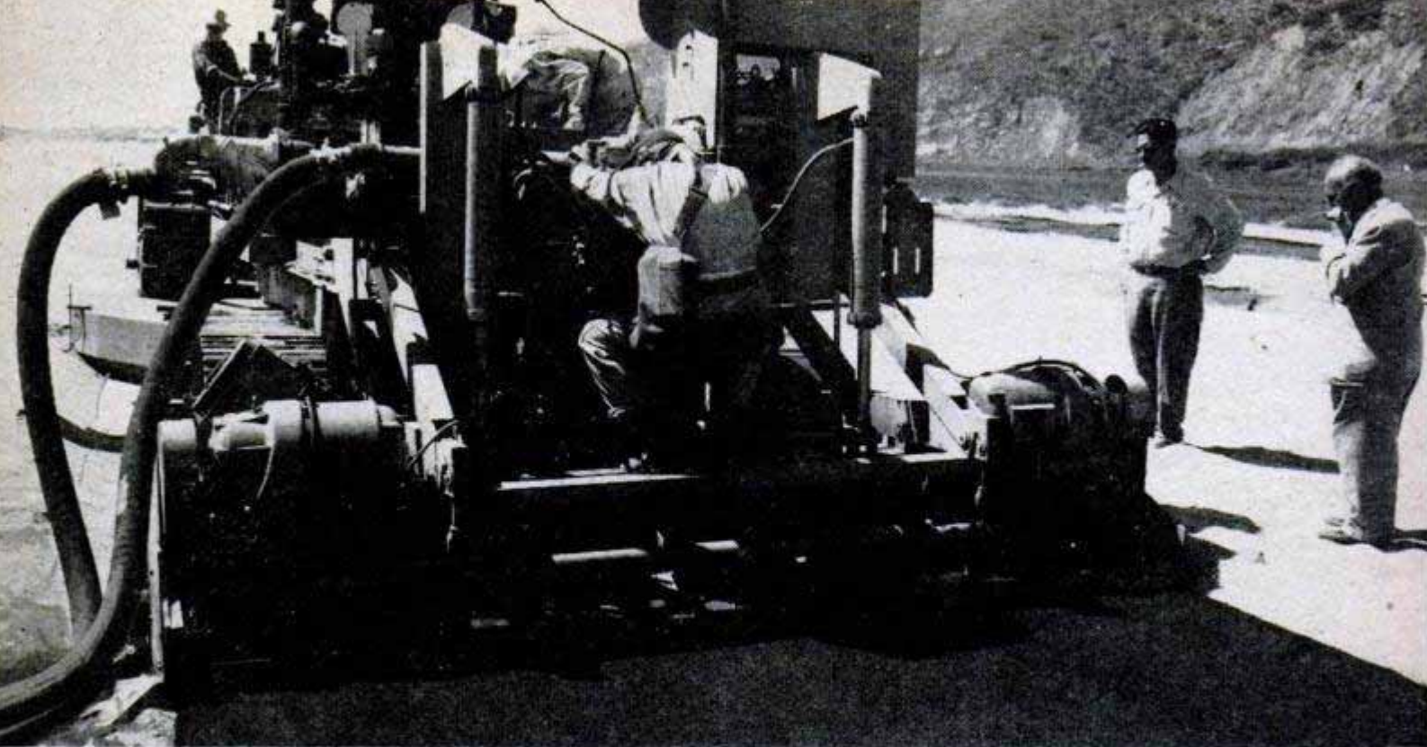
Sand mixed by this machine with a compound made partly from corncobs produces an asphalt-hard pavement
