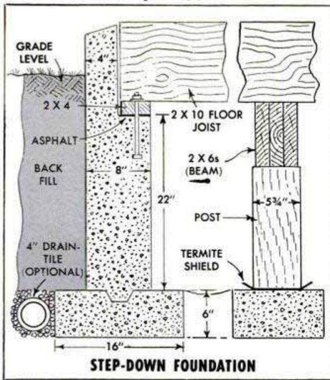
Each beam on which the floor joists rest is built up by spiking together three 2 x 6s on edge. As the joist plan indicates, two separate beams are required
