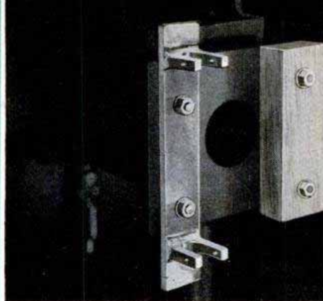
Special floating-rail base and hardwood spacer block are permanently installed
