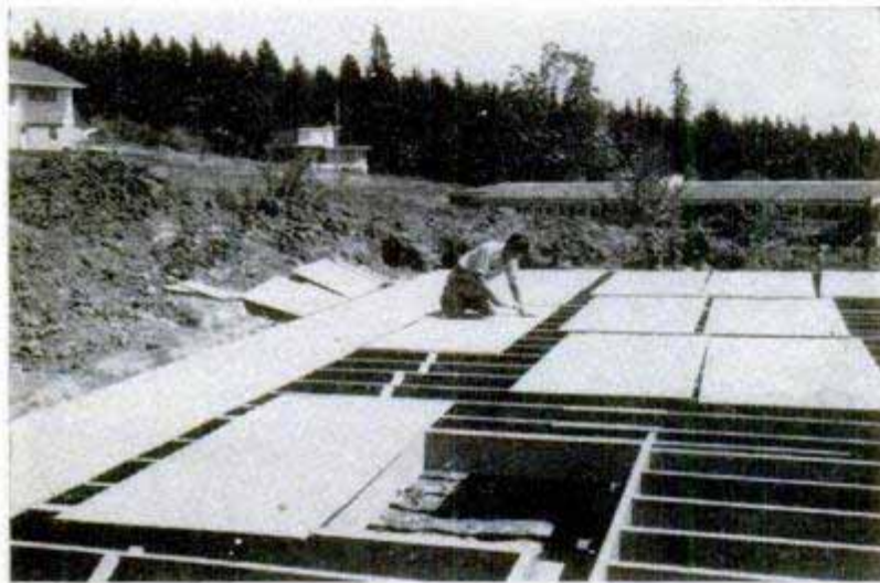
Above, architect Whelan, right, explains how trimmings from plywood subfloor are economically used later as truss gussets. Below, see how fast and easy the subfloor goes down. Plywood sheets previously used for forms are cleaned off and laid so that the joints are staggered four feet on the floor joists
