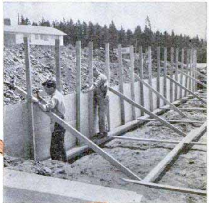
Above, this is the next step after pouring the footings. Here I am checking the inside corner of the anchor plates for the foundation forms. Below, using sheets of \frac{5}{8} -in. plywood, Norman Chapman and I are beginning to erect the forms along rear of house
