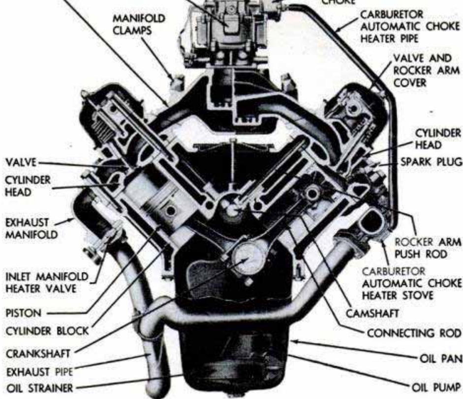
Cross-section view from the front of the new Studebaker 120-horsepower V-8 engine with overhead valves. This is the engine Floyd Clymer tested
