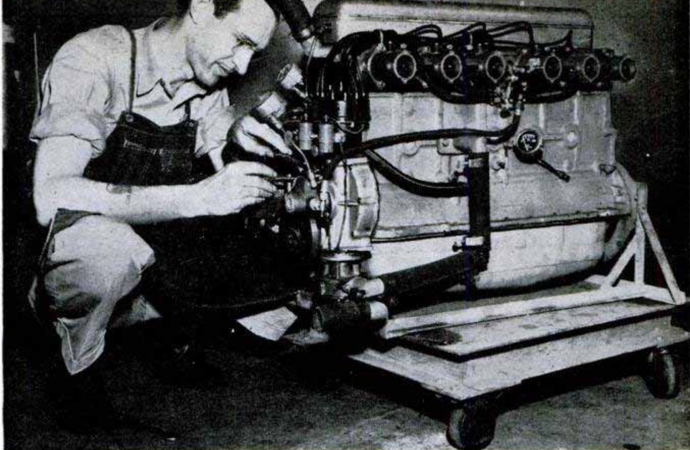
Rebuilt truck engine, fitted with overhead valves and fuel injection, will power the hot-rod entry this year
