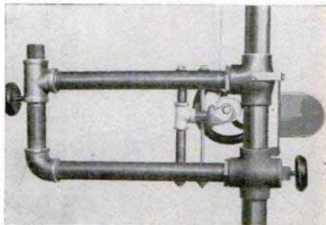
Weight of the camera and sliding arm are counterbalanced by spring sash balance on sliding members
