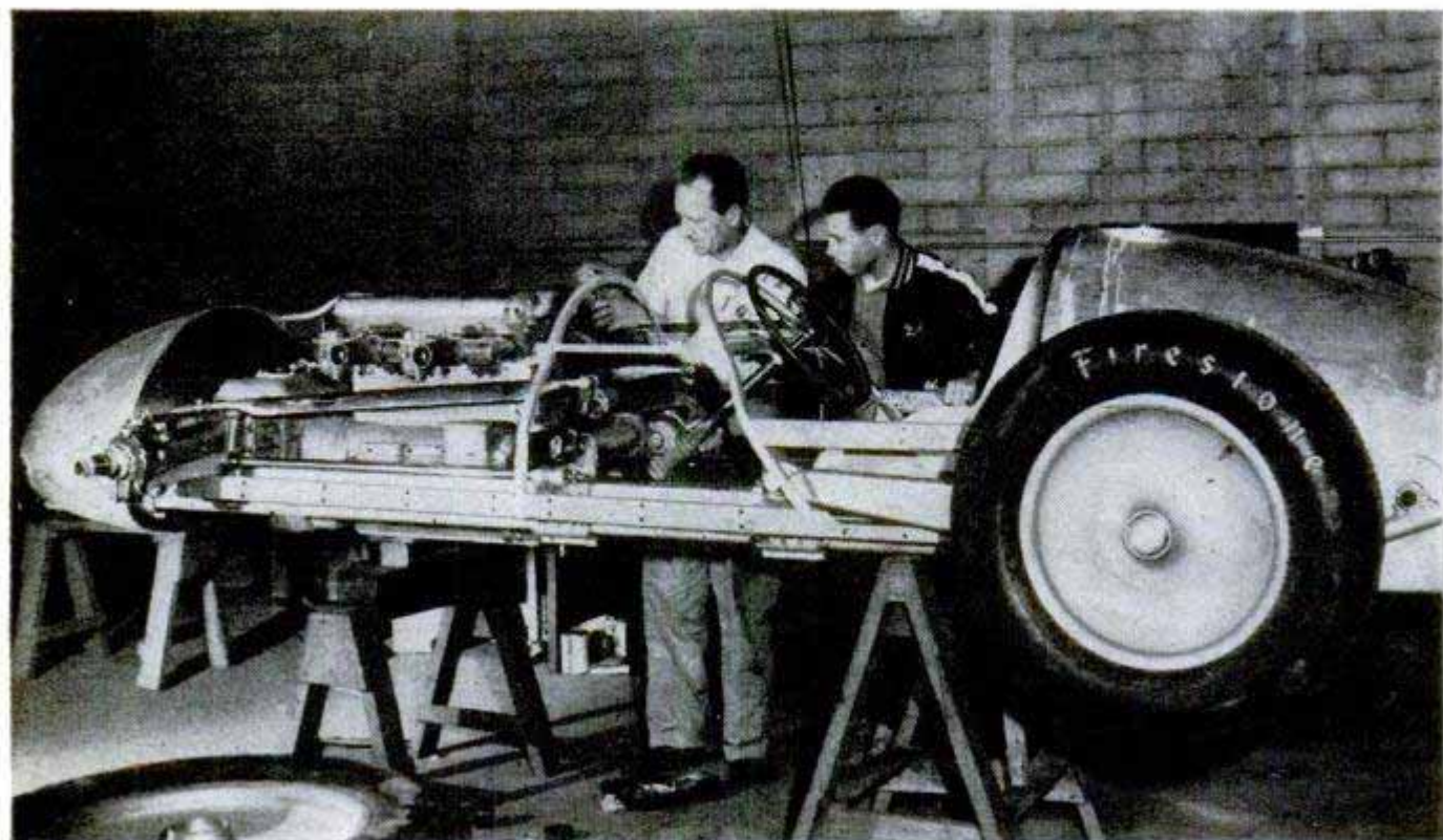
Front-wheel-drive car entered this year has aluminum and magnesium body parts which cut weight 350 pounds
