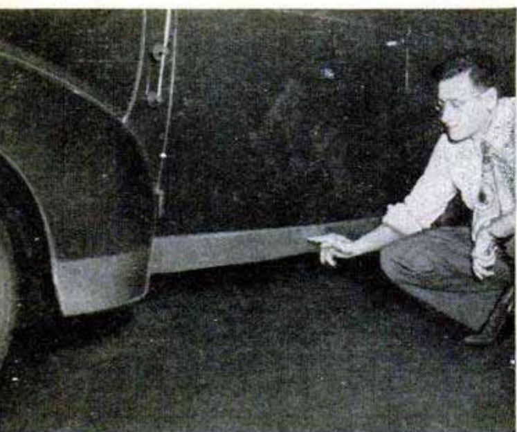
Where lower edges of fenders and body are extensively damaged by rust, full-length patch can be used
