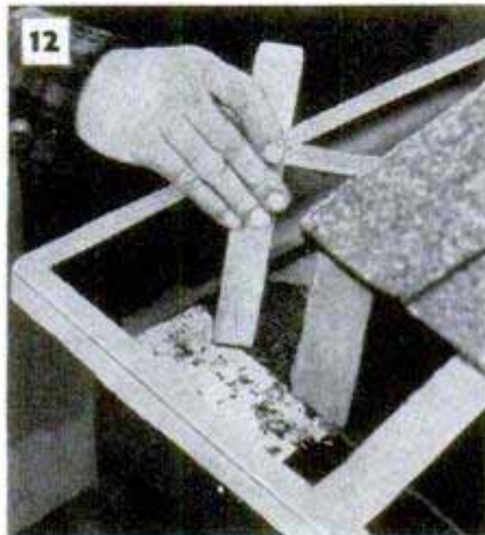
Small breaks in the metal can be closed by a fabric patch. First, apply compound with a brush as in Fig. 11, then press the canvas patch in place as in Fig. 12. Apply final coat over the fabric, including edges
