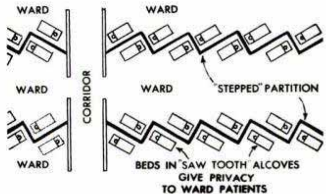
Diagram shows how beds are arranged in the modern hospital now nearing completion. The patient can see only the person directly across the room from him
