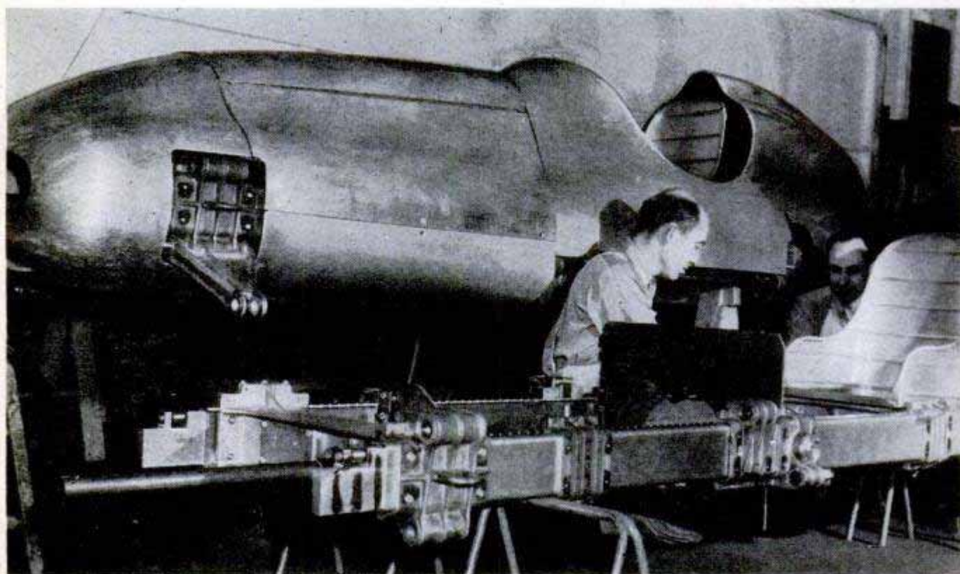
Working against time, car builders start frame of one of the last-minute entries for this year's race
