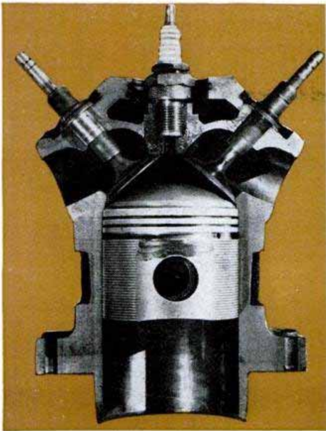
Cutaway cylinder from the 550-horsepower, supercharged Novi engine shows tiny combustion chamber
