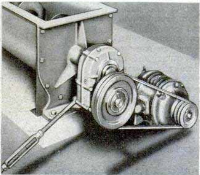
Dodge Mfg. Corp., Mishawaka, Ind. TORQUE-ARM REDUCER for output speeds from 115 to 330 r.p.m. is new item in the field of power-transmitting equipment. It is said to be the first shaft-mounted speed reducer designed for this speed range. The unit is attached to the shaft to be driven by means of two locking collars, one being placed on each side of the housing which is anchored to floor by a torque arm
