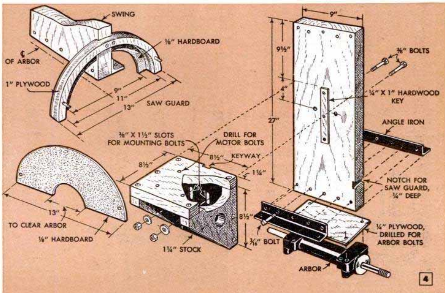
Details below show the construction of column and angle-iron pad on which the saw arbor is mounted
