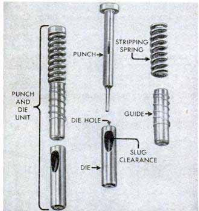
SINGLE DIE UNIT of the multiple hole-punching system is pictured above disassembled to show various parts. These are available to users as individual units for assembling setups to suit their own requirements. Dies are inserted in holes drilled in the plates
