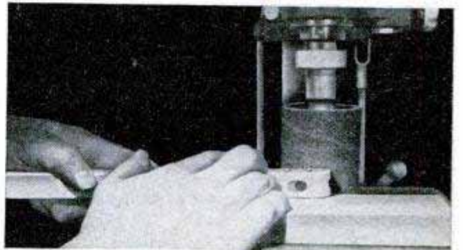
Ends of the handle are ground to shape on the drill press by attaching aluminum-oxide sleeve to drum
