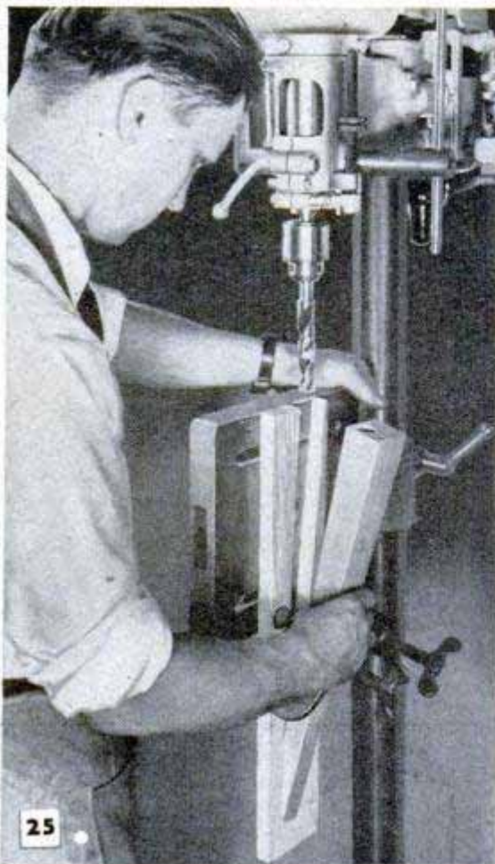
DOWEL HOLES OFTEN REQUIRE ANGULAR POSITIONING OF WORK BUT THE HOLE ITSELF IS ALWAYS AT RIGHT ANGLES TO SURFACE OF JOINT
