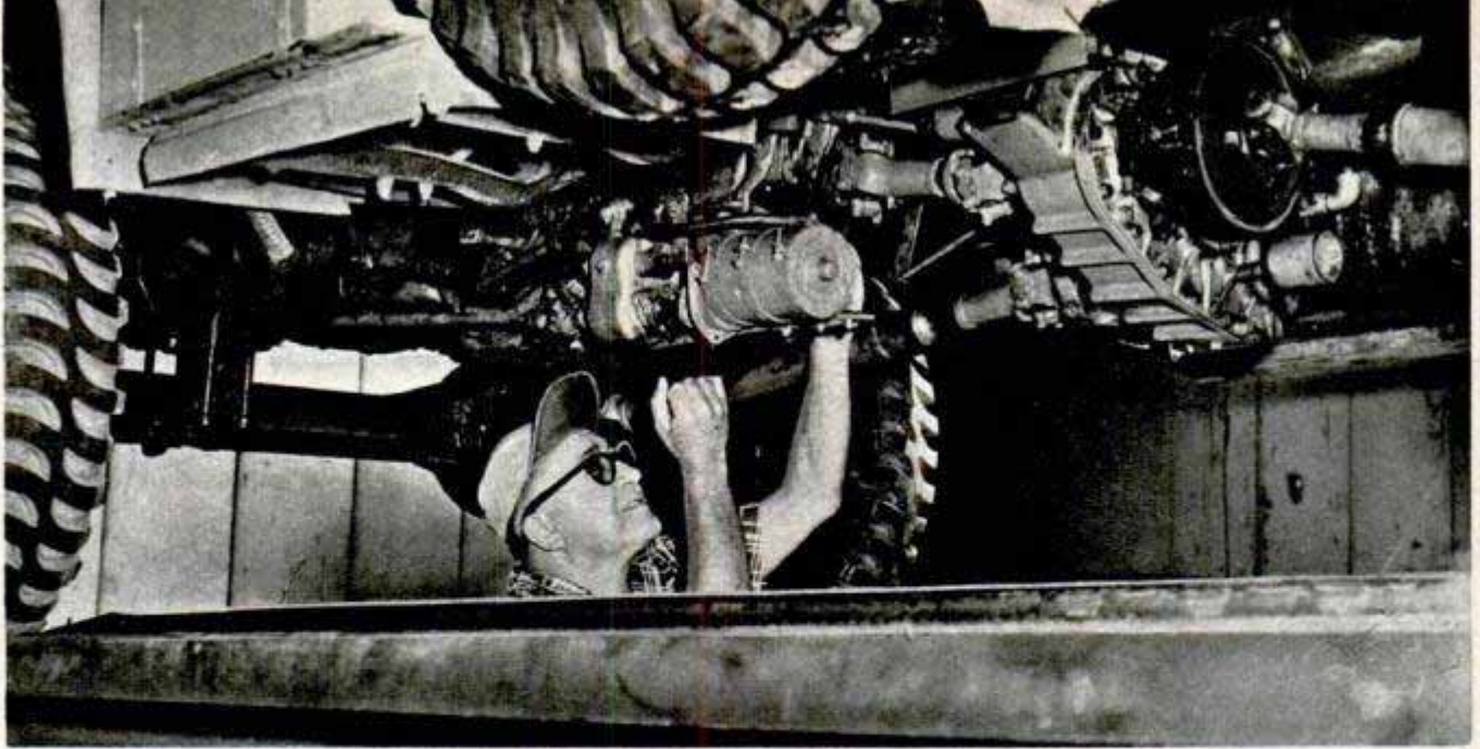
Sturdy two-speed transfer case from a GI armored truck replaces the original, lighter, single-speed job
