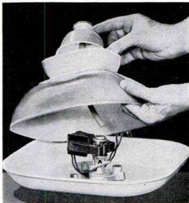
Simplest type of fountain is made from plastic bowls. Rubber tubing replaces pump-outlet tube and waterproof wiring is used to run line over side of pool
