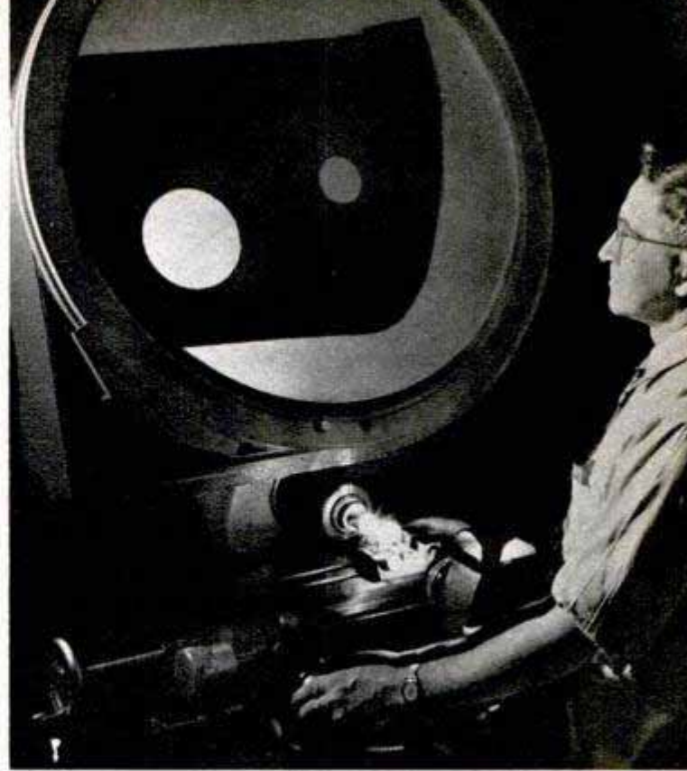
Silhouette of a tiny gauge is cast on a screen. Large outline is measured to check dimensions of the gauge
