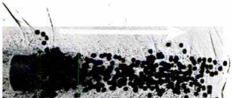
Old-type top wad could disarrange the shot. Below, new crimp-top shell has nothing in front of pellets
