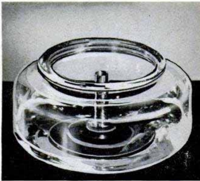
Ready-made fish bowl for use with recirculating pump is fitted with tube to carry wires for motor. Rubber gaskets seal joint between tubing and hole in glass
