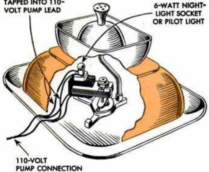
Night light wired in parallel to pump leads is used to illuminate fountain from inside. Even though waterproof wiring is used, connections must be out of water
