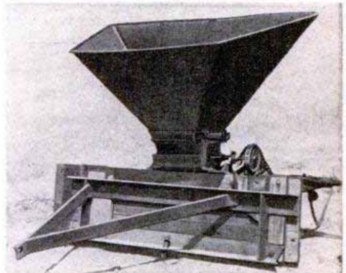
Endgate seeder is mounted on a special angle-iron frame for use with Ford tractor. Seeder usually comes equipped with wooden endgate of standard width
