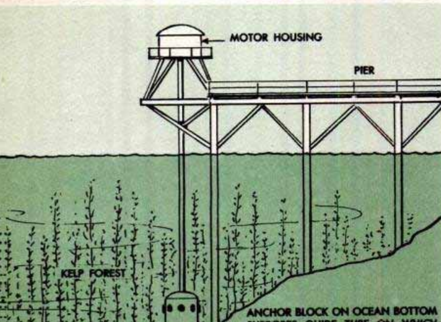
Below, left, sketch explains diving-bell operation. Right, structure above bell houses motor and compressor
