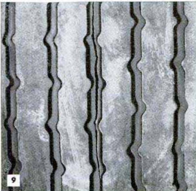
9 Continued overinflation results in tread breaks like that shown above. It is extremely hazardous to drive on crowded highways with tires in this condition
