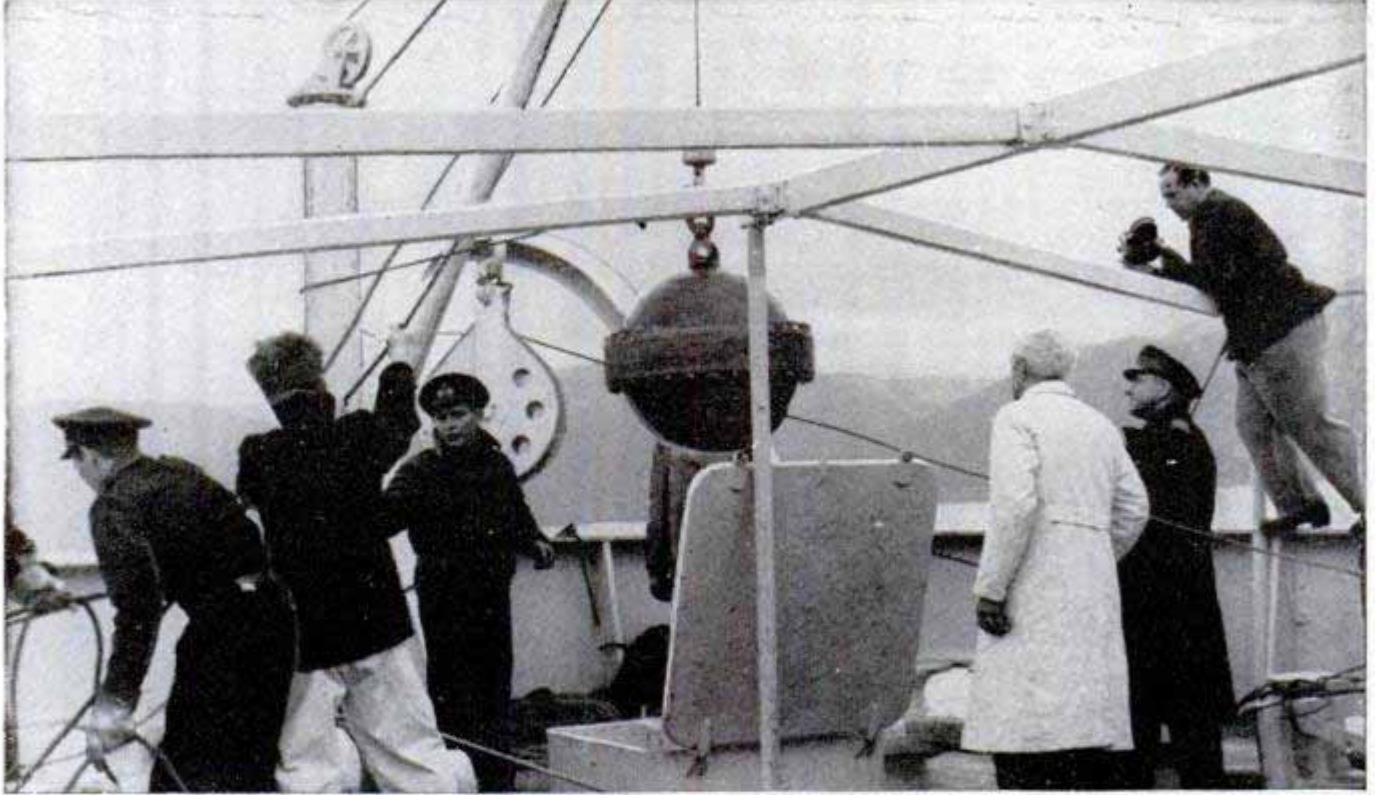
Preliminary to world cruise, bronze sphere built for magnetism studies is tested off Norway shore
