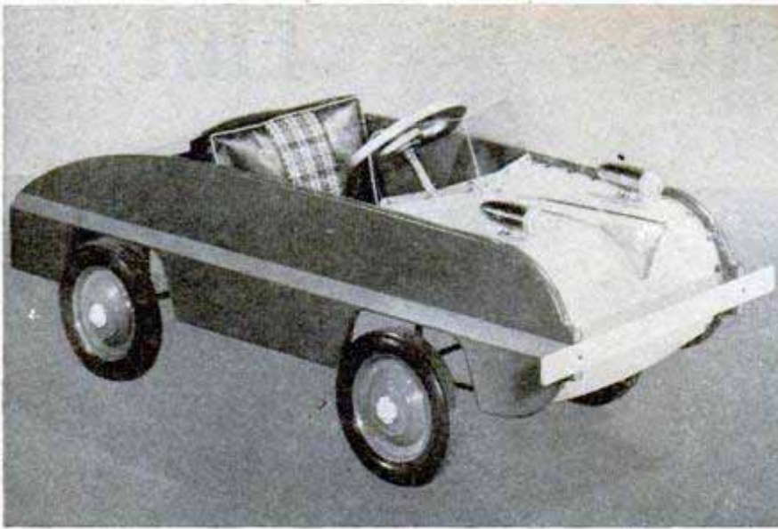
The wooden radiator ornament is screwed to the hood from the underside, while two roundheaded screws hold the flat-iron bumper in place
