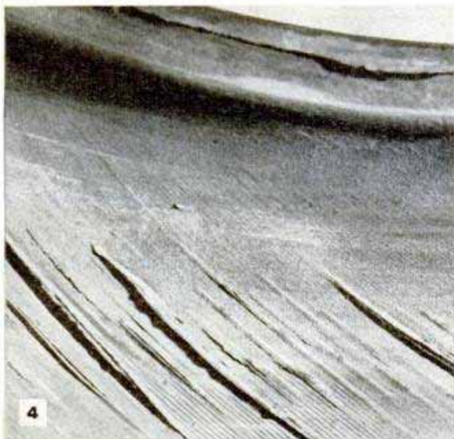
Flex breaks and ply separations in inner sidewalls often cause hazardous blowouts which can occur without warning. Note diagonal direction of the breaks
