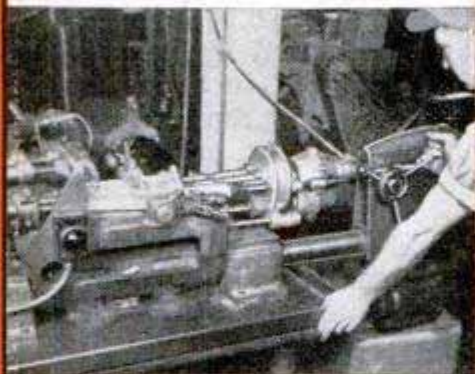
Drill press head used horizontally in special multiple drill-and-tap set-up. CRAFTSMAN is "tops" for versatility in dozens of such industrial set-ups!
