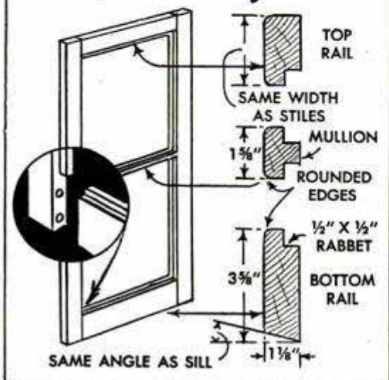
STORM SASH MUST HAVE 5/16" CLEARANCE ALL AROUND
