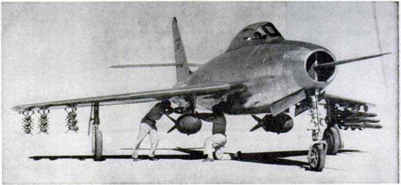
Armorer's attaching a 1000-pound bomb beneath swept wing of new Thunderjet. Below, underside view of 450-gallon fuel tanks
