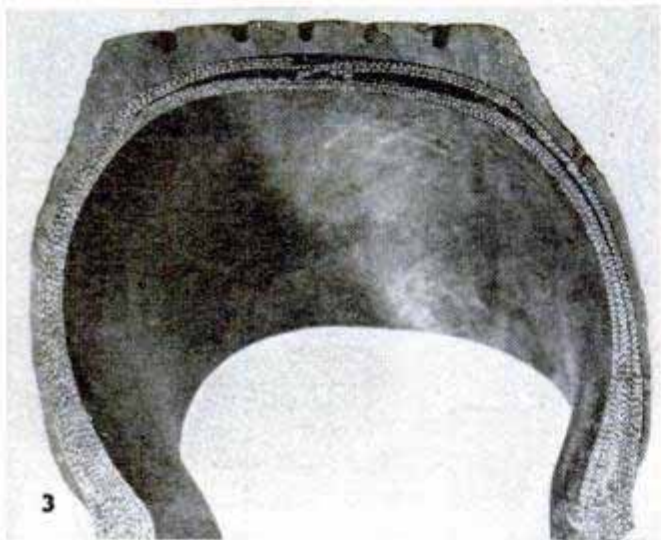
From the outside, you can't see ply separations and breaks in fabric that result from running tire under-inflated. Ply separations are costly to repair
