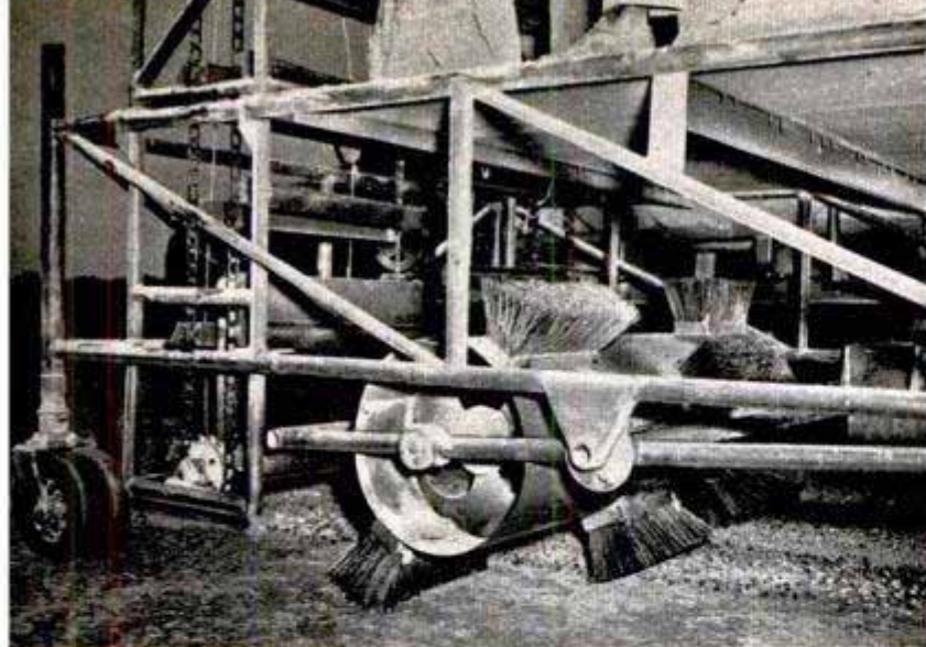
Powered by a small air-cooled engine, sweeper brushes push dried potatoes toward elevator buckets that lift them into truck
