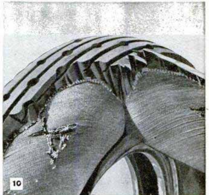
10 The inevitable end result of a tread break like that pictured at the left is a blowout like this. Sudden escape of the air has torn away a part of the tread
