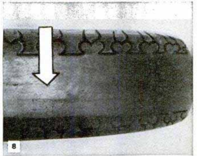
8 Overinflated tires gradually take on a high crown, because of abnormal wear and stretching of fabric. Arrow indicates point where wear usually is greatest
