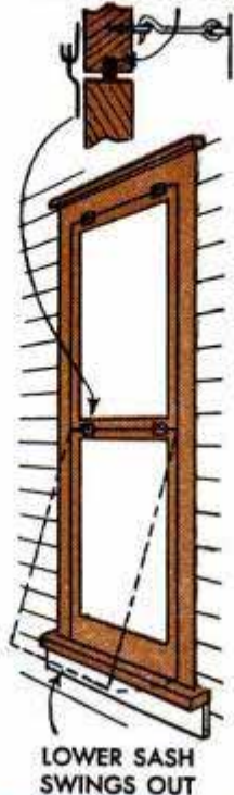
SPONGE-RUBBER STRIP IN GROOVE. SPRING-TYPE WEATHERSTRIP ALSO USED
