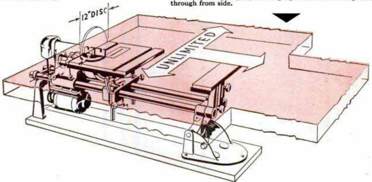
8-INCH CIRCULAR SAW. Using the sturdy extension table, you get an effective table area of 54" x 17"—twice that of the finest saws. Maximum blade to fence distance is 48"—the exact center of full-size plywood panels. Maximum depth of cut, 2-1/4". When table is tilted, crosscutting capacity extends from floor to ceiling.
