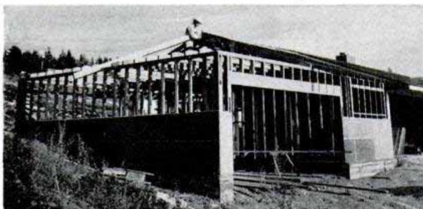
Above, setting end rafters for the two-car garage. To the right of the garage, the enclosed breezeway can be seen. Below, Riley uses a power saw to cut the plywood sheets into lengths of lapped siding
