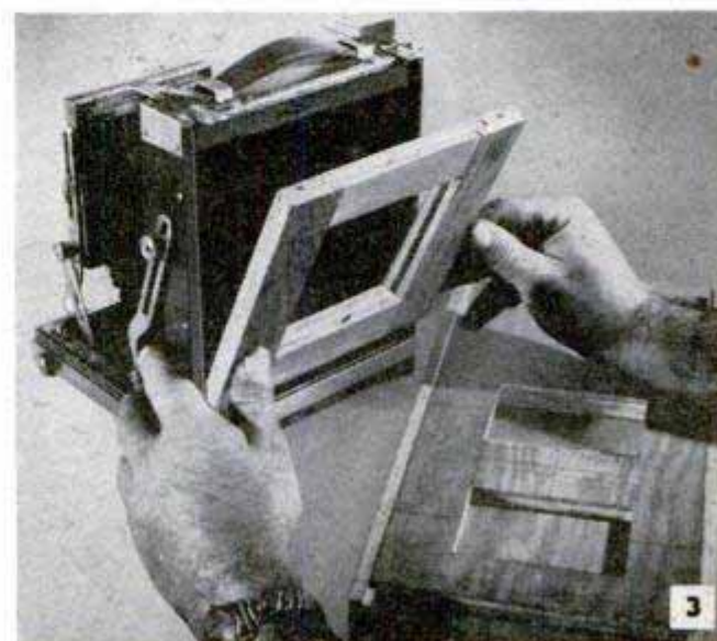
Above, the roll-film adapter in position for taking a horizontal picture. Panel has been moved down to bring film holder in position for exposure. Below, the camera-back adapter being checked for correct fit
