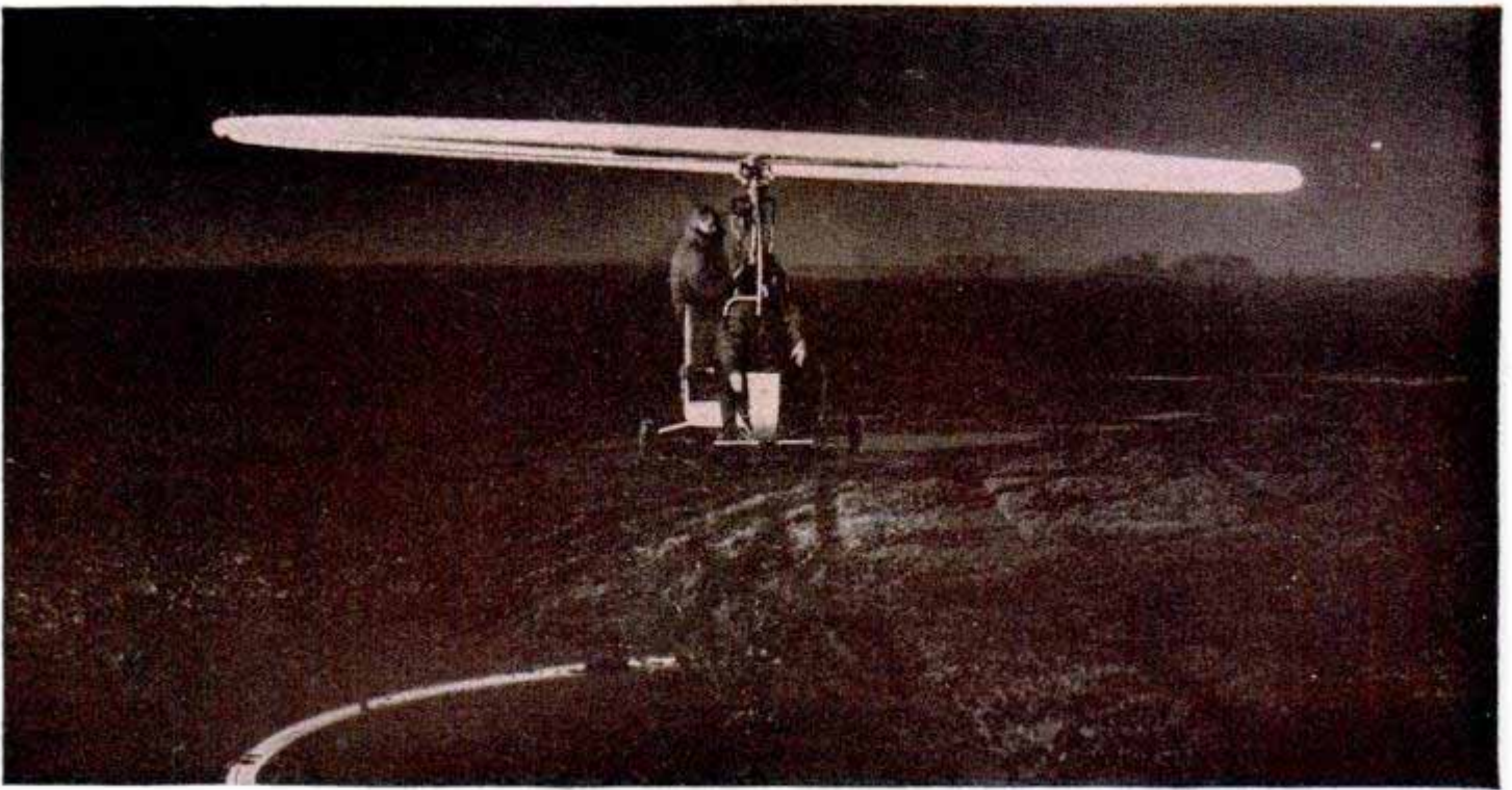
Running smoothly, the ramjets at a tip speed of 450 miles an hour produce a halo like this after dark
