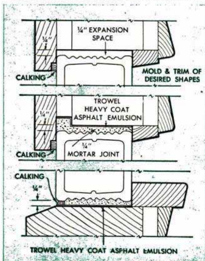
Above, lay the blocks in mortar joints troweled to a uniform thickness of ¼ in. Below, run a line of calking compound all around the completed panel
