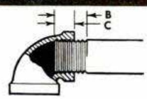
THREAD DATA FOR STANDARD-WEIGHT PIPE
