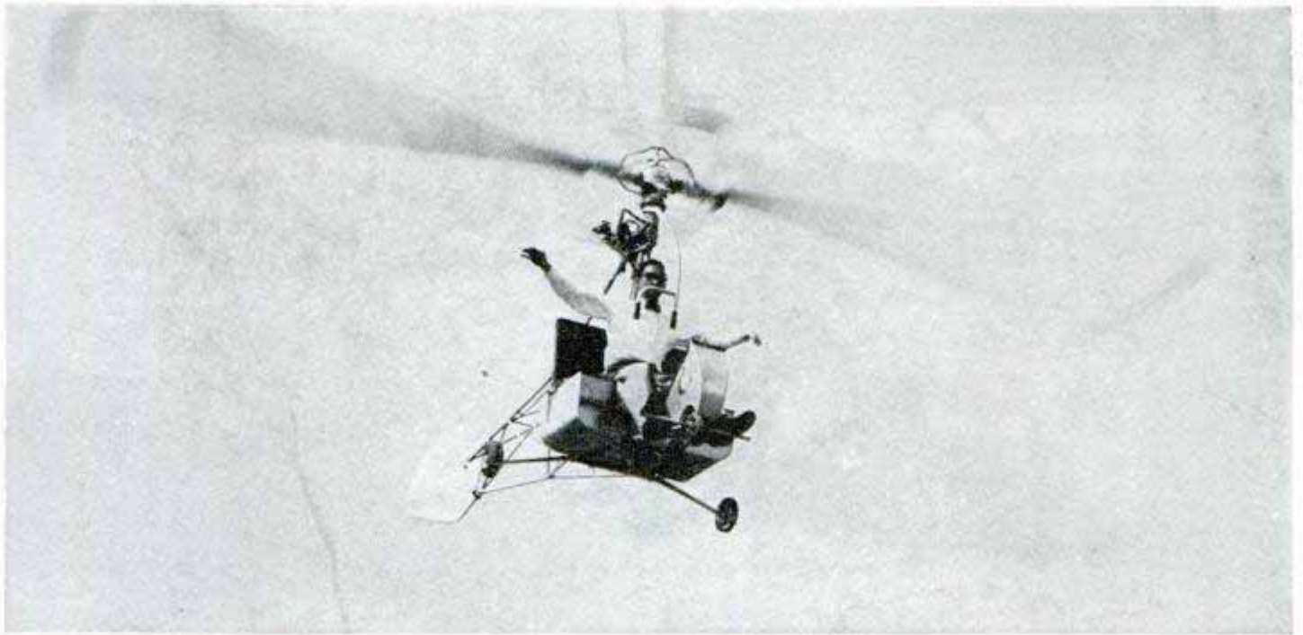
Stable control system of "Hornet" permits "hands off" flight in any attitude
