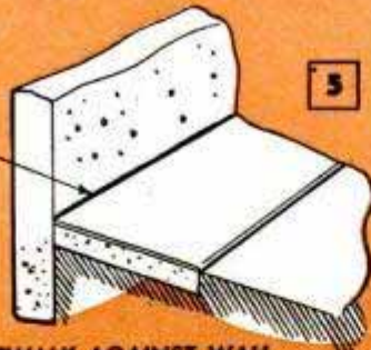
SIDEWALK AGAINST WALL SHOULD BE SEALED AT JOINT AND HAVE A DRAINAGE SLOPE
