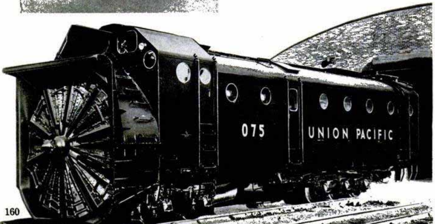
Below, here's the new Lima-Hamilton diesel rotary snowplow that will get its final test this spring over the track between Ashton and West Yellowstone
