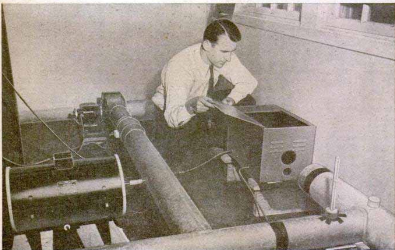
Above, complex apparatus measures tiny amounts of sulphur dioxide in the air. Below, transmissometer in box sends a beam of light into the large smog-filled pipe and measures the visibility loss caused by the vapor
