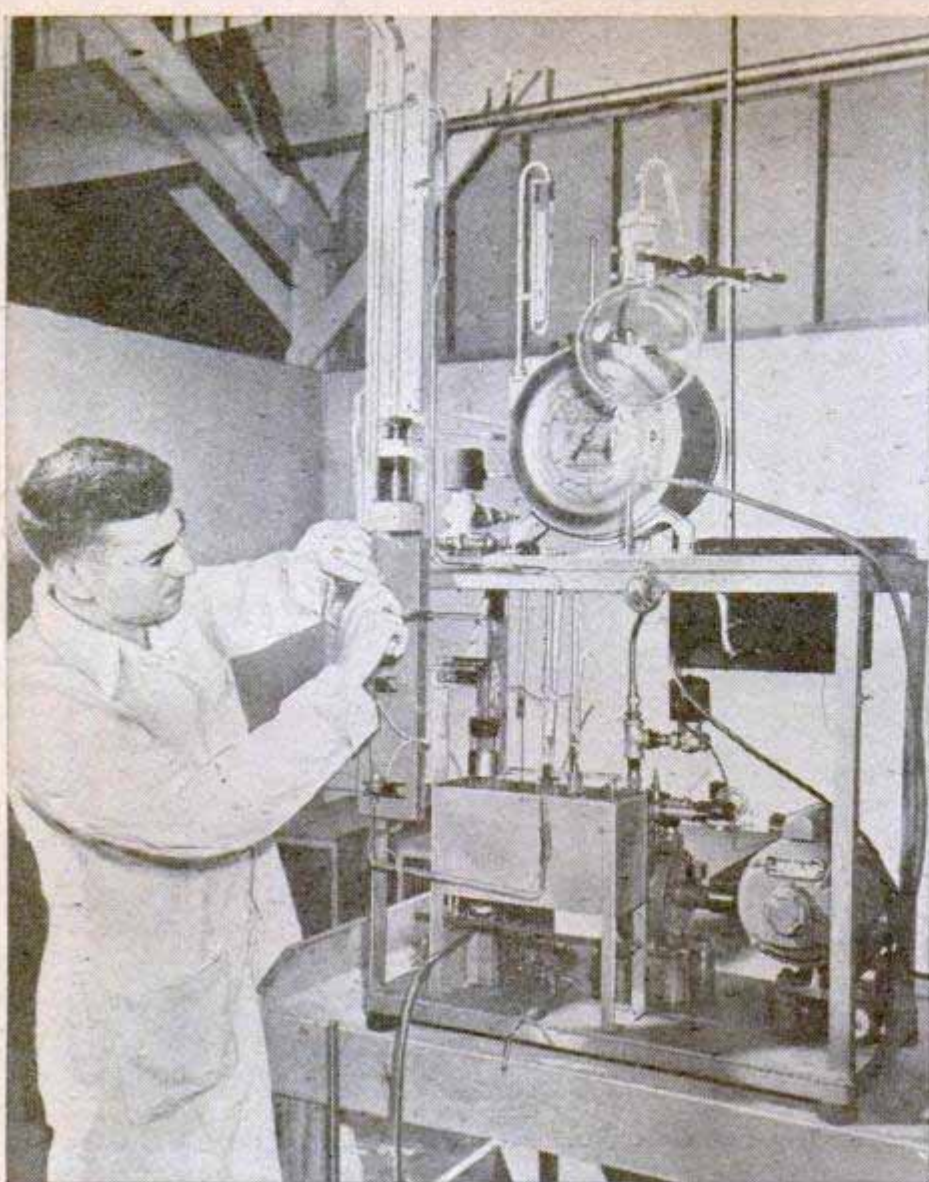
Above, complex apparatus measures tiny amounts of sulphur dioxide in the air. Below, transmissometer in box sends a beam of light into the large smog-filled pipe and measures the visibility loss caused by the vapor
