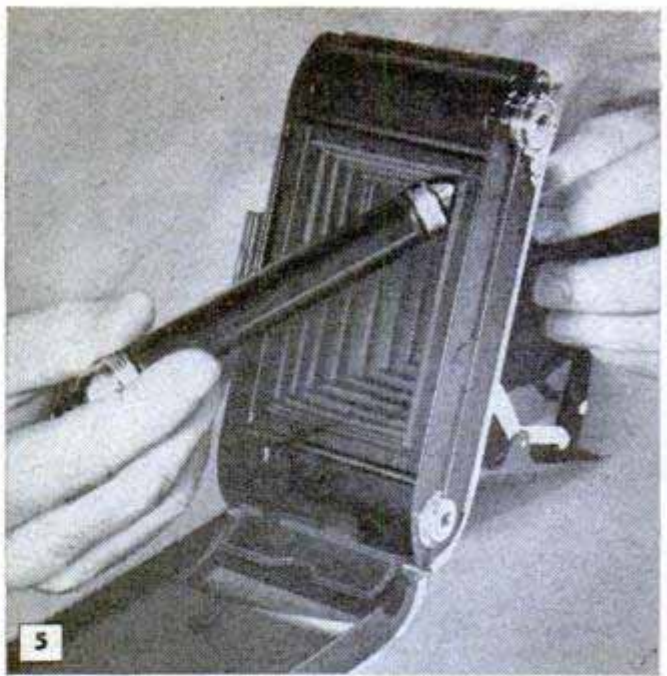
5 To locate a light leak, press a flashlight against inside corners of bellows and inspect outer surface
