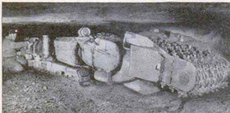
Below, the Joy Continuous Miner has its control panel about 14 feet behind the nose. Left, the Joy machine in operation underground. Notice its low profile
